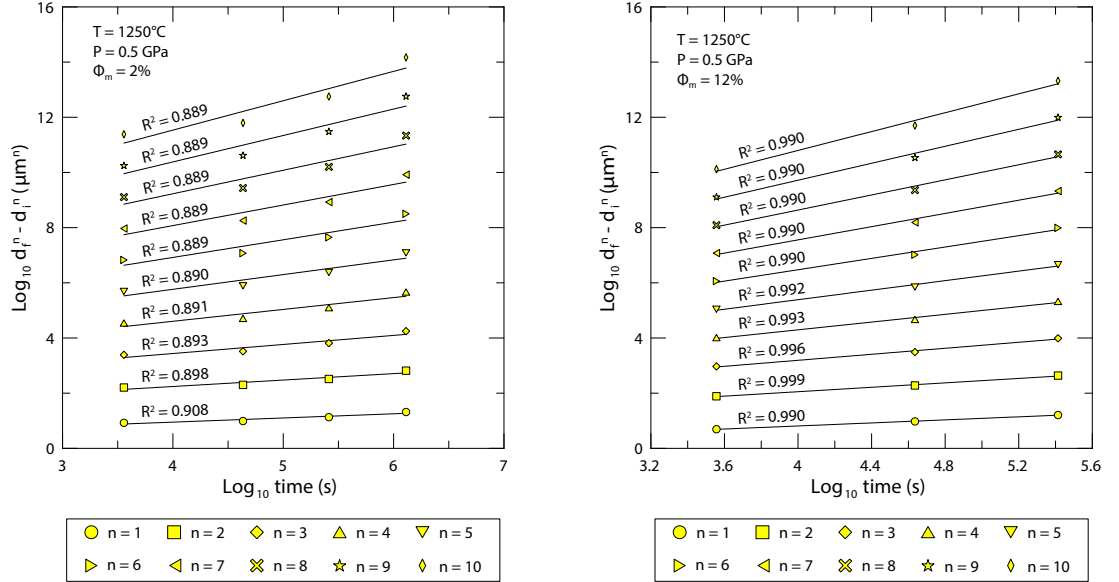
(c) Static grain growth experiments containing 2 wt. % melt at 0.5 GPa and 1250 °C. Data indicate that n = 1 .
