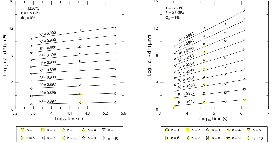
(a) Nominally melt-free static grain growth experiments at 0.5 GPa and 1250 °C. Data indicate that n = 10 .
