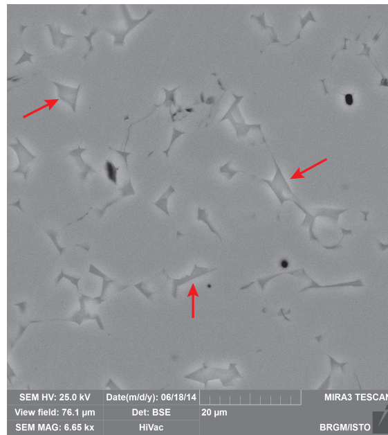
(c) Sample 12PR-PC2 containing 12 wt. % melt
