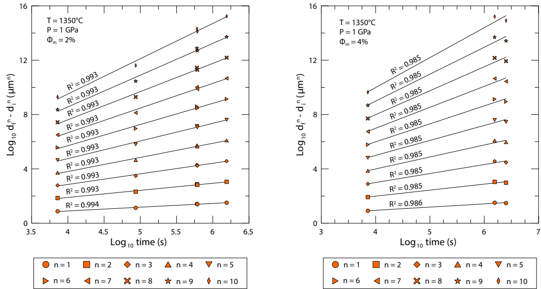
(a) Static grain growth experiments containing 2 wt melt at 1 GPa and 1350 °C. Data indicate that n = 1 .
