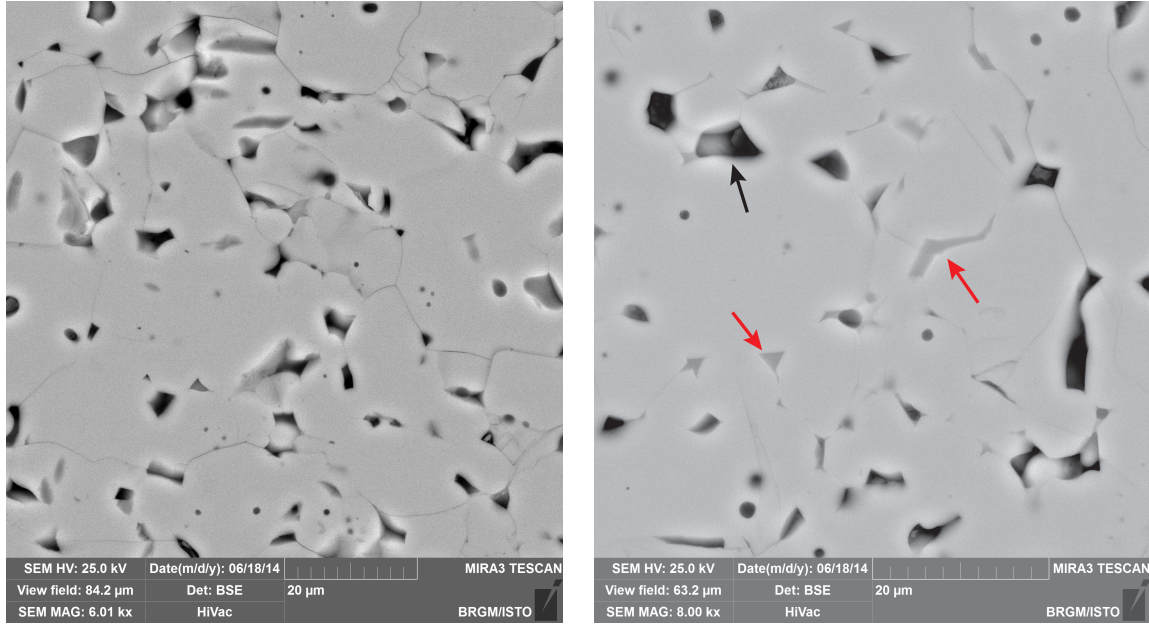
(a) Sample 0PR-PC2 containing 0 wt. % melt
