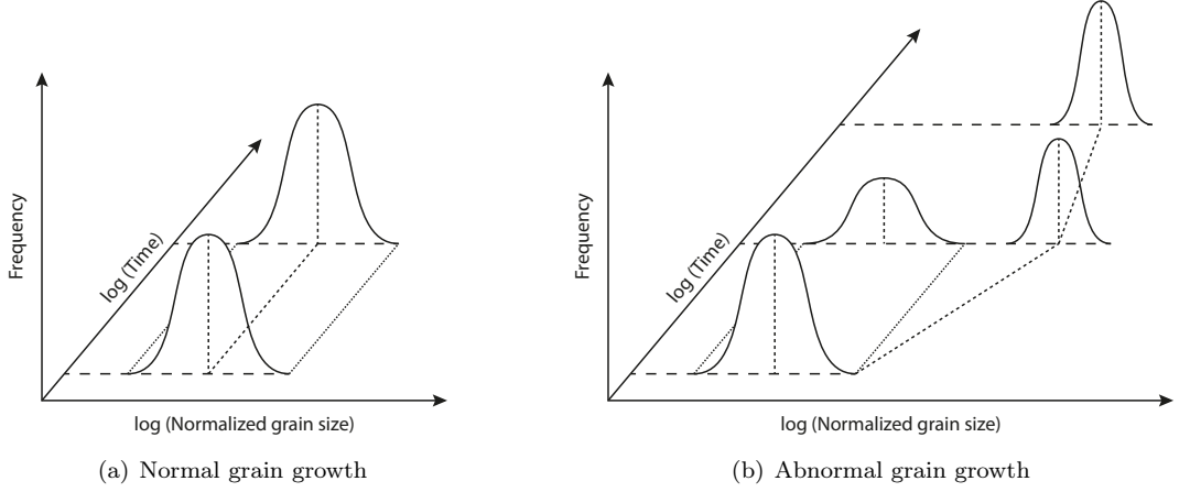
Figure 1 – Schematic evolution of the grain size distribution (after Detert (1978)).
