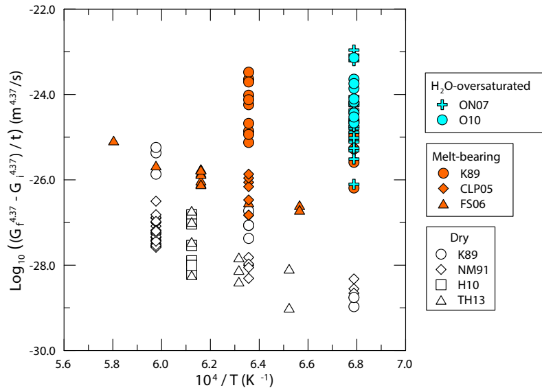
Figure 2 – Olivine grain growth rates vs. absolute reciprocal temperature for previously published experimental grain growth of olivine aggregates. Experiments are from Karato (1989) (K89), Nichols and Mackwell (1991) (NM91), Hiraga et al. (2010) (H10) and Tasaka and Hiraga (2013) (TH13), Cabane et al. (2005) (CLP05), Faul and Scott (2006) (FS06), Ohuchi and Nakamura (2007a,b) (ON07), Ohuchi et al. (2010) (O10).
