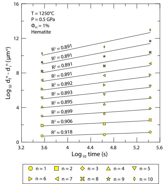
(f) Static grain growth experiments containing 1 wt. % melt at 0.5 GPa and 1250 °C (hematite experiment). Data indicate that n = 1 .
