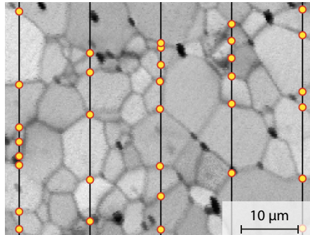
Figure B.1 – Example of grain size measurement by the linear intercept method (image quality map from EBSD measurements on sample OPR-PC5 from my study). Black lines are randomly drawn on the studied section and grain boundaries are highlighted (yellow symbols) for grain counting. The average grain size is determined by dividing the line length by the number of intersected grains.
