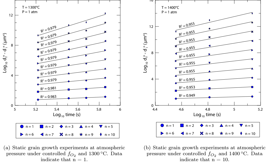
Figure A.2 – Dataset from (Karato, 1989) showing different grain size exponent values ( n = 1 to 10) as a function of time. Although the same starting material was used at 1300 and 1400 °C, n = 1 at 1300 °C and n = 10 at 1400 °C.
