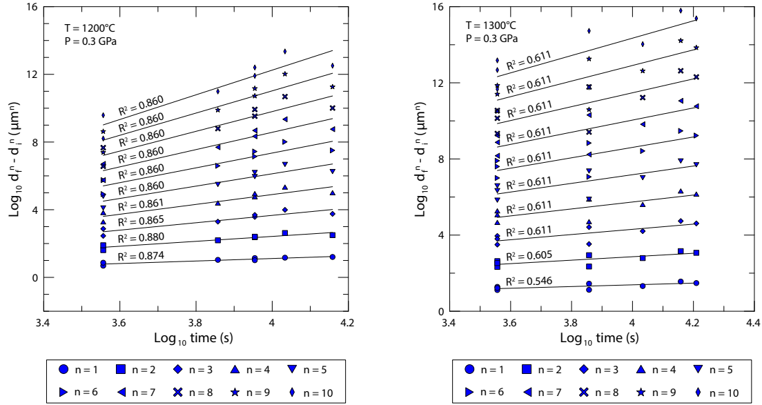
(a) Static grain growth experiments at 0.3 GPa and 1200 °C. Data indicate that n = 2 .
