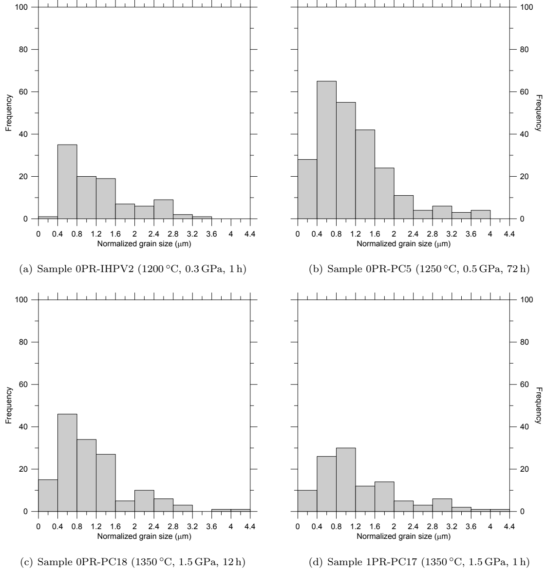
Figure C.2 – Typical grain size distributions. Normalized grain size correspond to the measured grain size divided by the median size.
