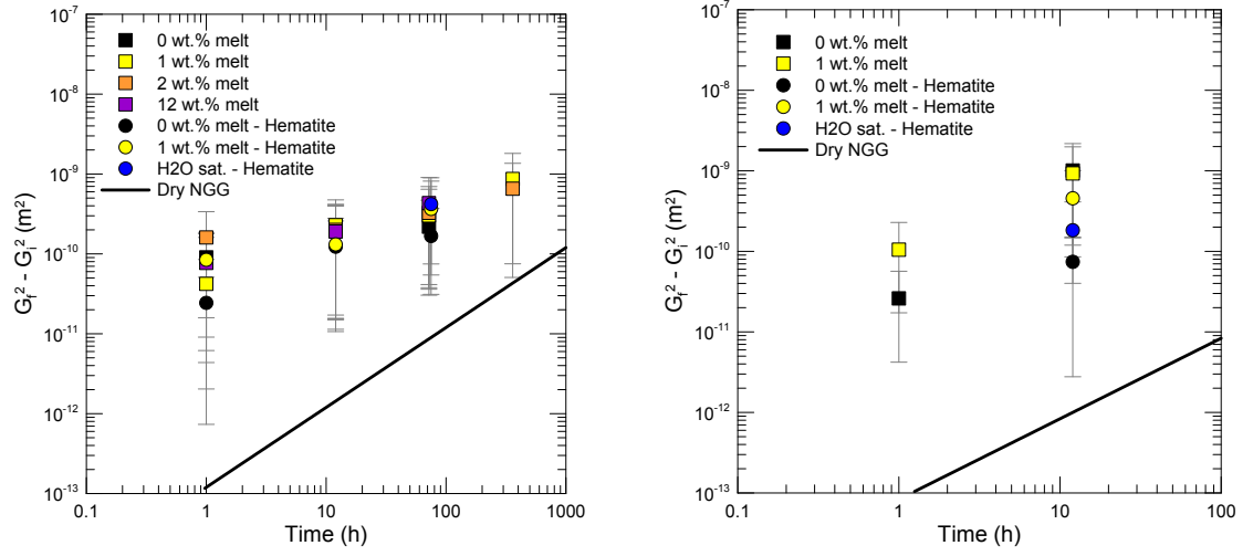
(a) T = 1250\text{ }^{\circ}\text{C} - P = 0.5\text{ GPa}
