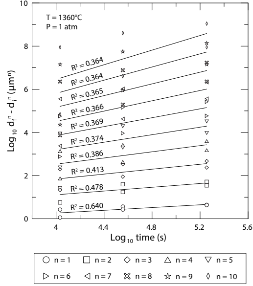
Figure A.4 – Dataset from (Hiraga et al., 2010) showing different grain size exponent values ( n = 1 to 10 ) as a function of time. The static grain growth experiment was conducted at atmospheric pressure and 1360^\circ\text{C} , yielding n = 1 .
