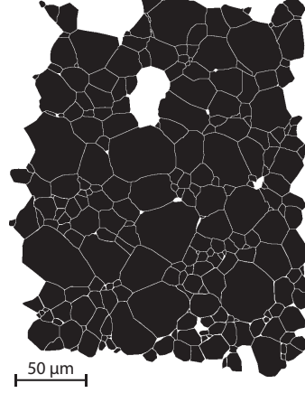
Figure B.2 – Example of grain size measurement by the area method (sample 0PR-PC5 from my study). Grains are outlined to obtain the area of each grain, which is then converted into grain sizes from the conventional derivation of 2\sqrt{S/\pi} by assuming each grain to be a perfect sphere.
