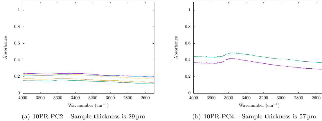
Figure C.1 – FTIR spectra.
