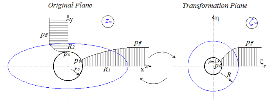
Fig. 2-2: The distribution of pore pressure in the original plane and in the transformation plane
