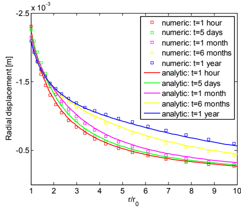
a) Radial displacement in the horizontal direction
