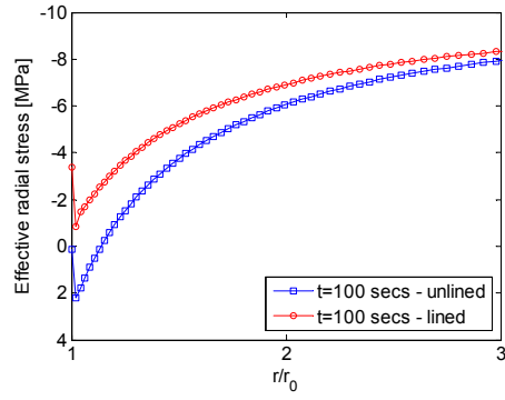
Effective radial stress in the horizontal direction
