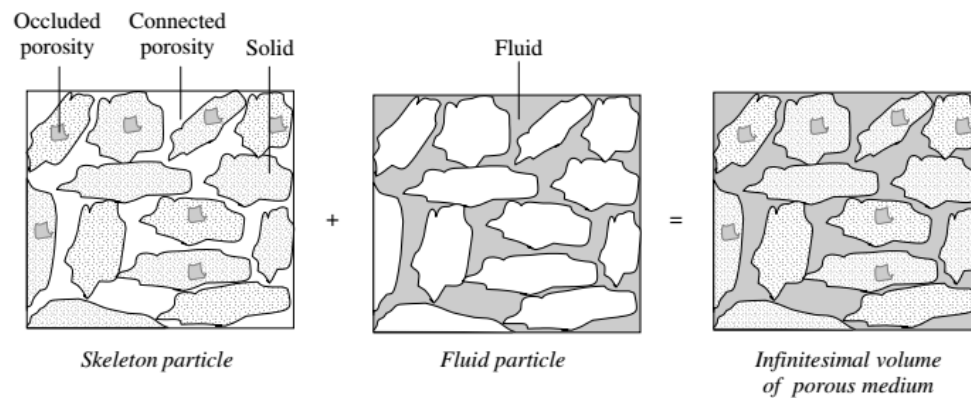
Fig. 1-3: A schematic of the porous media idealization (Coussy 2004)
