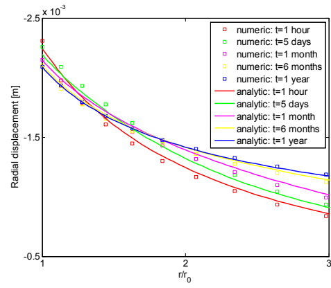
b) Radial displacement in the horizontal direction (zoom around the tunnel)
