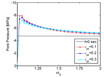
a) Pore pressure in the horizontal direction
