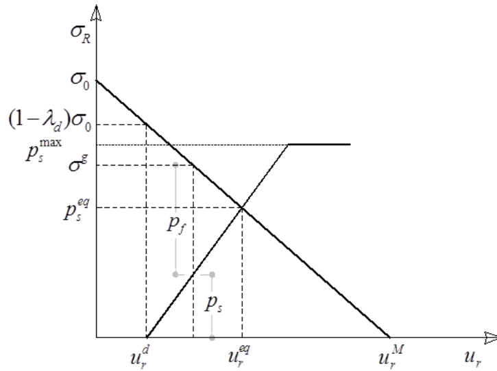
Fig.4-7: Relation between the stress on the tunnel wall and the stress applied to the extrados of the support after the support installation
