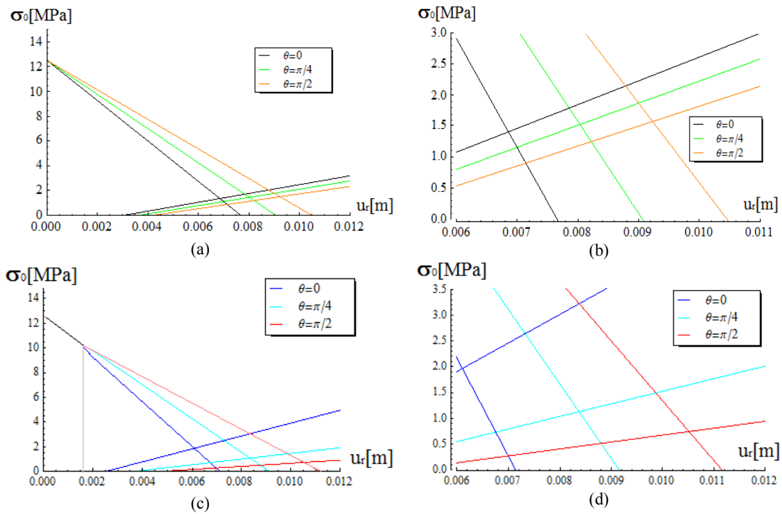
Fig. 4-9: Ground characteristic curve and support characteristic curve for three points in the perimeters of tunnel (corresponding to directions \theta=0, \pi/4 and \pi/2 ) for: a) un-drained case; b) un-drained case with zoom around the equilibrium state; c) drained case; d) drained case with zoom around the equilibrium state
