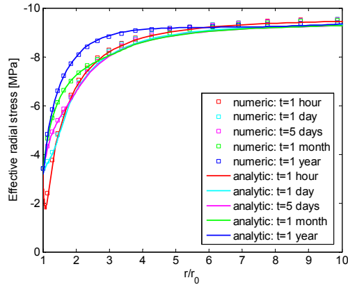
a) Effective radial stress in the horizontal direction
