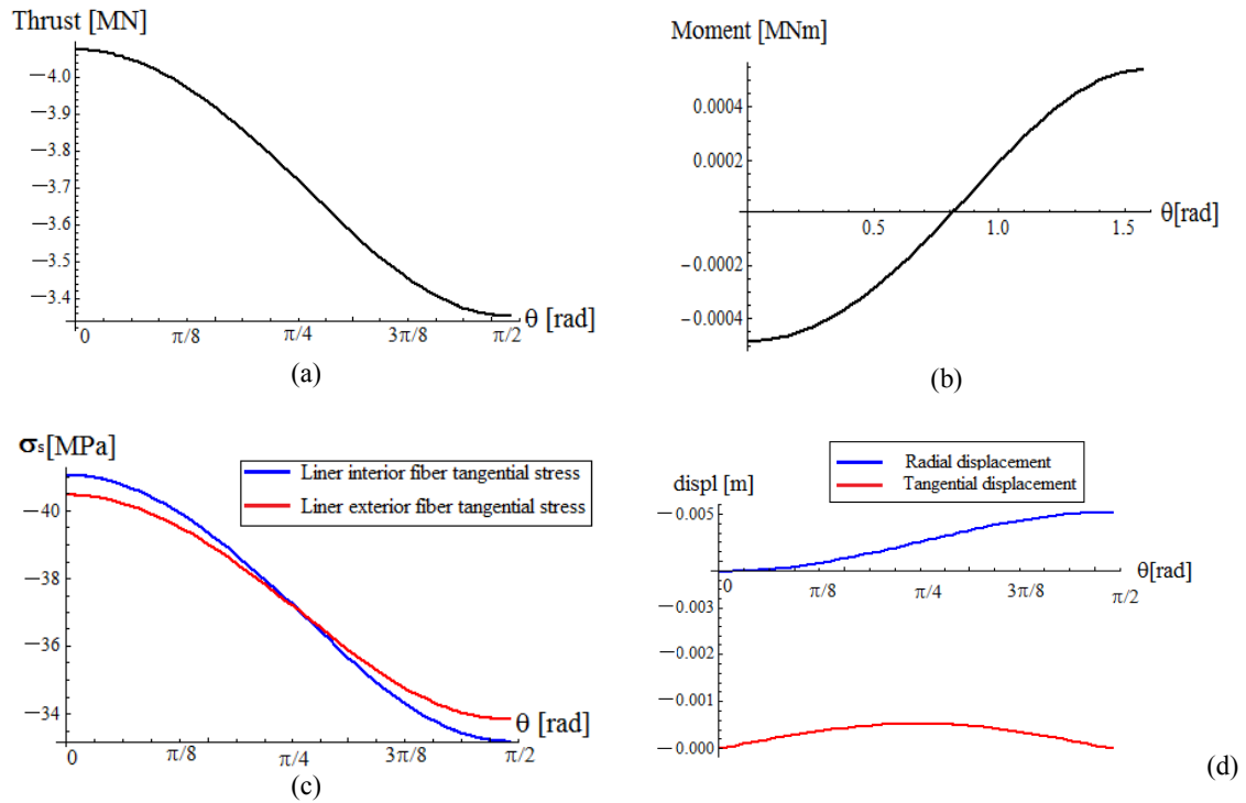
Fig. 4-10: The thrust, moment, stresses and the displacement of the liner in the case of \lambda_d=0.4 and un-drained condition
