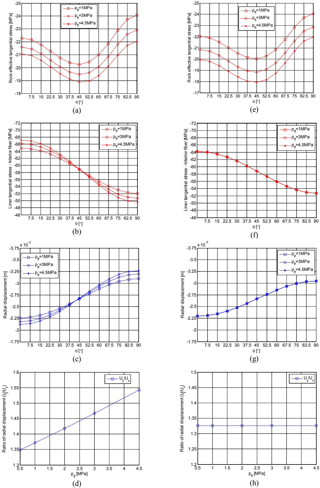
Fig. 2-19: Influence of the far-field pore pressure ( p_{ff} ) on the rock effective tangential stress, the liner tangential stress, the radial displacement, and the ratio of radial displacement respectively at the circumference of tunnel which is excavated: in drained rock (a, b, c, d) or in saturated rock with uniform pore pressure (e, f, g, h).
