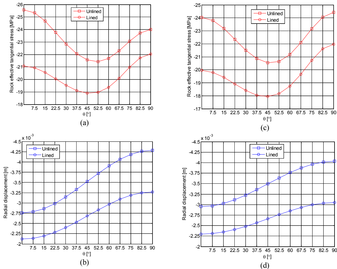
Fig. 2-24: Rock effective tangential stress and radial displacement on the rock-liner contact whether there is liner or not
