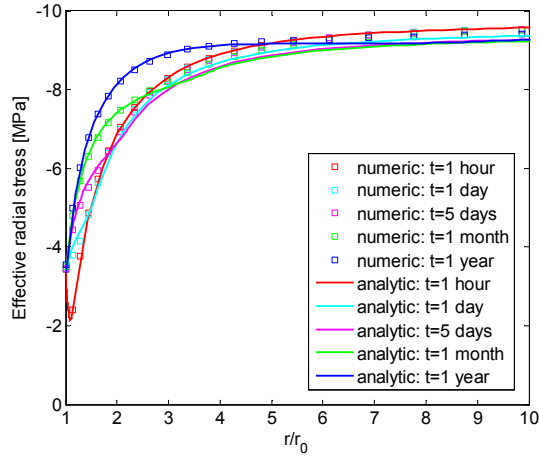
a) Effective radial stress in the horizontal direction
