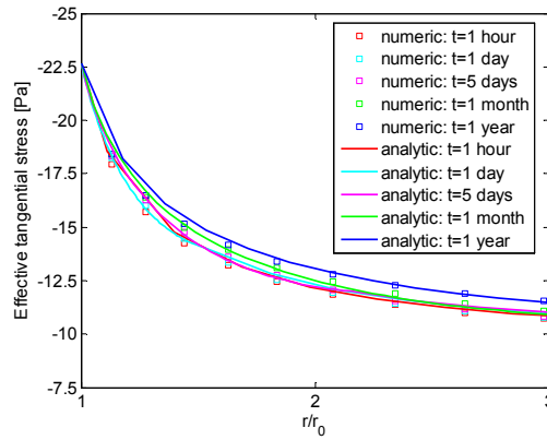
(d) Effective tangential stress in the vertical direction (zoom around the tunnel)
