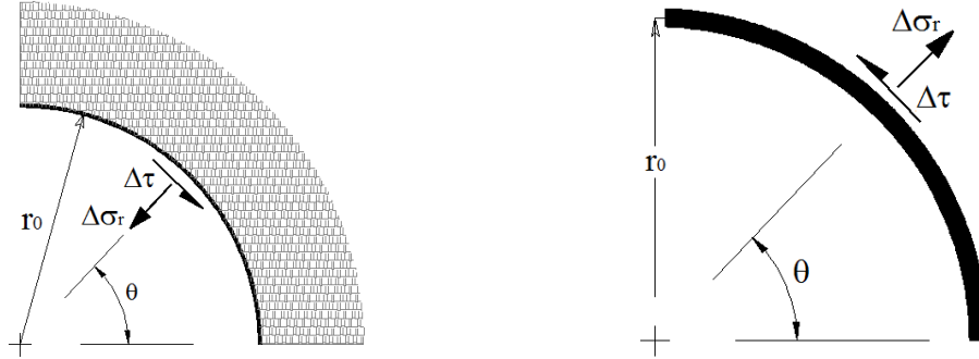
Fig. 2-5: Stresses at the rock-liner interface
