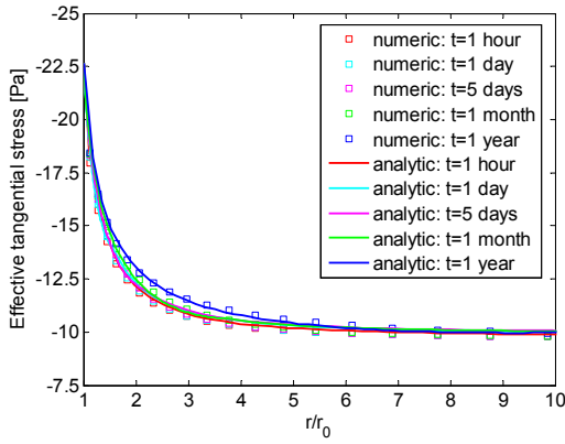
(c) Effective tangential stress in the vertical direction
