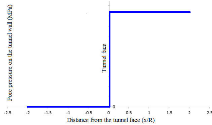
Fig. 4-6: Evolution of the pore pressure in function of distance from the study section to the tunnel face
