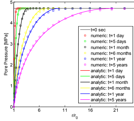
Fig. 3-5: Distribution of pore pressure in the radial direction (case of saturated rock with isotropic hydraulic properties k_a=k_x/k_y=1 ).
