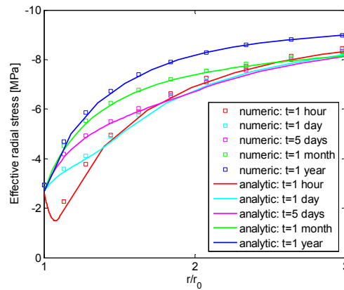
(c) Effective radial stress in the vertical direction (zoom around the tunnel)
