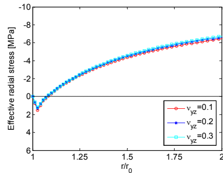
d) Effective radial stress in the vertical direction
