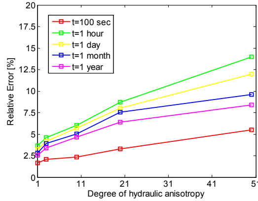
c) Relative error of effective tangential stress (case r_0=1.5 m)
