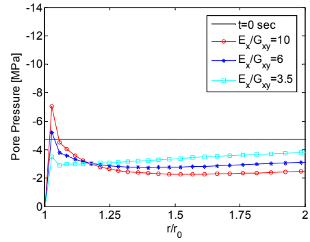
b) Pore pressure in the vertical direction
