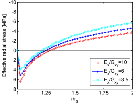
c) Effective radial stress in the horizontal direction
