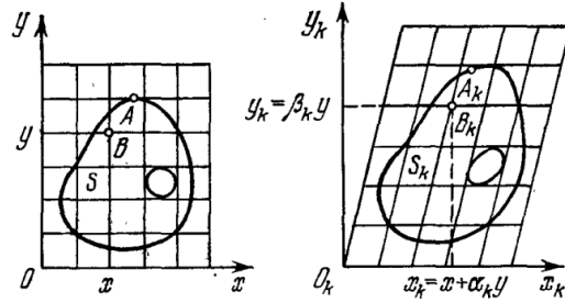
Fig. 1-9: Geometric representation of an affine transformation (Lekhnitskii, 1963)
