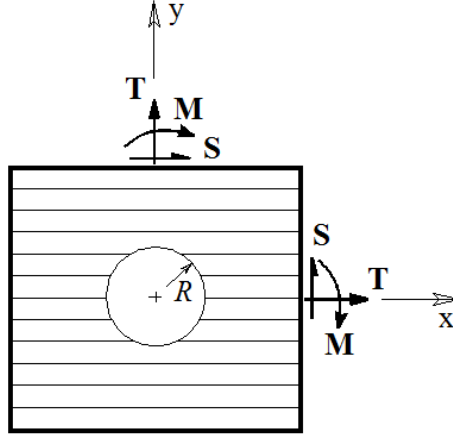
Fig. 1-11: The excavation in the anisotropic medium- Green and Zerna's solution
