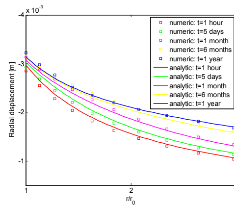
d) Radial displacement in the vertical direction (zoom around the tunnel)
