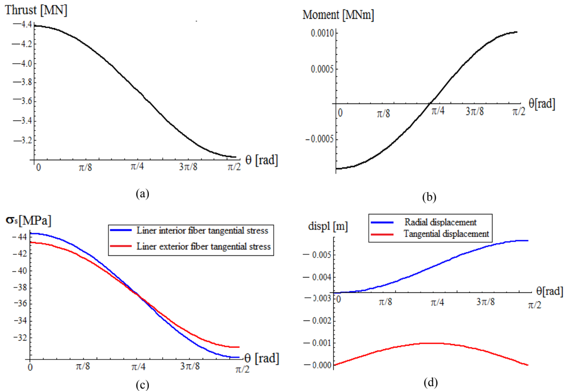
Fig. 4-11: The thrust, moment, stresses and the displacement of the liner in the case of \lambda_d=0.4 and drained condition in steady state
