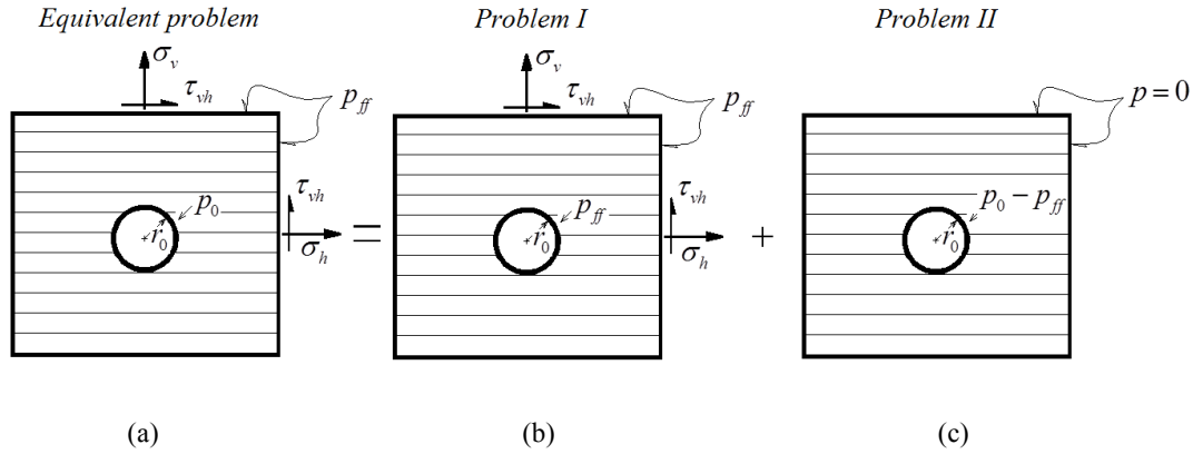
Fig. 3-2: Decomposition of the equivalent problem into two sub-problems (which is similar as one presented in chapter 2, see Fig. 2.6): problem I and problem II. In this latter problem the transient flow of groundwater is considered.
