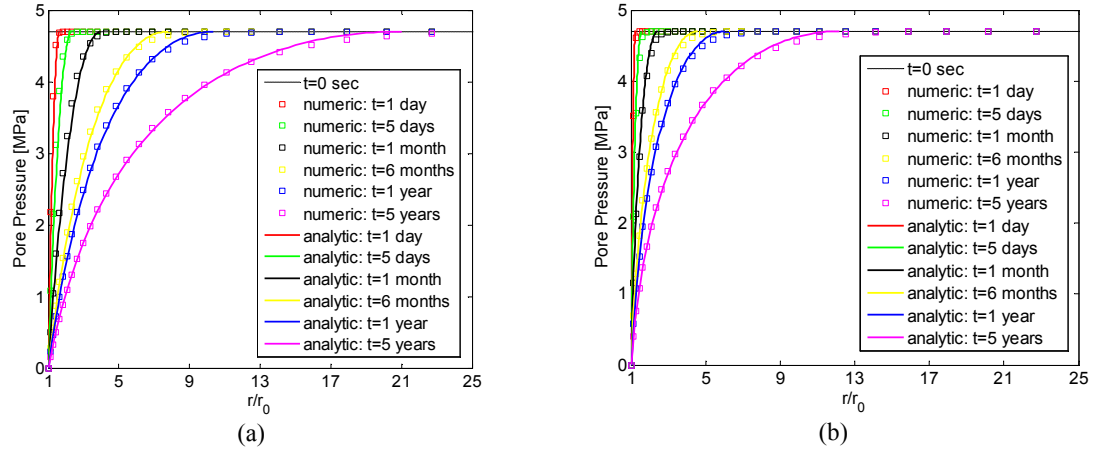
Fig. 3-9: Distribution of pore pressure: (a) in the horizontal direction, (b) in the vertical direction (case of saturated rock with anisotropic hydraulic properties k_a = k_x/k_y = 3 ).
