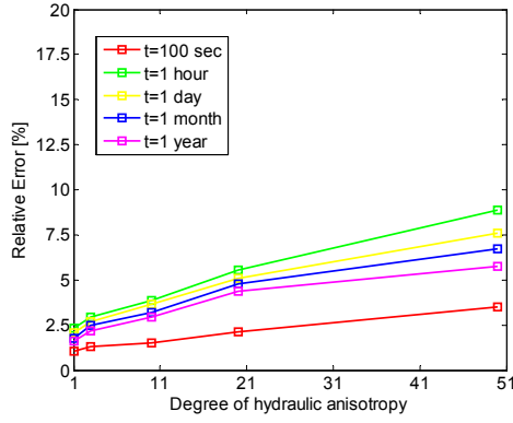
a) Relative error of effective tangential stress (case r_0=0.5 m)
