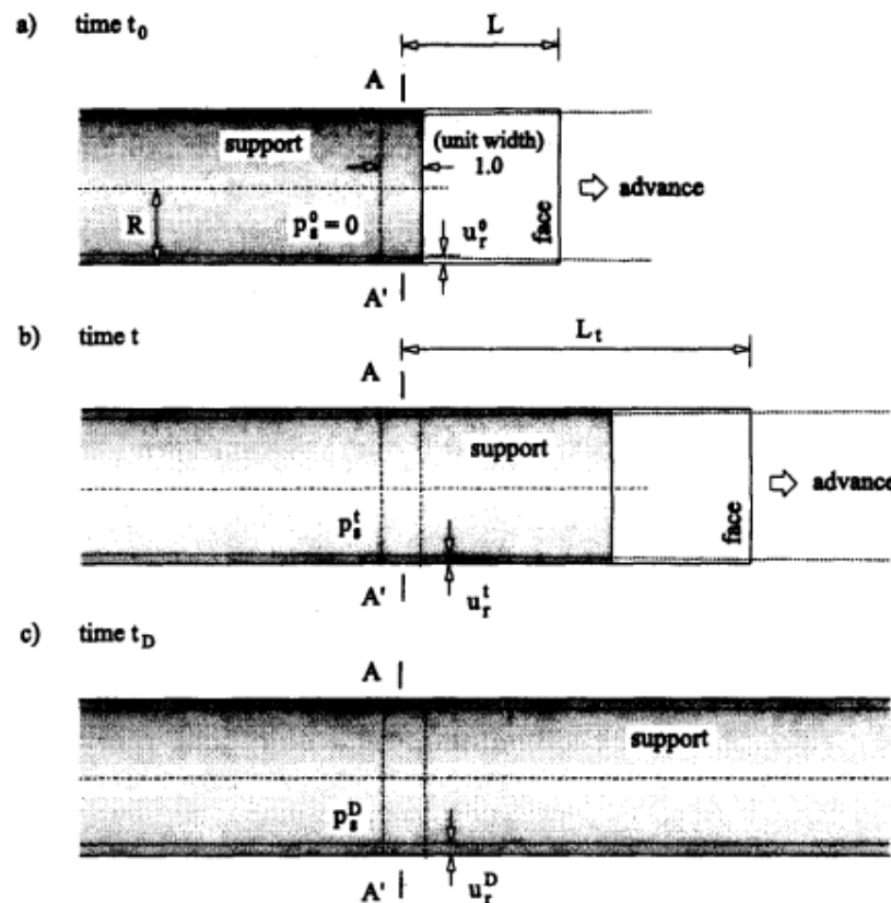
Fig. 4-2: Loading of the support at section A-A' due to progressive advance of the tunnel face (Carranza-Torres and Fairhurst, 2000)
