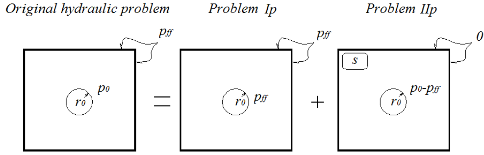
Fig. 3-1: Decomposition the original purely hydraulic diffusion in the transient state into two sub-problems
