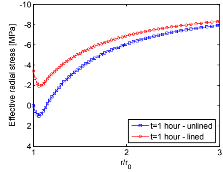
Effective radial stress in the horizontal direction
