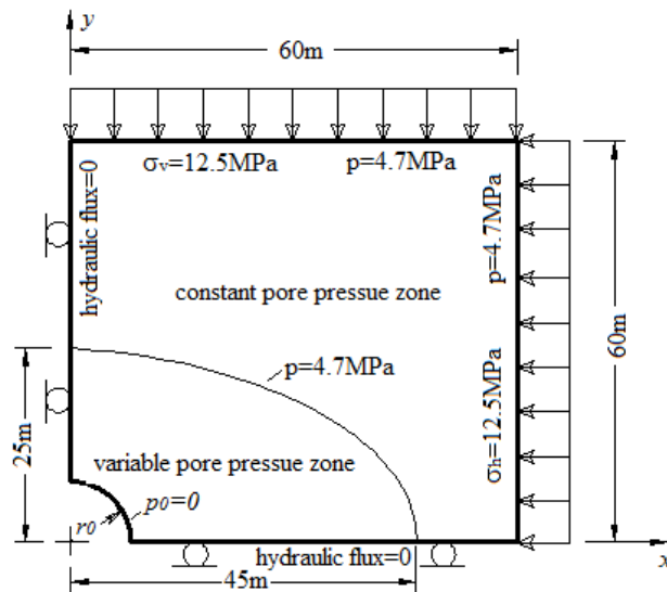
Fig. 2-7: 2D plane strain model used in the numerical simulation by FEM
