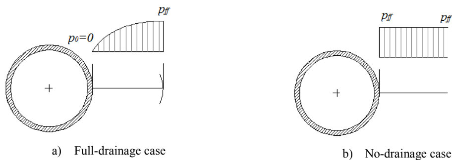
Fig. 2-9: Two cases of drainage conditions considered for the tunnel problem
