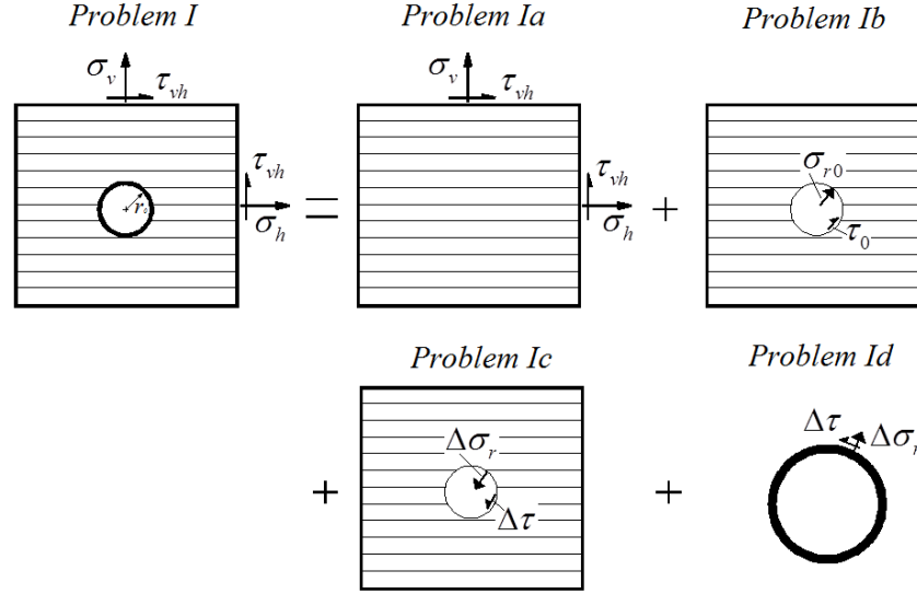
Fig. 2-4: Deep tunnel in anisotropic dry rock and its decomposition into four sub-problems (Bobet, 2011).
