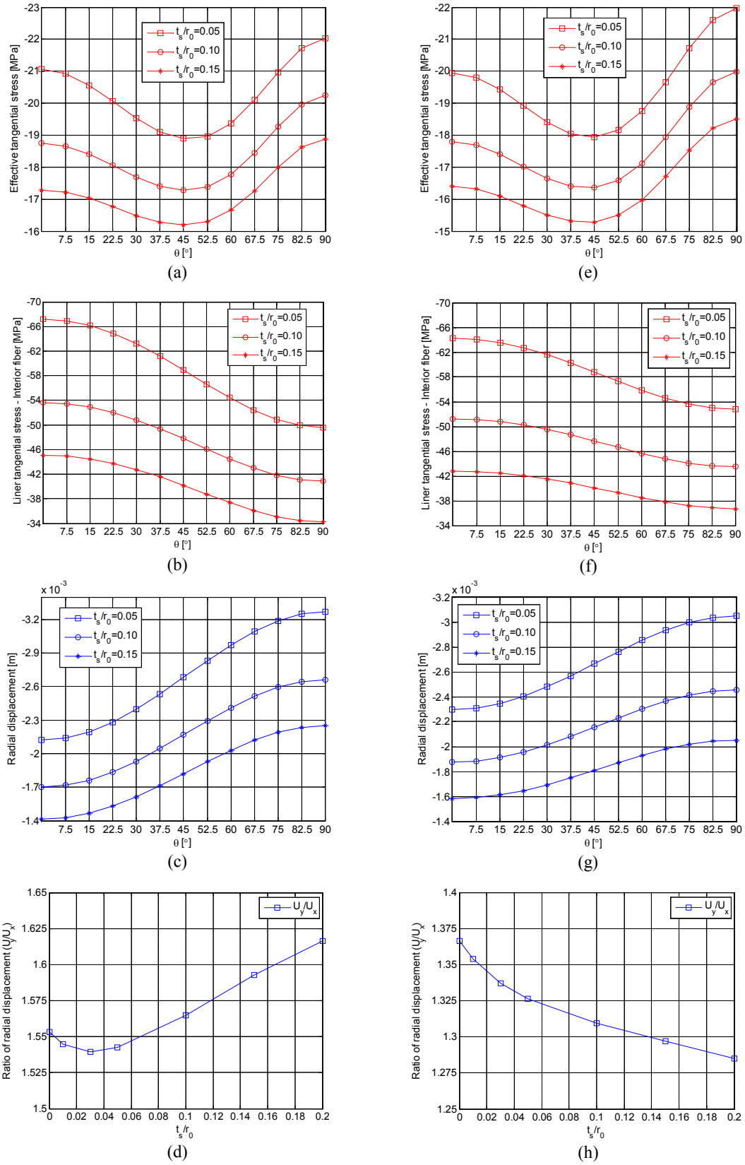
Fig. 2-22: Influence of the liner thickness ( t_s/r_0 ) on the rock effective tangential stress, the liner tangential stress, the radial displacement, and the ratio of radial displacement respectively at the circumference of tunnel which is excavated: in drained rock (a, b, c, d) or in saturated rock with uniform pore pressure (e, f, g, h).
