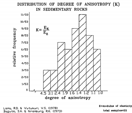
Fig. 1-1: Distribution of degree of anisotropy in sedimentary rocks according to Lama and Vutukuri, 1978
