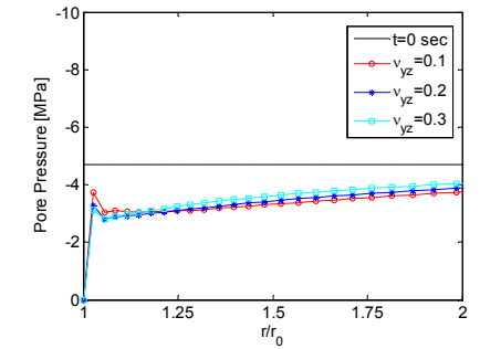
b) Pore pressure in the vertical direction
