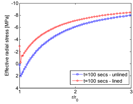
Effective radial stress in the vertical direction
