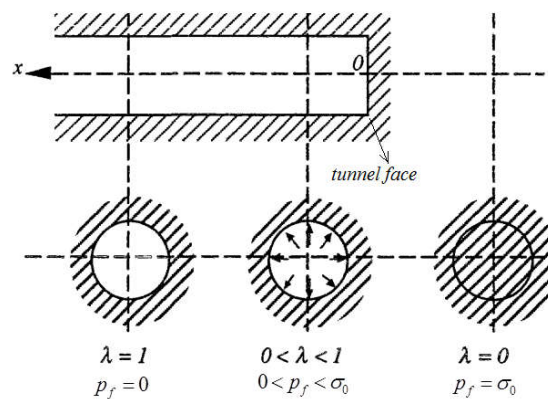
Fig. 4-3: Principle of deconfinement rate (Panet, 1995).
