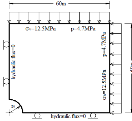
Fig.3-4: 2D plane strain model used in the numerical simulations by FEM
