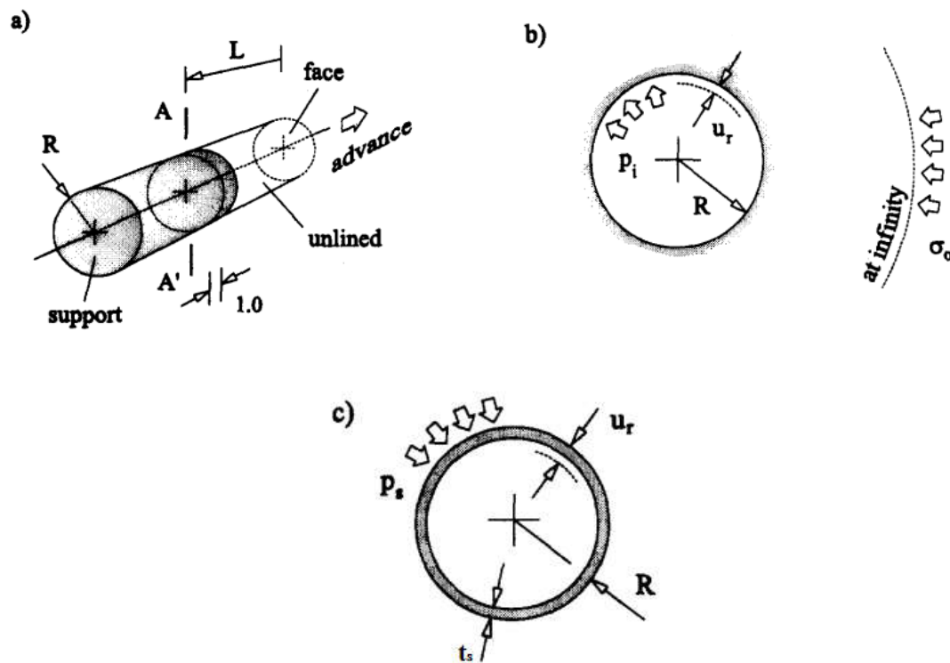
Fig. 4-1: a) Circular tunnel of radius R driven in the rock-mass; b) Cross-section of the rock-mass at section A-A'; c) Cross-section of the circular support installed at section A-A' (Carranza-Torres and Fairhurst, 2000).
