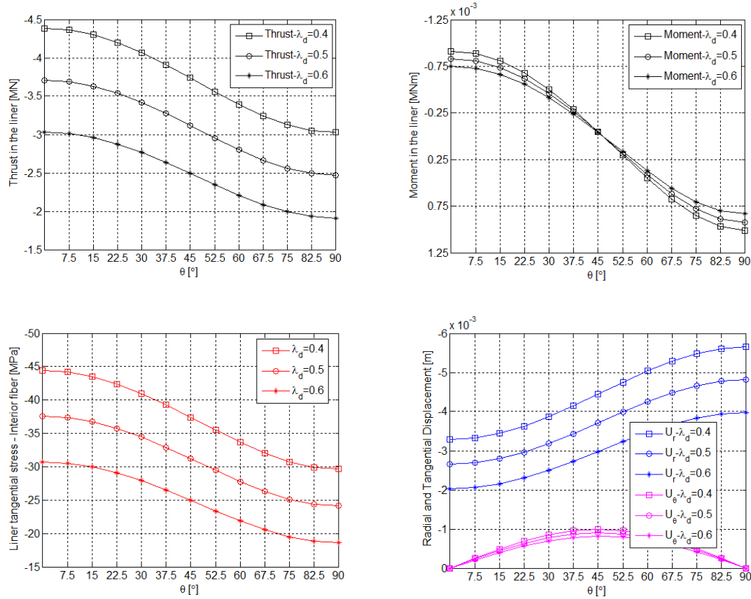
Fig. 4-12: The thrust (a), moment (b), stresses (c) and the displacement (d) of the liner corresponding to \lambda_d=0.4 , \lambda_d=0.5 and \lambda_d=0.6 for the case of drained condition in steady state
