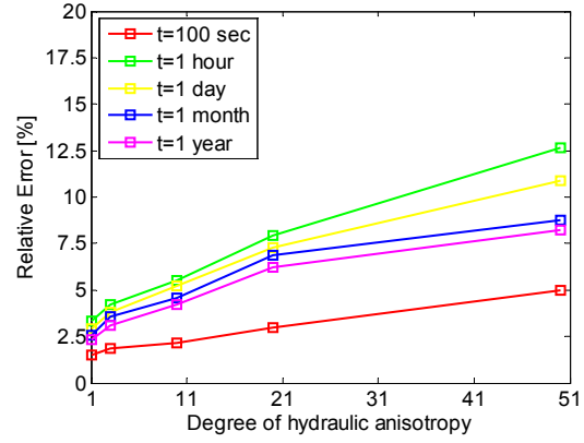
b) Relative error of effective tangential stress (case r_0=1.0 m)
