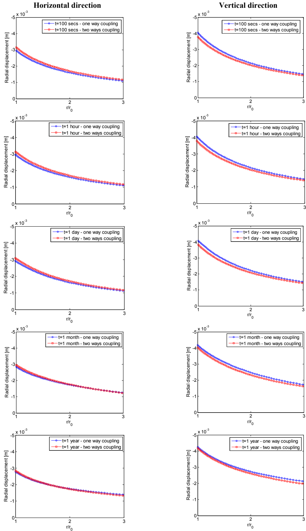
Fig.3-23: Distribution of radial displacement around the tunnel: comparison between the one way and two ways coupling at different instants.
