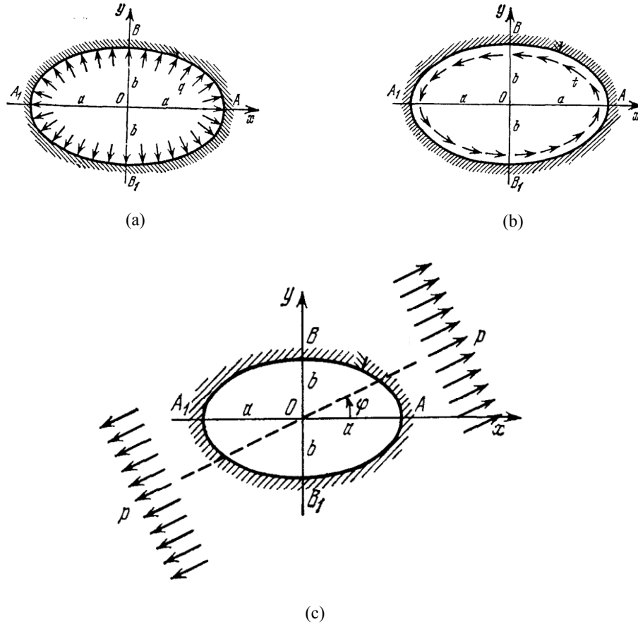
Fig. 1-10: Elliptical cavity considered by Lekhnitskii
