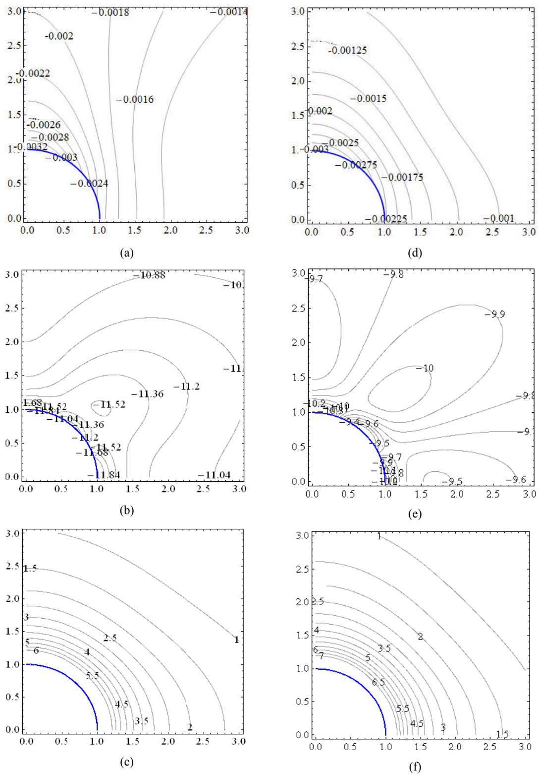
Fig. 2-10: Isovalue contours of radial displacement, mean stress and deviatoric stress respectively in rock mass for the case of drained rock (a,b,c) and for the case of uniform pore pressure (d, e, f).
