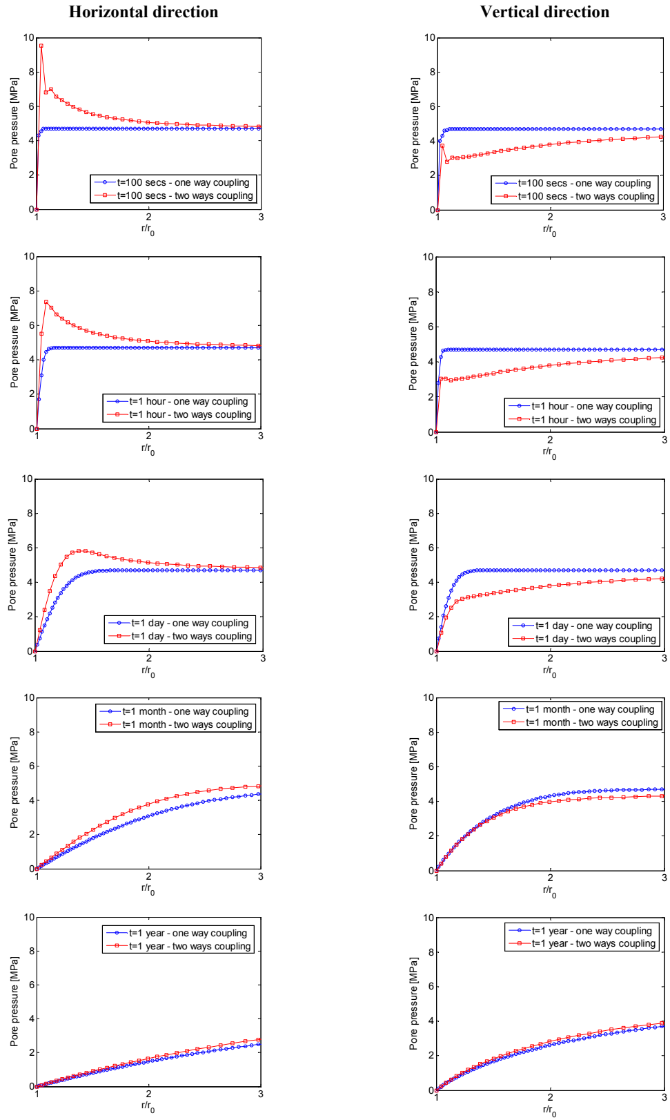
Fig.3-21: Distribution of pore pressure around the tunnel: comparison between the one way and two ways coupling at different instants.
