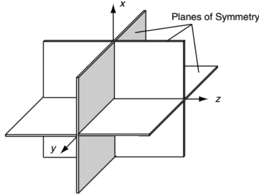
Fig. 1-5: Three planes of symmetry for an orthotropic material.
