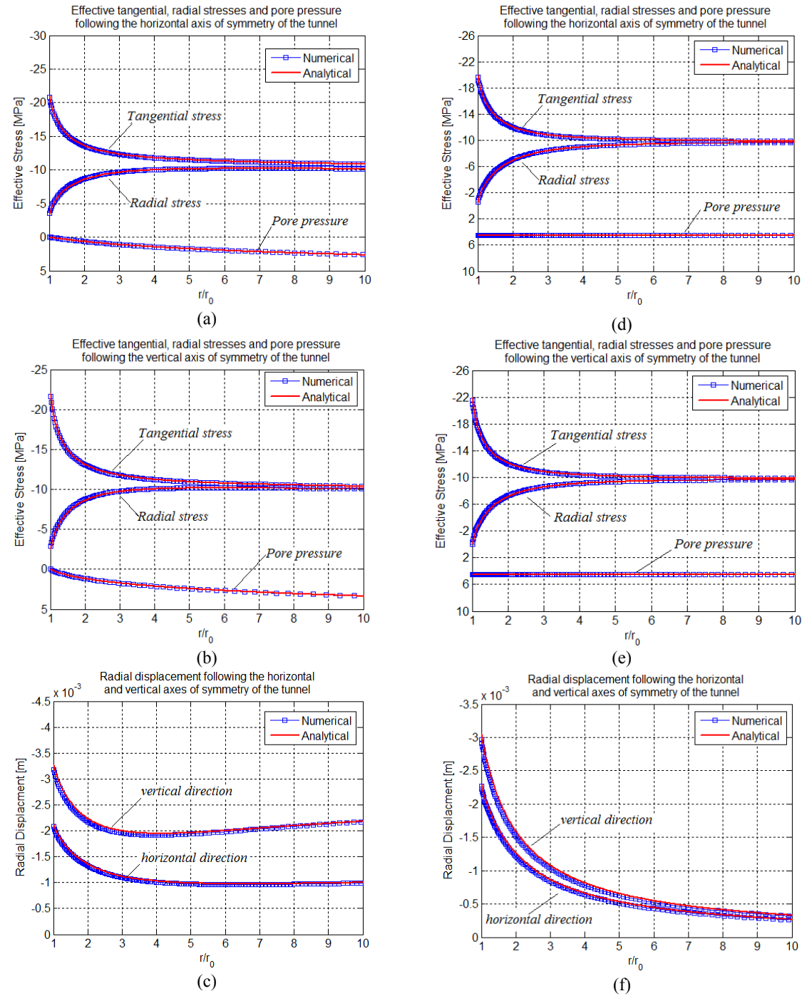
Fig. 2-8: Effective radial stress, effective tangential stress, pore pressure and radial displacements determined on the horizontal and vertical axes of symmetry of tunnel: comparison between the analytical and numerical solutions. These results are calculated for the case of excavation: in drained rock (a,b,c) and in saturated rock with uniform pore pressure (d,e,f).
