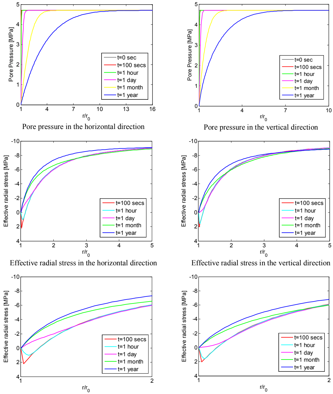
Fig.3.17: Pore pressure and effective radial stress in the horizontal and vertical direction of unlined tunnel. The results calculated at different instants.
