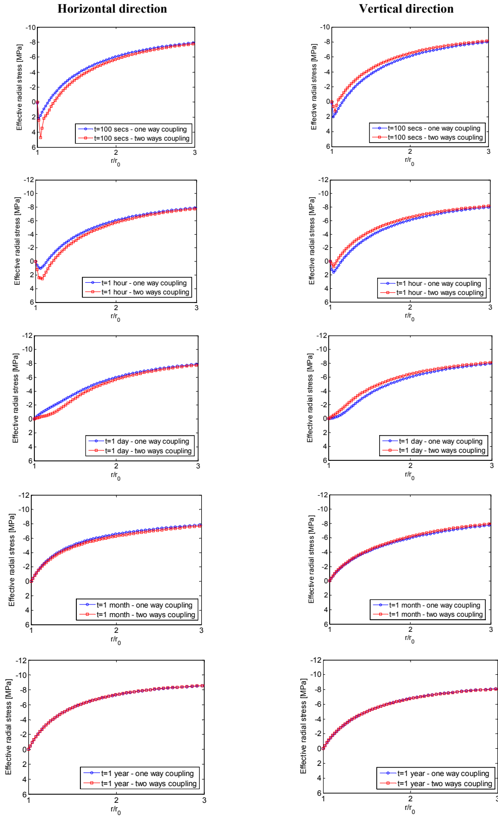
Fig.3-22: Distribution of effective radial stress around the tunnel: comparison between the one way and two ways coupling at different instants.
