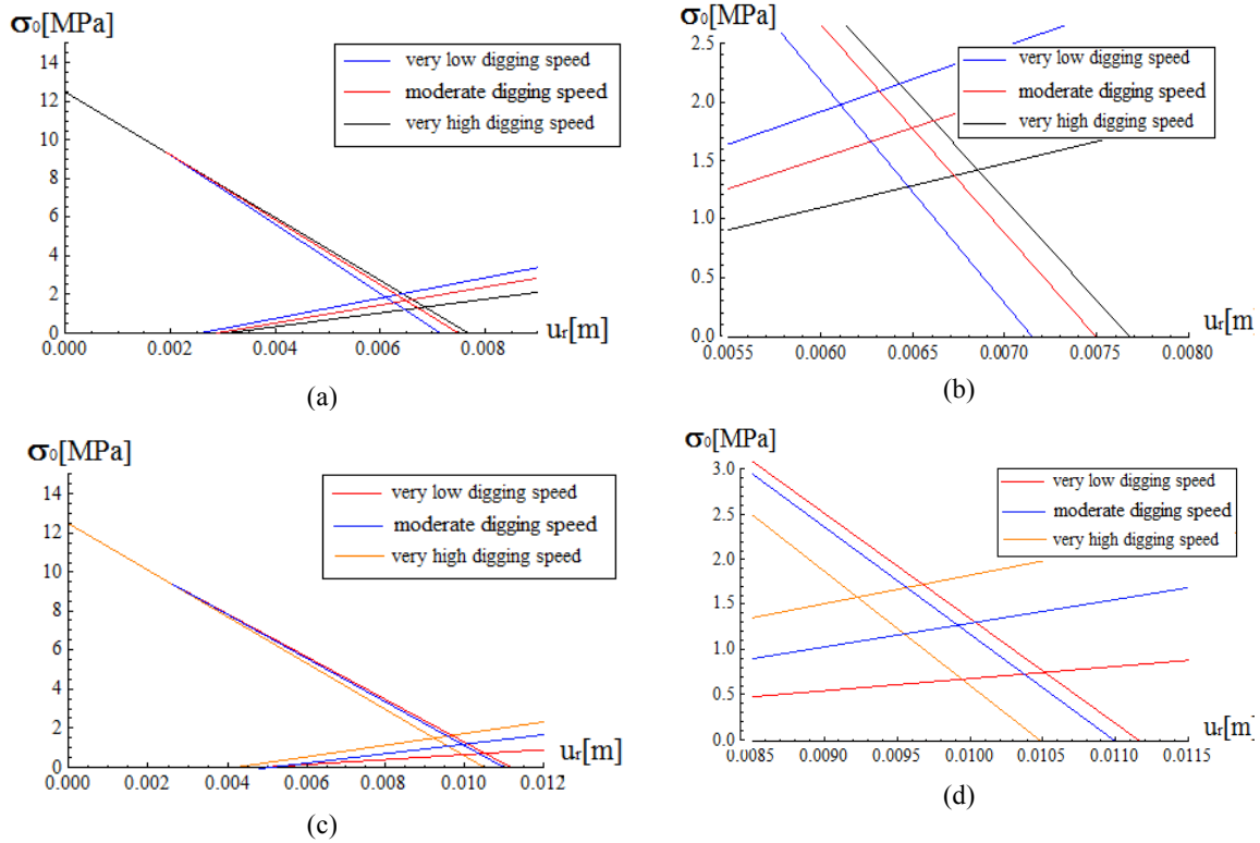
Fig. 4-8: Ground characteristic curve and support characteristic curve determined at two points in the tunnel wall a) at the springline of tunnel ( \theta=0 ), b) at the springline \theta=0 with zoom around the equilibrium state, c) at the crown of tunnel ( \theta=\pi/2 ), d) at the crown of tunnel ( \theta=\pi/2 ) with zoom around the equilibrium state
