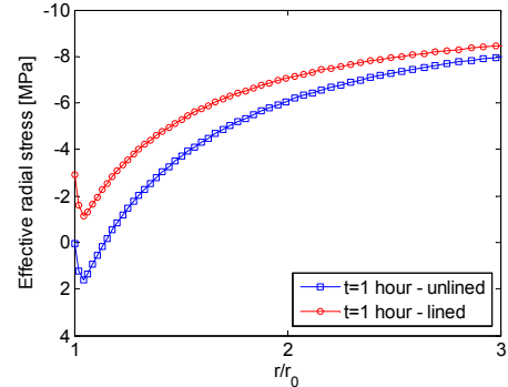
Effective radial stress in the vertical direction
