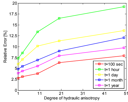
c) Relative error of effective radial stress (case r_0=1.5 m)
