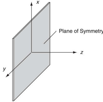
Fig. 1-4: Plane of symmetry for a monoclinic material
