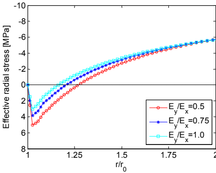
c) Effective radial stress in the horizontal direction
