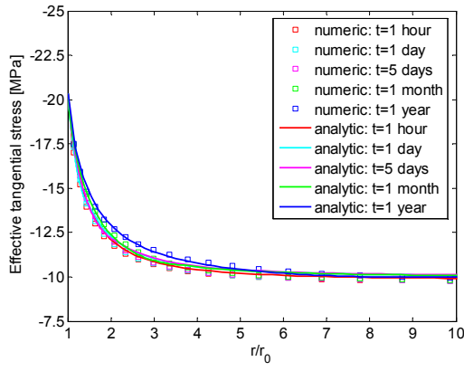
(a) Effective tangential stress in the horizontal direction
