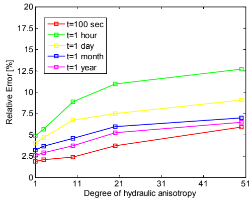
a) Relative error of effective radial stress (case r_0=0.5 m)
