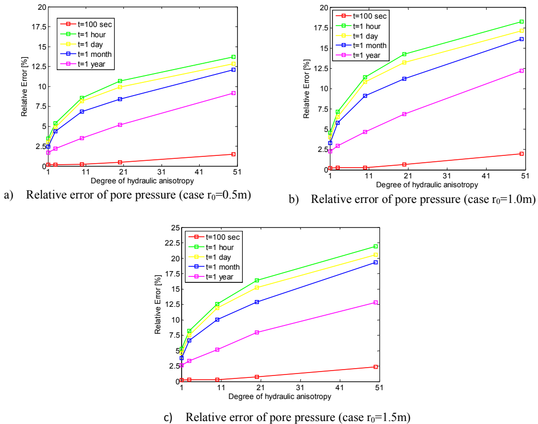
Fig.3-13: Relative error (%) between the analytical and numerical results of pore pressure in the horizontal direction as function of degree of hydraulic anisotropy ( k_a=k_x/k_y ) at different instants of time and with different radius r_0 of tunnel.
