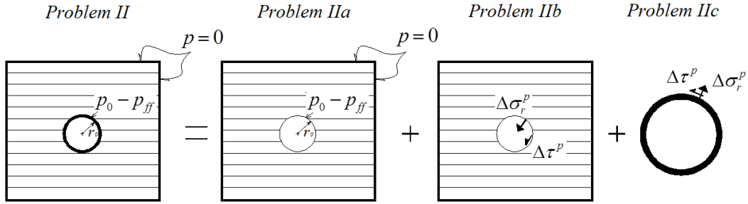
Fig. 3-3: Decomposition of the problem II into three sub-problems as ones detailed in chapter 2.
