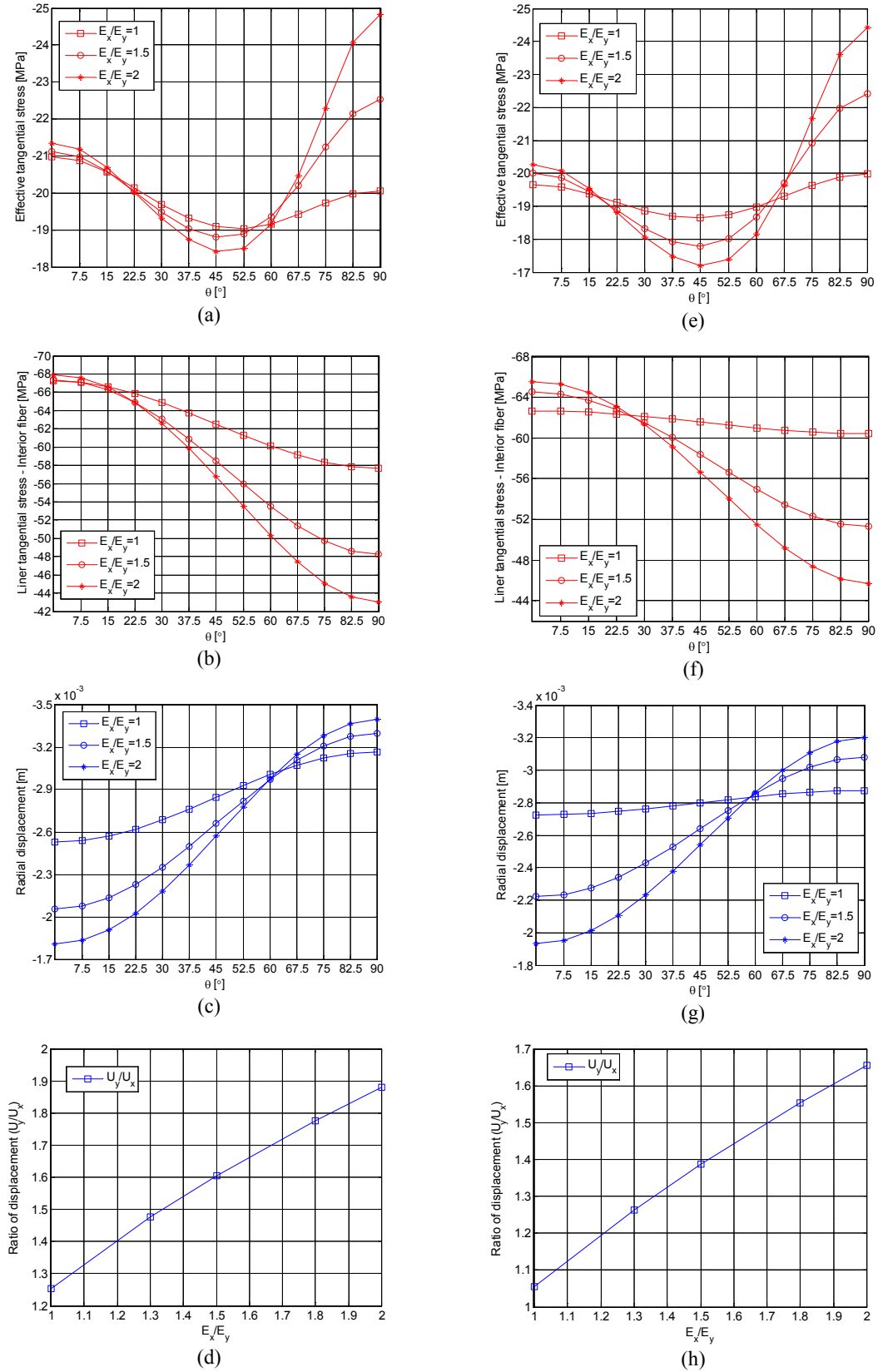
Fig. 2-14: Influence of the Young's modulus ratio ( E_x/E_y ) on the rock effective tangential stress, liner tangential stress, radial displacement, and the ratio of radial displacement respectively at the circumference of tunnel which is excavated: in drained rock (a, b, c, d) or in saturated rock with uniform pore pressure (e, f, g, h).
