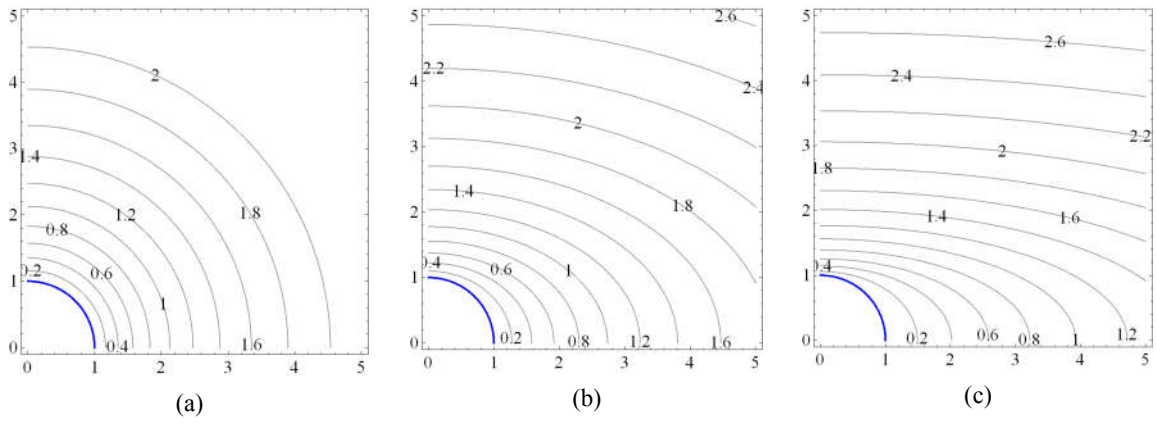
Fig. 2-16: Contours of the pore pressure around the opening tunnel in the cases: k_x/k_y=1 (a), k_x/k_y=3 (b), k_x/k_y=10 (c)
