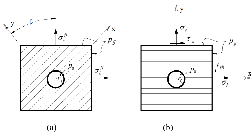
Fig. 2-1: The initial problem of deep tunnel excavated in a transversely anisotropic ground whose axes of elastic symmetry make an angle \beta with the principle stress axis at far-field (a). The equivalent problem after a rotation of angle \beta (b).
