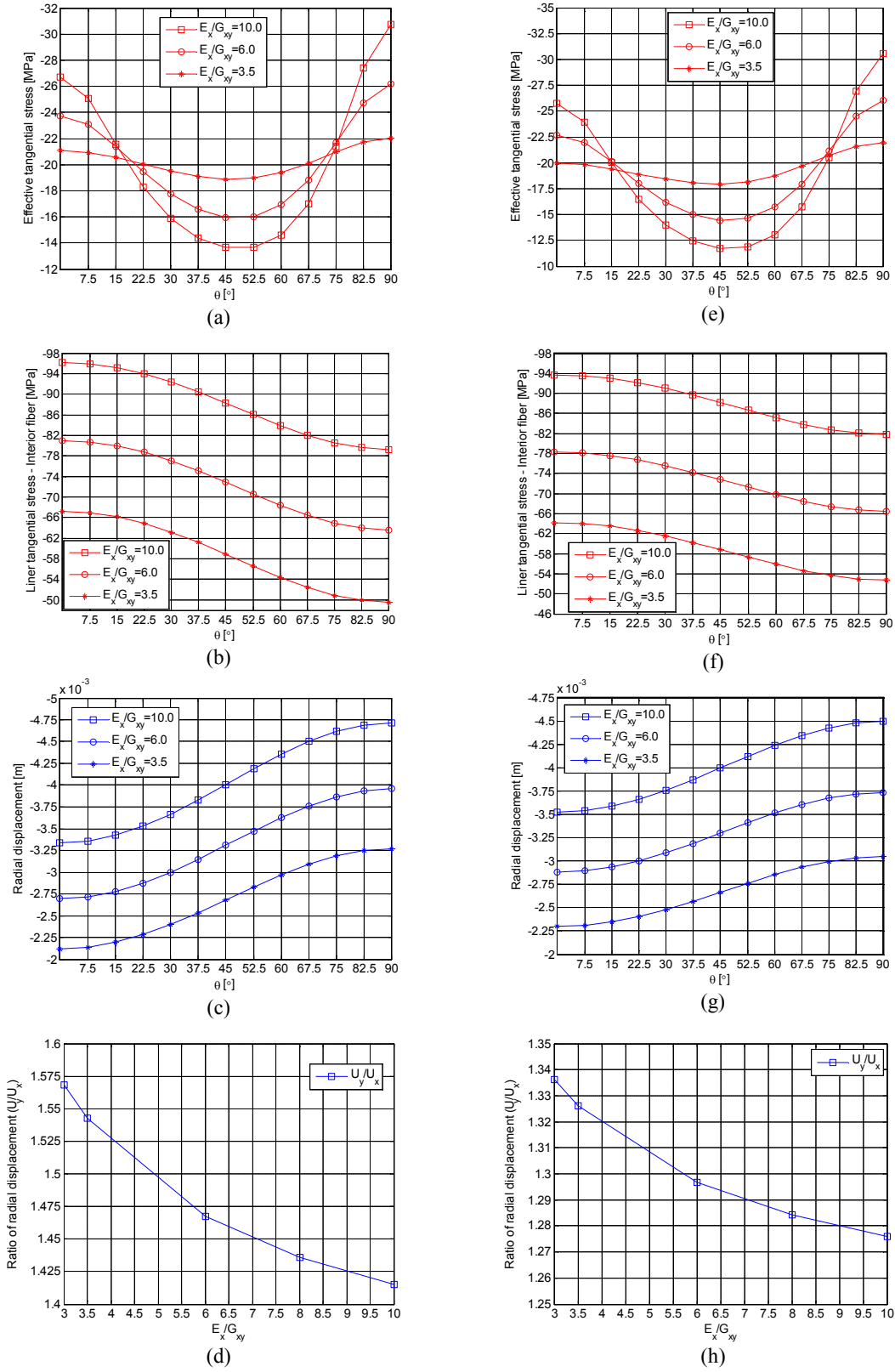
Fig. 2-13: Influence of the shear modulus G_{xy} on the rock effective tangential stress, the liner tangential stress, the radial displacement, and the ratio of radial displacement respectively at the circumference of tunnel which is excavated: in drained rock (a, b, c, d) or in saturated rock with uniform pore pressure (e, f, g, h).
