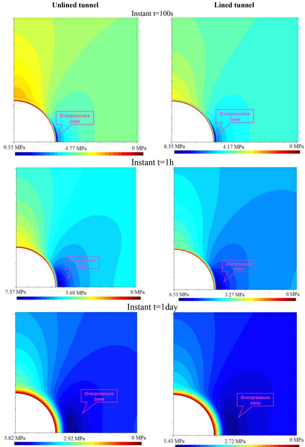
Fig.3-19: Distribution of pore pressure around the tunnel (with and without liner) at different instants. The results highlight the appearance of the overpressure zone near the tunnel when the two ways hydro-mechanical coupling is accounted for.
