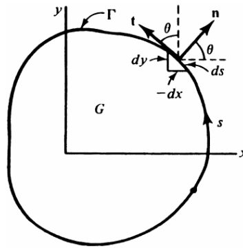
Fig. 1-8: Tangential and normal directions of boundary surfaces (Boresi, 1965 )
