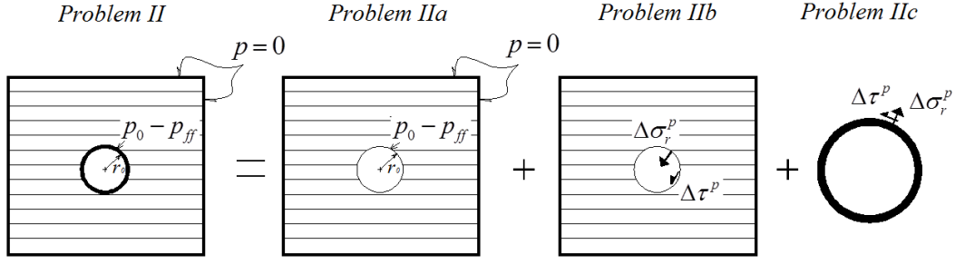
Fig. 2-6: Decomposition of the problem II into three sub-problems
