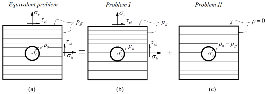
Fig. 2-3: Decomposition of the equivalent problem into two sub-problems.
