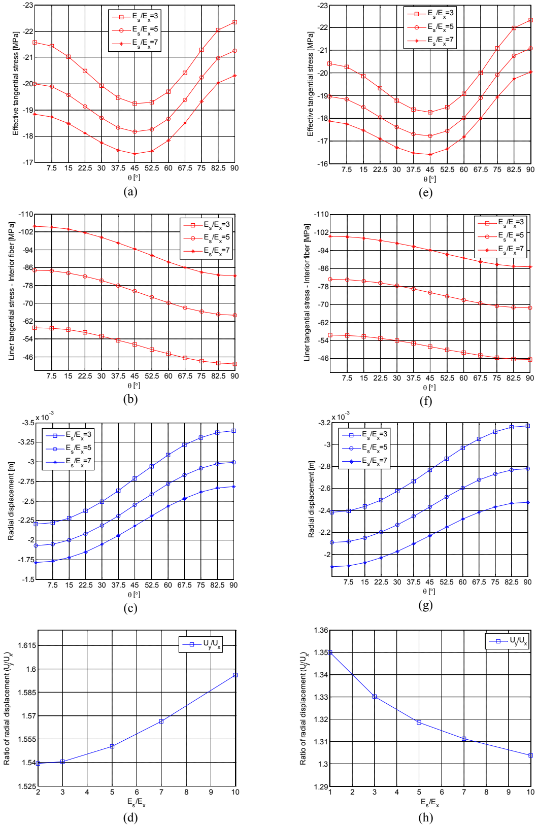
Fig. 2-23: Influence of the liner stiffness ( E_s / E_x ) on the rock effective tangential stress, the liner tangential stress, the radial displacement, and the ratio of radial displacement respectively at the circumference of tunnel which is excavated: in drained rock (a, b, c, d) or in saturated rock with uniform pore pressure (e, f, g, h).
