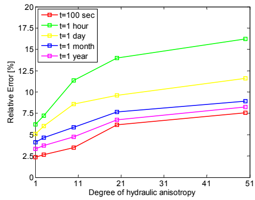
b) Relative error of effective radial stress (case r_0=1.0 m)
