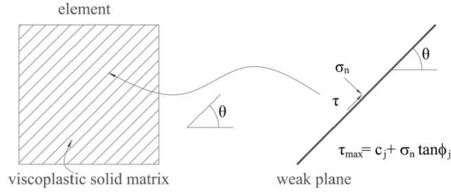
Fig. 1-6: Ubiquitous joint modeling a viscoplastic matrix
