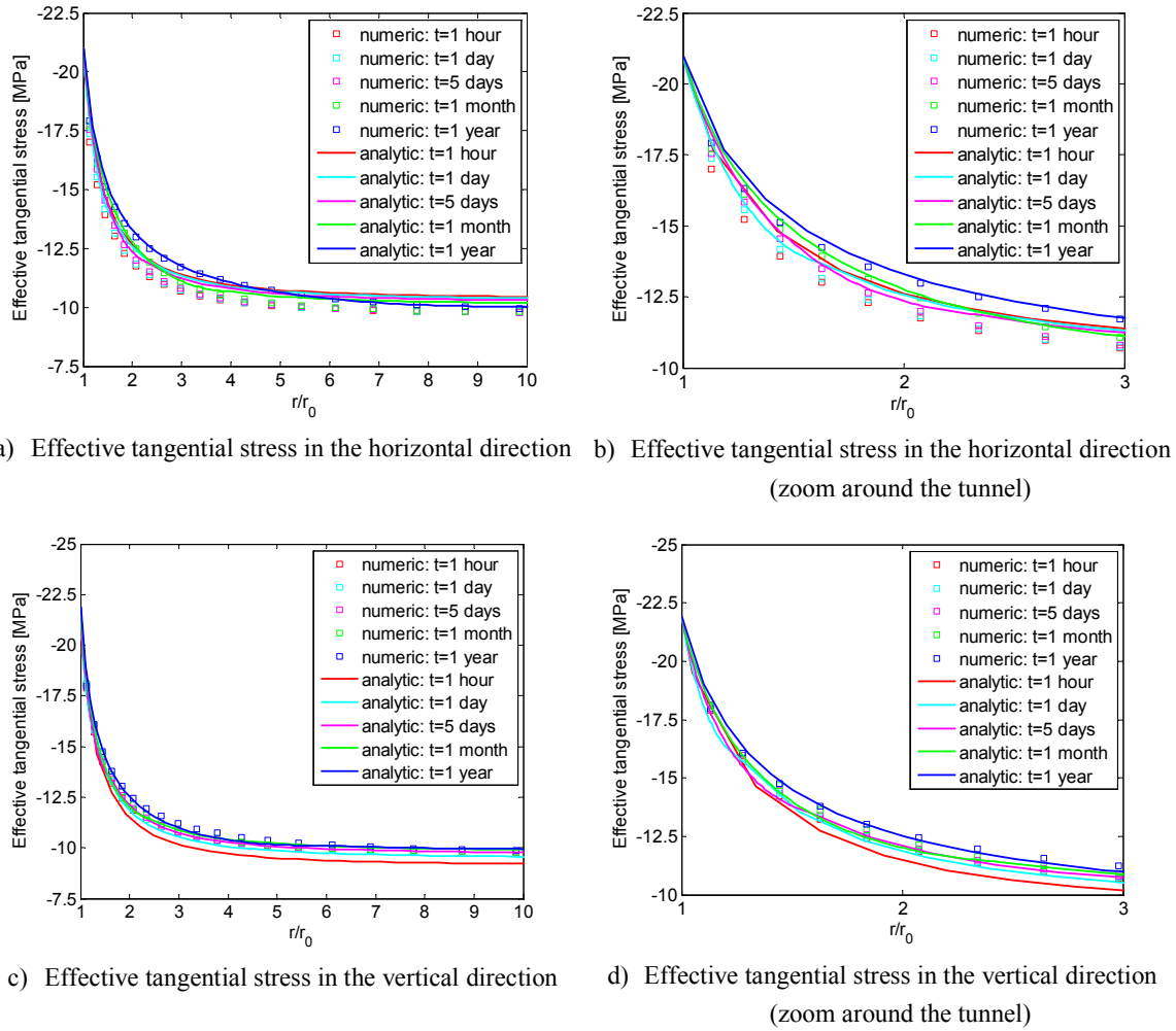
Fig.3.12: Effective tangential stress determined in the horizontal and vertical axes of symmetry of tunnel: comparison between the analytical and numerical solutions (case of saturated rock with anisotropic hydraulic properties k_a=k_x/k_y=3 ).
