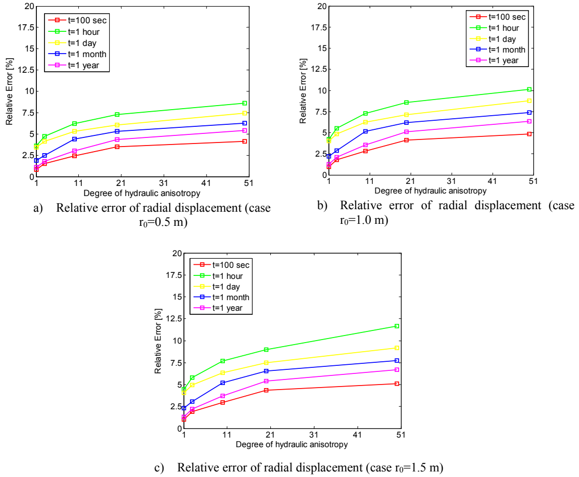
Fig.3.16: Relative error (%) between the analytical and numerical results of radial displacement in the horizontal direction as function of degree of hydraulic anisotropy ( k_a=k_x/k_y ) at different instants of time and with different radius r_0 of tunnel.
