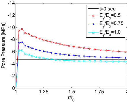
a) Pore pressure in the horizontal direction
