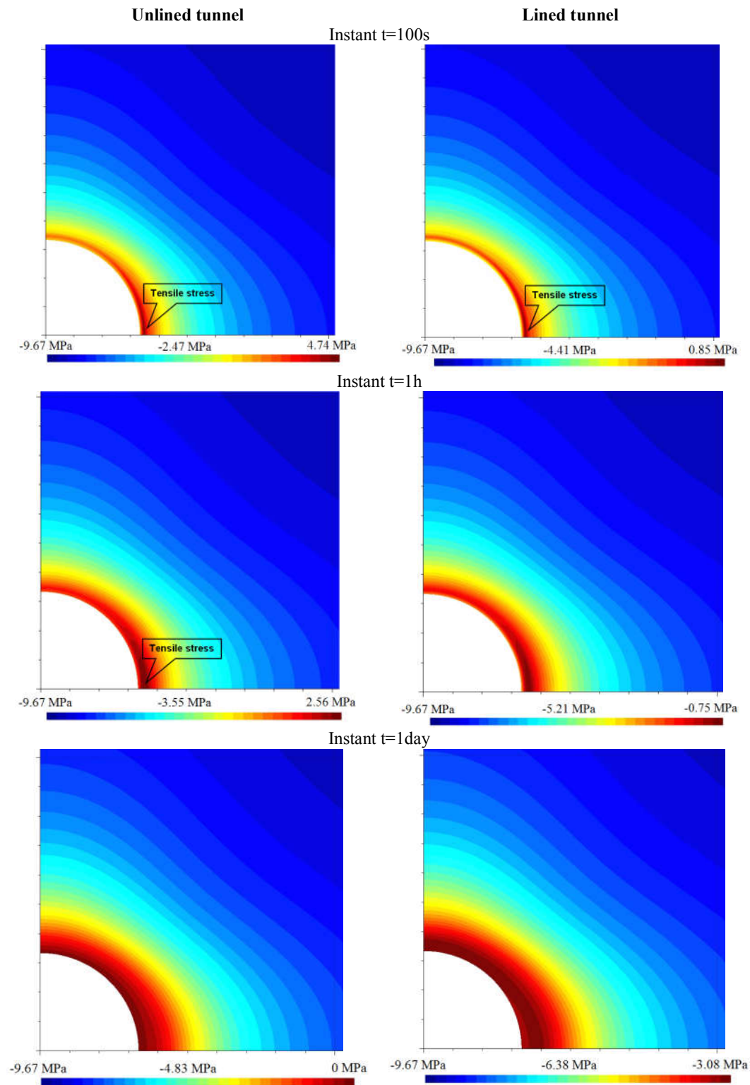
Fig.3-20: Distribution of effective radial stress around the tunnel (case with and without liner) at different instants. The results highlight the appearance of the tensile stress near the tunnel without liner at small times.
