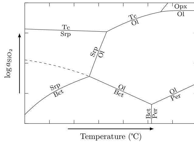
Figure 3.8: T - \log a_{\text{SiO}_2} diagram showing relative stability fields of minerals associated with serpentinization (modified from Frost and Beard, 2007 ). The dashed line is the metastable extension of the Ol-Bct equilibrium.
