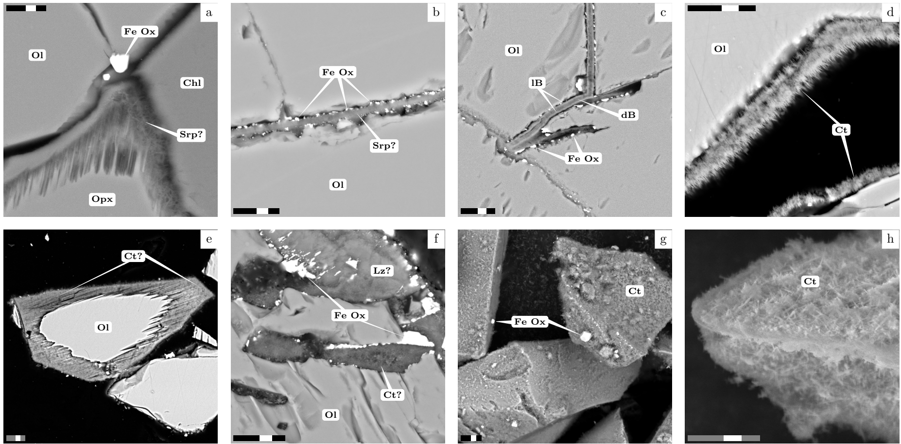
Figure 4.2: SEM images of reacted dunite (a) and San Carlos olivines (b-h). For each view, the scale bar is 10 µm. Mineral abbreviations same as in Table 4.1. (a-f): polished sections, (g-h): unpolished preparations. (a): BSE image of dunite reacted in AgPd ( Run3 , Table 4.1). Orthopyroxene is more markedly dissolved than olivine. The nature of the Fe-oxide (either magnetite or maghemite) is undetermined. The fibrous material developed at the grain interface is serpentine, most probably chrysotile. (b): vein developed in olivine crystal, the middle of the vein is occupied by fibrous material, probably chrysotile; Fe-oxides are concentrated in “void” between olivine and the vein material (BSE, Run40 , Table 4.1). (c): texture similar to (b) except that the band is filled with material with different contrast, light (IB) and dark (dB); each band is composed of fibrous material but the difference in contrast remains unclear (BSE, Run35 , Table 4.1). (d and e): chrysotile layers around olivine crystals (BSE, Run22 and Run25 , respectively, Table 4.1). (f): dissolution gulf filled with large Fe-oxides and serpentine, probably chrysotile (BSE, Run32 , Table 4.1). (g): Fe-oxides and chrysotile developed on the surface of olivine crystals (BSE, Run21 , Table 4.1). (h): fibrous texture of chrysotile (SE, Run21 , Table 4.1).
