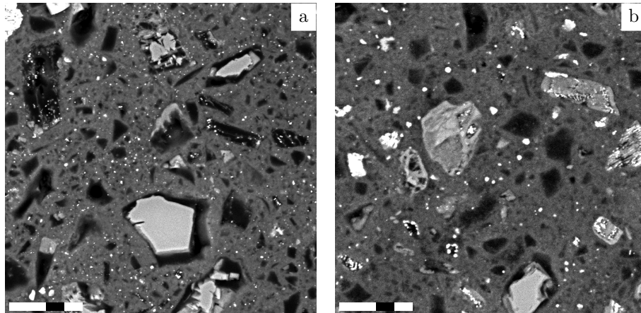
Figure 3.1: BSE images of the reacted harzburgite showing the global aspect of experimental charges. For each view, the scale bar is 50\mu\text{m} . (a) 250^\circ\text{C} (Run 43, Table 3.1) and (b) 300^\circ\text{C} (Run 45, Table 3.1). Two main components are identified: the serpentine-rich cement or “matrix” and isolated residual crystals (essentially Ol and Opx). Matrix, which forms the dominant fraction (up to 60 vol.%) of the charge, is quite homogeneous mineralogically, being essentially composed of serpentine minerals, of magnetite aggregates and locally of individual magnetite crystals. Magnetites seem more numerous but smaller at 250^\circ\text{C} (a) than at 300^\circ\text{C} (b). Matrix is considered to represent the product of advanced transformation of the dominant fine-grained fraction of the starting material. In contrast, residual crystals correspond to the coarsest fraction of starting powder and preserve less advanced stages of transformation. Voids surrounding crystals (in particular Ol) are of real significance whereas empty voids might result from sample preparation and loss of crystals.
