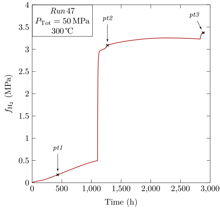
Figure 2.S3: f_{H_2} evolution in Run 47 where fluid sampling and f_{H_2} manometry were coupled (Table 2.1), performed at 50 MPa total pressure ( P_{Tot} ) and at 300°C. The membrane f_{H_2} shows an unusual type of response, marked by a major f_{H_2} jump at \approx 1100 h. Symbols pt1 to pt3 indicate when fluid sampling for the m_{H_2, aq} determinations (Table 2.2) was performed. The small bumps in f_{H_2} just before pt2 and pt3 result from readjustments of total pressure to 50 MPa (increases of 2 – 3 MPa).
