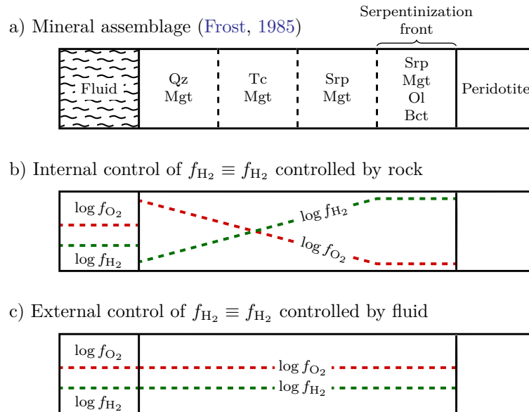
Figure 4.6: Schematic representation of fluid-mineral interactions in the oceanic crust illustrating internal and external f_{H_2} control. (a): sequence of mineral assemblages encountered assuming constant temperature and variable f_{O_2} , derived from the \log f_{O_2} vs. T diagram of the system Mg-Fe-Si-O-H system from Frost (1985). Qz: quartz; Mgt: magnetite; Tc: talc; Srp: serpentine; Ol: olivine; Bct: brucite. (b): internal control of f_{H_2} , and corresponding f_{O_2} , imposed by the sequence of mineral assemblages in (a). As \log f_{O_2} initially decreases, \log f_{H_2} progressively increases. Both the \log f_{O_2} and \log f_{H_2} are constant at the serpentinization front where serpentine, magnetite, olivine, brucite and fluid coexist (isobarically invariant assemblage in \log f_{O_2} vs. T space, Frost, 1985). (c): external control of f_{H_2} , and corresponding f_{O_2} , imposed by infiltrating fluid. The f_{H_2} is equal to that of the fluid and constant since the fluid to the front serpentinization. The infiltrating fluid is assumed to have a low f_{H_2} .
