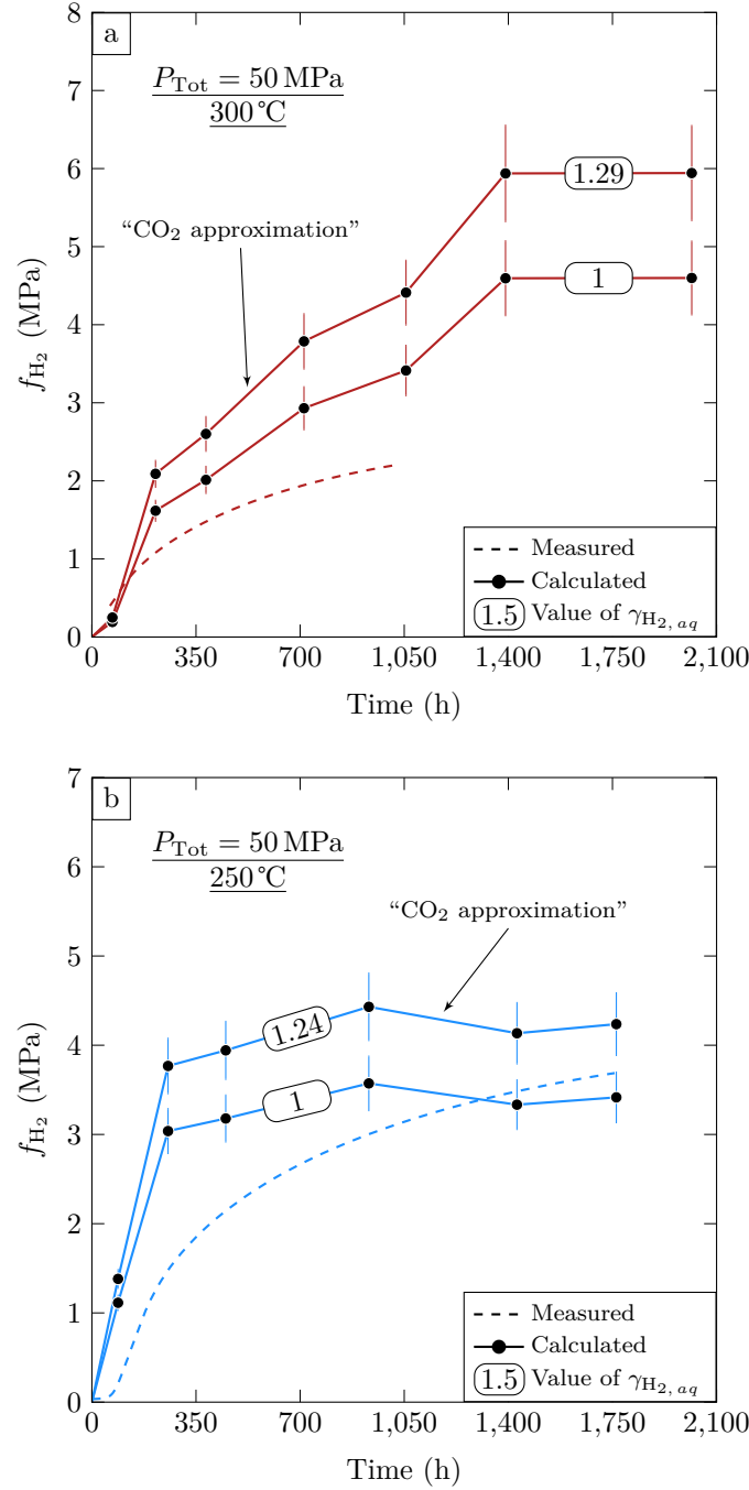
Figure 2.5: Comparison between calculated and measured f_{H_2} in serpentinization experiments carried out at 50 MPa total pressure ( P_{Tot} ). Measured f_{H_2} are indicated as dashed lines and calculated f_{H_2} as solid lines. a) Results at 300°C. Calculations use the m_{H_2, aq} measurements from Run41 to compute f_{H_2} ( m_{H_2, aq} ) using two different values of \gamma_{H_2, aq} . b) Results at 250°C. Calculations use the m_{H_2, aq} measurements from Run43 to compute f_{H_2} ( m_{H_2, aq} ) using two different values of \gamma_{H_2, aq} . The \gamma_{H_2, aq} of 1 in both (a) and (b) corresponds to the value determined for the pure H 2 O-H 2 system (Fauguerolles, 2016). The second \gamma_{H_2, aq} (1.29 in (a), 1.24 in (b)) is derived from “CO 2 approximation” (see text). At 300°C and whatever the \gamma_{H_2, aq} value, measured f_{H_2} are lower than calculated. The same behavior is observed at 250°C except that, for long durations, measured and calculated f_{H_2} become closer to each other.
