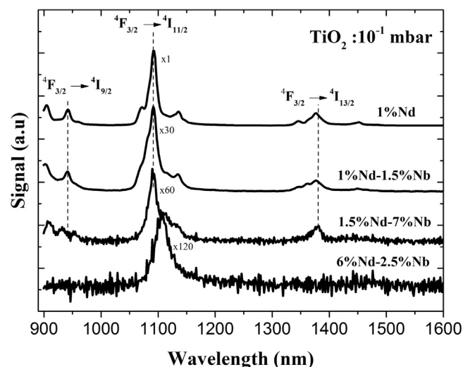
Fig. 6. PL spectra of nearly stoichiometric Nd-doped or Nd/Nb-codoped \text{TiO}_2 films. The PL spectrum of 1%Nd-doped \text{TiO}_2 film refers to results published previously [14].
