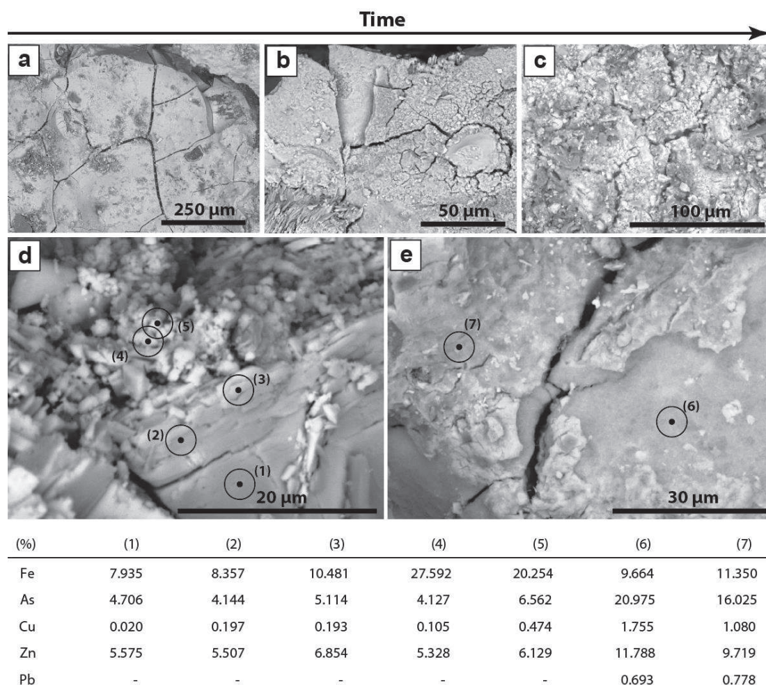
Figure 4.2: Backscattered electron images and relative concentrations of metals (% weight) of amorphous phases in the saturated soil. (a), (b) and (c) illustration of three amorphous phases sampled in the H4 level at T0, T4 and T8 respectively. (d) SEM picture of amorphous phases, sampled in H4 at T4, showing dissolution figures at the surface (elemental analyses (1) to (3)) and reprecipitation of amorphous phases (analyses (4) and (5)). (e) Surface of amorphous phases, sampled in H3 at T8, (analysis (6)) covered with a granular layer (analysis (7)).
