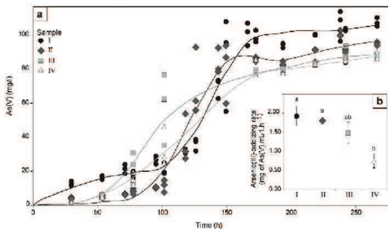
Fig. 7. Bacterial As(III) oxidizing activities (a): Evolution of As(V) concentration during the As(III)-oxidizing activity tests performed with triplicates on the four soils. (b): As(III) oxidation rates corresponding to the previous activity tests. Error bars represent the standard deviation of the mean of three replicates. Different letters denote significant difference between samples ( P < 0.05 , ANOVA, Tukey-HSD).
