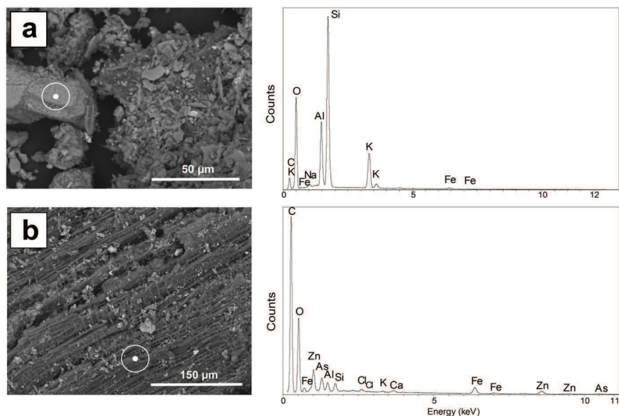
Figure 2.5: Observation and composition of inherited silicates and charcoals from black layer. a : backscattered electron images and EDS spectrum of a silicate mineral from soil sample IV. This grain was mainly composed of Si, Al and O. K and Na were also detected. The only metal(loid) detected was Fe. b : SEM picture and EDS analysis of a charcoal grain from soil sample I. These grains were identifiable by their woody structure, and contain carbon associated with. The EDS spectrum indicated charcoal containing many small quantities of elements, particularly Fe, Zn and As. The targets correspond to the location of EDS elemental analysis.
