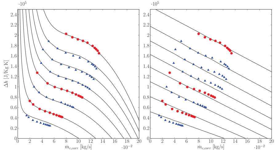
(b) Compressor 2
