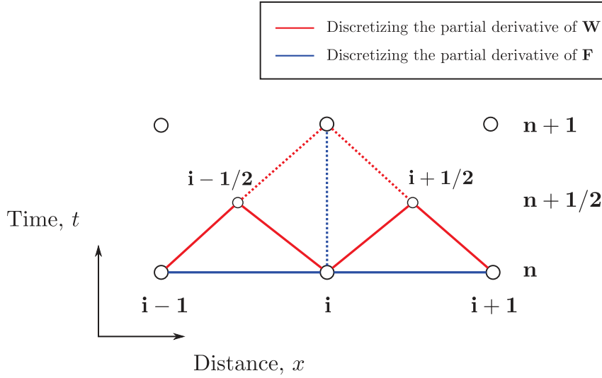
Fig. A.1.: Computational stencil of two-step Lax-Wendroff scheme
