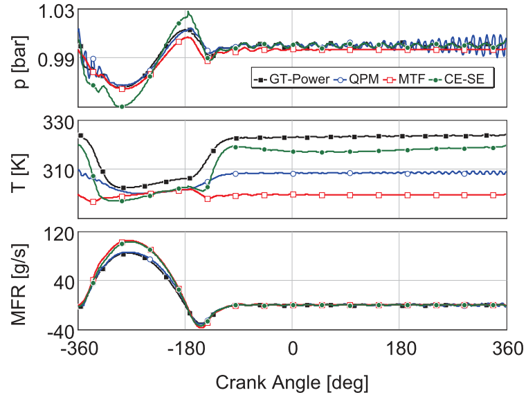
Fig. 6.2.: Predicted pressure, temperature and mass flow rate for 2000 RPM for the 1-Cylinder engine
