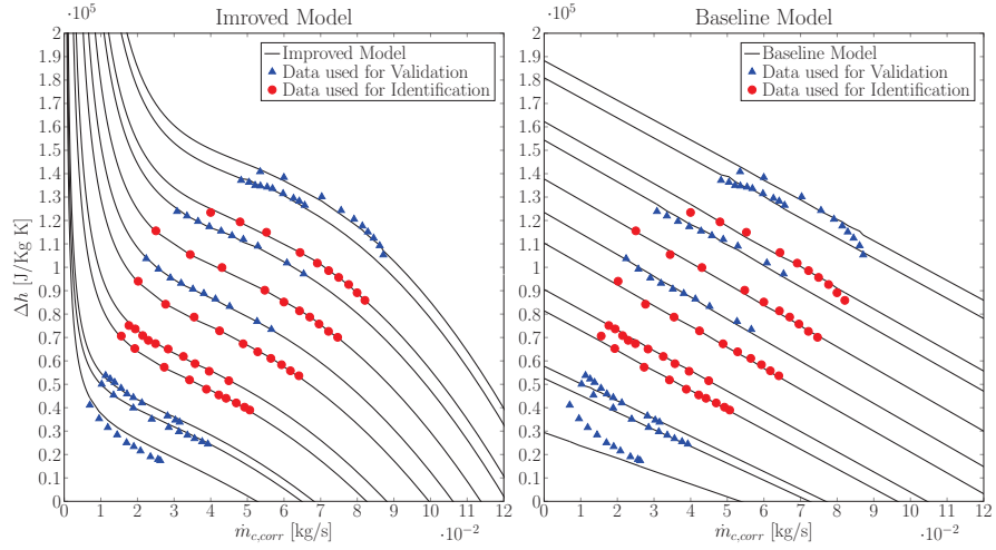
(a) Compressor 1
