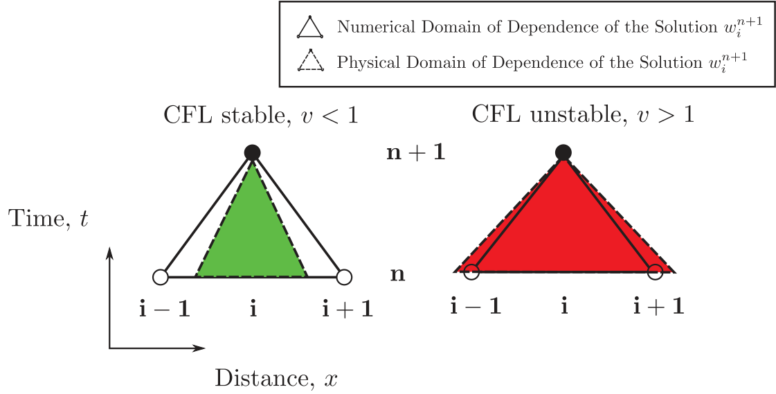
Fig. A.3.: Stencil of CFL stable and unstable selection of Courant Number v
