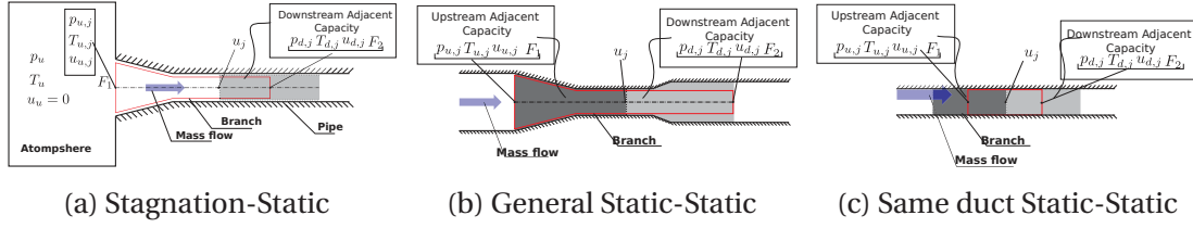
Fig. 3.4.: Illustration of the QPM boundary conditions combinations
