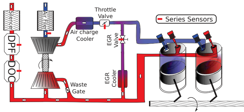
Fig. 6.12.: Air system and exhaust gas after-treatment for a two-cylinder in-line diesel engine
