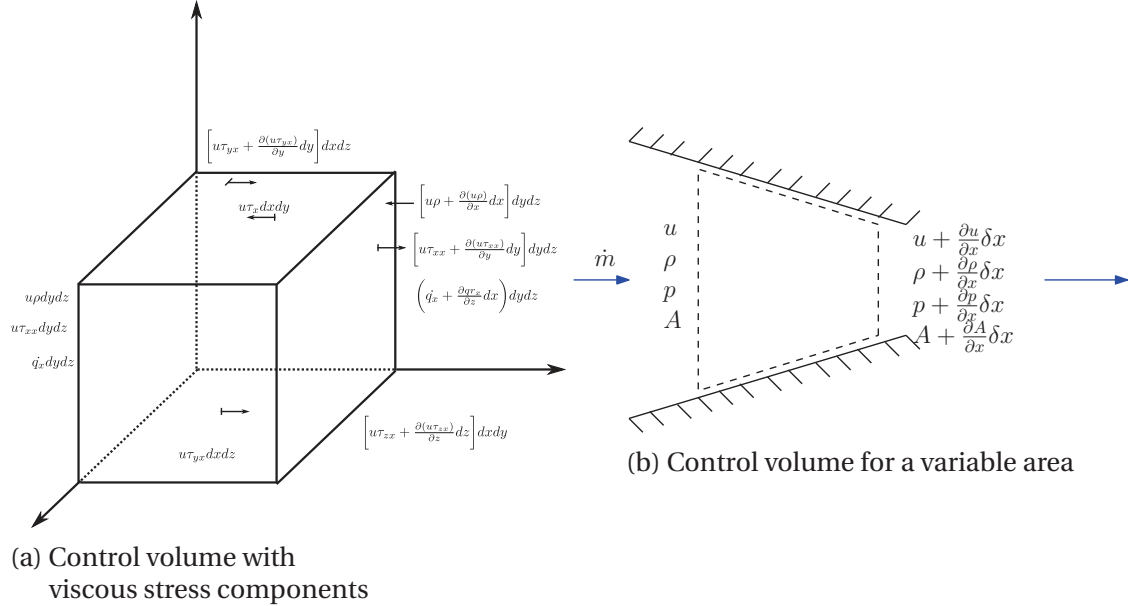
Fig. 2.2.: Comparison between 3D and 1D Modeling
