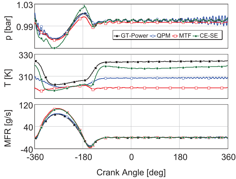
Fig. 6.3.: Predicted pressure, temperature and mass flow rate for 4000 RPM for the 1-Cylinder engine
