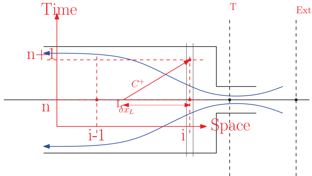
Fig. B.3.: The sudden area change with CIR
