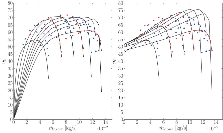
(b) Compressor 2
