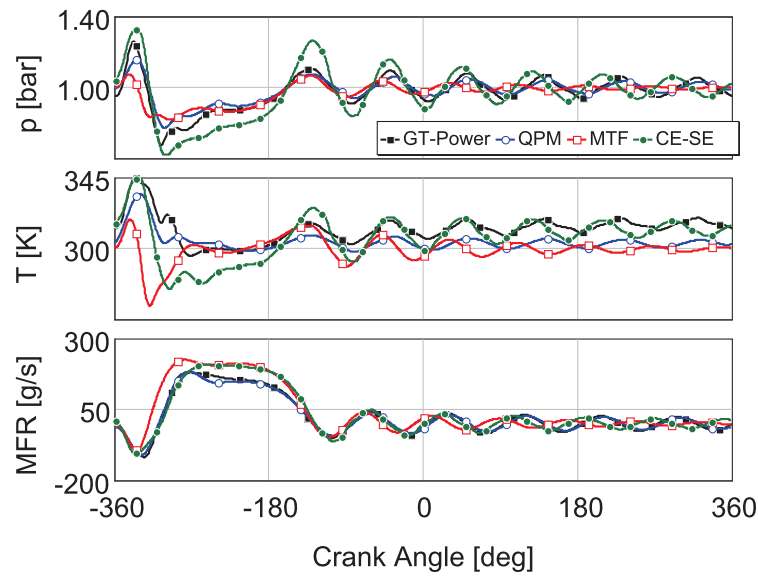
Fig. 6.4.: Predicted pressure, temperature and mass flow rate for 6000 RPM for the 1-Cylinder engine
