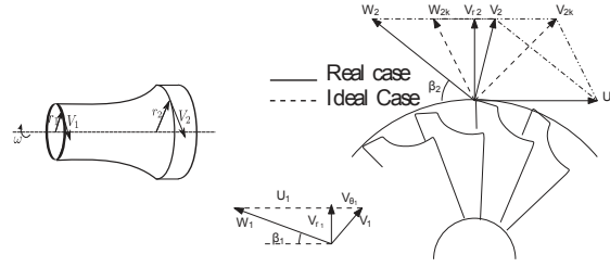
Fig. 5.4.: Euler equation for turbo-machines
