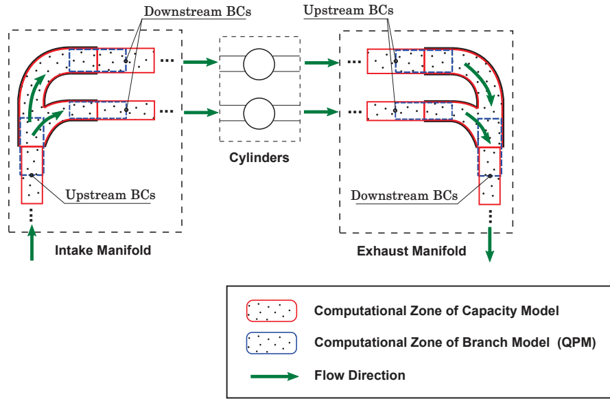
Fig. 6.16.: Modeling of the intake and exhaust manifolds by branches and capacities
