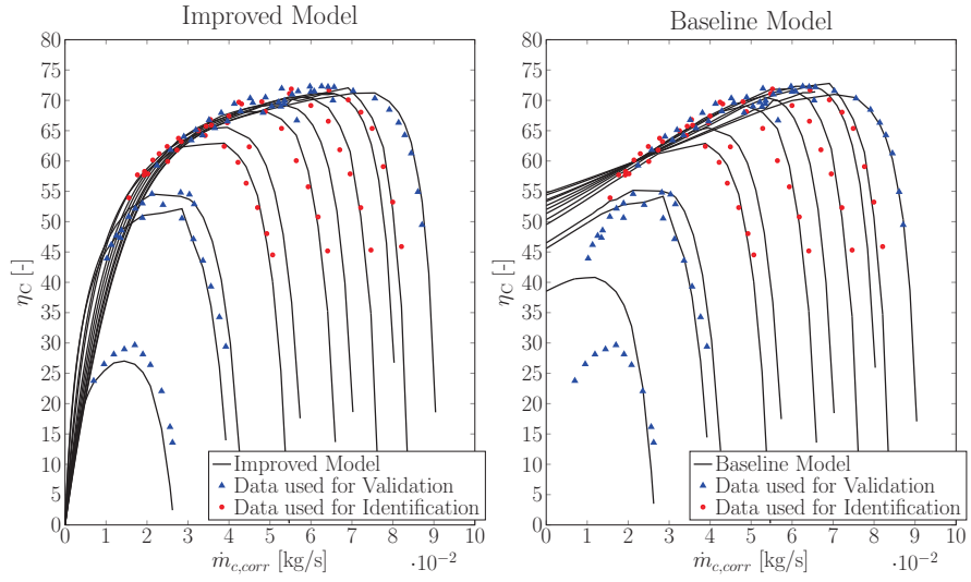
(a) Compressor 1
