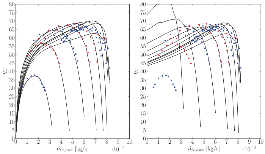
(c) Compressor 3
