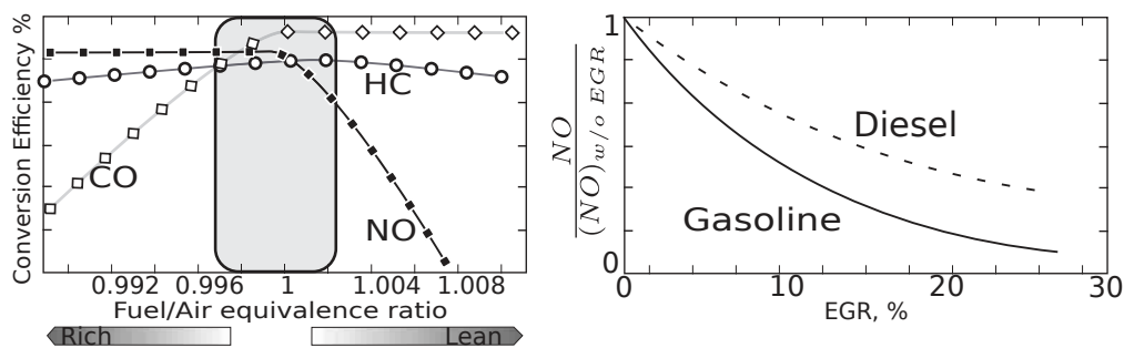
Fig. 1.9.: Effect of Fuel/Air on catalyst efficiency (left) and sensitivity of \text{NO} emissions on EGR concentrations (right)
