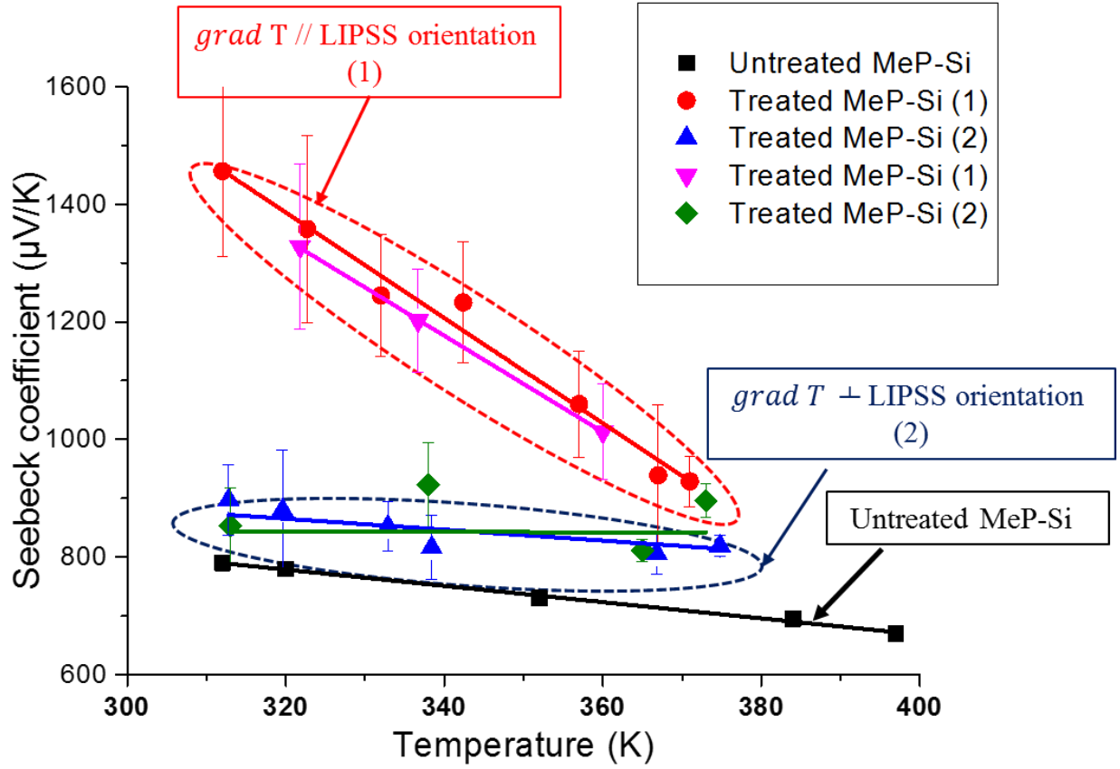
Figure.IV.17. Seebeck coefficient measurement (on nanostructured MeP-Si and untreated MeP-Si) vs temperature.
