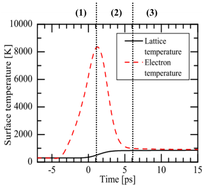
Figure.I.10. Simulation of electron and lattice temperature evolution for silicon irradiated by picosecond laser (3 ps of pulse duration) at 1030nm and a fluence per pulse of 0.58 \text{ J/cm}^2 [50].
