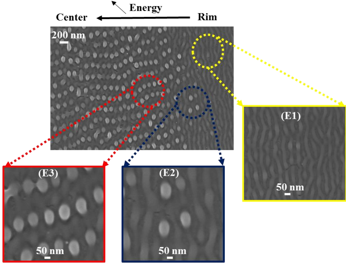
Figure.III.24. SEM views of the rim of the laser spot at 100 mJ/cm 2 and after 1000 shots.
