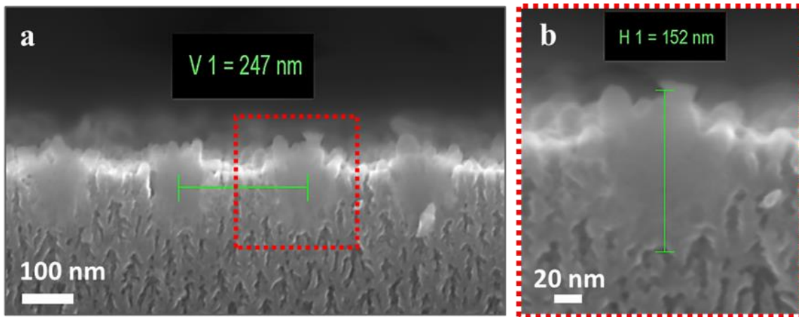
Figure.II.16. LIPSS SEM cross-section views formed at 20 mJ/cm 2 after 12000 pulses.
