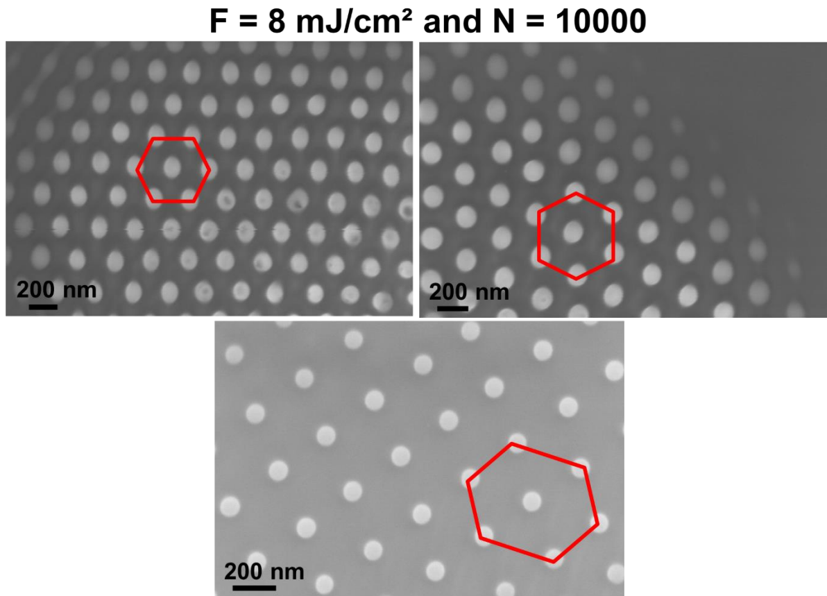
Figure.V.23. SEM views of 2D hexagonal dots organizations formed on polymer thin film surfaces irradiated by 100 fs @ 266 nm for F = 8 \text{ mJ/cm}^2 and N = 10000 ).
