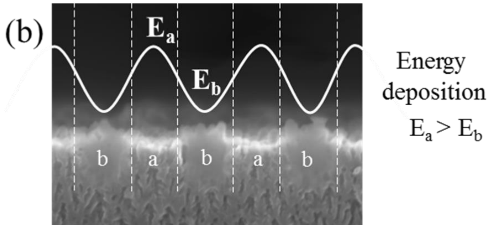
Figure.II.18. Illustration of hypothesis (b) proposed to explain the LIPSS formation mechanisms.
