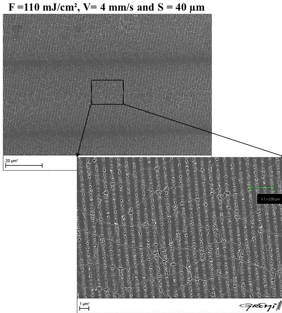
Figure.V.18. SEM images of \text{TiO}_{1.8} irradiated by 500 fs laser @ 1030 nm for N = 3000 and F = 110 \text{ mJ/cm}^2 .
