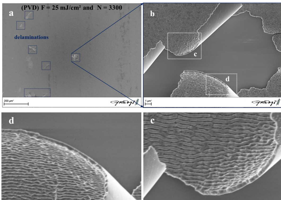
Figure.V.5 SEM characterization of TiO 1.8 (PVD) irradiated by 100 fs @ 266 nm. a) Surface view at low magnification, b) zoomed image of a), c) and d) zoomed images of c and d zones.
