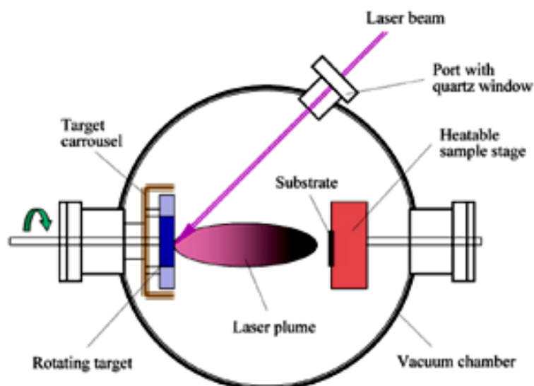
Figure.III.22. Scheme of PLD reactor used for \text{TiO}_x thin film deposition in GREMI.
