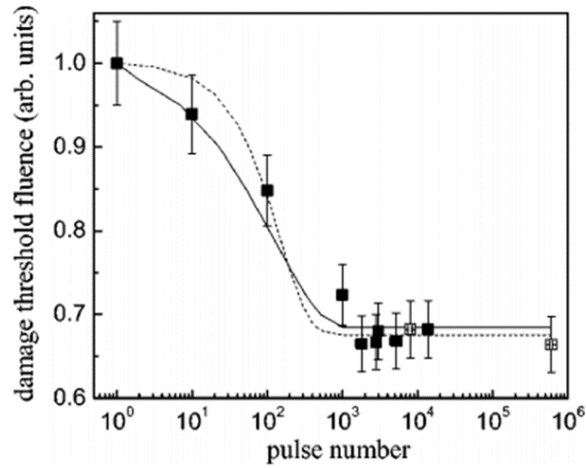
Figure.V.10. Damage threshold fluence as a function of the number of pulses for Ta 2 O 5 irradiated by 30 fs laser @ 800 nm [6].
