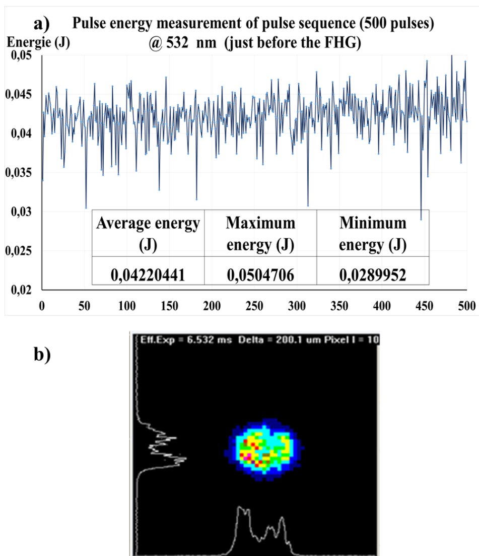
Figure.II.3. a) fluctuation of pulse energy of ps laser beam measured by powermeter @ 532 nm, b) Spatial distribution of ps laser beam characterized by WinCam D camera.
