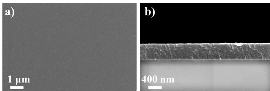
Figure.III.21. SEM characterization of \text{TiO}_{1.6} thin film: a) top view and b) cross section.
