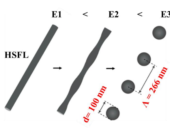
Figure.III.26. Schematic of Plateau-Rayleigh instability model showing a HSFL transformed into circular dots.
