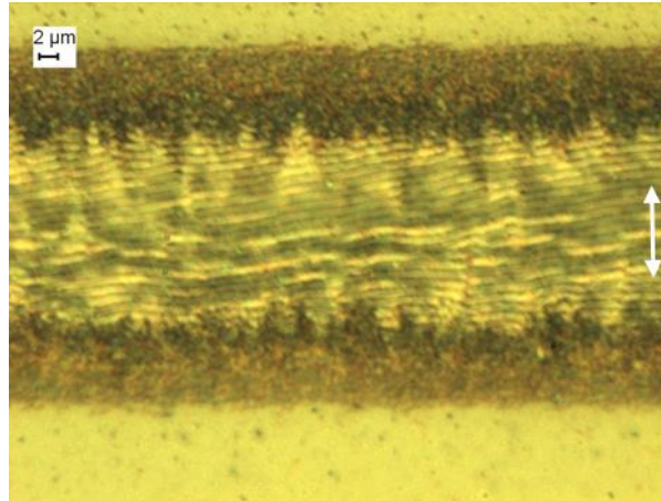
Figure.III.17. LSFL organization formed along of line drawn by 500 fs laser @ 1030 nm ( V=25 \text{ mm/s} and F= 62 \text{ mJ/cm}^2 ).
