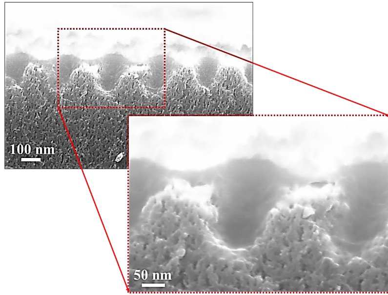
Figure.III.11. SEM cross-section views of LIPSS formed by laser scanning at 20\text{mJ}/\text{cm}^2 and after 13000 shots, by 266\text{ nm fs} beam.
