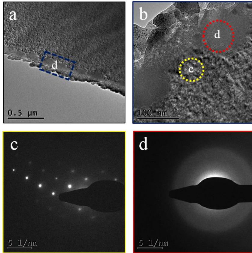
Figure.II.19. TEM analyses of LSFL formed by 266 nm ps irradiation at 20\text{mJ}/\text{cm}^2 and after 12000 pulses.
