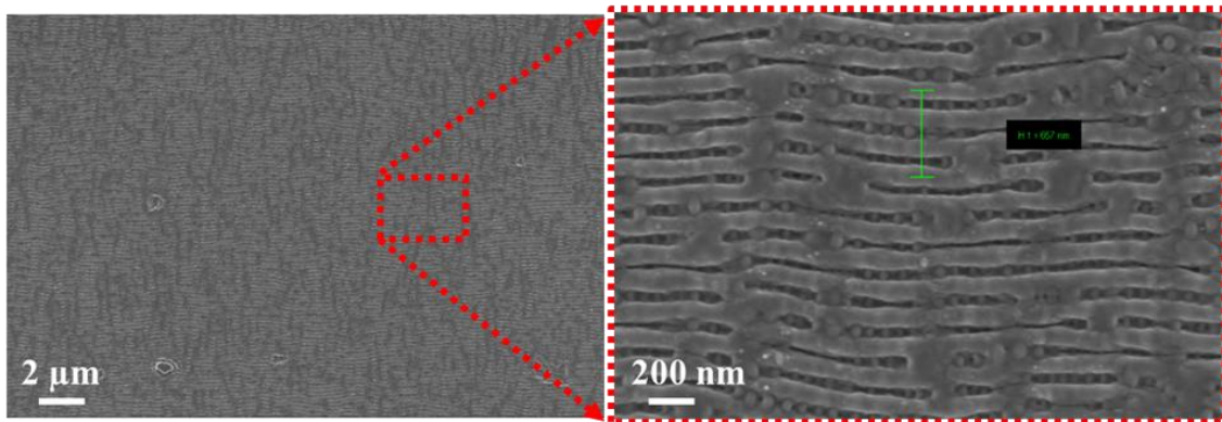
Figure.III.28. LSFL organization formed on 5 \times 5 \text{ mm}^2 \text{TiO}_{1.6} surface by 100fs laser @ 266 nm ( F=30 \text{ mJ}/\text{cm}^2 and N \sim 3300 ).
