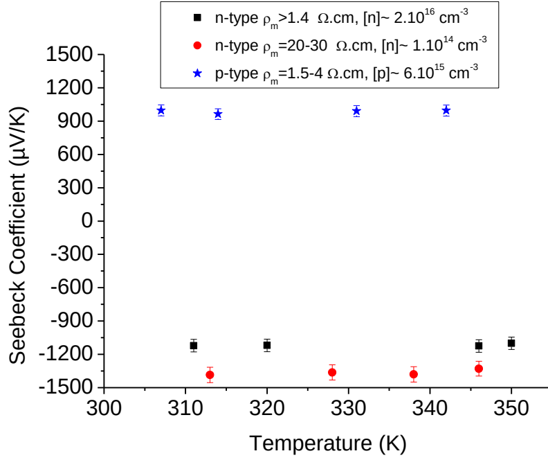
Figure.IV.8. Seebeck coefficient of n-type and p-type c-Si bulk materials as a function of the temperature ( \rho_m is the manufacturer value).
