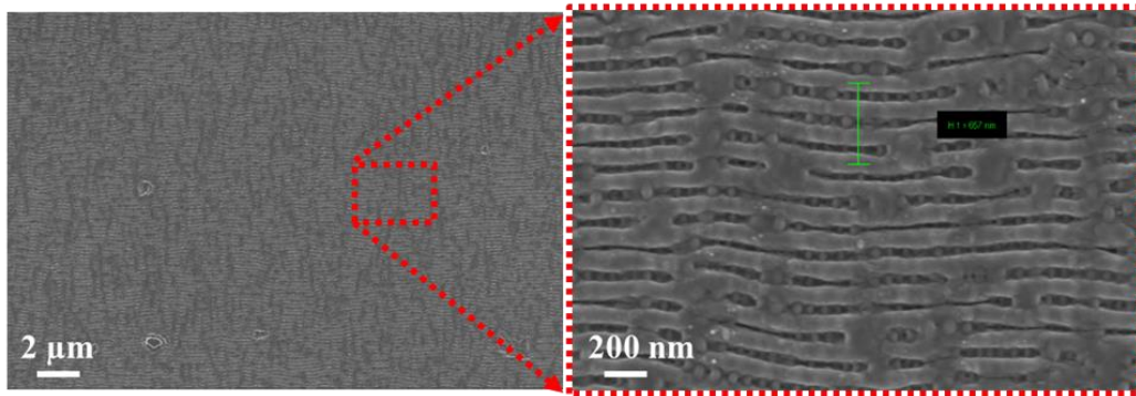
Figure.IV.19. LSPR organization formed on 5 \times 5 \text{ mm}^2 \text{TiO}_{1.6} surface by 100fs laser @ 266 nm ( F=30 \text{ mJ/cm}^2 and N \sim 3300 ).
