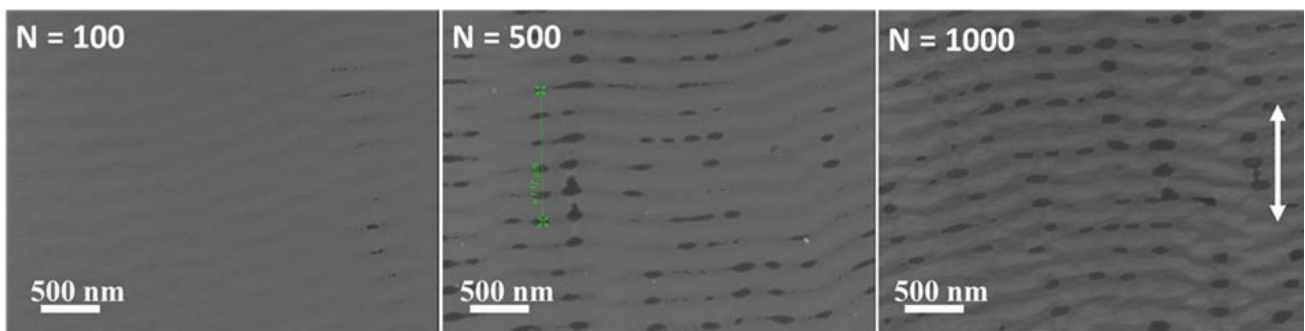
Figure.II.10. SEM views of silicon surfaces irradiated by picosecond beam at 20 \text{ mJ/cm}^2 @ 266 nm for 3 different N values of laser shots.
