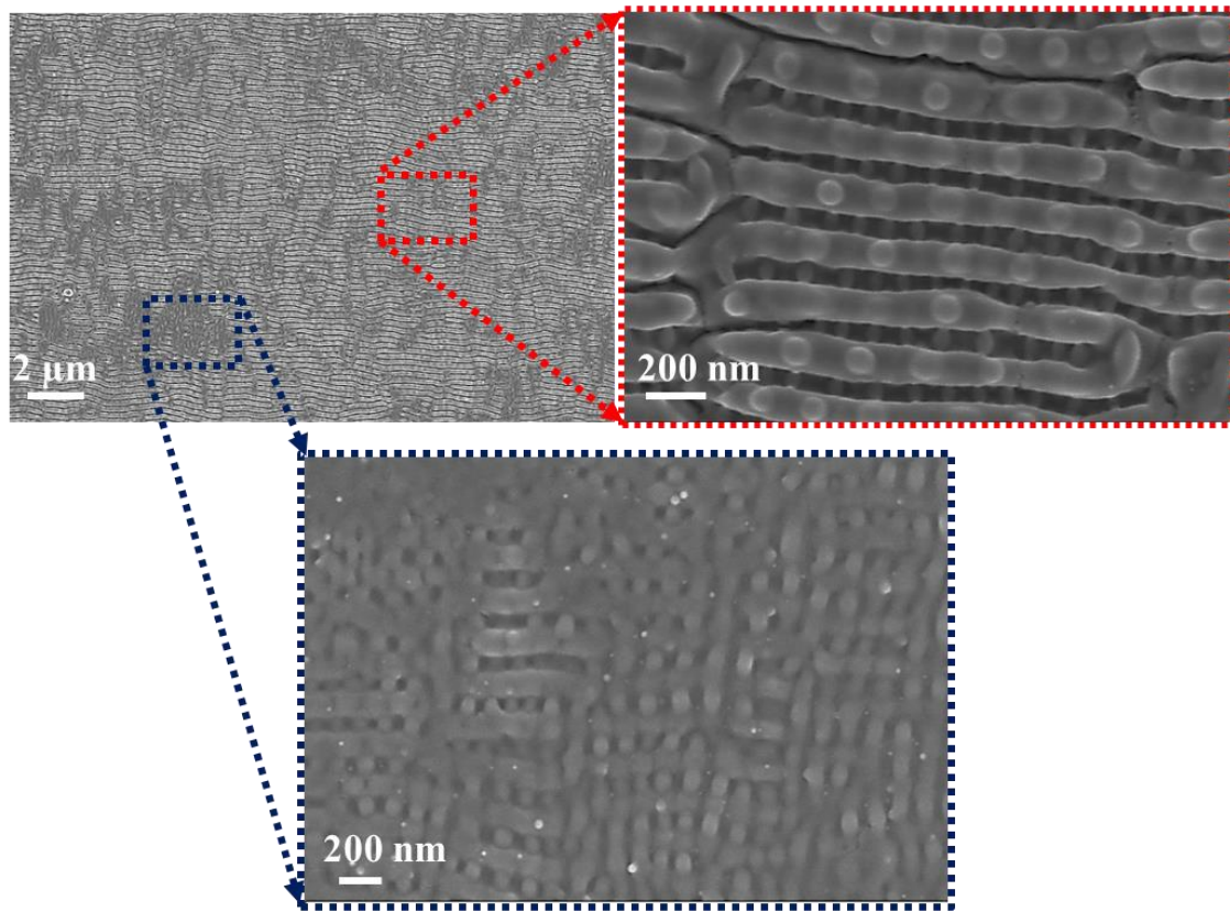
Figure.III.29. LSFL and dots organizations generated on 5 \times 5 \text{ mm}^2 TiO 1.6 surface by 100fs laser @ 266 nm ( F=25 \text{ mJ/cm}^2 and N \sim 3300 ).
