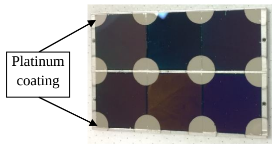
Figure.IV.2. Image of six samples after the deposition of platinum thin films by PVD on the four corners of each sample.
