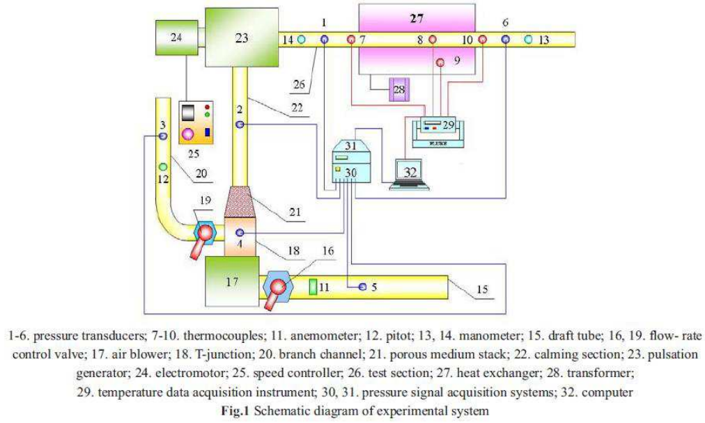
Figure 11: Experimental apparatus – Hua et al.
