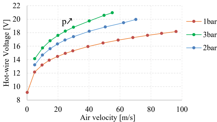
Figure 44: Impact of air pressure on Hot-Wire voltage
