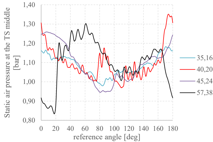
Figure 87: Static air pressures at the middle of the test-section for different pulsation frequencies
