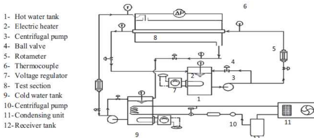
Fig. 1. Experimental apparatus.
