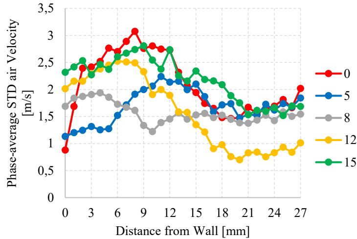
Figure 106: Phase-averaged turbulent component of the air velocity for a pulsating cold flow during periodic flow reversal, Re = 40000 , f = 10 Hz
