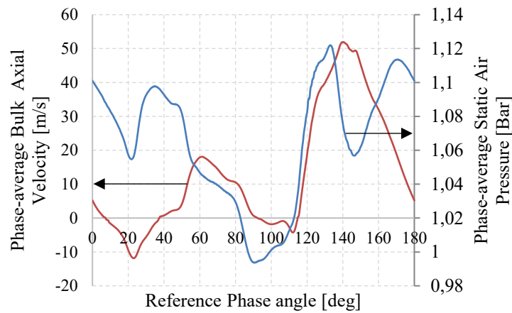
Figure 94: Phase-average bulk Velocity & Static pressure for a hot pulsating flow, Re = 30000 , f = 10 Hz
