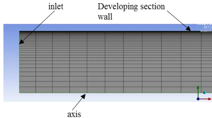
Figure 111: Mesh radial refinement
