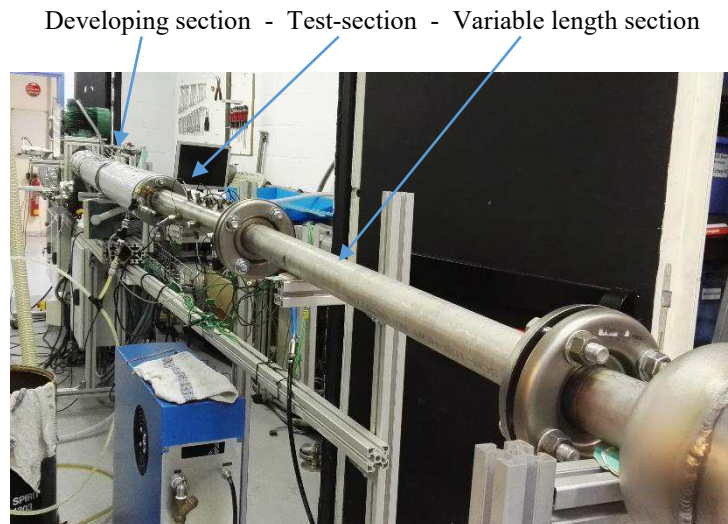
Figure 32: Experimental Apparatus 2
