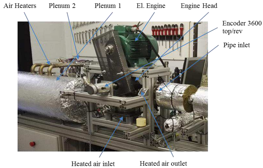
Figure 31: Experimental Apparatus 1
