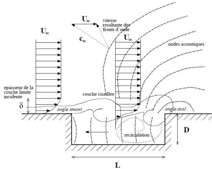
Figure 85: Sketch of cavity flow
