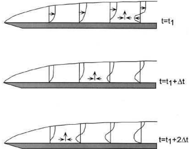
Figure 99: Schematic of streamwise boundary-layer profiles during periodic flow reversal
