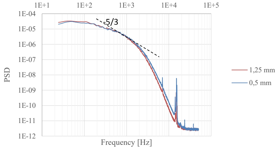
Figure 43: PSD of hot-wire measurement for a steady turbulent jet flow – Wire length investigation
