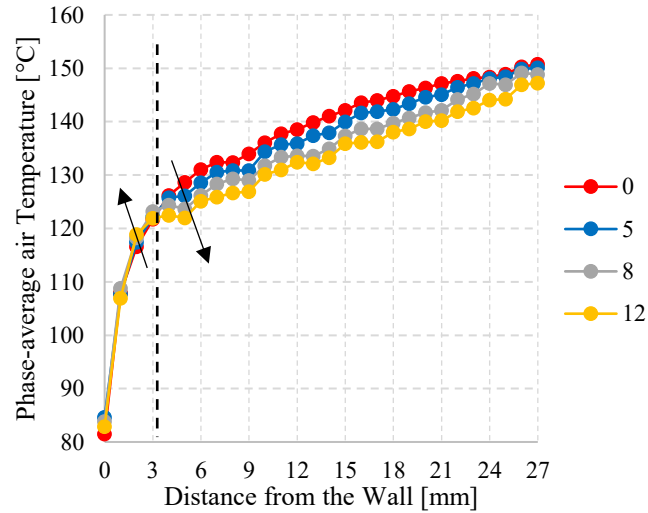
Figure 100: Phase-average air temperature profile for a pulsating hot flow during periodic flow reversal, Re = 30000 , f = 10 Hz
