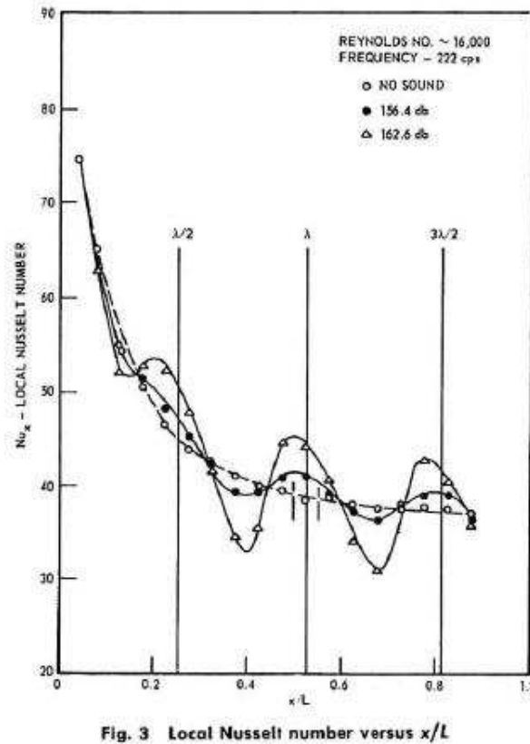
Figure 107: Local Nusselt numbers versus x/L for various sound pressure levels, Jackson et al.
