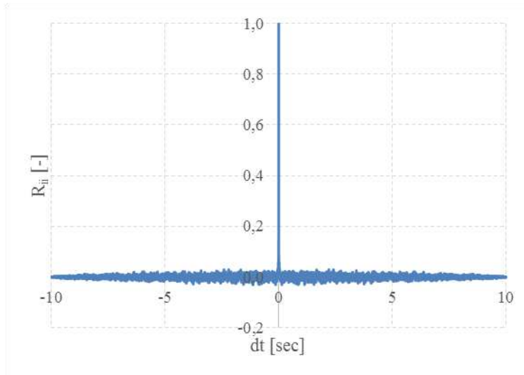
Figure 70: Autocorrelation of the velocity fluctuation component for a stationary flow, Re = 30000
