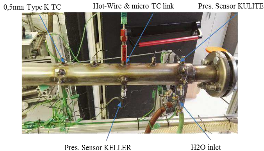
Figure 33: Test-Section detail
