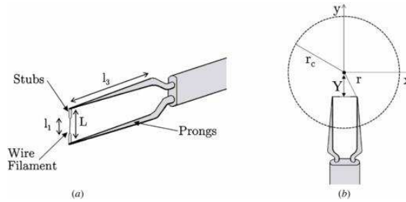
Figure 37: Hot-Wire Anemometer
