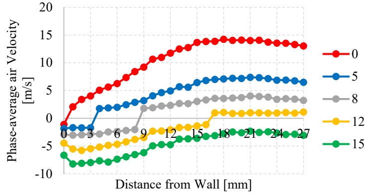
Figure 105: Phase-average air velocity profile for a pulsating cold flow during periodic flow reversal, Re = 40000 , f = 10 Hz
