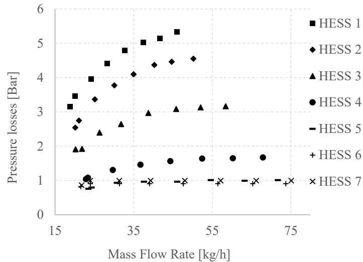
Figure 21: HESS Pressure losses in function of the MFR
