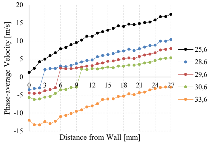
Figure 64: Phase-average axial velocity – Cold flow – ISO U_m , 20 Hz
