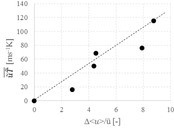
Figure 79: \tilde{u}\tilde{T} in function of \frac{\Delta\langle u \rangle}{\bar{u}}
