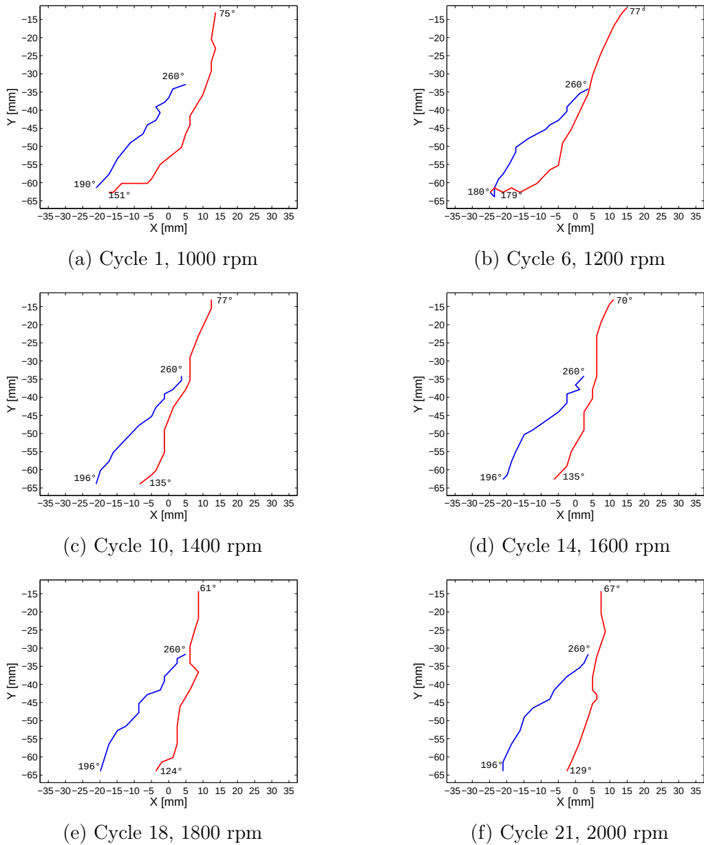
Figure 6.18: Trajectory of the tumble center for different engine speeds, Slow transient condition blue line: intake stroke, red line: compression stroke.
