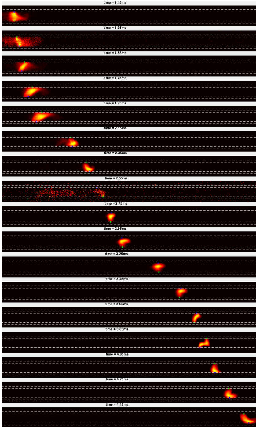
Figure 3.10: Parameter set 1, 230 V at 420 Hz with h = 5 mm. Sequence of frames from high-speed video imaging of the propagating arc. On each frame, the blue (x) denotes the cathode attachment while the green (x) indicates the anode attachment.
