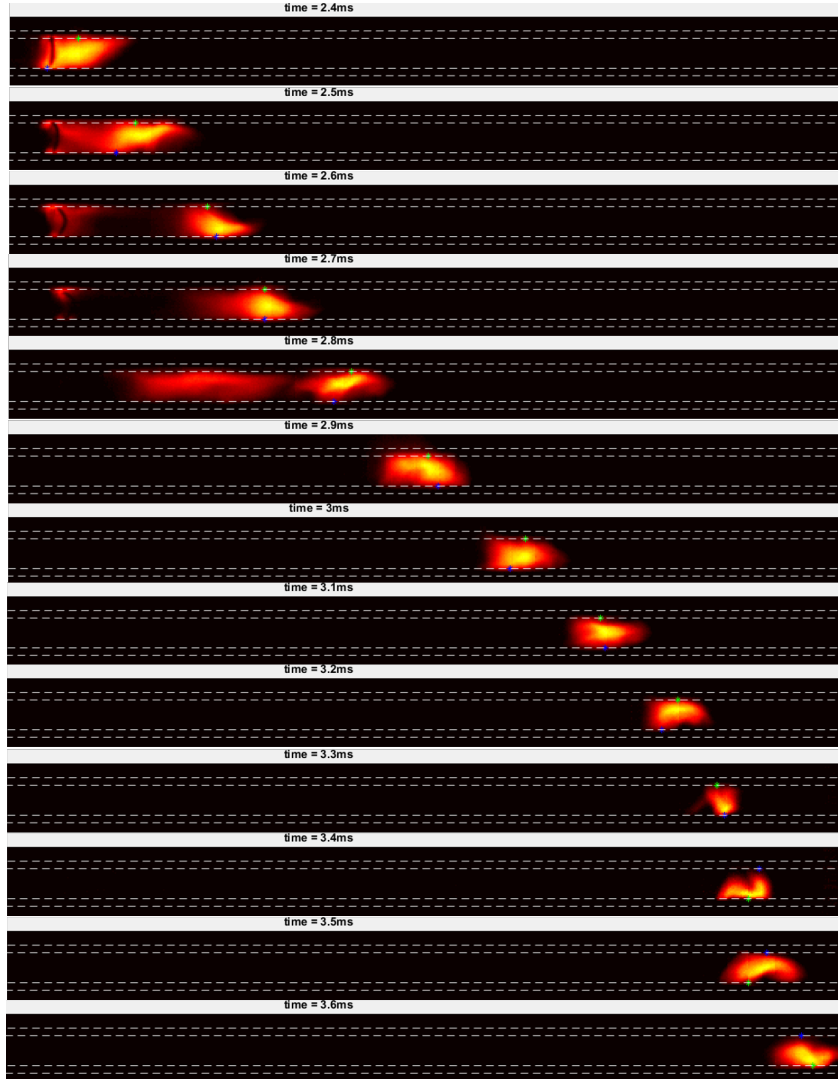
Figure 3.18: Parameter set 3, 115 V at 420 Hz with h = 5 mm. Sequence of frames from high-speed video imaging of the propagating arc. On each frame, the blue (x) denotes the cathode attachment while the green (x) indicates the anode attachment.
