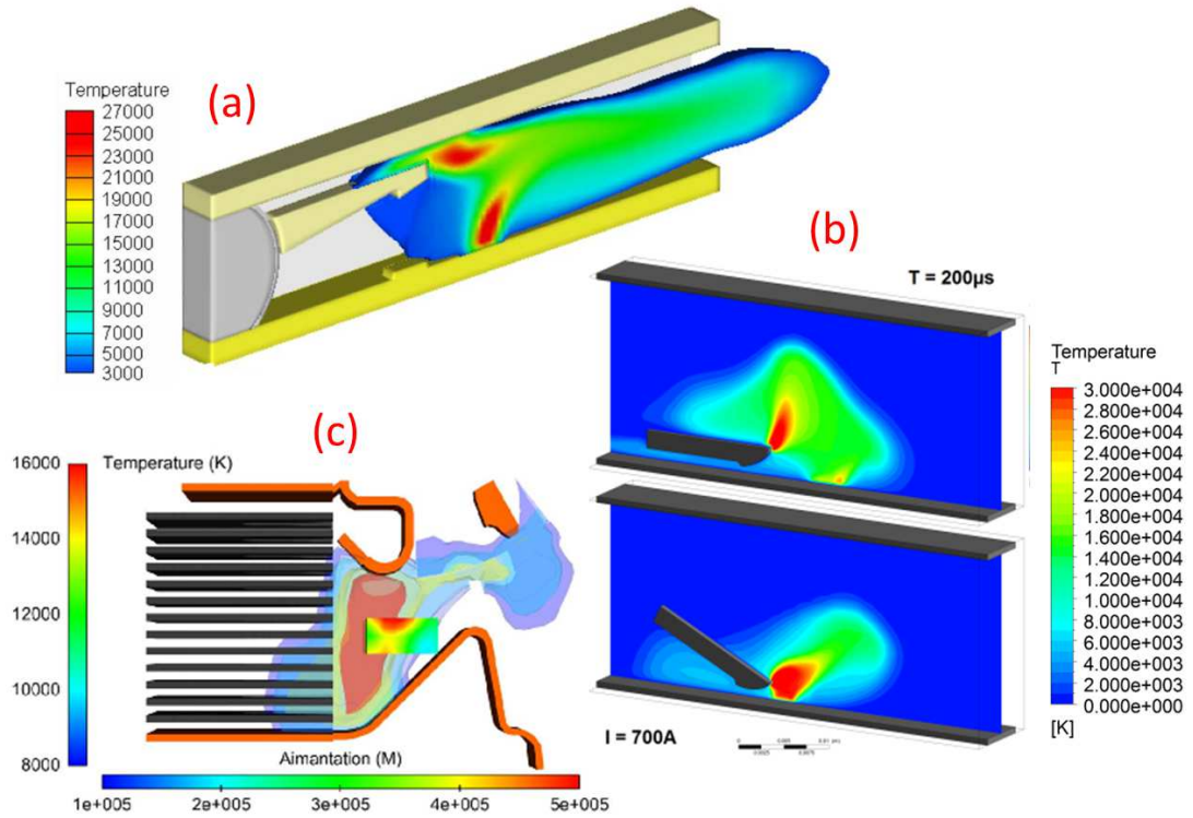
Figure 1.7: Three-dimensional temperature evolution of the arc plasma in air during the opening of the moving contact. (a) I = 1.5 \text{ kA} , t = 1.55 \text{ ms} [Wu 08b]; (b) I = 700 \text{ A} , t = 200 \mu\text{s} , for two mobile contact orientations [Quéméneur 17]; the arc temperature and the magnetization in the ferromagnetic plate, I_{max} = 4.5 \text{ kA} , 50 \text{ Hz} , t = 200 \mu\text{s} [Rondot 14].
