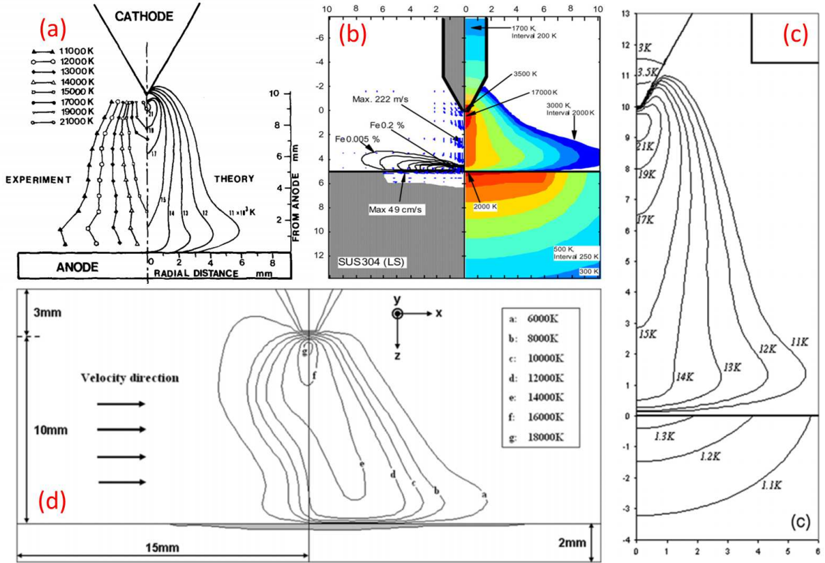
Figure 1.5: Examples of numerical simulations of free-burning electric arcs. DC current conditions, working gas is Ar. (a) Temperature isolines in the arc column experiment (left) and simulations (right), I = 200 A [Hsu 83a]; (b) Evaporation rate of the iron anode material (left) and temperature distribution in the arc and the electrodes (right), I = 150 A, 20 s after ignition [Tanaka 10]; (c) Temperature isolines in the arc and copper anode I = 200 A [Bini 06]; (d) Temperature isolines in the arc column, simulations are computed in 3D, where the inflow from the side has a velocity 20 m/s is introduced in order to disturb the arc symmetry [Lago 06].
