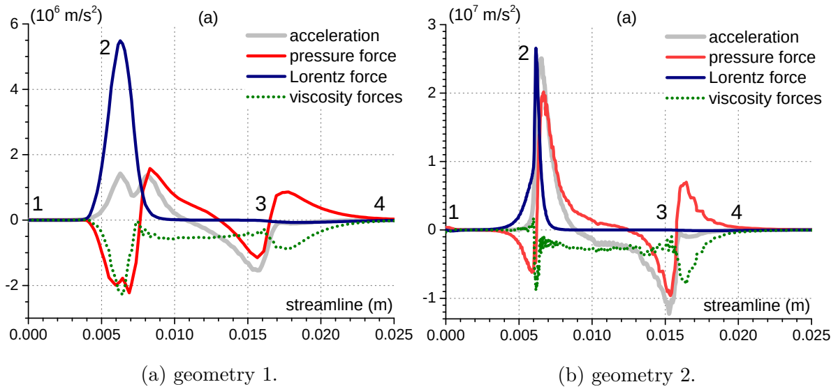
Figure 2.14: Forces and gas acceleration for the unit of mass distributions along streamline; I = 200 A.
