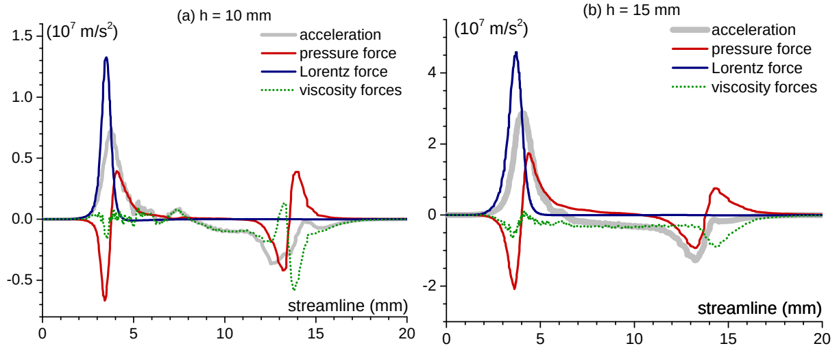
Figure 2.29: Forces and gas acceleration for the unit of mass distributions along streamlines for different cathode lengths; I = 200 A.
