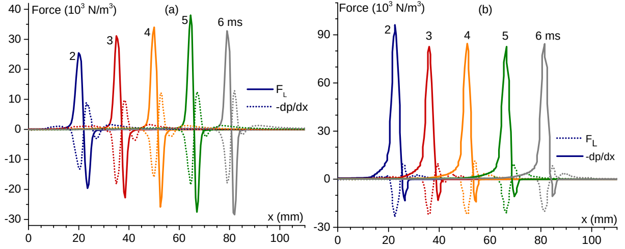
Figure 4.11: Forces (per unit of volume) acting on the plasma at (a) mid-plane longitudinal cut ( z = 10 mm); (b) near the anode. DC current I = 200 A at 1 atm. ( z = 19.5 mm)
