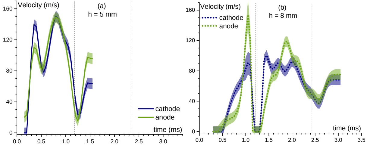
Figure 3.20: Parameter set 3, 115 V at 420 Hz. Temporal evolution of the cathode and anode root velocity for (a) h = 5 mm and (b) h = 8 mm electrode gaps.
