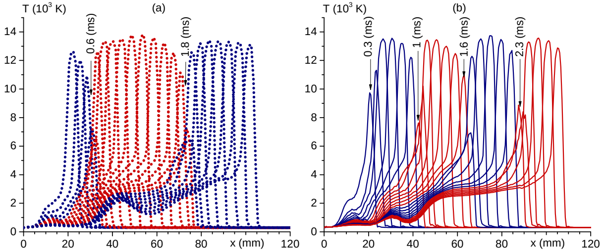
Figure 4.27: Time sequences of the arc temperature profile on the longitudinal mid-plane. I_{max} = 600 A and h = 8 mm for an oscillation frequency of, (a) 420 Hz and (b) 760 Hz. The time interval between two successive curves is 0.1 ms.
