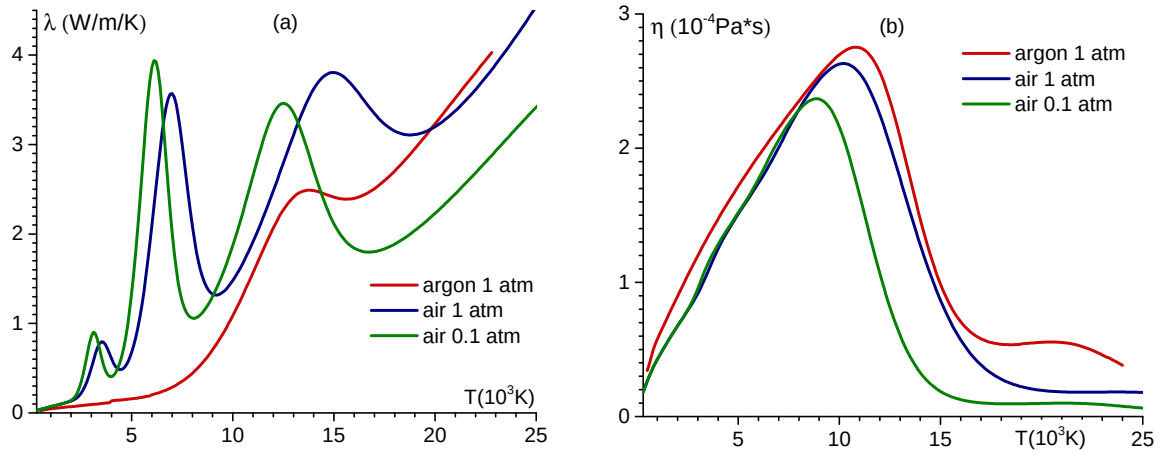
Figure 5.2: (a) Thermal conductivity, (b) Dynamic viscosity.
