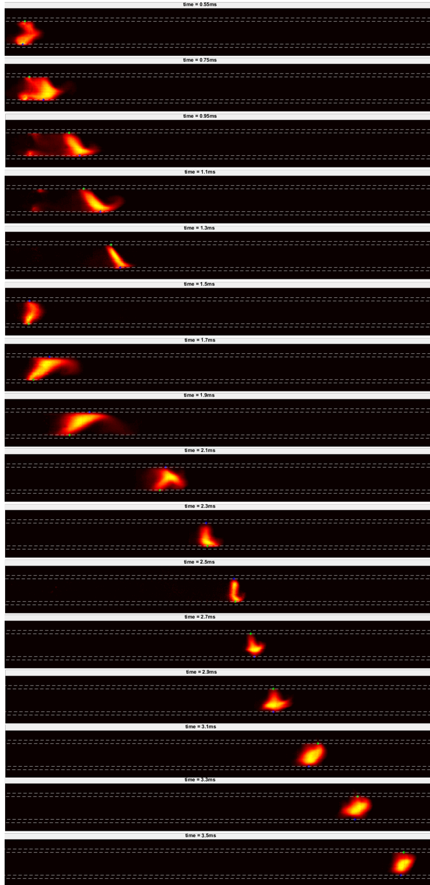
Figure 3.11: Parameter set 1, 230 V at 420 Hz with h = 8 mm. Sequence of frames from high-speed video imaging of the propagating arc. On each frame, the blue (x) denotes the cathode attachment while the green (x) indicates the anode attachment.
