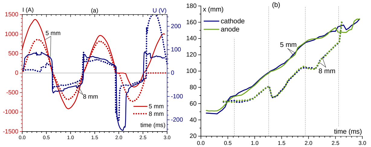
Figure 3.21: Parameter set 4, 115 V at 760 Hz with h = 5 mm and h = 8 mm electrode gap. (a) Waveforms of the arc current and arc voltage; (b) Time evolution of the cathode and anode attachments position.
