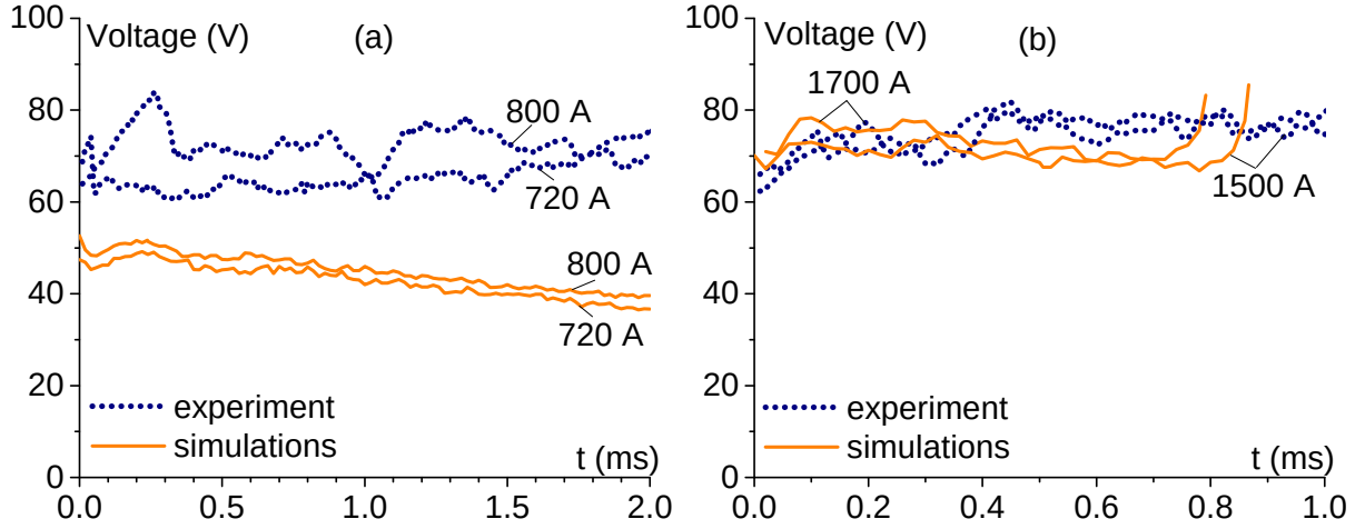
Figure 4.18: Comparison of the arc voltage recorded from the experiments with the simulated arc column voltage. (a) I_{max} < 1.0\text{ kA} , (b) I_{max} > 1.0\text{ kA} , at 1 atm.
