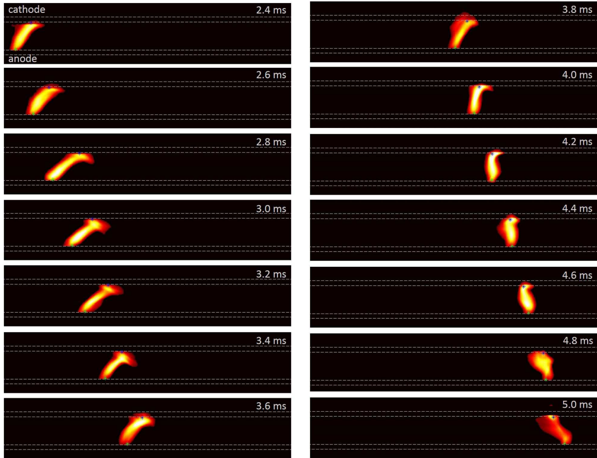
Figure 3.5: Sequence of images recorded by means of a high-speed video camera for a current pulse of I_{max} = 1.5 \text{ kA} . On each frame, the blue (*) denotes the cathode attachment while the green (*) indicates the anode attachment.
