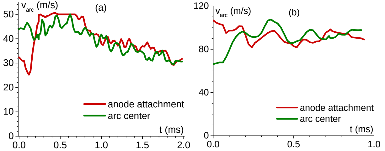
Figure 4.17: Arc displacement velocity for two current conditions, I_{max} = 800 A and (b) I_{max} = 1.5 kA at 1 atm.
