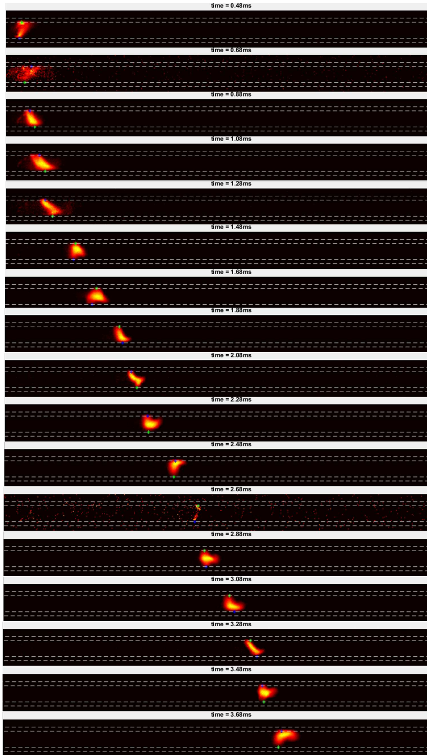
Figure 3.14: Parameter set 2, 230 V at 760 Hz with h = 5 mm. Sequence of frames from high-speed video imaging of the propagating arc. On each frame, the blue (x) denotes the cathode attachment while the green (x) indicates the anode attachment.
