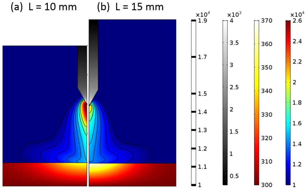
Figure 2.26: Temperature distributions in the LTE arc and the electrodes (in K); (a) L = 10 mm; (b) L = 15 mm. I = 200 A, 1 atm argon, thoriated-tungsten cathode, copper anode.
