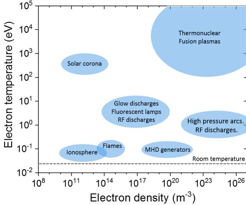
Figure 1.4: Classifications of plasmas adapted from [Boulos 94].
