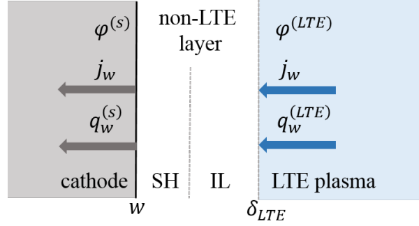
Figure 2.6: Schematic representation of the plasma-cathode interface.
