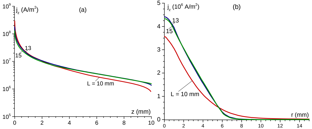
Figure 2.28: Axial component of the current density along the axis (a) and the radius with z = 5 mm (b); I = 200 A.
