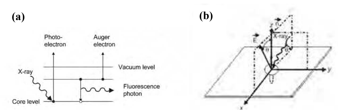
Figure I.10 – (a) Energy diagram of the photo-absorption process and the subsequent filling of the hole by emission of a photon or Auger electron. (b) Representation of the geometry of \pi^* vector orbitals (vertical to the xy plane) and \sigma^* planes (within the xy plane) with respect to the incident beam and the electric field vector, E [204].
