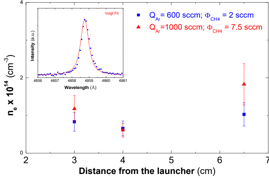
Figure II.25 – Axial variation of the electron density. (inset) Emission profile of Balmer-beta line ( Q_{Ar} = 1000 sccm, Q_{CH_4} = 7.5 sccm, P = 1kW , z = 3 cm) Material characterization
