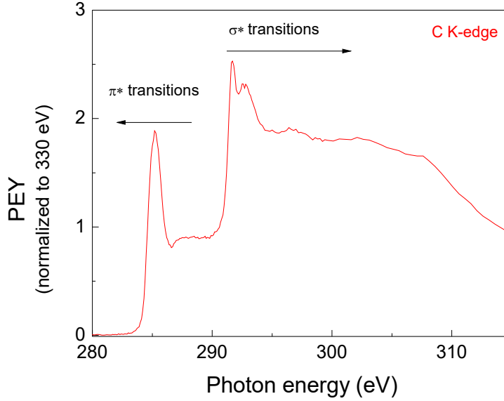
Figure II.16 - NEXAFS spectrum at C K edge of the graphene sheets synthesized at P = 2 kW, Q_{Ar} = 1200 sccm and Q_{Eth} = 30 sccm and applied IR radiation ( T_{wall} = 240^\circ\text{C} ). Normalized to the absorption jump, with post-edge intensity at 330.0 eV is set at 1 [222].
