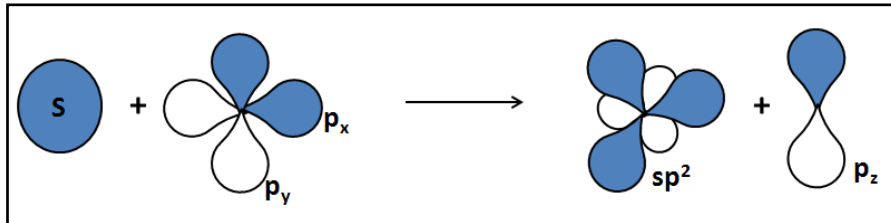
Figure I.2 - Graphene orbitals configuration
