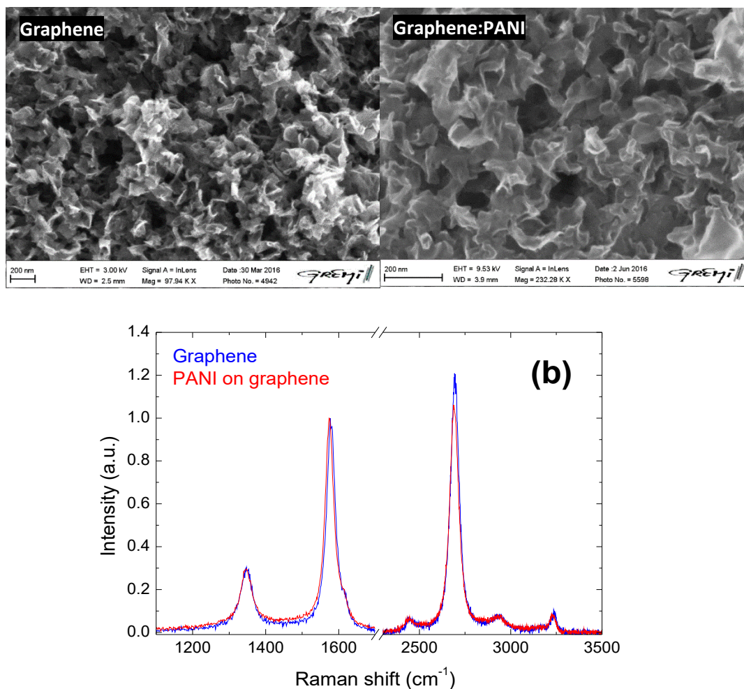
Figure II.60 – SEM images of graphene before and after plasma polymerization and respective Raman spectra. PANI plasma polymerization P= 5W , f= 25 Hz, p= 0.18 mbar, Q_{Ar}= 20 sccm and Q_{ANI}=1 sccm.
