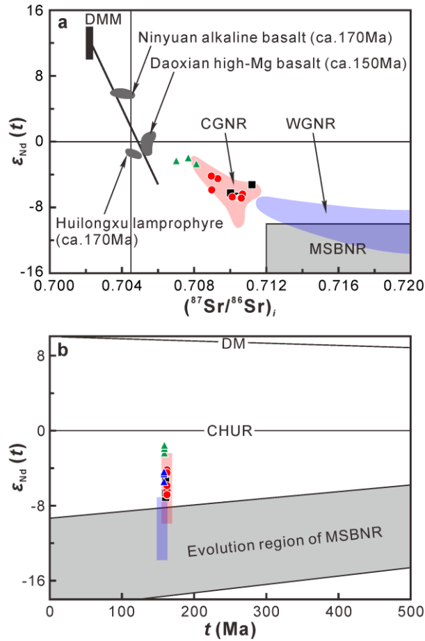
Figure 4-8. Sr-Nd isotopic compositions of granitoids from the Tongshanling-Weijia area. (a) \epsilon_{Nd}(t) -( ^{87}Sr/^{86}Sr ) i diagram, the Sr-Nd isotopic compositions of the Precambrian metasedimentary basement of the Nanling Range (MSBNR) are from Zhu et al. (2008) and Xie et al. (2013) , the Ninyuan alkaline basalt and Daoxian high-Mg basalt are from Li et al. (2004) and Jiang et al. (2009) , and the Huilongxu lamprophyre are from Wang et al. (2003b) . (b) \epsilon_{Nd}(t) - t (Ma) diagram, the Nd isotopic evolution region of the Precambrian metasedimentary basement of the Nanling Range are from Sun et al. (2005) . The legends and data sources of the Middle-Late Jurassic Cu-Pb-Zn-bearing (CGNR) and W-bearing (WGNR) granitoids in the Nanling Range are the same as Figure 4-6 .
