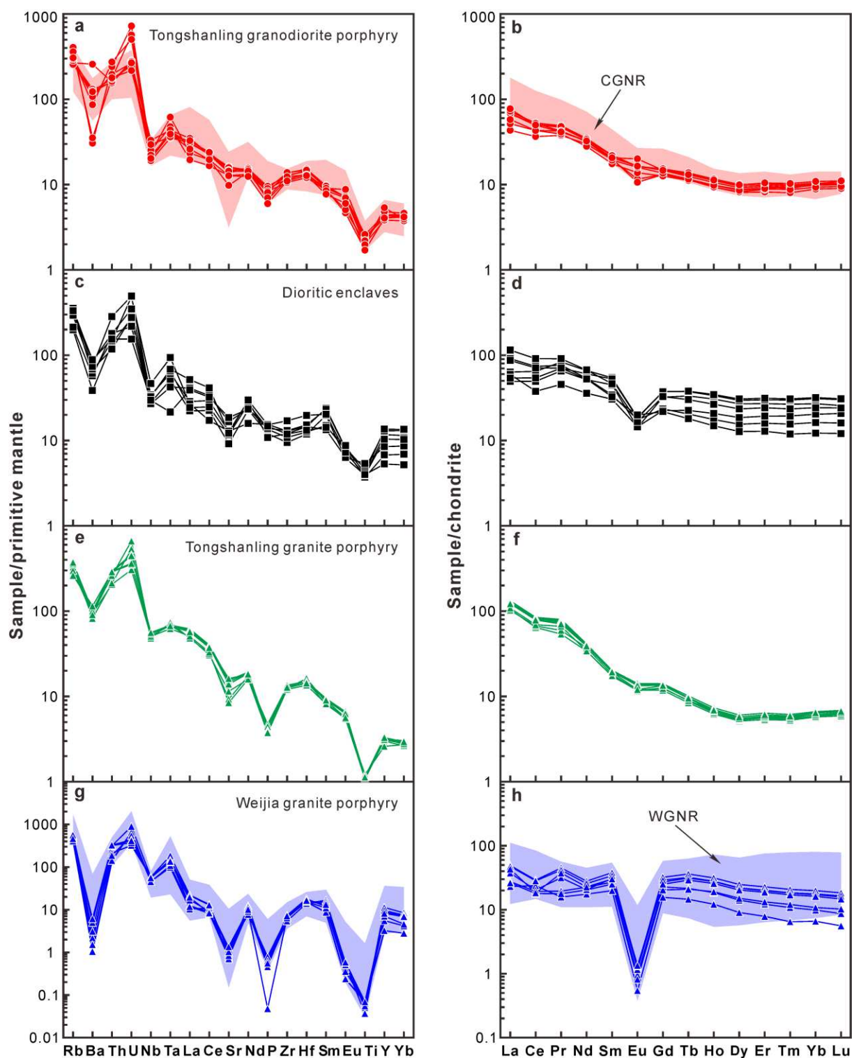
Figure 4-7. Primitive mantle-normalized (Sun and Mcdonough, 1989) spider diagrams and chondrite-normalized (Boynton, 1984) REE patterns of granitoids from the Tongshanling-Weijia area. The legends and data sources of the Middle-Late Jurassic Cu-Pb-Zn-bearing (CGNR) and W-bearing (WGNR) granitoids in the Nanling Range are the same as Figure 4-6.
