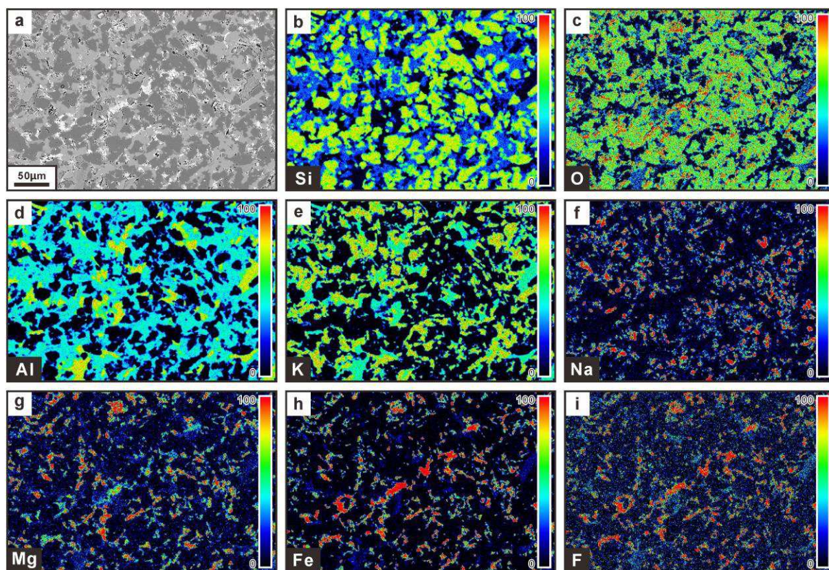
Figure 8-18. EDS elemental mapping of the matrix of the altered Weijia granite close to the magnesian skarn.
