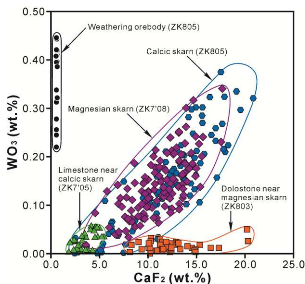
Figure 8-15. Binary plot of \text{CaF}_2 and \text{WO}_3 grades in representative drill cores of the magnesian and calcic skarns in the Weijia W deposit. The data sources are the same as Figure 8-14 .
