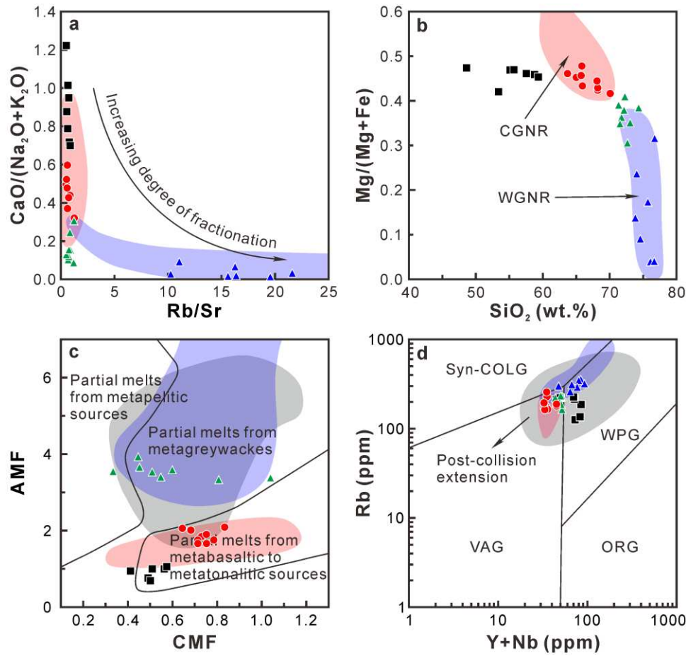
Figure 4-9. (a) \text{CaO}/(\text{Na}_2\text{O}+\text{K}_2\text{O}) -Rb/Sr diagram. (b) \text{Mg}/(\text{Mg}+\text{Fe}) - \text{SiO}_2 (wt.%) diagram. (c) AMF-CMF diagram, after Altherr et al. (2000), AMF = molar \text{Al}_2\text{O}_3/(\text{MgO}+\text{FeO}_{\text{Total}}) , CMF = molar \text{CaO}/(\text{MgO}+\text{FeO}_{\text{Total}}) . (d) Rb (ppm)-(Y+Nb) (ppm) diagram, after Pearce et al. (1984) and Förster et al. (1997), Syn-COLG: syn-collision granites; VAG: volcanic arc granites; WPG: within plate granites; ORG: ocean ridge granites. The legends and data sources of the Middle-Late Jurassic Cu-Pb-Zn-bearing (CGNR) and W-bearing (WGNR) granitoids in the Nanling Range are the same as Figure 4-6.
