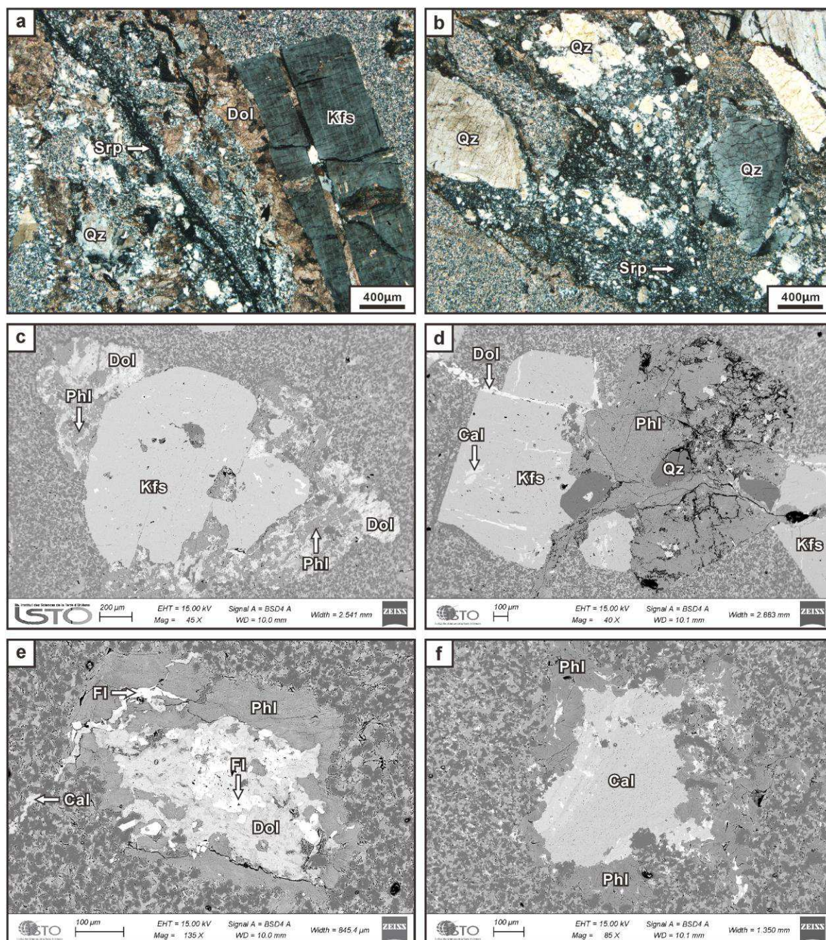
Figure 8-5. Petrographic photomicrographs (crossed-polarized light) and BSE images of the altered Weijia granite near the magnesian skarn. (a) Serpentine cuts the granite as veinlet coexisting with abundant dolomite. (b) Serpentine brecciates and replaces the quartz phenocryst. (c) K-feldspar phenocryst replaced by phlogopite and dolomite with a residual core. (d) Pseudomorphic replacement of a K-feldspar phenocryst by phlogopite. (e) Alteration mineral clot constituted by a core of dolomite and fluorite and a rim of phlogopite. (f) Alteration mineral clot constituted by a core of calcite and a rim of phlogopite. Mineral abbreviations: Cal = calcite, Dol = dolomite, Fl = fluorite, Kfs = K-feldspar, Phl = phlogopite, Qz = quartz, Srp = serpentine.
