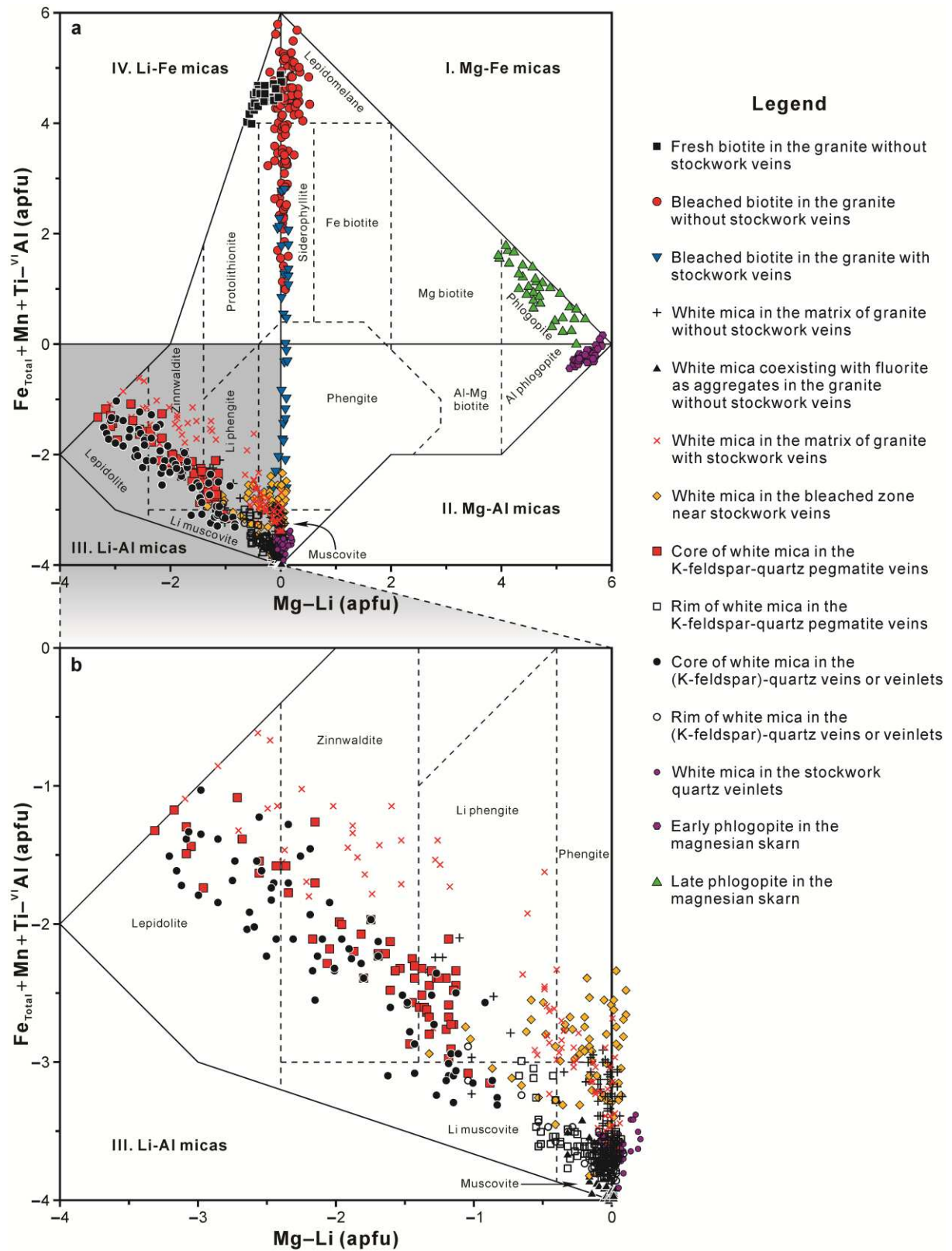
Figure 8-23. (\text{Fe}_{\text{Total}} + \text{Mn} + \text{Ti} - \text{VIAl}) (apfu)- (\text{Mg} - \text{Li}) (apfu) classification diagram of micas (after Tischendorf et al., 1997) from the Weijia W deposit.
