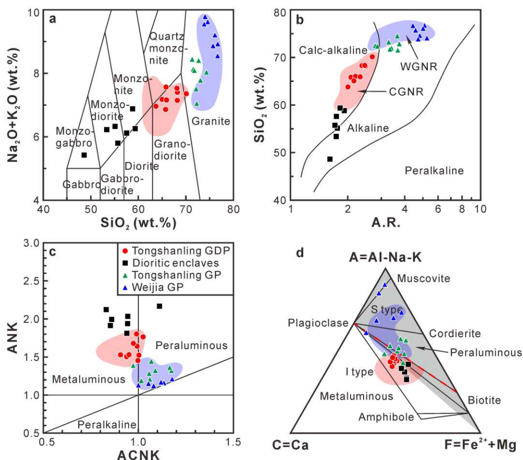
Figure 4-6. Major element diagrams of granitoids from the Tongshanling-Weijia area. (a) TAS [(Na 2 O+K 2 O) (wt.%) - SiO 2 (wt.%) ] classification diagram, after Middlemost (1994) . (b) SiO 2 (wt.%) - A.R. diagram, after Wright (1969) . (c) ANK - ACNK diagram. (d) ACF diagram, after Hine et al. (1978) . GDP: granodiorite porphyry; GP: granite porphyry. The whole-rock geochemical data of the Middle-Late Jurassic Cu-Pb-Zn-bearing granitoids in the Nanling Range (CGNR) are from Wang et al. (2003a) , Jiang et al. (2009) , Xie et al. (2013) , Zuo et al. (2014) , Zhao et al. (2016b) , and unpublished data from our research group; the whole-rock geochemical data of the Late Jurassic W-bearing granites in the Nanling Range (WGNR) are from Zhang (2004) , Zhang (2014) , Zhao et al. (2016b) , and unpublished data from our research group.
