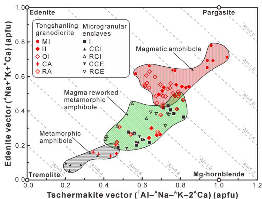
Figure 5-11. Plot of the generalized tschermakite [ (^{T}\text{Al}-^{A}\text{Na}-^{A}\text{K}-2^{A}\text{Ca}) (apfu)] vs. edenite [ (^{A}\text{Na}+^{A}\text{K}+^{A}\text{Ca}) (apfu)] components for amphibole from the Tongshanling granodiorite and its microgranular enclaves (after Schumacher, 2007). Legends are the same as Figure 5-4.
