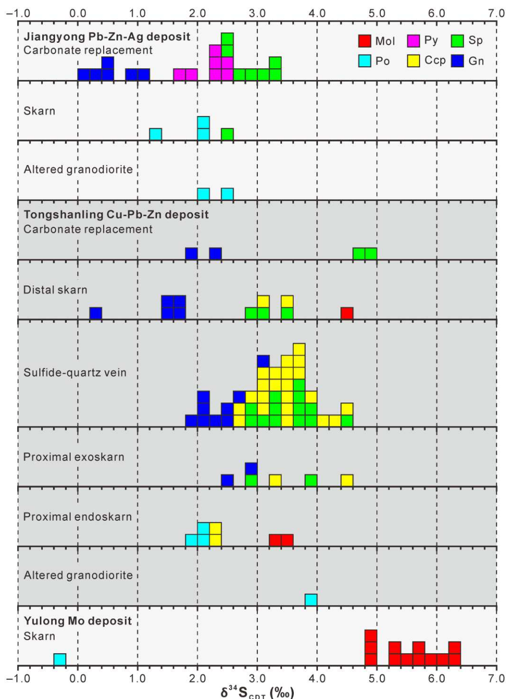
Figure 7-13. S isotopic compositions of sulfide minerals from the Tongshanling Cu-Pb-Zn deposit, Jiangyong Pb-Zn-Ag deposit, and Yulong Mo deposit. Mineral abbreviations: Ccp = chalcopryite, Gn = galena, Mol = molybdenite, Po = pyrrhotite, Py = pyrite, Sp = sphalerite.
