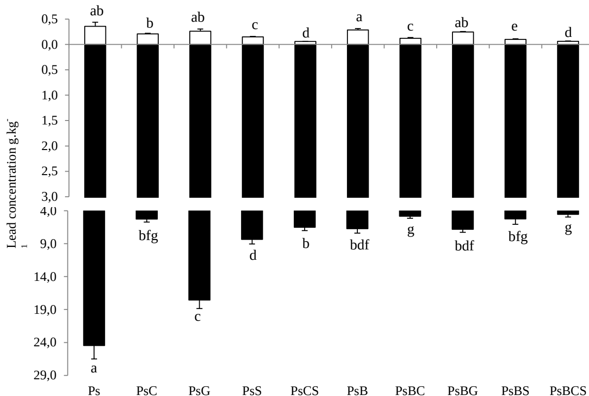
Figure 3.3: Lead concentrations (g.kg -1 ) in dwarf bean organs (aerial parts (white column), roots (black column)) at the end of the experiment period (13 days). (P): Pontgibaud soil, (PC): P + Compost (C) 5%, (PG): P + Garden soil (G) 5%, (PS): P + Slag (S) 2.5%, (PCS): P + C 5% + S 2.5%, (PB): P + Biochar (B) 2%, (PBC): P + B 2 % + C 5% , (PGB): P + B 2% + G 5%, (PBS): P + B 2% + S 2.5%, (PBCS): P + B 2% + C 5% + S 2.5%. Results are expressed as the mean value and standard error (n=10), letters on bar graphs indicate a significant difference (p<0.05).
