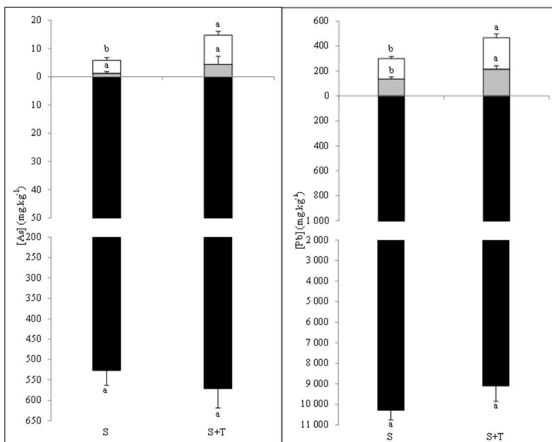
Figure 3.8 : Arsenic concentration (a) and lead concentration (b) (mg.kg -1 ) in the different Salix organs: leaves (whites columns, stems (greys columns) and roots (blocks columns) placed on the Pontgibaud soil amended with biochar for 3 modalities at the end of the experiment (T105). Vegetated only with clover (T), vegetated only with willow (S), and the combination of willow and clover (S+T). The lowercases letters indicate a significant difference for modalities.
