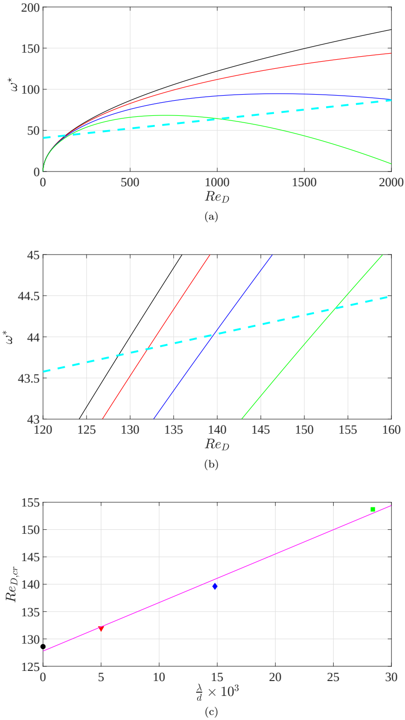
Figure 6.24 – Model for the production of vorticity at the surface of a sphere. (—), no-slip \lambda = 0 \mu\text{m} . (—), \lambda = 25 \mu\text{m} . (—), \lambda = 74 \mu\text{m} . (—), \lambda = 142 \mu\text{m} . (a) non-dimensional vorticity \omega^* as a function of the Reynolds number Re_D (see Eq. 6.36). (---), empirical law by Magnaudet & Mougin (2007), reported in Eq. 6.37. (b), detail of the critical region in (a). (c), critical Reynolds number Re_{D,cr} as a function of the non-dimensional slip length \frac{\lambda}{d} . (—), fit of the data in the least-mean squares sense.
