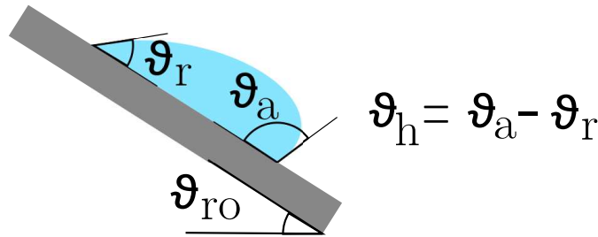
Figure 3.3 – Definition of roll-off angle \vartheta_{ro} as the lowest tilt angle that forces the drop to be removed from the solid surface. In the case of SH materials, the drop tends to roll-off rather than slide. The hysteresis angle \vartheta_h is defined as the difference of the advancing \vartheta_a and receding \vartheta_r angles.
