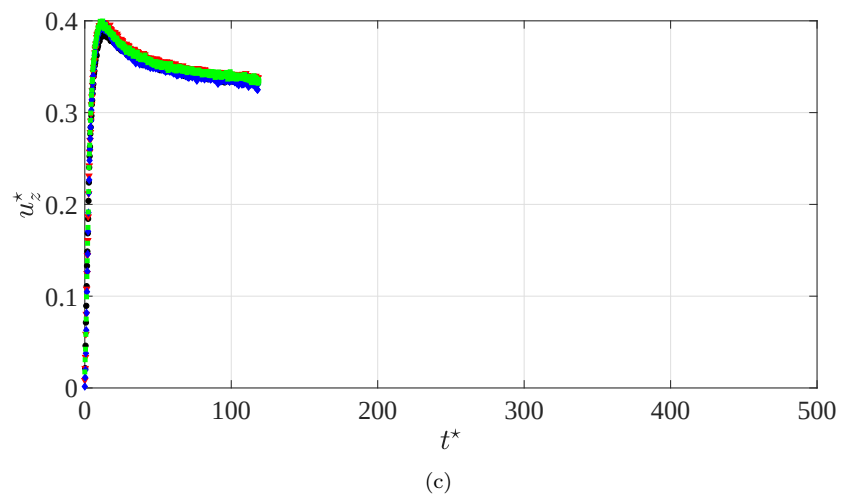
Figure 6.3 – Instantaneous vertical velocity u_z^* for all the analysed coatings in the glycerine tests. \bullet , reference. \blacktriangledown , SH-NAR. \blacklozenge , SH-220. \blacksquare , SH-80. (a), d = 5 mm. (b), d = 8 mm. (c), d = 10 mm.
