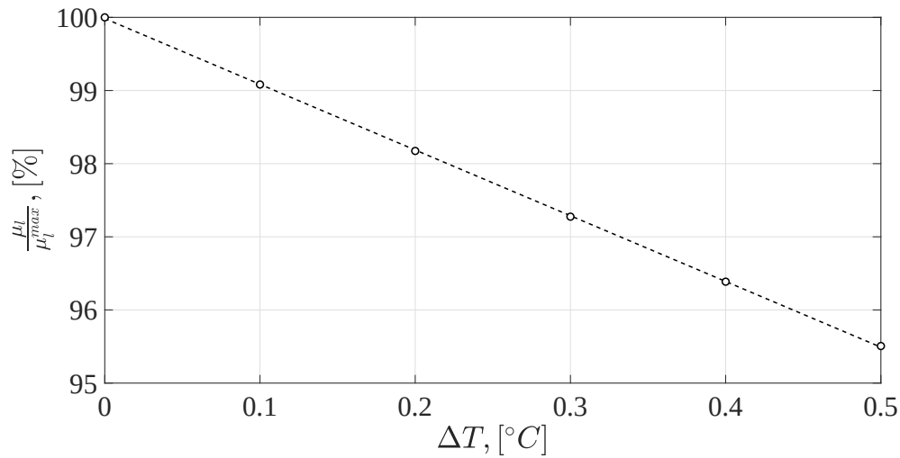
Figure 6.5 – Non-dimensional dynamic viscosity \frac{\mu_l}{\mu_l^{max}} variation as a function of an imposed temperature variation, according to the empirical laws by Cheng (2008) discussed in §4.3. (---), fit of the evaluated data to highlight the linear behaviour.
