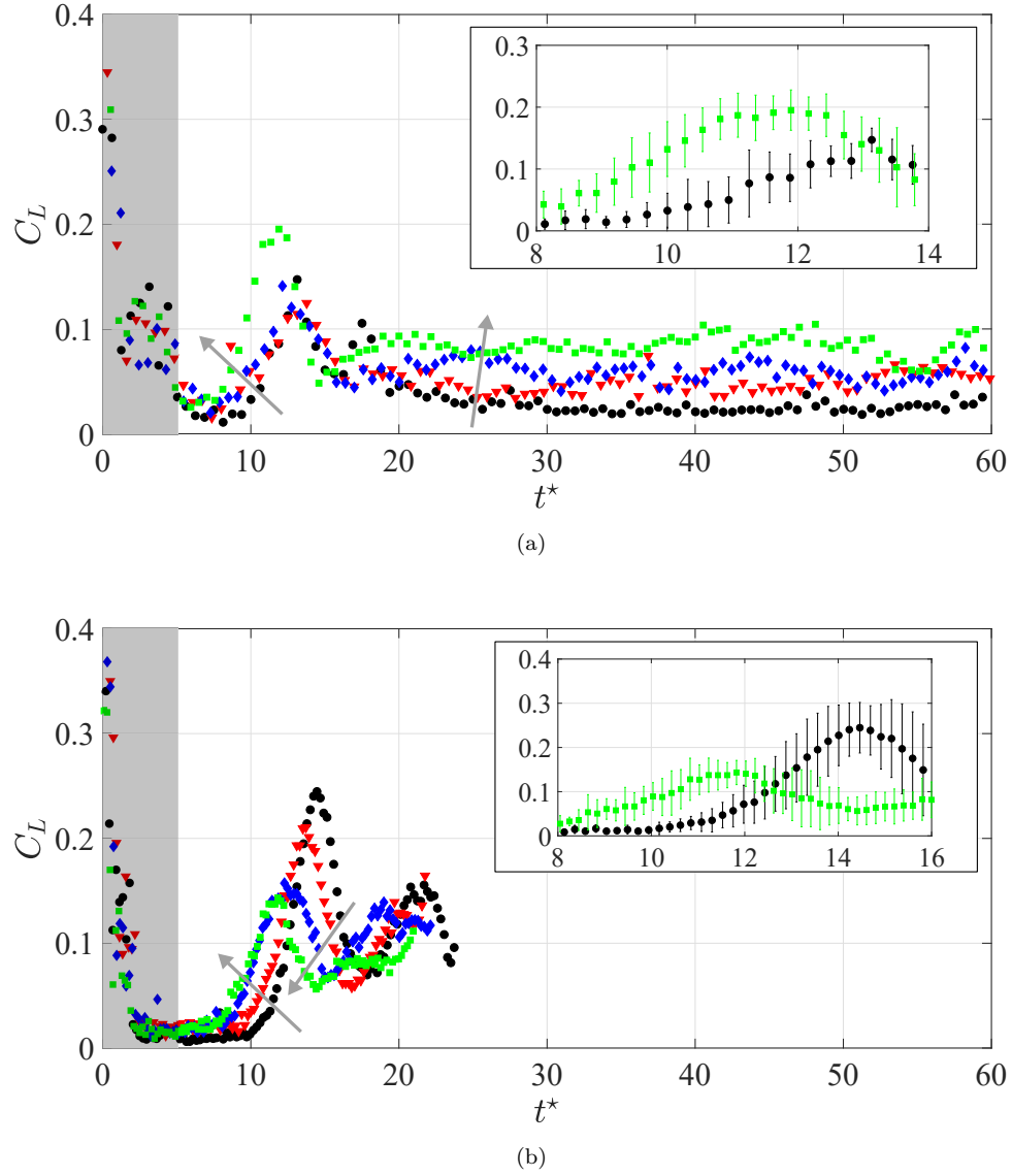
Figure 6.36 – Time evolution of the lift coefficient C_L for all the analysed coatings in pure water. (a), d = 5 mm. (b), d = 20 mm. •, reference. ▼, SH-NAR. ♦, SH-220. ■, SH-80. For the sake of clarity, one point out of two is reported. The grey arrows indicate increasing \frac{\lambda}{d} . The shaded regions identify the portion of drop where lift estimation is corrupted by low signal-to-noise ratio. The two inserts show the errorbars (95% confidence level) in the wake instability occurrence region.
