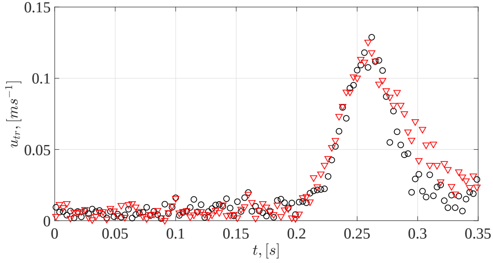
Figure 4.18 – Transversal velocity u_{tr} of a d = 10 mm stainless steel reference sphere in water in the region corresponding to the onset of transversal motion. \circ , one night settling time. \nabla , 15 min settling time. For the sake of clarity, one point out of three is reported. Non-significant differences between the two settling times are noticed.
