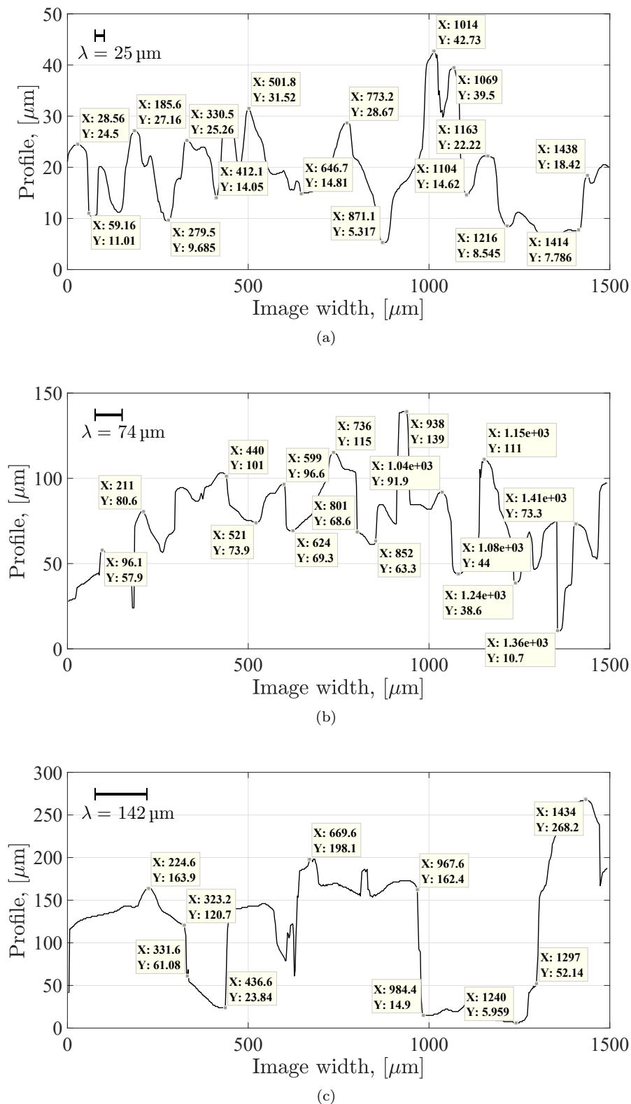
Figure 3.9 – Profilometer approach on 3D digital microscopy images. (a), SH-NAR. (b), SH-220. (c), SH-80. The black bars indicate the corresponding surface roughness \lambda . The same behaviour is retrieved by multiple profiles along the length of the available images.
