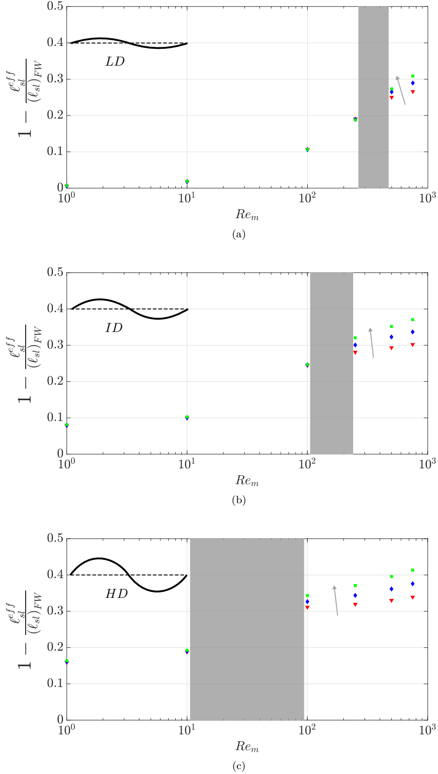
Figure 7.11 – Evolution of the normalised (with respect to the corresponding FW simulation with the same \ell_h ) effective slip length \ell_{sl}^{eff} over the whole analysed Re_m range. (a), LD configuration with \frac{\delta}{h} = 0.05 . (b), ID configuration with \frac{\delta}{h} = 0.075 . (c), HD configuration with \frac{\delta}{h} = 0.10 . \blacktriangledown , \ell_{sl} = 10 \mu m . \blacklozenge , \ell_{sl} = 50 \mu m . \blacksquare , \ell_{sl} = 100 \mu m . The gray arrows indicate increasing \ell_{sl} . The gray-shaded rectangles indicate the regions where the onset of recirculation inside the valleys of the lower wavy wall occurs.
