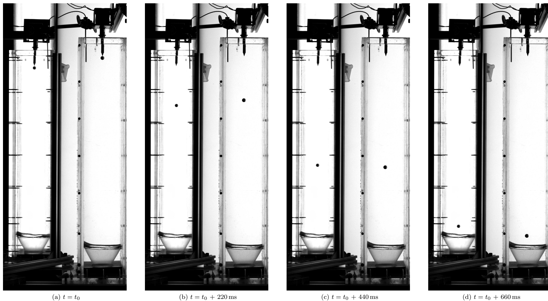
Figure 4.6 – Frames sampled from a drop of a d = 10 mm stainless steel reference sphere, recorded at 1000 fps. (a)-(d), increasing falling time, starting from the beginning of the drop (indicated by t_0 in (a)) until when the sphere reached the bottom of the tank (d). The left side of each image shows the side view, while the right side shows the front view. The bottom of the tank was made of a cone shaped outlet covered by a soft foam to avoid coating damage.
