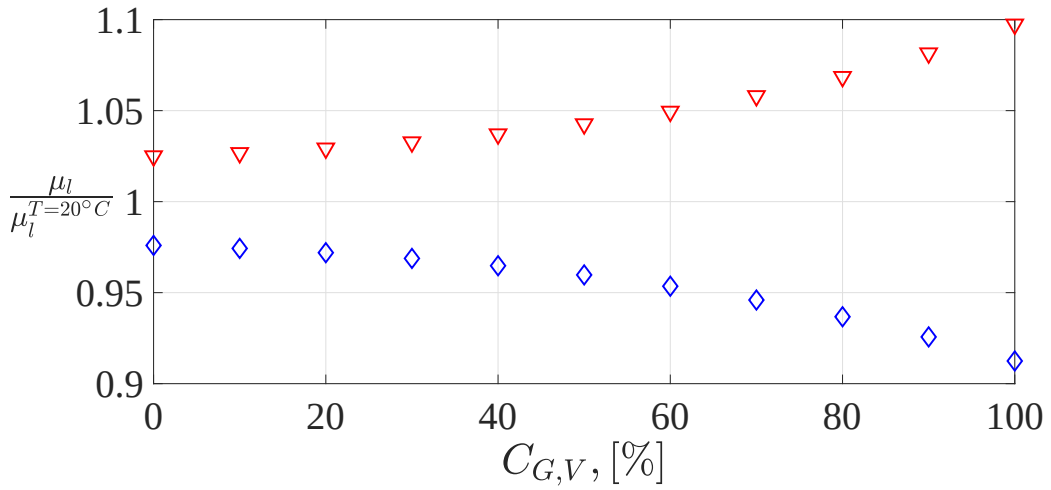
Figure 4.17 – Effect of the temperature on the evolution of the non-dimensional mixture dynamic viscosity \frac{\mu_l}{\mu_{l,T=20^\circ C}} for increasing glycerine volumetric fraction C_{G,V} . Data are evaluated from Eq. 4.12 and normalised with respect to the corresponding value at a temperature T = 20^\circ C . \nabla , T = 19^\circ C . \diamond , T = 21^\circ C .
