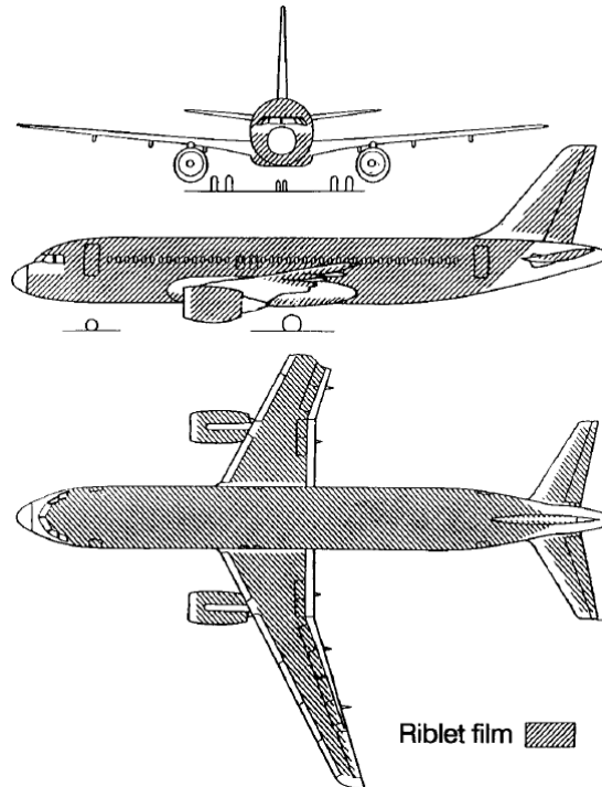
Figure 2.14 – Schematic of an A320 covered by a riblet film (adapted from Szodrich 1991). Approximately 70 % of the surface is coated, with a consequent 80 kg weight increase.
