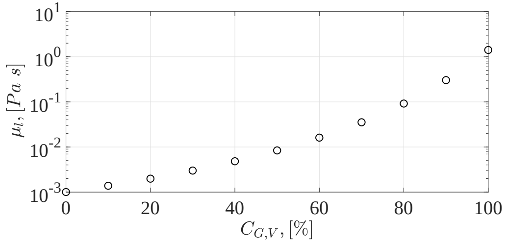
Figure 4.16 – Evolution of the mixture dynamic viscosity \mu_l for increasing glycerine volumetric fraction C_{G,V} . Data are evaluated from Eq. 4.12 at a temperature T = 20^\circ C .
