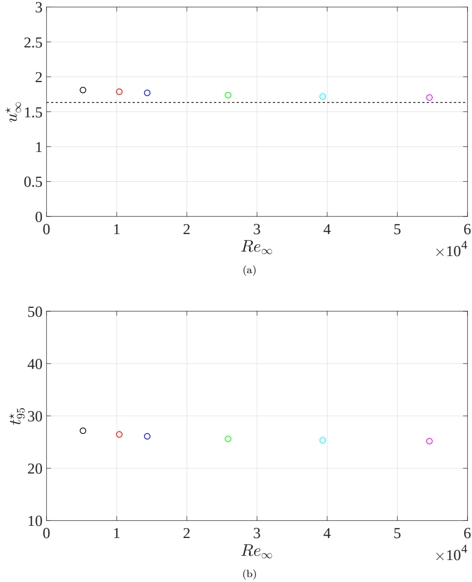
Figure 4.13 – Evolution of the non-dimensional characteristic parameters of the drop over a Reynolds number variation of one order of magnitude. (a), terminal velocity u_{\infty}^* = \frac{u_{\infty}}{u_D} . (---), prediction of the u_{\infty}^* value via evaluation of Eq. 4.3 at terminal conditions and considering C_{D\infty} = 0.5 , which is the typical value indicated in the analysed sub-critical regime. (b), transient time t_{95}^* = \frac{t_{95}}{t_D} . Same color code as in Fig. 4.10.
