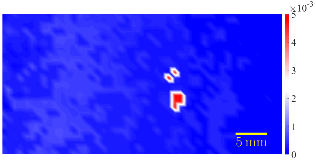
Figure A.3 – Preliminary estimation of the local air layer thickness t over a SH-NAR plate, obtained by solving the system of Eqs. A.5. The colorscale is expressed in m units.
