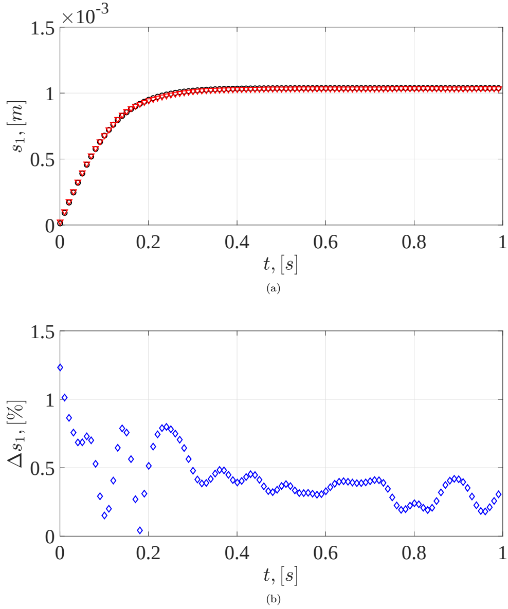
Figure 5.11 – Estimation of the instantaneous sphere vertical displacement s_1(t) for a d = 5 mm reference stainless steel sphere falling in pure water (W100_G000). (a), comparison between: \circ , synthetic profile imposed via Eq. 4.3 and \nabla , results of the cross-correlation code. (b), percentage difference (with respect to the displacement maximum value) on the displacement estimation (see Eq. 5.6).
