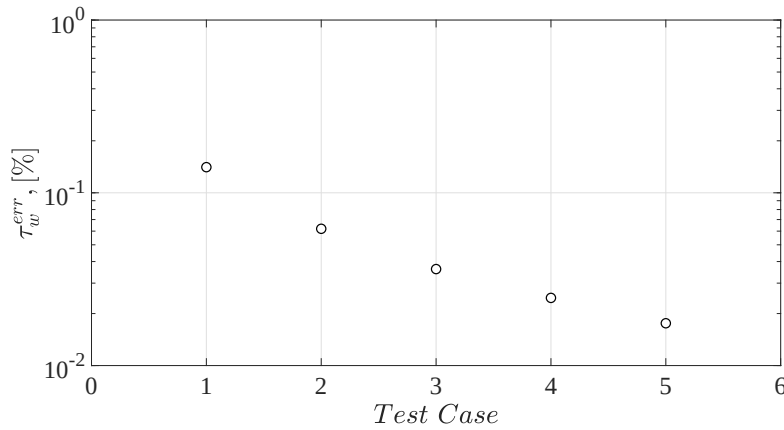
Figure G.5 – Variation of the relative error on the estimation of the wall shear stress \tau_w with respect to the analytical solution (Eq. 7.9(c)) in the case of a flat, no-slip lower wall ( \frac{\Lambda}{h} = 1 and \frac{\delta}{h} = 0 ) at Re_m = 1000 . The grid points per each wave are increased by 50 % on each consecutive test. The mesh selected for the execution of the 2D laminar numerical simulations corresponds to the test case #2.
