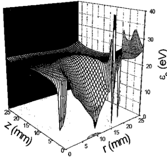
Figure 30: Costin's electrons mean energy \varepsilon_e (22 eV) [86].
