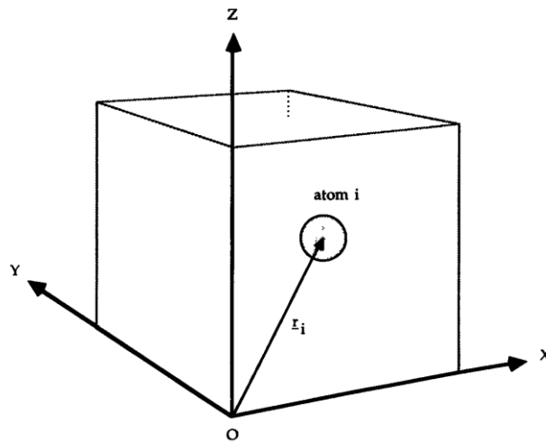
Figure 38: Cartesian, laboratory-fixed reference frame (X, Y, Z) used to define a position vector \vec{r}_i that locates atom i in a system [151].
