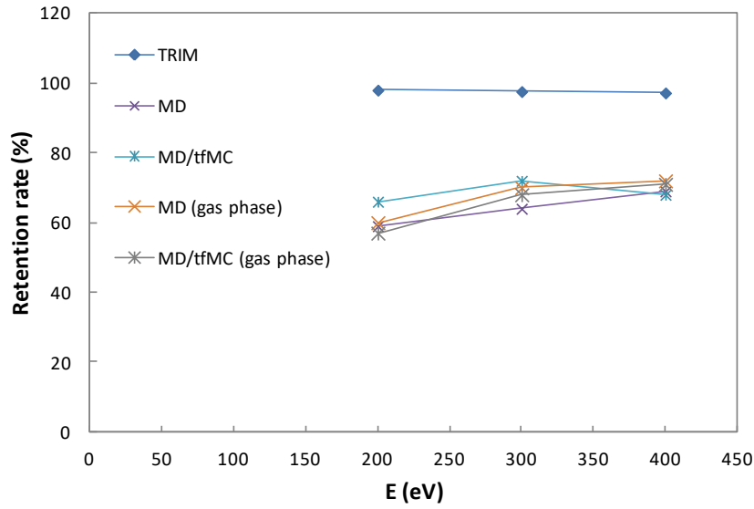
Figure 64: \text{Ar}^+ retention rate as a function of \text{Ar}^+ energies.
