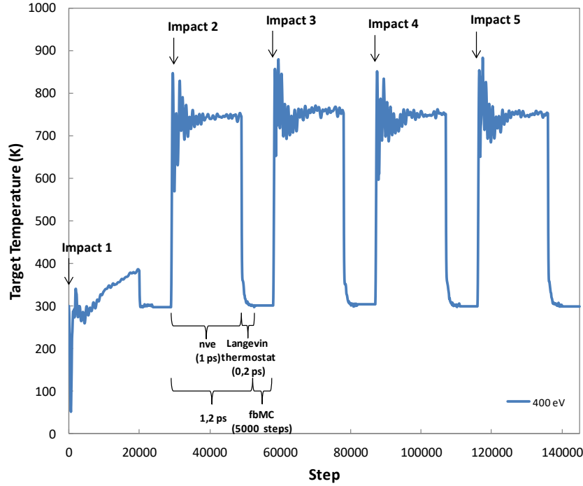
Figure 52: Evolution of the temperature in the thermostated region during 5 impacts of \text{Ar}^+ at 400 eV.
