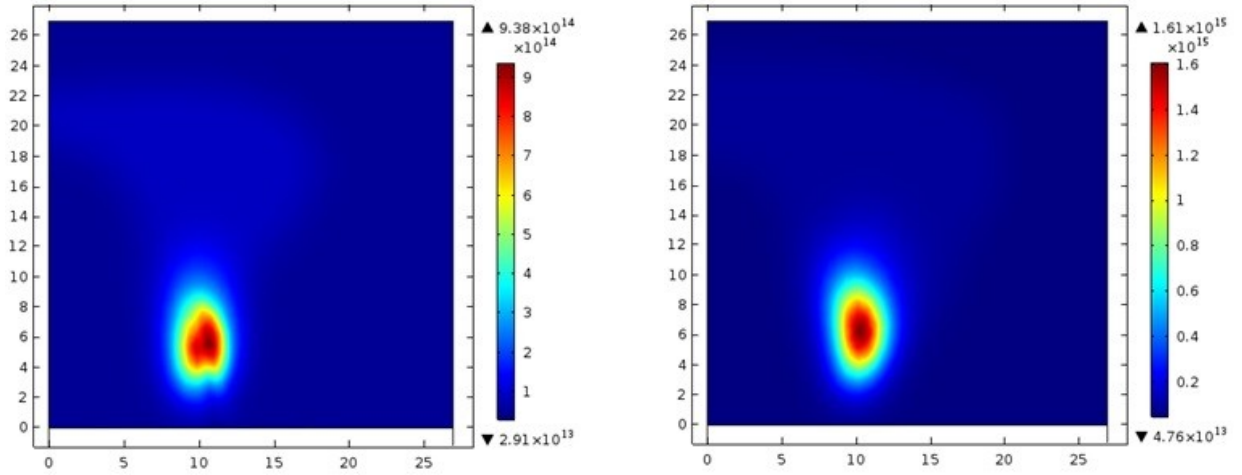
Figure 34: Electrons (left) and ions (right) densities for a magnetization of M_0/10 ( 1/\text{m}^3 ).
