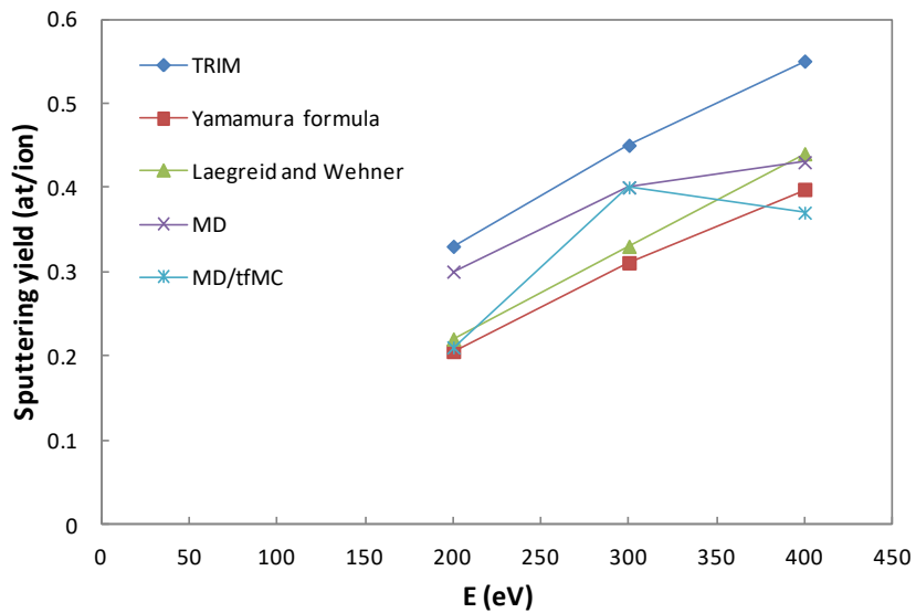
Figure 55: Ti sputtering yields as a function of \text{Ar}^+ energies.
