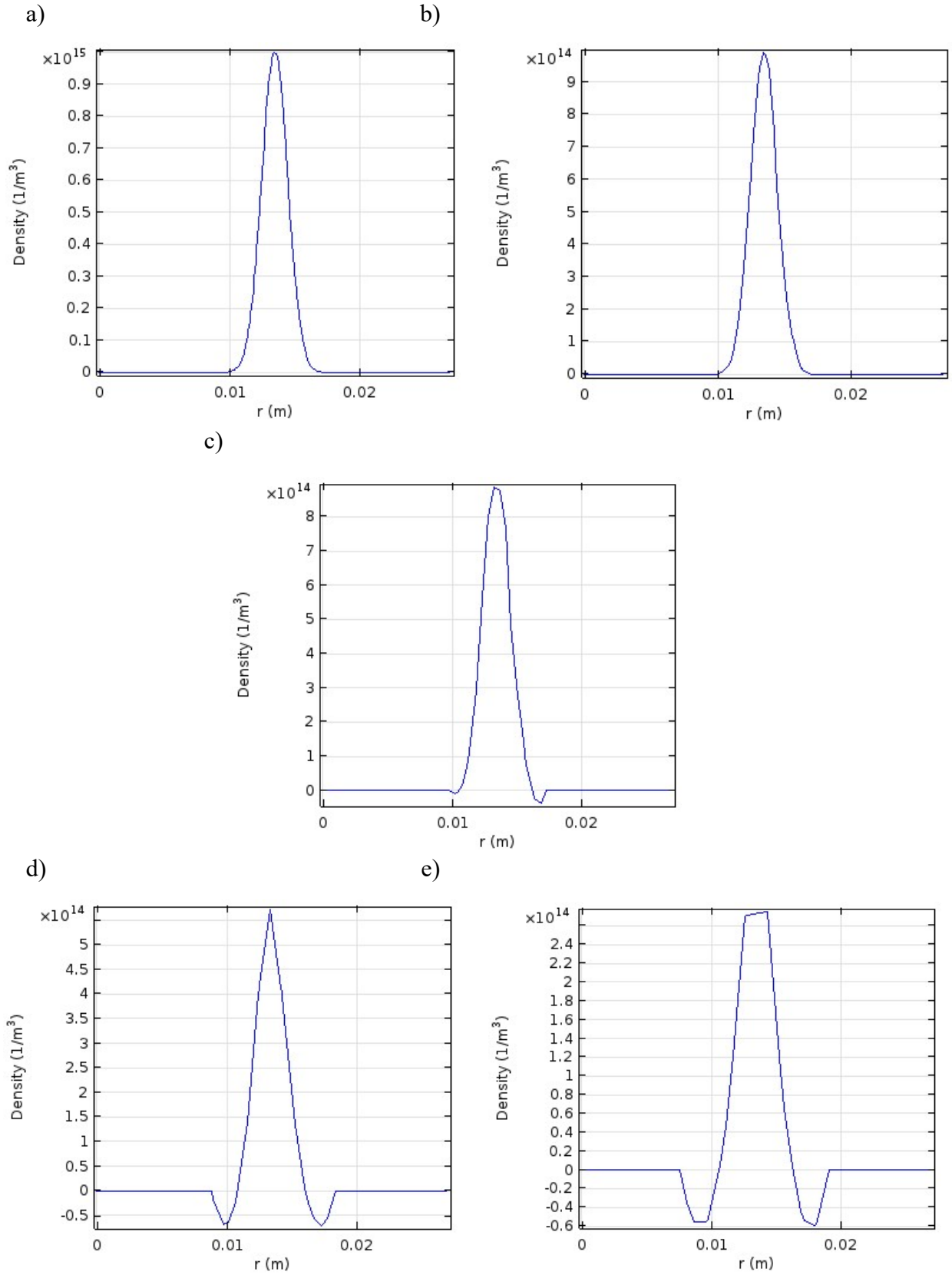
Figure 9: The profile of Gaussian density according to different meshes: a) Extremely Fine mesh, b) Finer mesh, c) Normal mesh, d) Coarser mesh and e) Extremely Coarse mesh.
