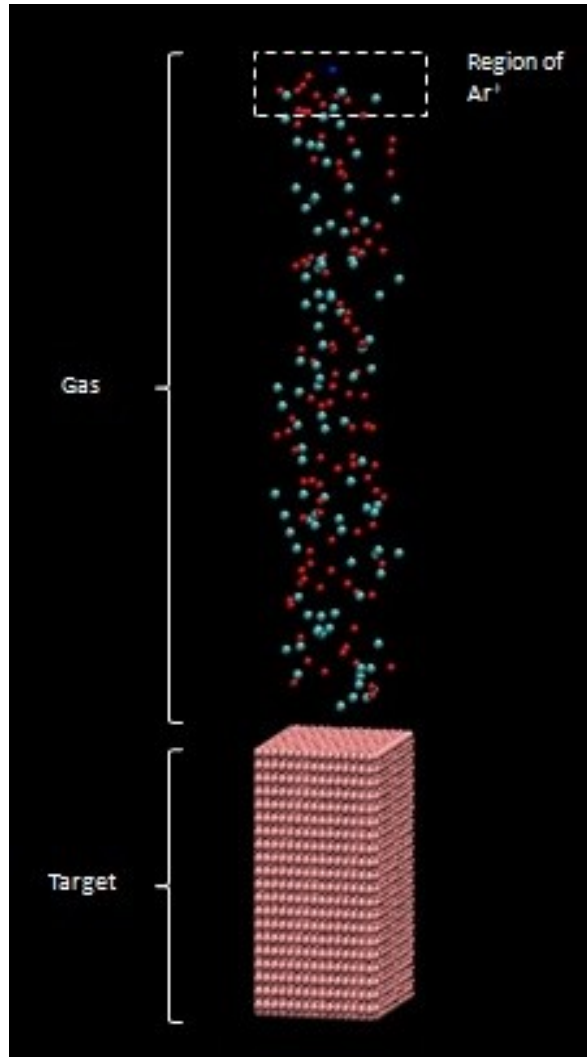
Figure 40: Initial configuration of the simulation of Ti reactive sputtering. The gas phase is composed of argon and oxygen. The color spheres of pink, red cyan and blue represent Ti, O, Ar and \text{Ar}^+ respectively.
