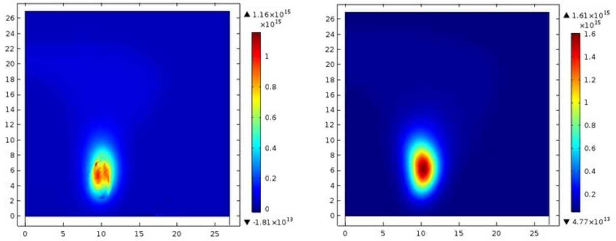
Figure 36: Electrons (left) and ions (right) densities for a magnetization of M_0/100 ( 1/\text{m}^3 ).
