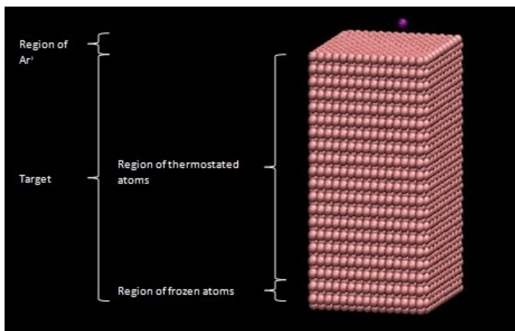
Figure 39: Initial configuration of the simulation of Ti sputtering. The color spheres of pink and purple represent Ti and \text{Ar}^+ respectively.
