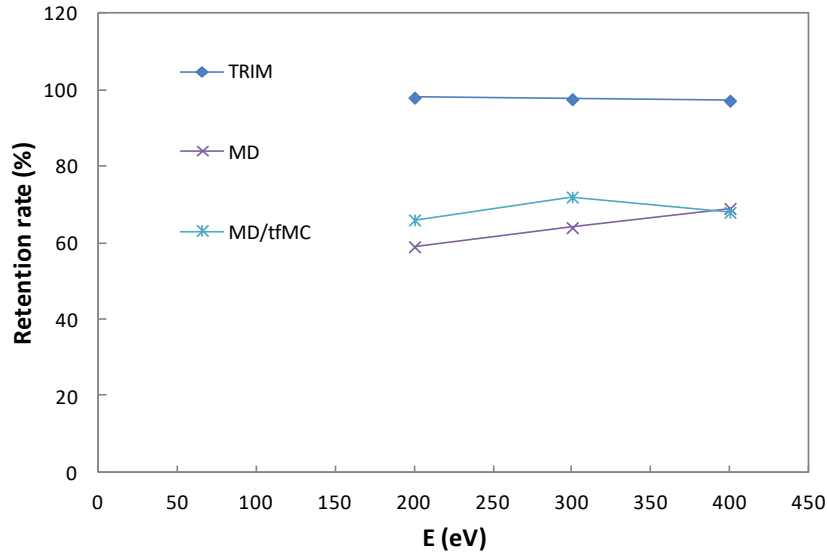
Figure 57: \text{Ar}^+ retention rate as a function of \text{Ar}^+ energies.
