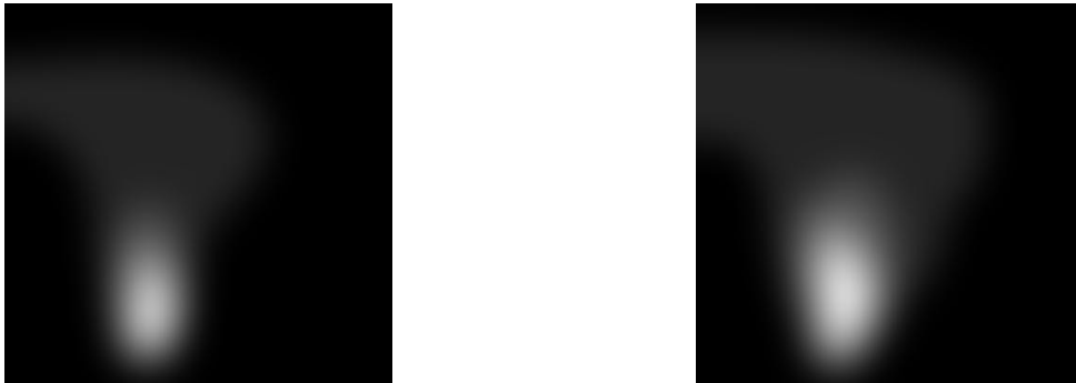
Figure 27: Electrons (left) and ions (right) densities input profiles.
