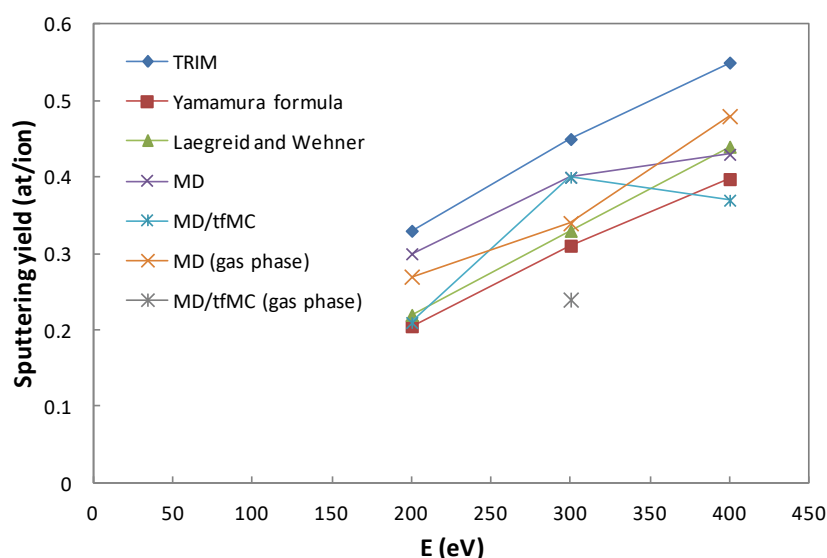
Figure 61: Ti sputtering yields as a function of \text{Ar}^+ energies.
