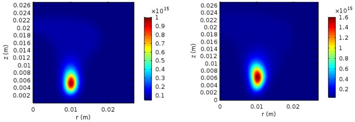
Figure 28: Input electrons (left) and ions (right) densities ( 1/\text{m}^3 ).
