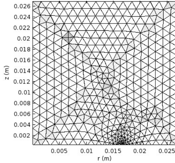
Figure 12: Finer mesh.
