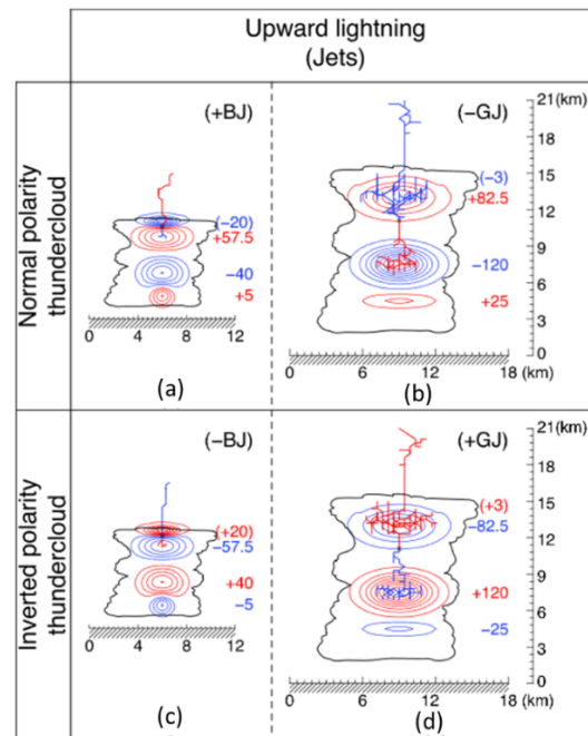
Figure 1-8. BJ and GJ simulation for normal- and inverted-polarity storms. Modified from Krehbiel et al. [2008].
