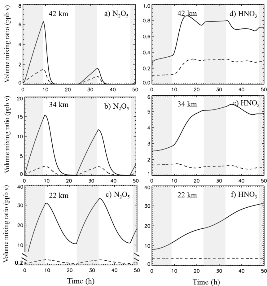
Figure 5-6. As in Figure 5-5, but for N_2O_5 and HNO_3 .
