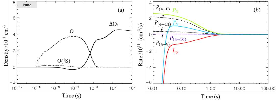
Figure 4-4. (a) Time evolution of densities of ground state atomic oxygen and excited \text{O}(^1\text{S}) , \Delta\text{O}_3 at 27 km. The shaded area indicates the time period of the electric pulse. (b) Loss and production rate densities of atomic oxygen associated with reactions (4-8)-(4-13) after 10^{-2} s.
