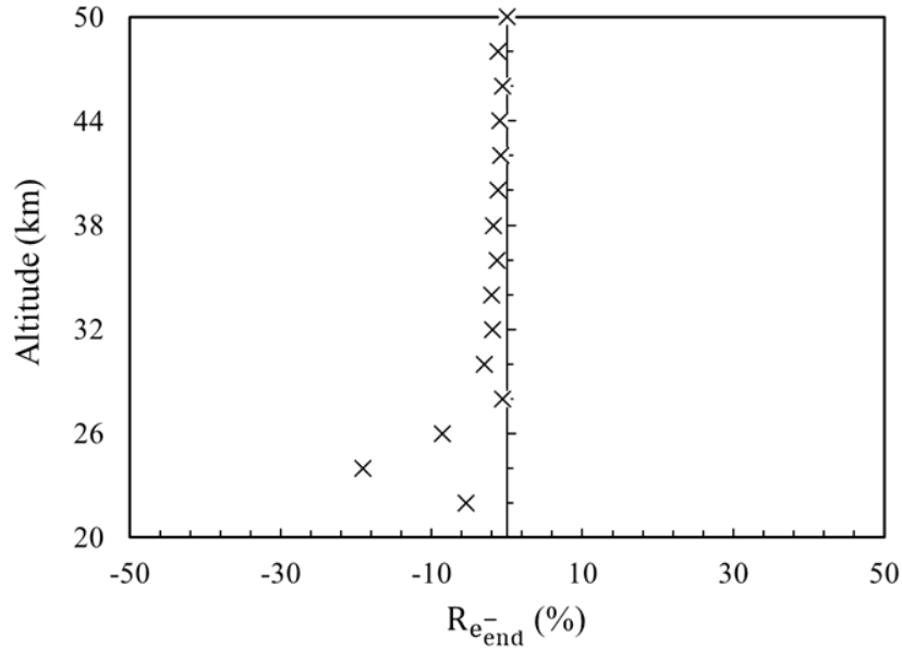
Figure 5-1. Relative differences in the electron densities at the end of the streamer between those deduced from scale factors (calculations) and those obtained from simulations at altitudes of 20-50 km.
