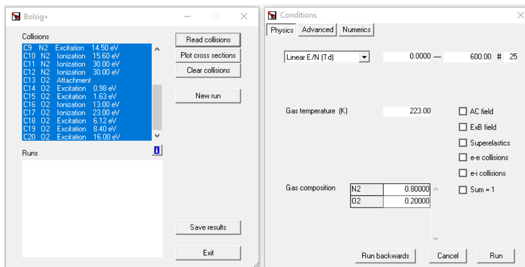
Figure 2-2. The BOLSIG+ solver starts by reading the collision files of cross-section (left) and setting calculation background conditions (right).
