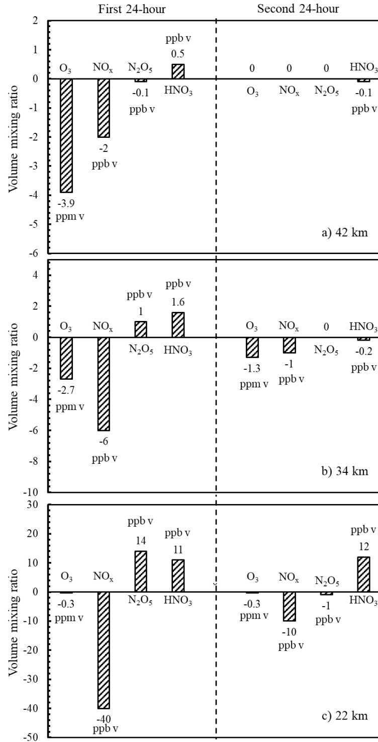
Figure 5-7. Changes in the VMRs of O 3 , NO x , N 2 O 5 and HNO 3 during the first 24 hours and second 24 hours of streamer simulations at a) 42 km, b) 34 km, c) 22 km.
