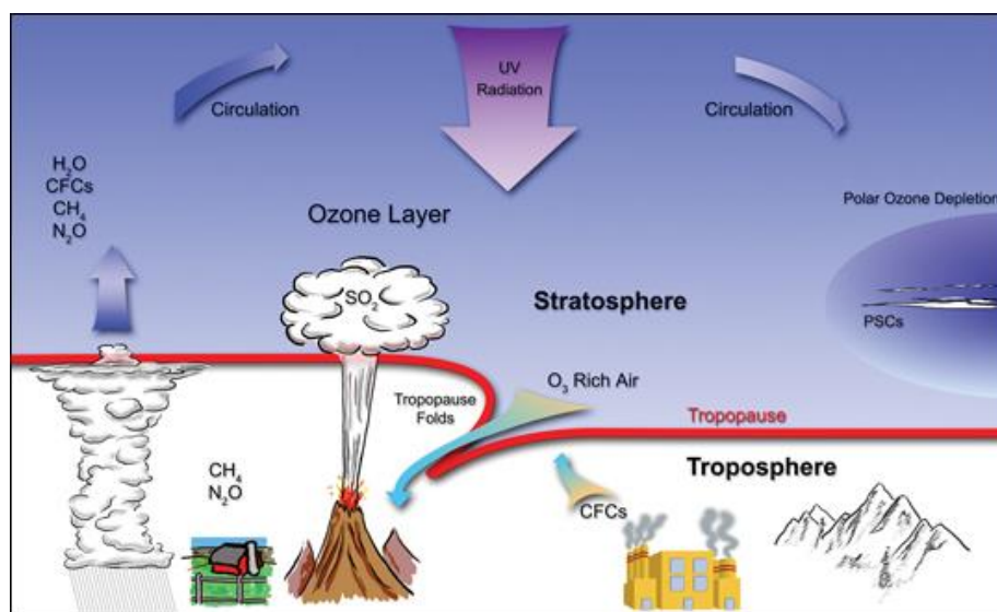
Figure 1-2. Natural and anthropogenic mechanisms associated with the stratospheric ozone layer. Credit from Barbara Summery, SSAI.
