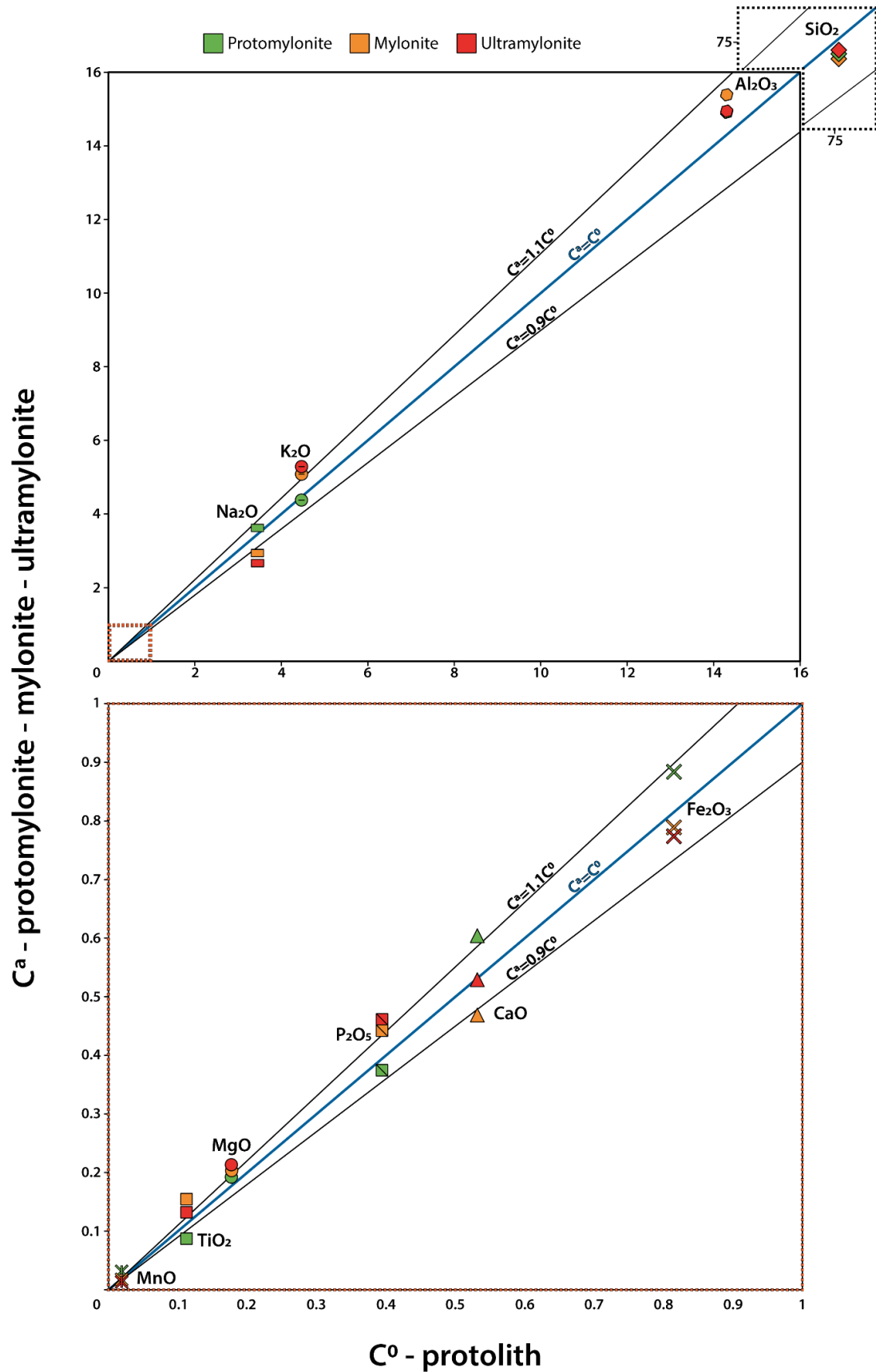
Fig. 12: Isocon diagram comparing the chemical composition of the protolith ( C^0 ) with those of protomylonite, mylonite and ultramylonite ( C^a ). The blue line ( C^a = C^0 ) represents the constant concentration, while the black lines represent 10% gains and 10% losses of components in C^a compared to C^0 .
