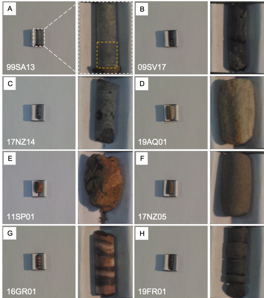
Fig. 6. Step 2: selected core samples imaged with HRC emulator conditions at a resolution of 17 mm/pixel. Samples were each imaged in two light conditions. Field of view is equivalent to that planned for HRC images (17.4 x 17.4 cm). Yellow box in A indicates size of the FOV3 of CLUPI (cf. Fig. 3A). A) Sample 99SA13, metapelite with carbonate. B) Sample 09SV17, tholeiitic basalt. C) Sample 17NZ14, basalt-pyroxenite. D) Sample 19AQ01, calcitic quartz arenite. E) Sample 11SP01, conglomerate. F) Sample 17NZ05, coarse volcanogenic sandstone. G) Sample 16GR01, ferruginous chert. H) Sample 19FR01, finely laminated, organic-rich mudstone.
