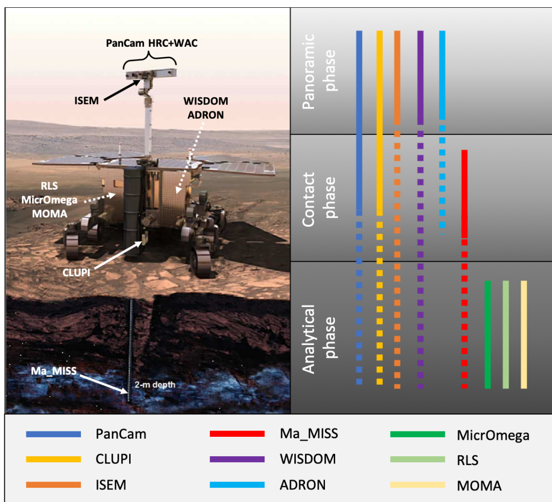
Fig. 1. The highly interconnected instrumental suite aboard the ExoMars 2020 Rosalind Franklin rover. The locations of the instruments on the rover are indicated, and their roles throughout the scientific protocol of ExoMars 2020 (see Vago et al., 2017; Hickman-Lewis et al., in revision) are shown. Solid lines indicate that the instrument is directly used at the corresponding stage of analysis; dotted lines indicate that the results obtained by the instrument are crucial in governing the process of analysis at a subsequent phase of analysis.
