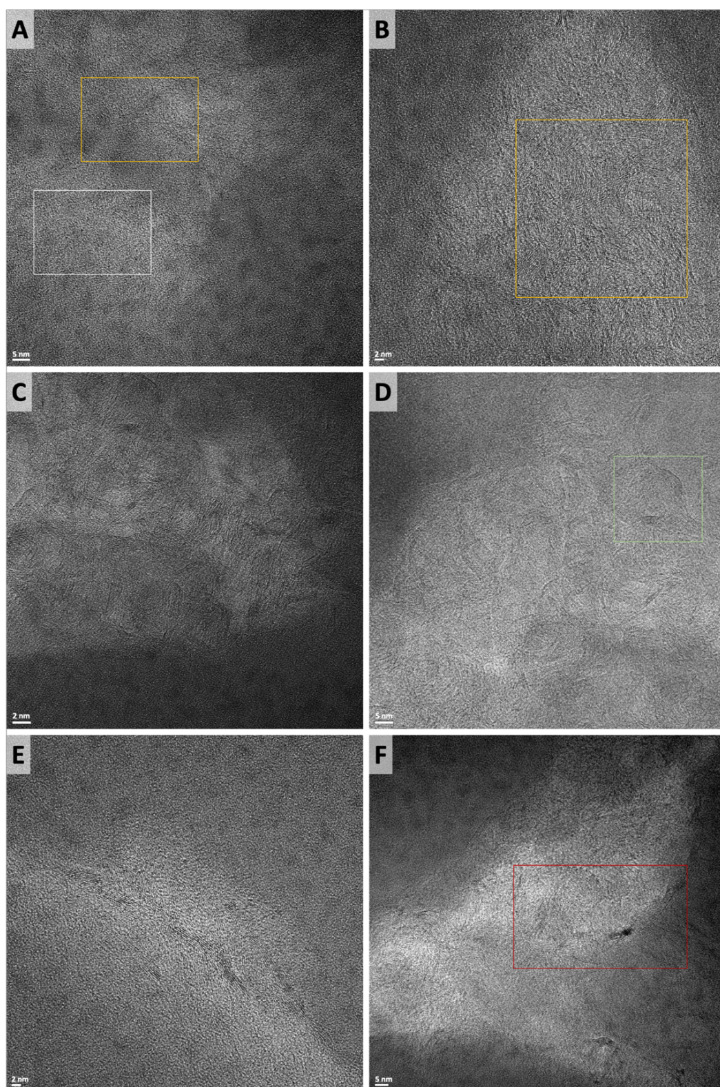
Fig. 6. Nanostructures of carbonaceous material identified in HRTEM micrographs in a sequence of increasing graphitisation (inspired by Buseck et al., 1988 ). Note the heterogeneity of structures in each micrograph. A) Mostly amorphous carbon (white box) associated with some poorly ordered, stacked fringes (orange box) corresponding to turbostratic carbon. Amorphous carbon corresponds to regions of polyaromatic hydrocarbons (after De Gregorio and Sharp, 2006 ). B) Poorly ordered turbostratic carbon with some swirled and curling nanostructures with increased stacking of graphene sheets (orange box) indicating increased ordering. C) Region of well-developed curled and swirling carbon nanostructures interspersed with amorphous carbon. D) Highly
