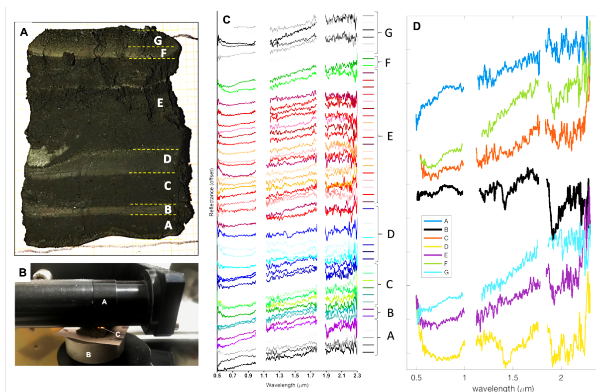
Fig. 7. Ma_MISS spectral acquisition. A) Cut sample showing designation of layering. B) Ma_MISS breadboard setup showing the Ma_MISS tip (A), the sample holder containing sample 1 (B), and the illumination spot focussed on sample 1. C) All spectra obtained, assigned to layers in the sample. D) End-member spectra for each layer, derived from the spectra in C.
