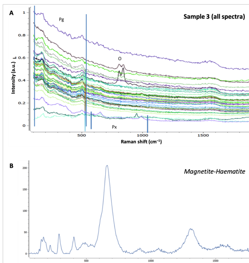
Fig. 10. RLS characterisation of sample 3. A) All spectra obtained using the automatic procedure. B) Extracted spectra corresponding to magnetite and haematite.
