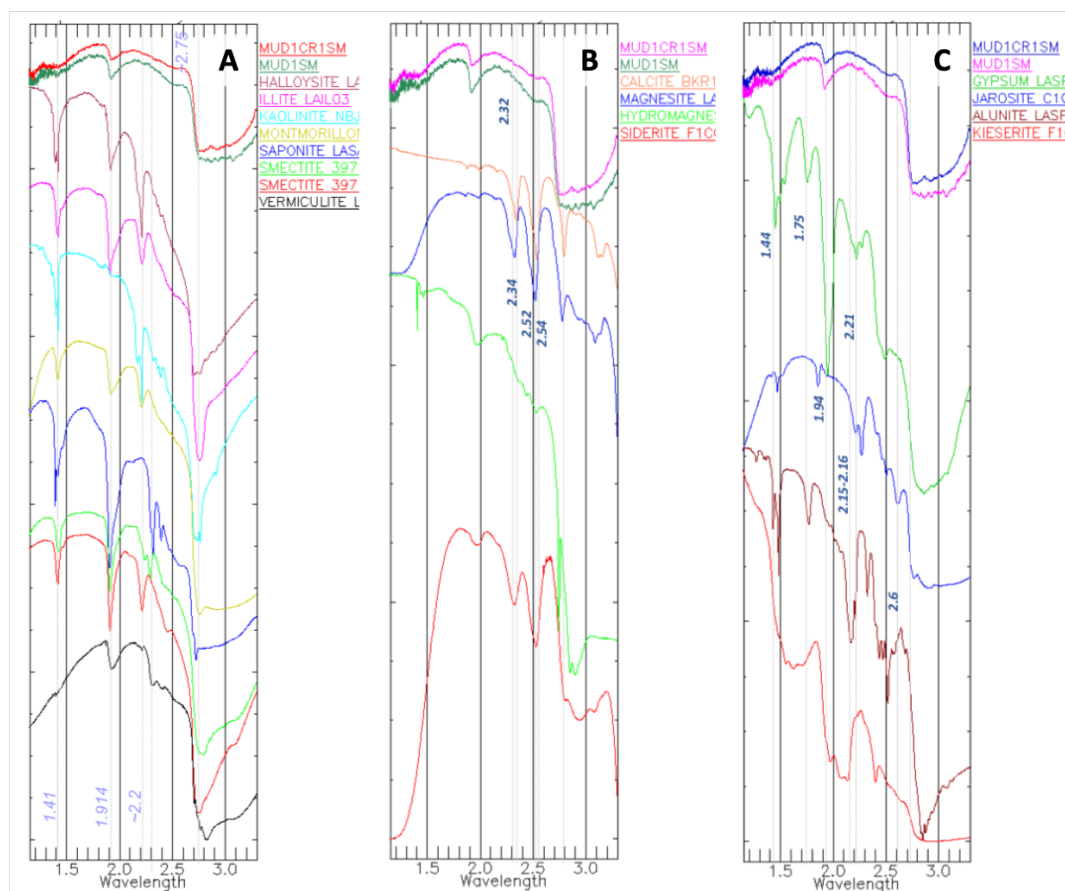
Fig. 6. Comparison of ISEM spectra (raw, MUD1CRISM; smoothed, MUD1SM) with selected CRISM spectra for phyllosilicates (A), carbonates (B) and sulphates (C). Results for sample 1 shown.
