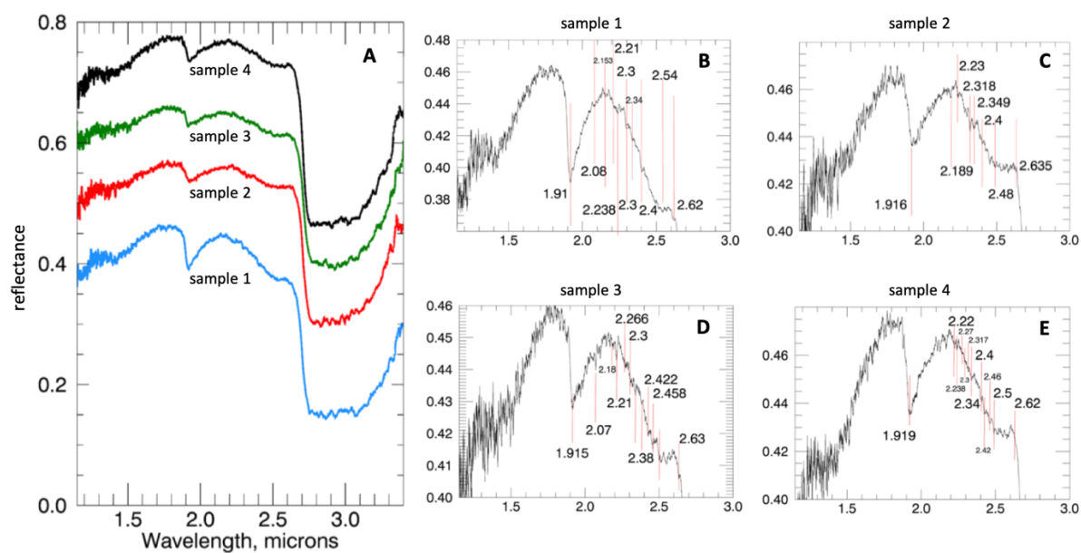
Fig. 5. ISEM spectral acquisitions. A) Comparison of the four spectra obtained. B-D) Details of each spectra with prominent spectral features identified from which mineral identifications were made (compare with CRISM library spectra in Figure 6).
