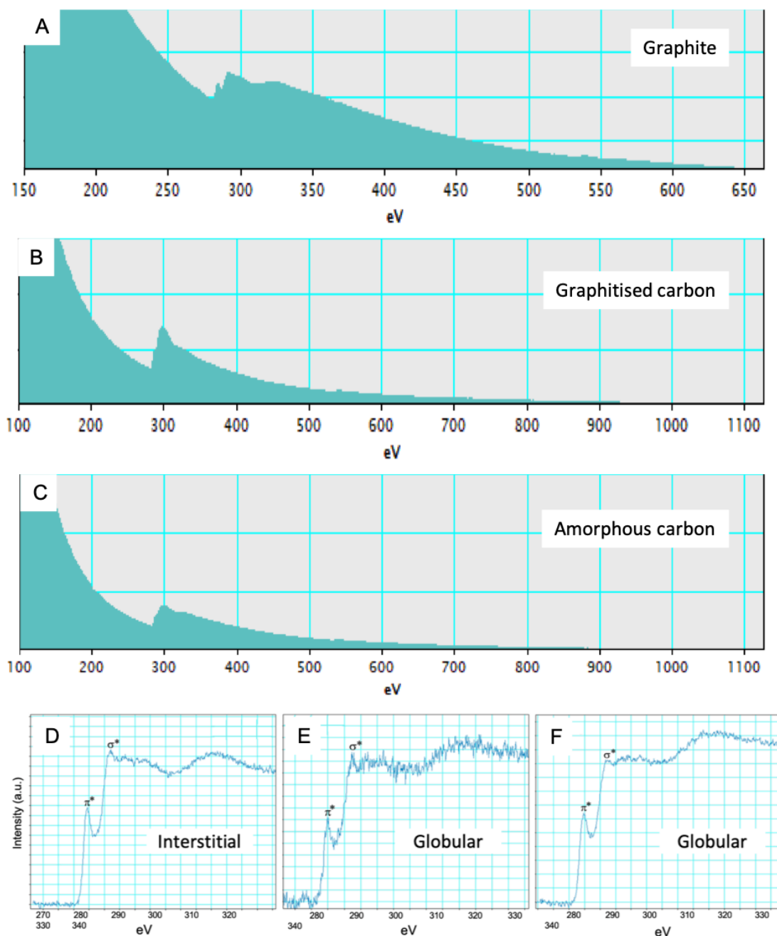
Fig. 8. EELS spectra from carbonaceous clots. A) EELS spectra of highly graphitised carbon with well-defined \pi^* and \sigma^* transitions at 285 eV and 291.7 eV, respectively, and a flattened C K-edge structure between 300 and 325 eV. B) EELS spectra of less well-graphitised carbon with incipient \sigma^* transition, which is considered to be the first indicator of graphitisation (after De Gregorio and Sharp, 2006 ), but no separate \pi^* transition. C) EELS spectra from amorphous carbon showing a more rounded shape and a slight hump in place of the \pi^* transition at 285 eV. D) Representative EELS spectra of interstitial carbon showing well-defined \pi^* and \sigma^* transitions and C K-edge fine structure between 295 and 325 eV, indicating a dominance of sp^2 bonding, consistent with graphitised carbon. E-F) Representative EELS spectra of globular carbon showing well-defined \pi^* transitions and a clear \sigma^* transition peak only in E. In F, there is neither a well-developed \sigma^* peak nor fine C K-edge structure between 295 and 325 eV. E is thus consistent with more graphitised carbon, whereas F shows the characteristics of mostly amorphous carbon.
