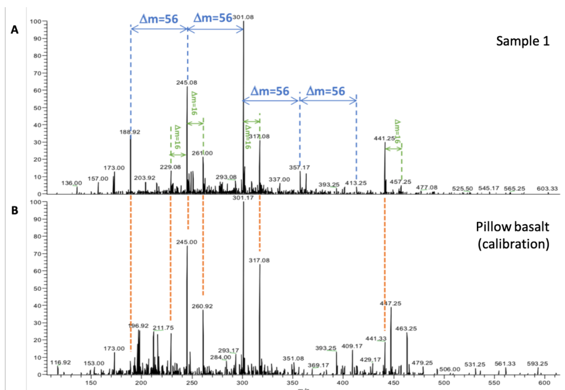
Fig. 12. Results of LDMS analyses of sample 1 compared with a pre-characterised Cretaceous igneous sample.
