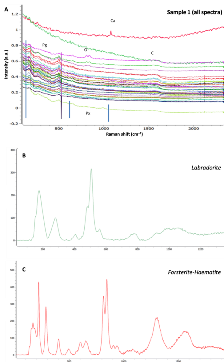
Fig. 8. RLS characterisation of sample 1. A) All spectra obtained using the automatic procedure. B) Extracted spectra corresponding to labradorite, the dominant mineral phase. C) Spectra corresponding to forsterite and haematite potentially associated with carbonaceous material.
