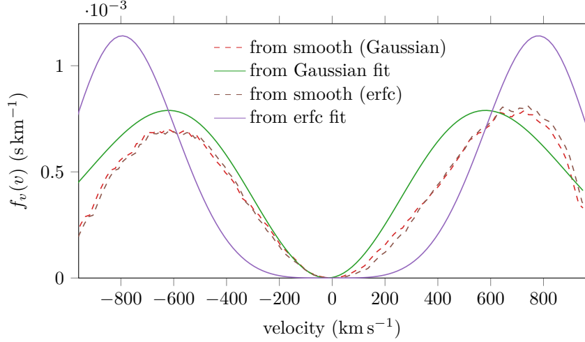
Figure 3.11: EVDFs obtained from a Thomson scattering spectrum. The solid lines correspond to the theoretical EVDFs obtained from the fitting functions shown in Figure 3.8 (green line for Maxwell-Boltzmann distribution and purple line for Druyvesteyn distribution). The dashed lines correspond to the experimental EVDFs obtained from the smoothing functions shown in Figure 3.10 (red dashed line for Maxwell-Boltzmann distribution and brown dashed line for Druyvesteyn distribution).
