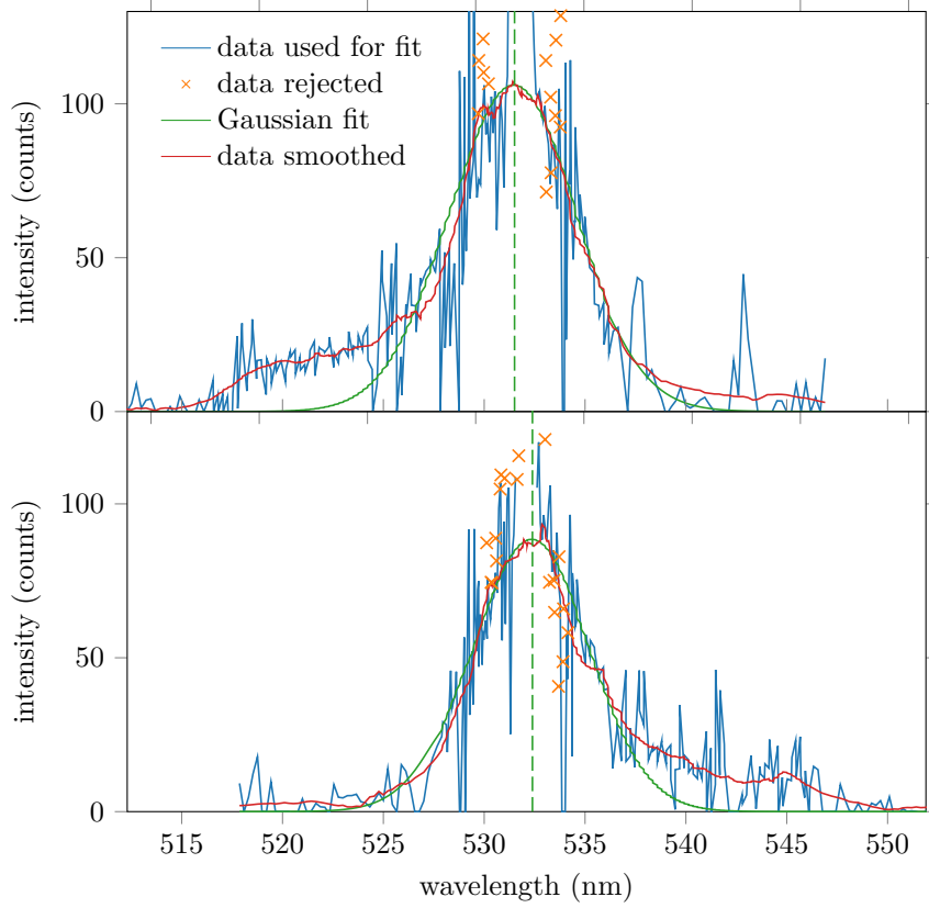
Figure 6.28: Thomson spectra obtained along the “azimuthal direction” 2 mm from the exit plane of the ISCT200-MS, for a discharge voltage of 150 V and a discharge current of 2.17 A. The Gaussian fit and the position of its center are shown with respectively a solid and dashed (vertical) green line. Top: magnetic field lines directed towards the inner pole and injection of a xenon flow of 2.1 \text{ mg s}^{-1} near the anode; the Gaussian fit gives n_e = (1.6 \pm 0.1) \times 10^{17} \text{ m}^{-3} , T_e = (7.9 \pm 0.7) \text{ eV} and v_{e,drift} = (130 \pm 20) \text{ km s}^{-1} . Bottom: magnetic field directed towards the outer magnetic pole (xenon mass flow rate was adjusted to 2.15 \text{ mg s}^{-1} to keep the discharge current at the nominal value); the Gaussian fit gives n_e = (1.3 \pm 0.1) \text{ m}^{-3} , T_e = (7.4 \pm 0.7) \text{ eV} and v_{e,drift} = (110 \pm 20) \text{ km s}^{-1} .
