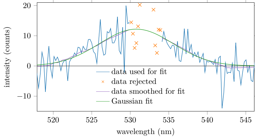
Figure 6.9: Thomson spectrum example obtained along the “azimuthal direction” with the ISCT200-GEO thruster. The corresponding electron density and temperature are ((2.6 \pm 0.2) \times 10^{16} \text{ m}^{-3}) and (20 \pm 2) \text{ eV} , respectively. Discharge parameters are a xenon flow rate of 1.6 \text{ mg s}^{-1} , discharge voltage of 250 \text{ V} and a discharge current of 1.13 \text{ A} . This spectrum is obtained for an axial distance from the exit plane of 4 \text{ mm} and peak magnetic field of 25 \text{ mT} at the exit plane.
