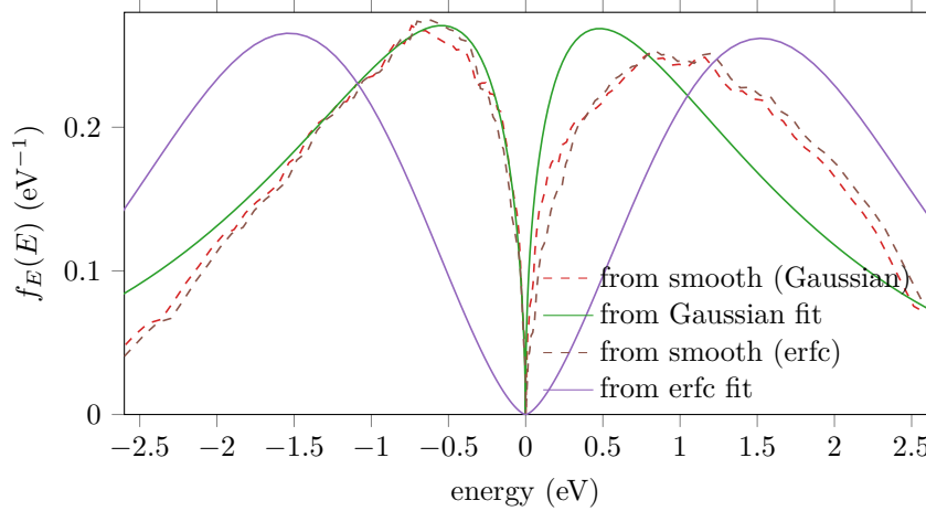
Figure 3.12: EEDFs obtained from a Thomson scattering spectrum. The solid lines correspond to the theoretical EEDFs obtained from the fitting functions shown in Figure 3.8 (green line for Maxwell-Boltzmann distribution and purple line for Druyvesteyn distribution). The dashed lines correspond to the experimental EEDFs obtained from the smoothing functions shown in Figure 3.10 (red dashed line for Maxwell-Boltzmann distribution and brown dashed line for Druyvesteyn distribution).
