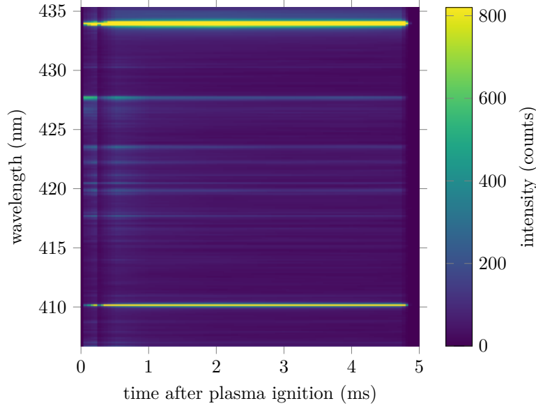
Figure 5.11: Spectrogram obtained during the 5 ms duration of the RF pulse. The instantaneous RF power and the dihydrogen pressure were, respectively, 470 W and 3.3 \times 10^{-2} Pa. The intensity range was adapted to the intensity of the vibrational lines.
