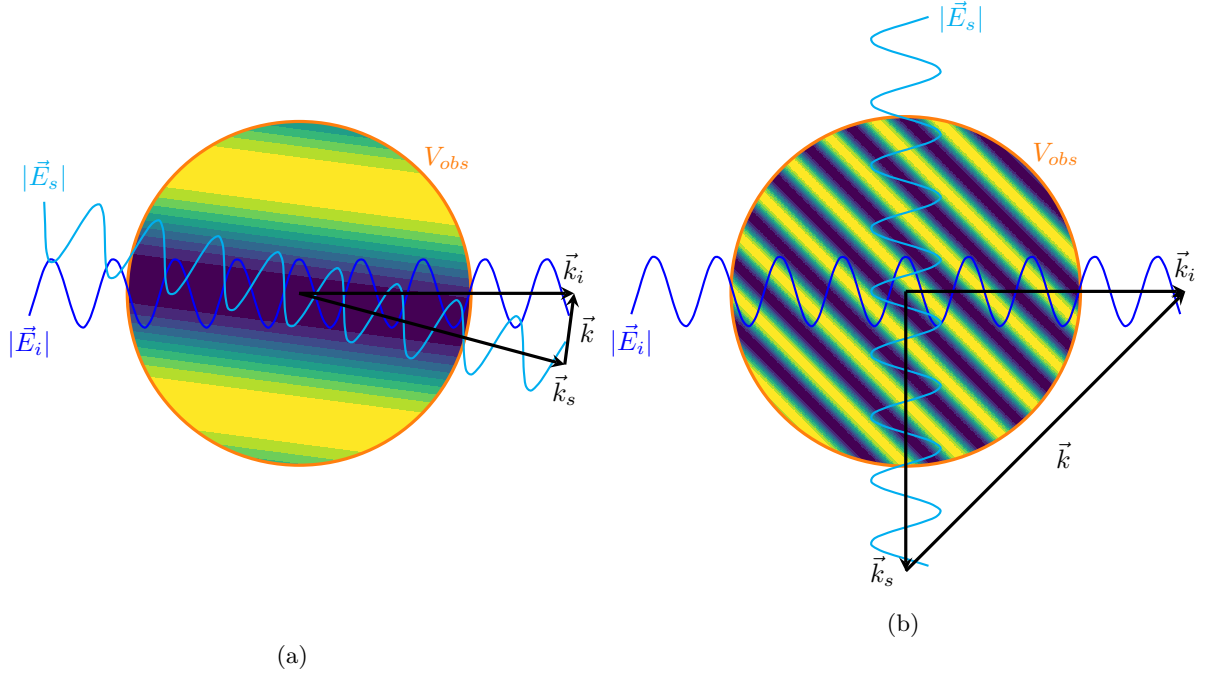
Figure 2.5: Pattern of the \cos\left(\Phi(\vec{e}_s, \vec{i}, t) - \Phi(\vec{e}_s, \vec{j}, t)\right) function over the observation volume ( V_{obs} ) for two scattering configurations. A scattering configuration with \theta=15^\circ is shown on the left (a) and a configuration with \theta=90^\circ is shown on the right (b).
