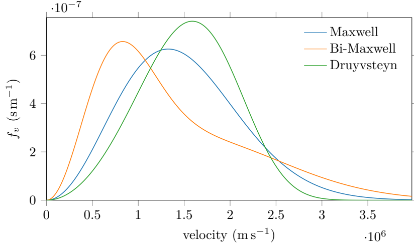
Figure 2.9: EVDF in the case of a Maxwell-Boltzmann, a Bi-Maxwell-Boltzmann and a Druyvesteyn distribution. The following parameter values are chosen for the plot: \sigma=9.38 \times 10^6 \text{ m s}^{-1} , \eta_c = \eta_h=0.5 and T_{e,h}/T_{e,c}=5 .
