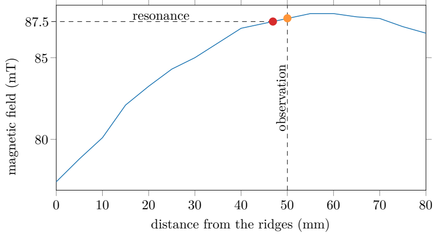
Figure 5.2: Axial profile of the magnetic field intensity along the axis of the plasma chamber for the configuration with ( I_{B1}=64 A; U_{B1}=14.2 V) and ( I_{B2}=68 A; U_{B2}=14.8 V).
