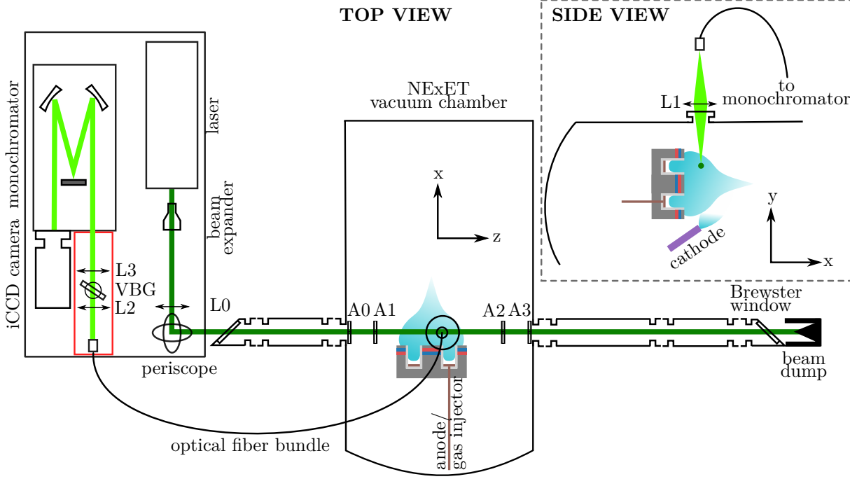
Figure 6.6: Schematic view of the THETIS diagnostic setup for Hall thruster investigations (not to scale). The transmission branch is indicated with a dark green line and the detection branch with a light green line. L0, L1, L2, and L3 indicate lenses; A0, A1, A2, and A3 indicate apertures; VBG indicates the notch filter. The blue area corresponds to the plasma volume.
