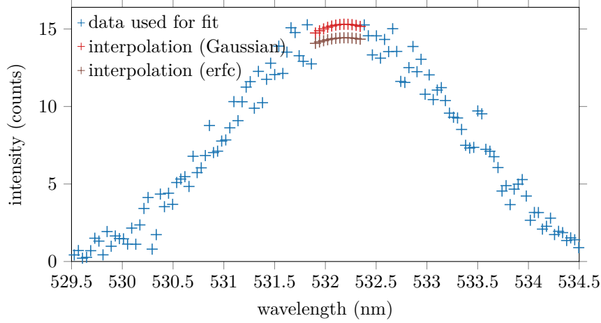
Figure 3.9: Example of the same Thomson scattering spectrum as Figure 3.8 with the data inside the rejection interval interpolated by the values of the Gaussian fit (red “+” symbols) or erfc fit (brown “+” symbols).
