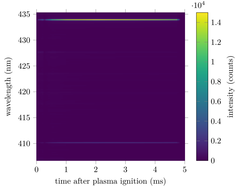
Figure 5.10: Spectrogram obtained during the 5 ms duration of the RF pulse. The instantaneous RF power and the dihydrogen pressure were, respectively, 470 W and 3.3 \times 10^{-2} Pa.
