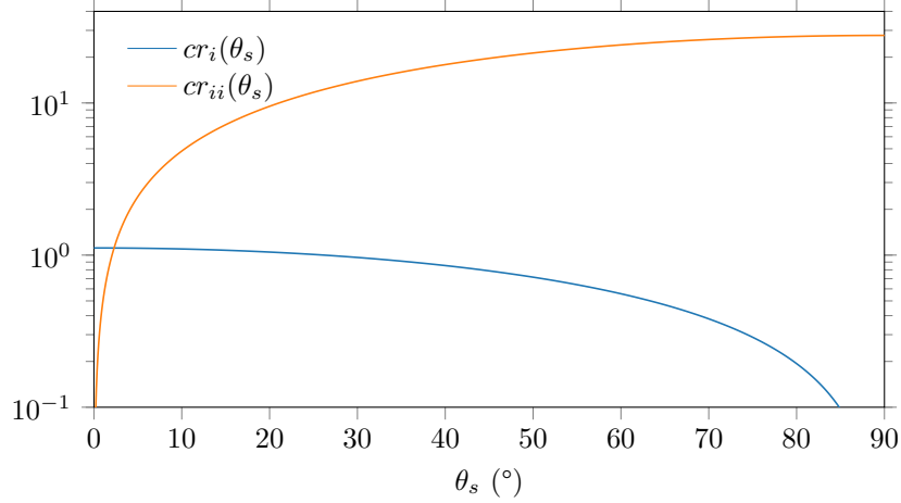
Figure 3.14: Representation of the criterion necessary for detection of Thomson spectrum modulation for various value of the \theta_s angles. The “best case scenario” were considered for the choice of the input parameters of the functions.
