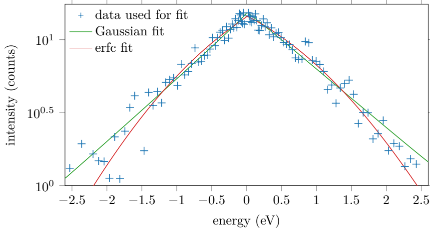
Figure 3.13: Representation of the logarithm of the Thomson scattering intensity as a function of the energy of the corresponding scattering electron (i.e., square of the spectral shift). The “+” symbols represent experimental data and the green and red lines correspond to the fitting functions for Gaussian and Druyvesteyn EVDFs, respectively.
