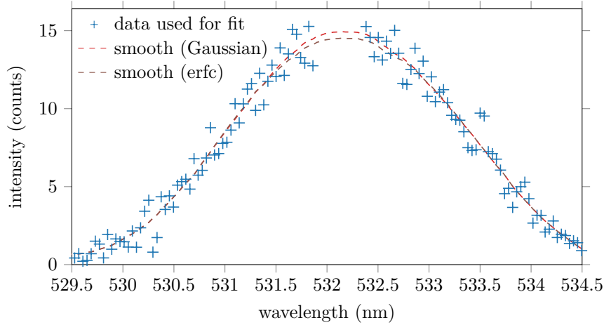
Figure 3.10: Example of the same Thomson scattering spectrum as Figure 3.8 with the analytic functions obtained from a smoothing procedure when Gaussian (red dashed line) and erfc (brown dashed line) fitting functions are considered for the interpolation inside the rejection interval.
