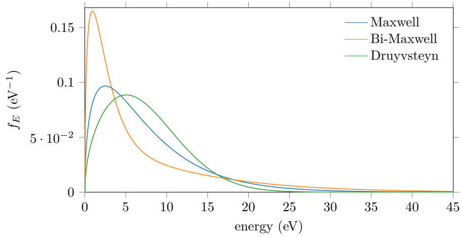
Figure 2.10: EEDF in the case of a Maxwell-Boltzmann, a Bi-Maxwell-Boltzmann and a Druyvesteyn distribution. The following parameter values are chosen for the plot: \sigma=9.38 \times 10^6 \text{ m s}^{-1} , \eta_c = \eta_h=0.5 and T_{e,h}/T_{e,c}=5 .
