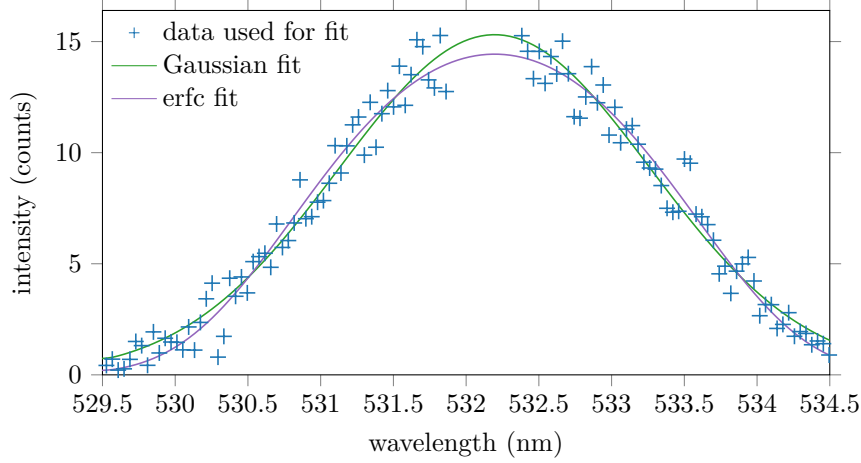
Figure 3.8: Example of a Thomson scattering spectrum obtained with the 2400 lines \text{mm}^{-1} grating and a spectrometer slit width of 300 \mu\text{m} . From the experimental data indicated with “+” symbols the best Gaussian and erfc fit functions are estimated.
