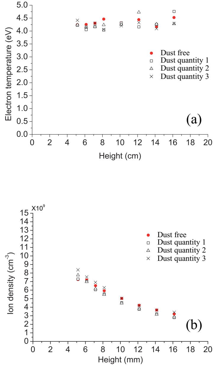
Figure 7.7: (a) Electron temperature and (b) ion density in function of height at the centre of the chamber with and without dust particles. Amount of dust particle in the chamber for each case was shown in Fig. 7.6.
