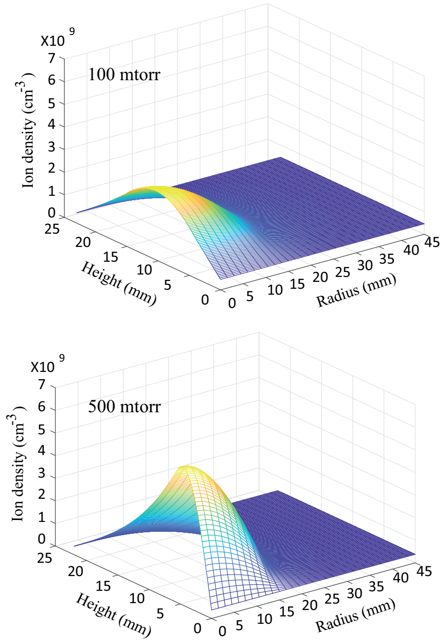
Figure 6.2: Calculation results of spatial distribution of ion density under conditions 100 and 500 mtorr in gas pressure, 100 V in RF voltage.
