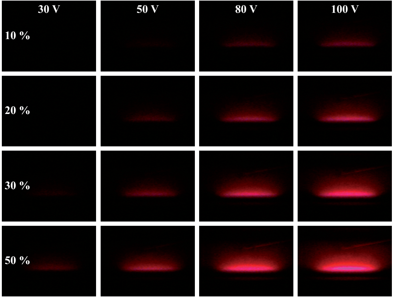
Figure 7.1: Photographes of RF plasmas under different discharge conditions. Pressure is 400 mtorr. Frequency of pulse-time modulation is 10 kHz. Duty cycle of pulse-time modulation varies from 50% to 10%. RF voltage varies from 30 to 100 V.
