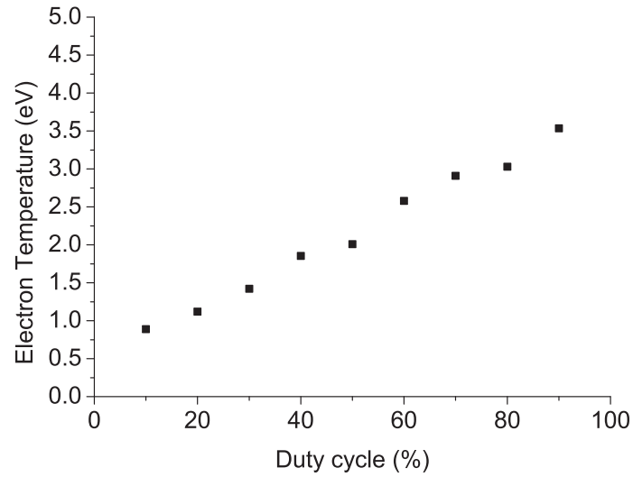
Figure 7.10: Electron temperature in function of duty cycle of the pulse-time modulation.
