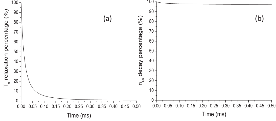
Figure 5.2: Simulation result of the time evolution of T_e relaxation (a), and plasma density decay (b).
