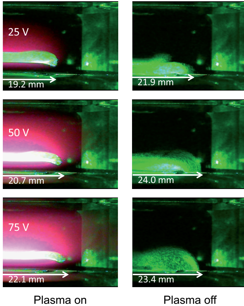
Figure 7.16: Particles fall down by shutting down RF power when the RF voltages are set at 25, 50 and 75 V.
