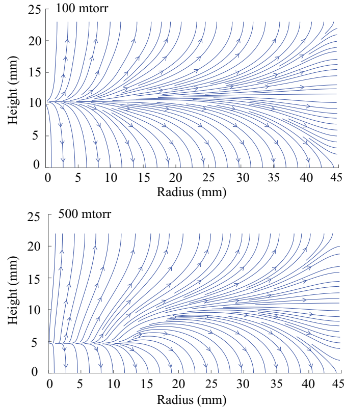
Figure 6.4: Ion flow direction calculated by using ambipolar diffusion model for the case of 100 and 500 mtorr in gas pressure, based on the spatial distribution of ion densities.
