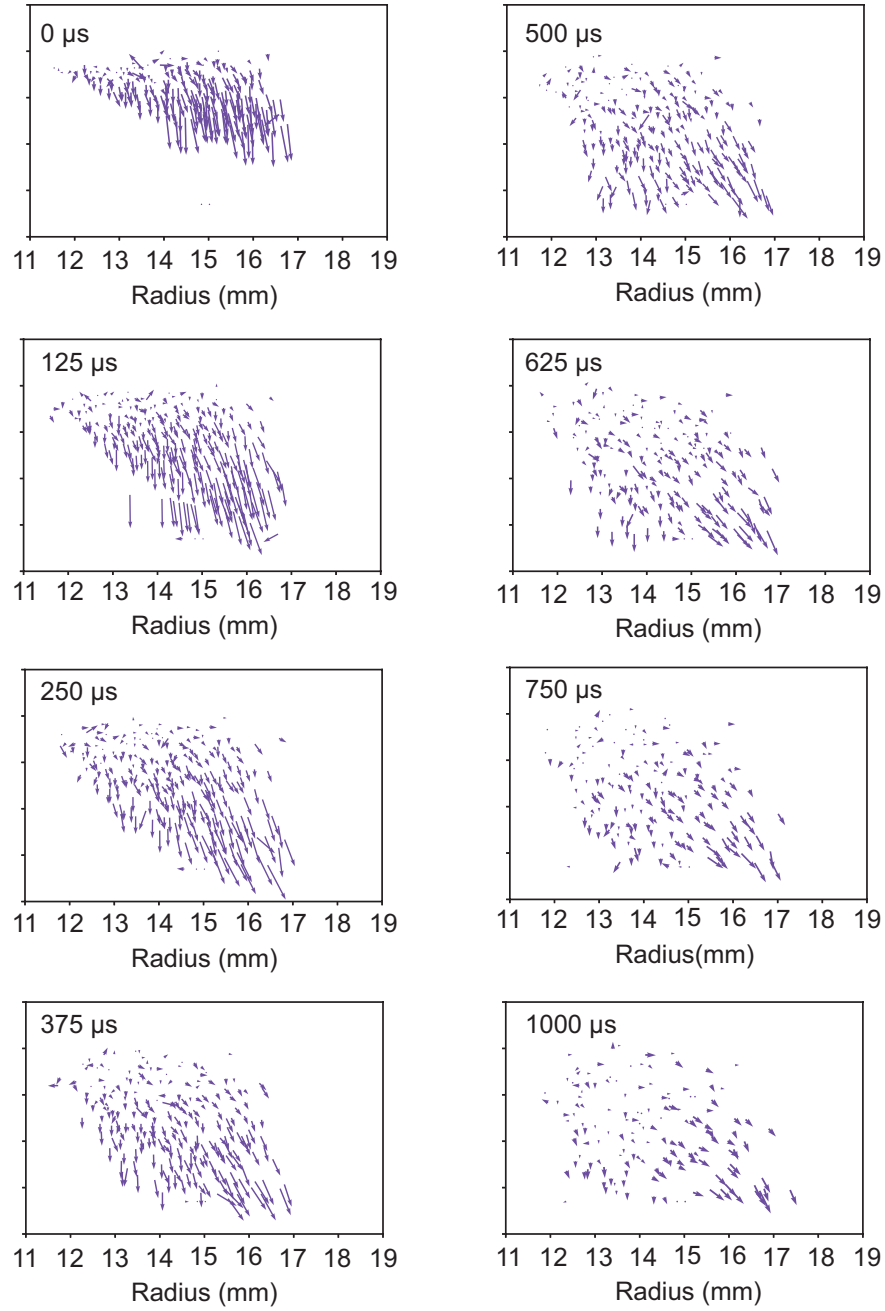
Figure 7.18: Falling down process of particles by shutting down RF power, Particles are filmed by hight speed camera and analysed by particle tracking. Arrows represent particle speed and current position.
