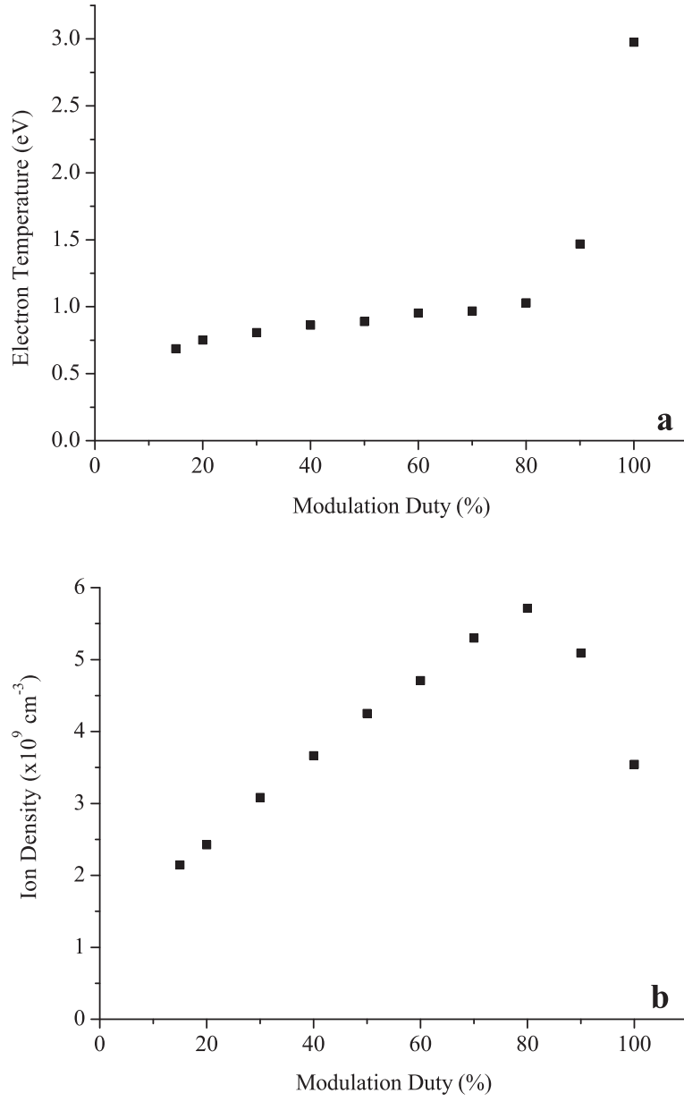
Figure 7.34: (a) Electron temperatures as functions of modulation duty cycle. (b) Ion densities as functions of modulation duty cycle. The frequency and RF voltage were 10 kHz and 100 V, respectively.
