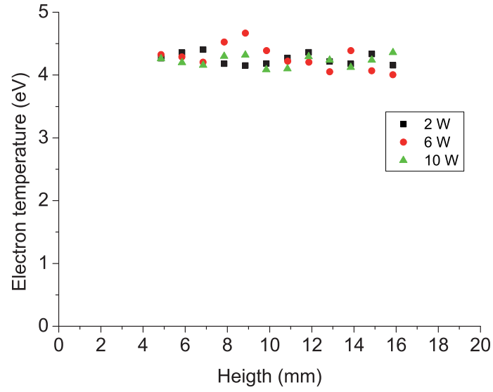
Figure 7.9: Electron temperature in function of height at the centre of the reactor chamber for the RF voltage of 2, 6 and 10 W.
