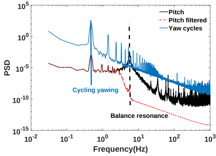
Figure 3.19 – Power spectral density of the yaw motion and pitch moment.
