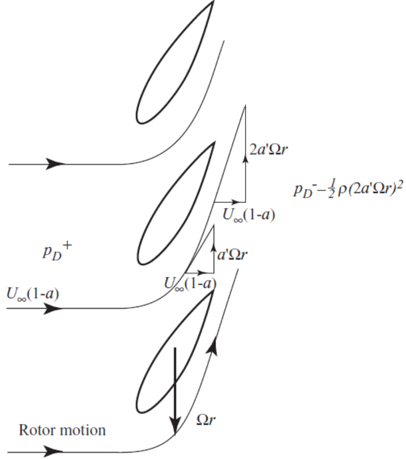
Figure 2.5 – Tangential speed through the rotor disc from Burton et al. [2011]
