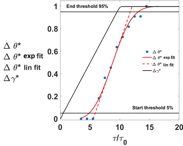
Figure 4.11 – Example of cycle-averaged wake deviation history during yaw manoeuvre for configuration HIT1 P1 during a positive yaw variation. Symbols: — \Delta\gamma^* , ● \Delta\theta^* , - - - \Delta\theta^* linear, — \Delta\theta^* exp fitted, - - start thresholds. Data fitted for \tau > \tau_{lag} .
