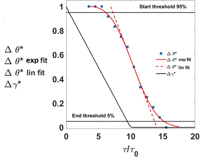
Figure 4.12 – Example of cycle-averaged wake deviation history during yaw manoeuvre for configuration HIT1 P1 during a negative yaw variation. Symbols: — \Delta\gamma^* , \bullet \Delta\theta^* , - - - \Delta\theta^* linear, — \Delta\theta^* fitted, - - start thresholds. Data fitted for \tau > \tau_{lag} .
