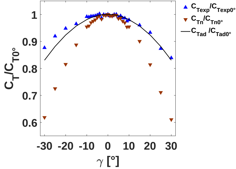
Figure 4.6 – Normalised thrust coefficient of the upstream wind turbine compared with the theoretical law from the actuator disc theory.
