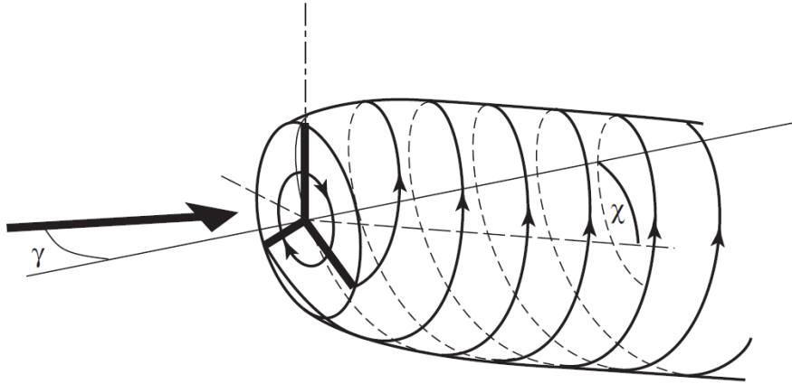
Figure 2.12 – Scheme of the deflected vortex wake for yawed conditions. From Burton et al. [2011].
