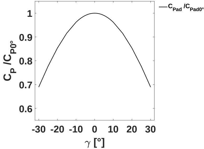
Figure 4.7 – Normalised power coefficient of the upstream wind turbine predicted by the the theoretical law from the actuator disc theory.
