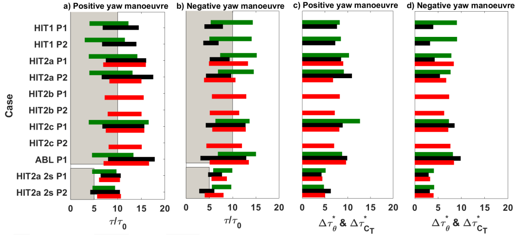
Figure 4.17 – Timeline representation of the wake deviation, the available wind power density and the thrust variations for different porosity levels and flow conditions. For figures a & b, the horizontal bar extremes represent the start and the end of the studied phenomenon. a) Positive yaw manoeuvre main parameters, b) Negative yaw manoeuvre main parameters, c) Positive yaw manoeuvre duration, d) Negative yaw manoeuvre duration. Colors: green = values retrieved by the center wake position, black = values retrieved by the wind power density, red = values retrieved by the thrust variations, gray = expected yaw manoeuvre duration
