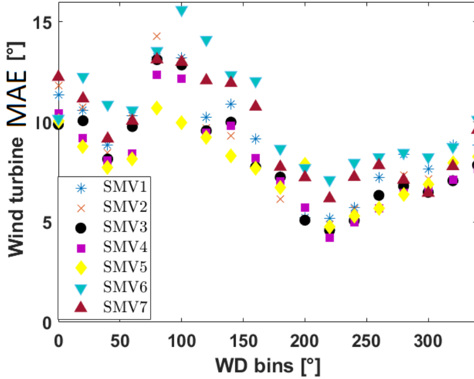
Figure 5.4 – SCADA wind direction measurements mean absolute errors (MAE)
