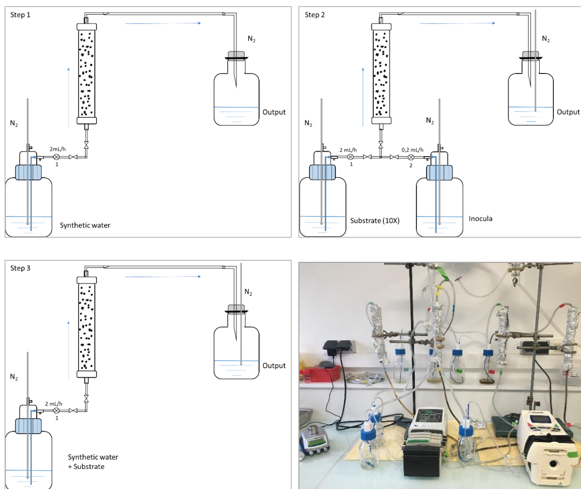
Figure V-2. Photo and sketch (protocol in 3 steps) of the columns experiment.
