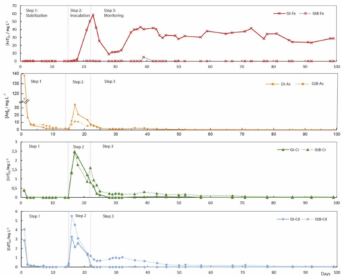
Figure V-10. Temporal evolution of dissolved [\text{FeT}]_D (upper panel), [\text{AsT}]_D , [\text{CrT}]_D and [\text{CdT}]_D (lower panel) monitored at the outlet of the goethite columns: Gt (inoculated column) and GtB (un-inoculated Blank column).
