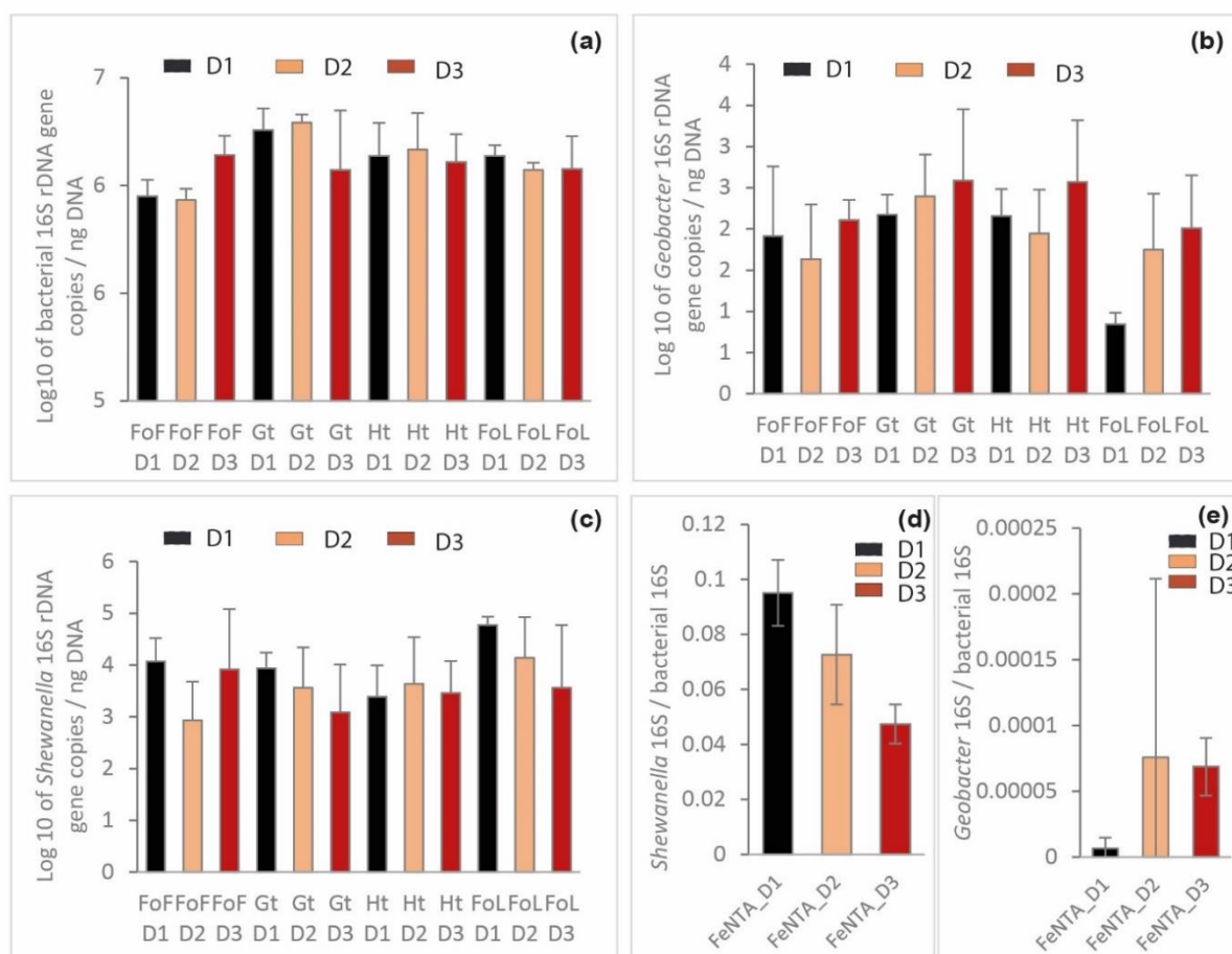
Supplementary Figure III-S5. Parameters linked to bacterial abundance: (a) Log10 of bacterial 16S rRNA ( rrs gene) copies, (b) Log 10 of Geobacter 16S gene copies, (c) Log 10 of Shewanella 16S gene copies, for the three site samples D1, D2 and D3; Ratios of Shewanella 16S (d) and Geobacter 16S (e) over bacterial 16S rRNA genes copies in Fe(III)-NTA enrichments. Error bars represent the standard deviation of triplicate measurements.
