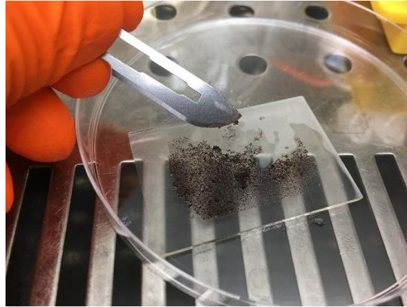
Figure IV-3. Solid culture collection for DNA extraction after incubation
