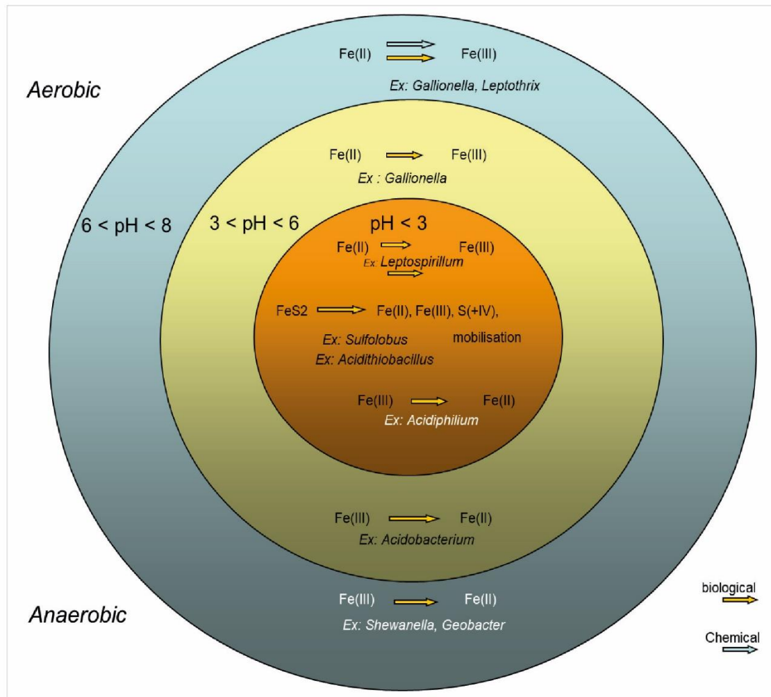
Figure I-3. Bacterial group \text{Fe(II)} oxidation in oxic condition and \text{Fe(III)} reduction in anoxic conditions with a large range of pH
