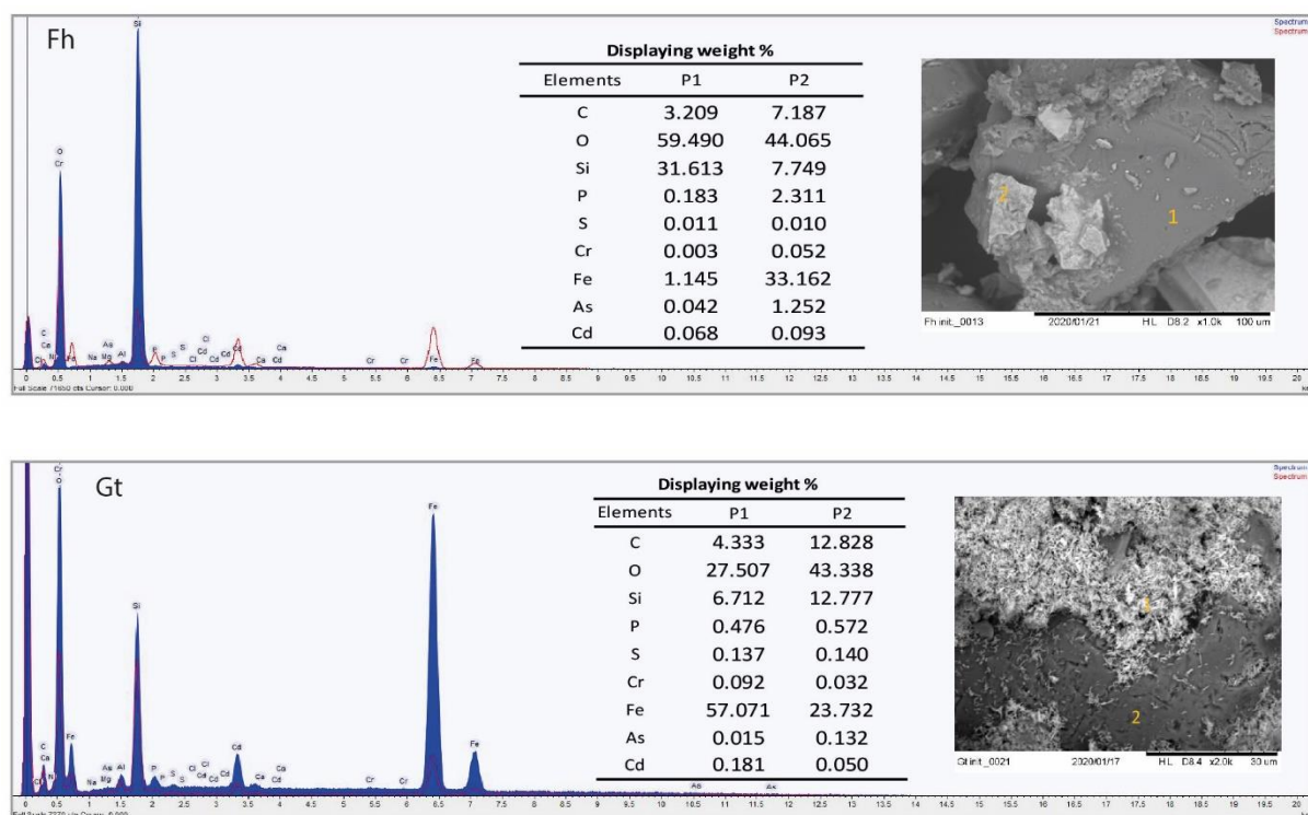
Figure V-21. SEM-EDS analysis of initial samples for ferrihydrite (Fh) and goethite (Gt) columns. The blue and red spectra correspond to the analyses of point “1” and point “2” (abbreviated P1 and P2), respectively.
