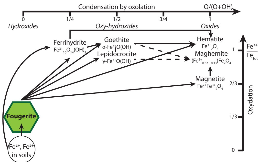
Figure I.4 – Location of fougurite in the formation pathways of Fe oxides. x-axis: molar ratio O/(O+OH) , increasing condensation by oxylation from left to right. y-axis: molar ratio of Fe^{3+}/Fe_{total} , increasing oxydation from the bottom to the top. Fougurite and ferrihydrite appear as key intermediate phases (reproduced and modified from Trolard et al. (2007), structural formulas taken from IMA database on RRUFF website).
