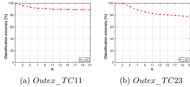
Figure 2.12: The performance of RAMBP for Gaussian noise with different k values in k -NN. Where k starts from 1 to 21 with a step of two to avoid tie problem, and \sigma parameter indicates Gaussian noise standard deviation.
