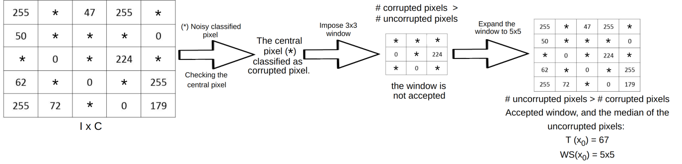
Figure 2.6: Threshold process example to facilitate understanding Algorithm 3.
