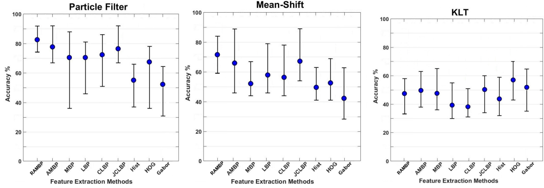
Figure 3.10: Accuracy of nerve tracking with bar error.
