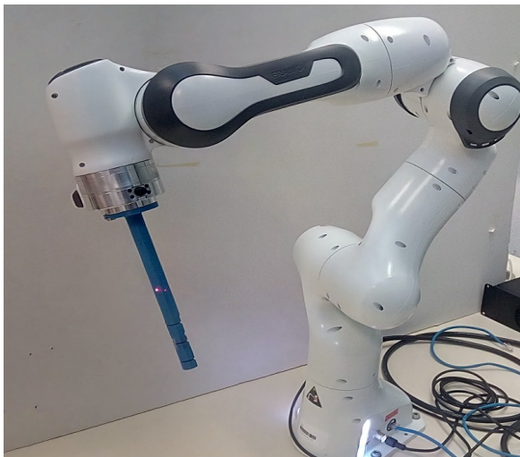
Figure 4.20: RCM results, where real robot images on the left column and the Rviz display on the right one.
