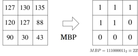
Figure 2.2: MBP operator applied to a 3 \times 3 neighborhood.
