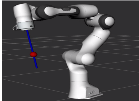
(b) The robot position after applying different rotations AND z-translations ( R_x = -30^\circ , R_y = -20^\circ , and T_z = 4cm ) at time (t) = 15 sec.
