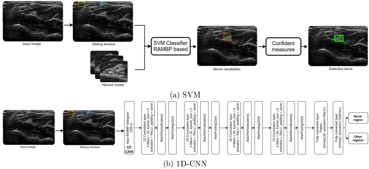
Figure 3.1: Schematic of nerve detection using RAMBP descriptor. (a) SVM classifier. (b) 1D CNN classifier.
