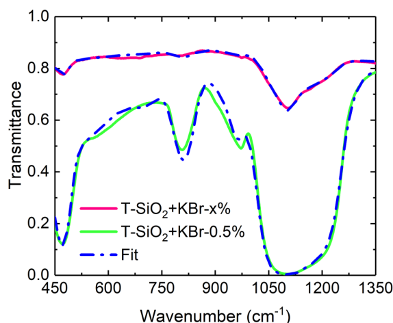
FIG. 5. Transmittance measurements on pellets containing 0.5% (green curve) and some traces noted x% (pink curve) of the \text{SiO}_2 nanopowders embedded in a KBr matrix. The dotted curves are fits of the spectra and are created using Eq. (3).
