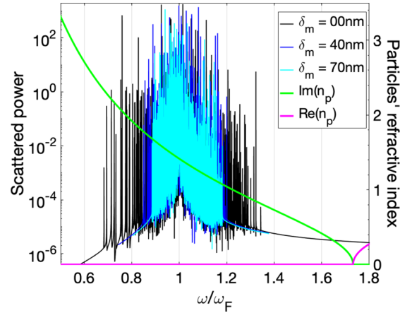
FIG. 2. Radiant flux for a random suspension of 90 particles in air against the frequency (normalized to the Fröhlich frequency). The minimum surface-to-surface distance between the particles is 0, 40, or 70 nm. The real and imaginary parts of the refractive index of the particles are also plotted.
