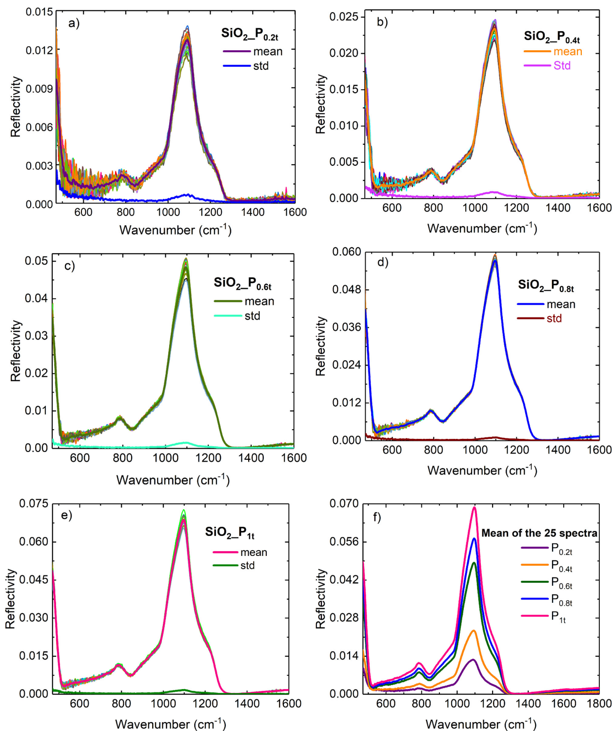
FIG. 3. Specular reflectivity spectra of amorphous \text{SiO}_2 pellets compacted at different pressure levels. Broad lines are the means and standard deviations (std) of a total of 25 spectra recorded for each sample. (f) presents the mean of the 25 spectra for each sample.
