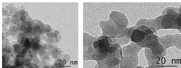
FIG. 2. TEM images, in bright-field mode, illustrating the morphology and size distribution of particles composing the silica nanopowder. The image on the right evidences the presence of strong interconnections between particles leading to highly porous and rigid nanoaggregates.
