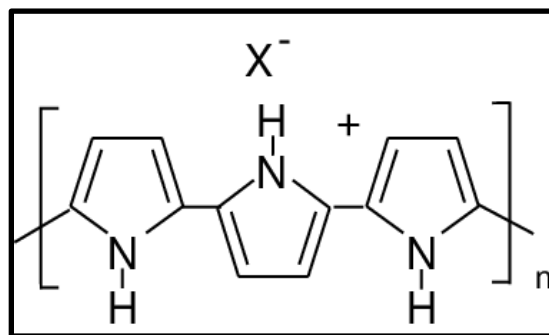
Figure 13. Polypyrrole structure with \pi conjugated double bonds.
