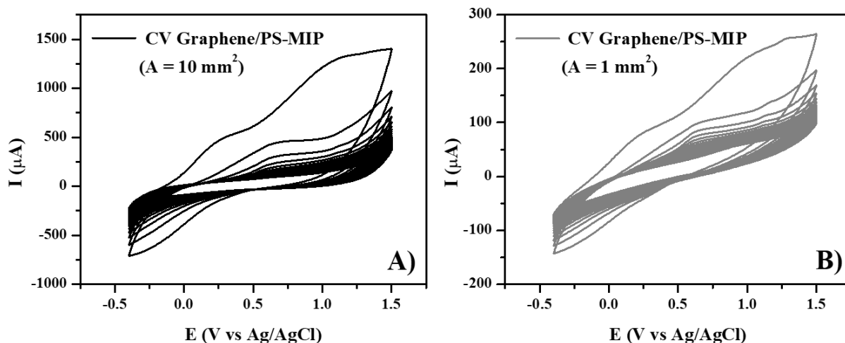
Figure 104. Isoproturon extraction from Graphene-MIP electrodes fabricated with our own method with different working surface area A) 10 \text{ mm}^2 , B) 1 \text{ mm}^2 , by cyclic voltammetry in an ethanol/water (70:30 v/v) solution of 0.1M \text{H}_2\text{SO}_4 . Scan rate 100 mV/s.
