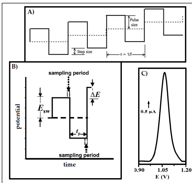
Figure 28. Square wave voltammetry, A) One potential cycle, B) Single potential cycle in SWV, C) square wave voltammogram obtained during determination of isoproturon ( c = 10^{-6} \text{ M} ).
