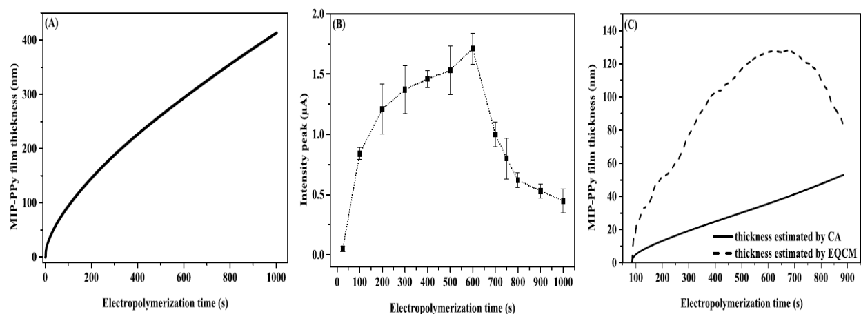
Figure 46. Effect of electropolymerization time on the electrochemical response of 5x10 -7 M of ISO at the MIP-GC electrode in ethanol/water (70:30 v/v) of H 2 SO 4 0.1 M, (A) the thickness of the MIP film estimated from the chronoamperogram (B) isoproturon electrochemical response, MIP film was formed by chronoamperometry setting the potential at 1.1 V, incubation time 15 min (C) comparative study of the MIP film thickness estimated by Faraday's law calculations and by EQCM experiments in order to follow the chronoamperometry electropolymerization process (potential applied 1.1 V, time duration 885 s) of ISO (1 mM) and pyrrole (0.01 M) on gold quartz used as a working electrode, electrolyte: 0.1M LiClO 4 in ethanol/water (80:20 v/v).
