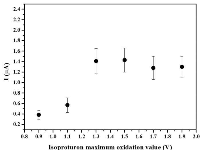
Figure 42. SWV determination of isoproturon ( 5 \times 10^{-7} M) at GC-MIP polypyrrole electrodes after template extraction by CV at different potential ranges.
