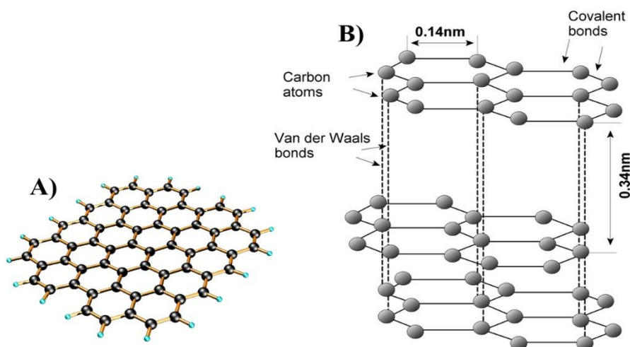
Figure 69. A) The honeycomb structure of graphene, B) Molecular arrangement of carbon in graphene and various bonding and forces involved during its self-assembly into graphite [258].
