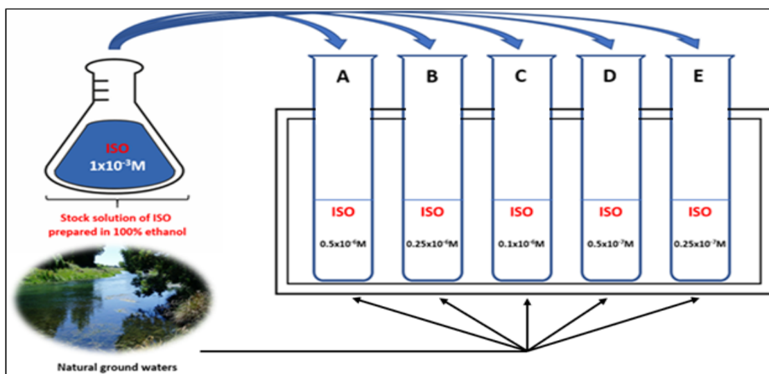
Figure 53. Schematically representation of the procedure used for the preparation of ground natural water samples for the isoproturon (ISO) analysis by using GC-MIPPy electrodes.
