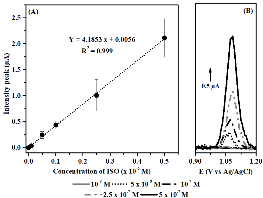
Figure 54. The calibration curves for isoproturon determination obtained at MIP-GC electrode in real natural water samples (A) includes calibration linear equation (B) square wave voltammograms obtained during electrochemical detection of isoproturon.
