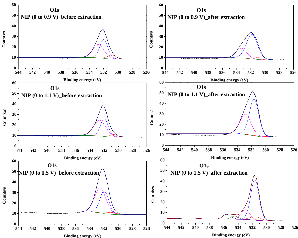
Figure 66. High resolution spectra of O1s obtained with GC-NIP films made by CV at different anodic potentials before and after extraction.
