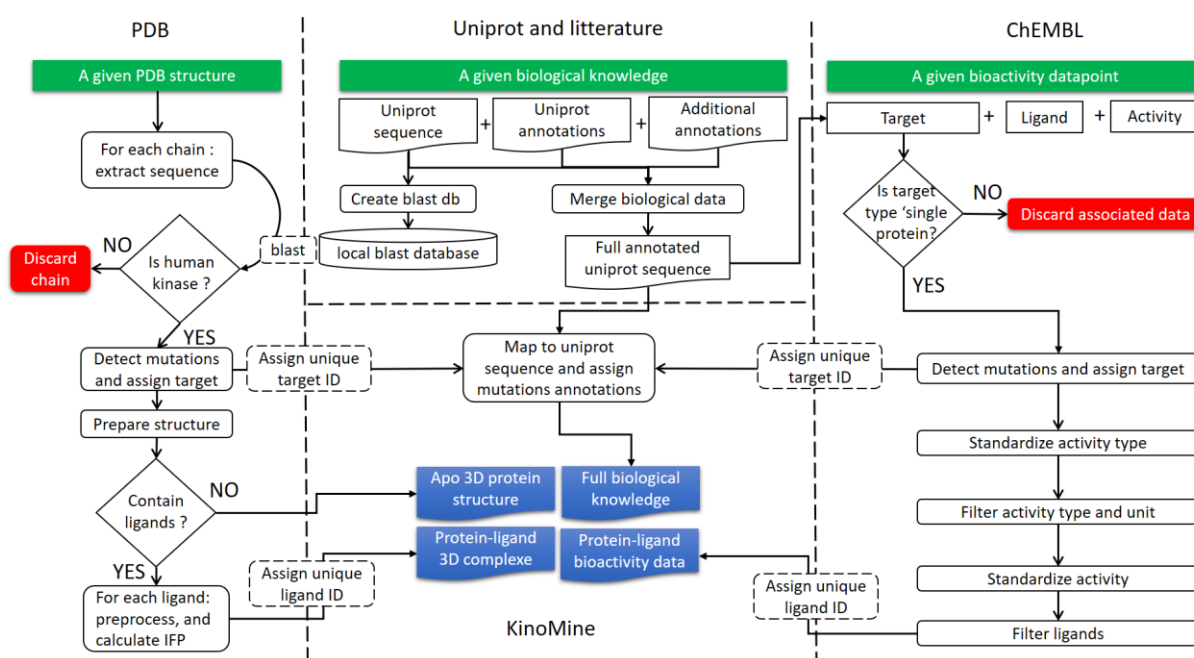
Fig. S4. Flowchart for preparation of kinase data. The process includes data ingestion of: (i) protein-ligand 3D structural data from the Protein Data Bank (PDB), (ii) biological knowledge from Uniprot and literature, and (iii) bioactivity and selectivity data from ChEMBL (green boxes). The curation and annotation process are described in white boxes. Discarded data in red and final data in blue.
