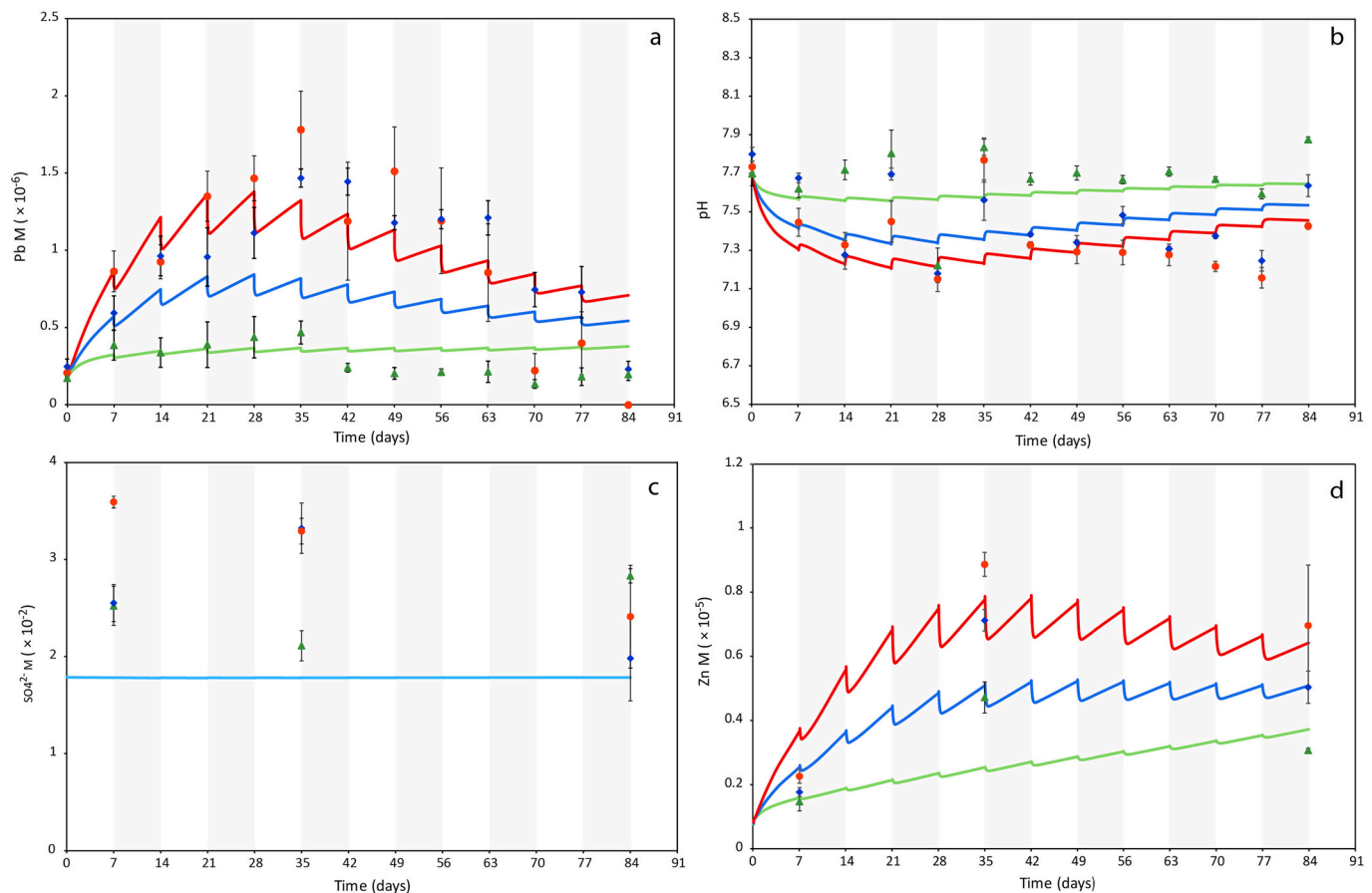
Fig. 5. Evolution with time of (a) Pb concentration, (b) pH, (c) \text{SO}_4^{2-} concentration, and (d) Zn concentration in solution, in the case of leaching experiments with tailings amended with 5 wt% ochre and manure with variable proportions (TOM). Red dots correspond to experimental data (Thouin et al., 2019), and solid lines to calculated values. The red line corresponds to 2 wt% manure, the blue line to 1 wt% manure, and the green line to 0.15 wt% manure. The light blue solid line represents the three proportions, the evolution of \text{SO}_4^{2-} concentration being independent of the amount of manure. (For interpretation of the references to colour in this figure legend, the reader is referred to the web version of this article.)
