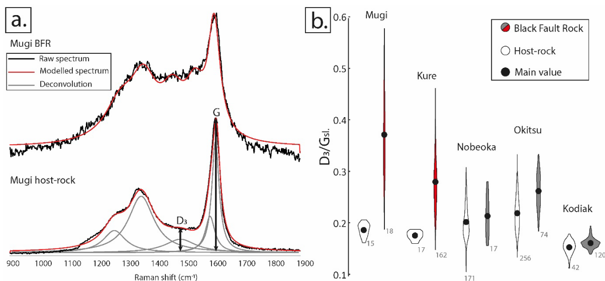
Figure VII.8 : D_3/G_{sl} ratio in Black Fault Rocks and respective host-rocks. a. Spectrum evolution in the BFR of Mugi and the host-rock indicating the intensity selected for the calculation of the D_3/G_{sl} ratio b. D_3/G_{sl} ratio diagram of 5 BFR and respective host-rocks from the Shimanto Belt and Kodiak Accretionary Complex.
