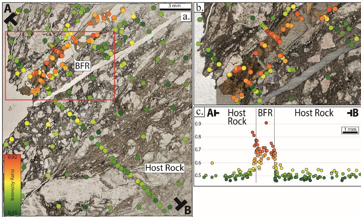
Figure VI.4: Raman Spectroscopy results obtained for the Nobeoka Black Fault Rock a . Distribution of intensity ratio over the sample – each dot corresponds to a carbonaceous particle measured by Raman spectroscopy b . Zoom in the contact of the Black Fault Rock with the host rock which shows discontinuity in the intensity ratio c . Cumulative cross-section showing the evolution of the intensity ratio perpendicular to the Black Fault Rock
