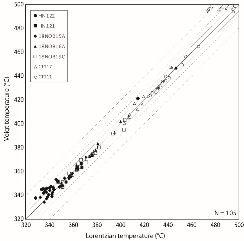
Figure III.14: Calculated temperature by the (Beyssac et al., 2002) calibration using deconvolutions with a Voigt function and Lorentzian function.
