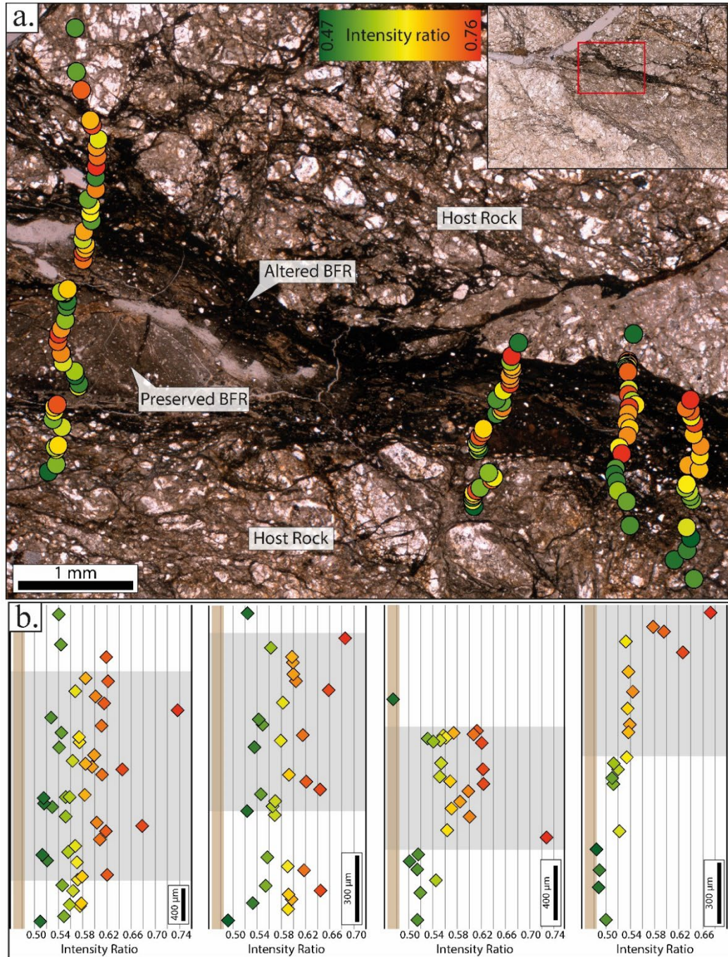
Figure VII.6 : Raman spectroscopy results obtained for the Mugi Black Fault Rock and its host-rock. a. Intensity ratio mapping along high-resolution cross-sections across the Black Fault Rock b. Intensity ratio evolution diagram along profiles.
