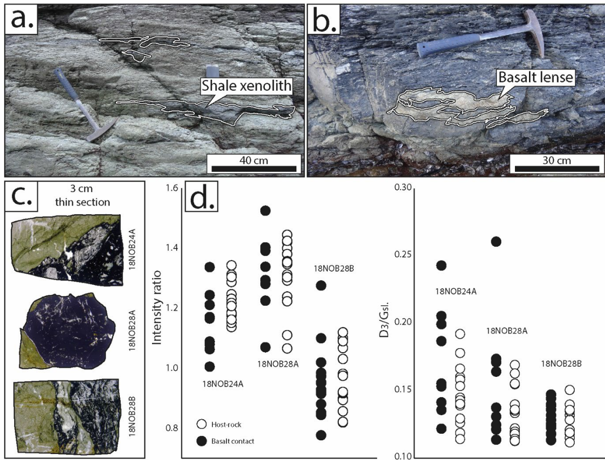
Figure VIII.5 : Structure and RSCM results in the Makimine unit. a. Xenolith of shale in metric body of basalt b. Basalt lens in a shale intercalation c. Thin sections of three samples selected from two basalt-shale contact occurrences d. Intensity ratio and D_3/G_{sl.} ratio evolution between the contact and reference material away from the contact ("host-rocks"). No systematic trend is visible.
