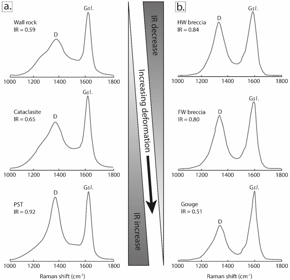
Figure II.6 – The seismic deformation effect on the Raman spectrum and intensity ratio. a. Evolution of the intensity ratio from the wall rock to the pseudotachylyte (PST) (Modified from (Ujii et al., 2021)). b. Evolution of the intensity ratio in the fault zone of Longmenshen from the fault core and surroundings (Modified from (Kuo et al., 2018)) HW = Hangingwall ; FW: Footwall.
