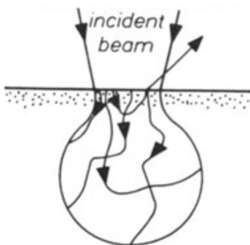
Figure A5. A schematic of the interaction between the electron beam and sample surface (produced by Roger Theisen 137 ).
