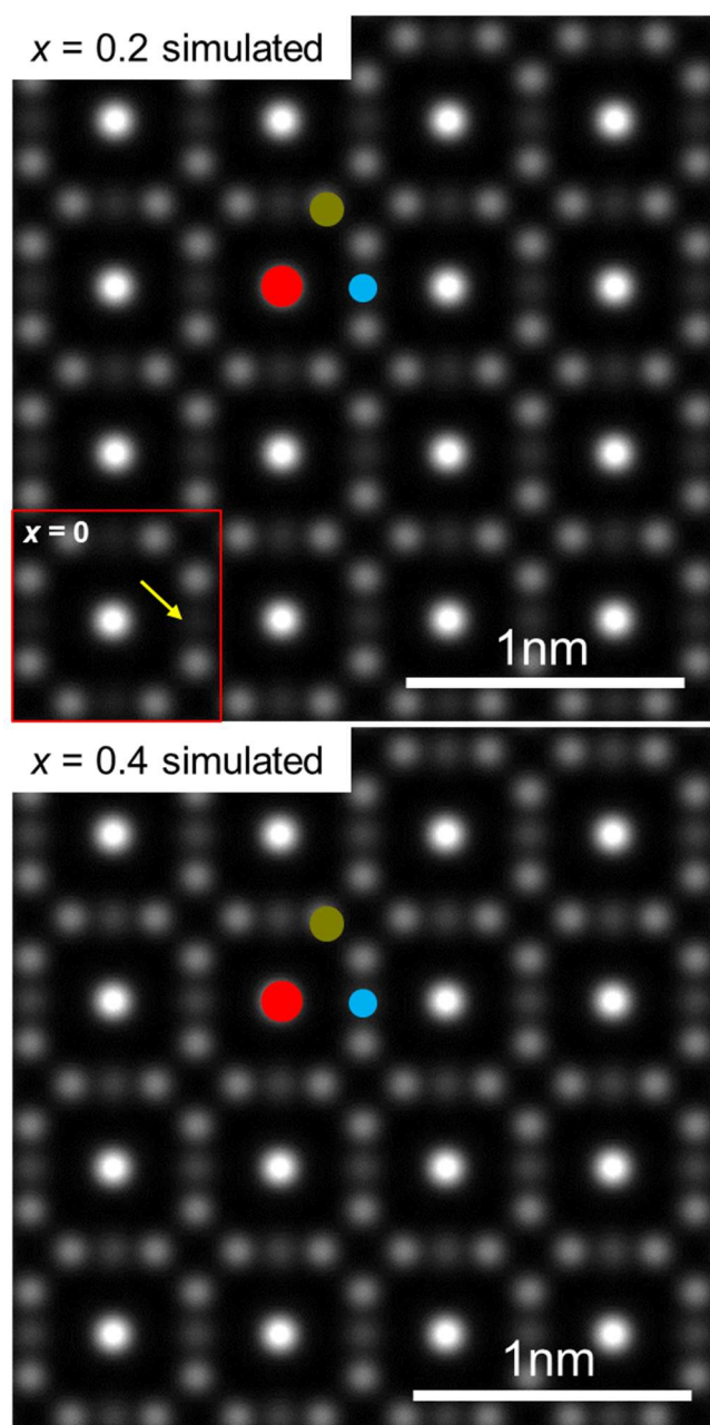
Figure 2.37. Simulated STEM-HAADF images of x = 0.2 ( \text{Y}_{3.2}\text{Al}_{4.8}\text{O}_{12} , above) and x = 0.4 ( \text{Y}_{3.4}\text{Al}_{4.6}\text{O}_{12} , below). The red, dark yellow and blue dots indicate the three typical atomic columns. The insert at the left bottom corner of the simulated STEM-HAADF image of x = 0.2 is a cropped simulated STEM-HAADF image of x = 0 ( \text{Y}_3\text{Al}_5\text{O}_{12} ), the yellow arrow indicates the 2\text{Al}1 atomic column.
