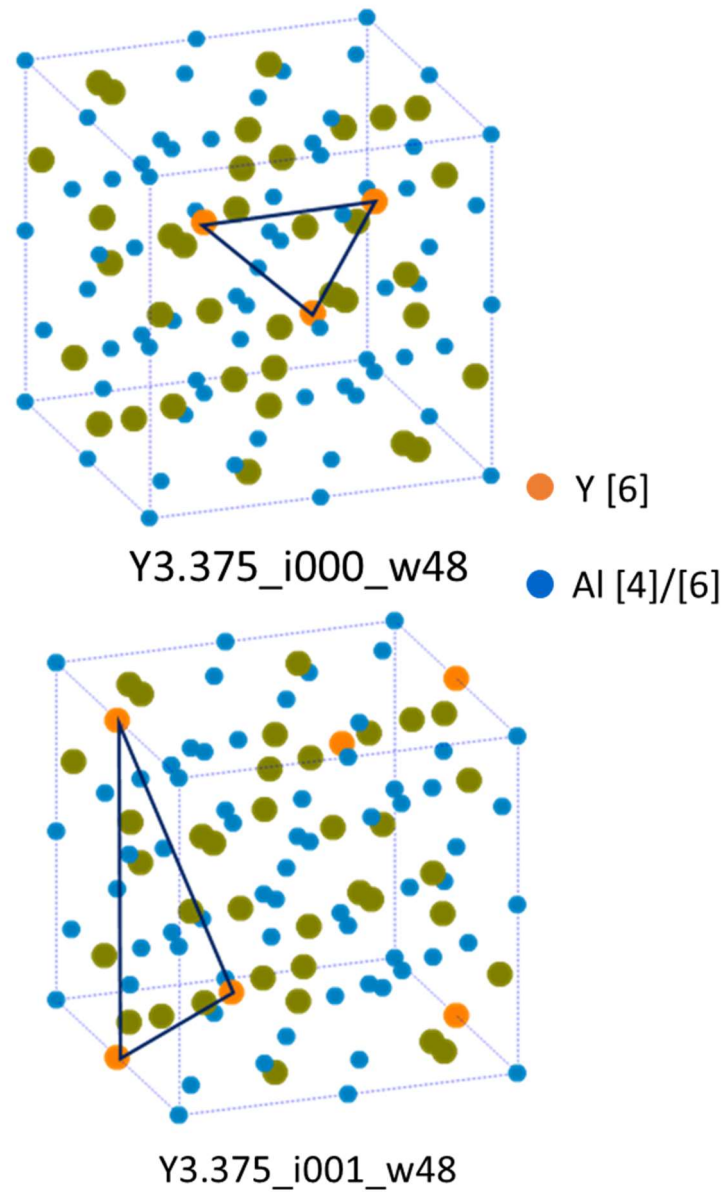
Figure 2.45. Two examples of Y_{3.375}Al_{4.625}O_{12} model with three Y defects. The vertex of the black triangle connects the involved Y defects in the models. Y defects (6-coordiante) are labelled as closed orange circles and Al (4- and 6- coordinate) atoms are labelled as closed blue circles. Oxygen atoms are not shown in these models for the sake of clarity.
