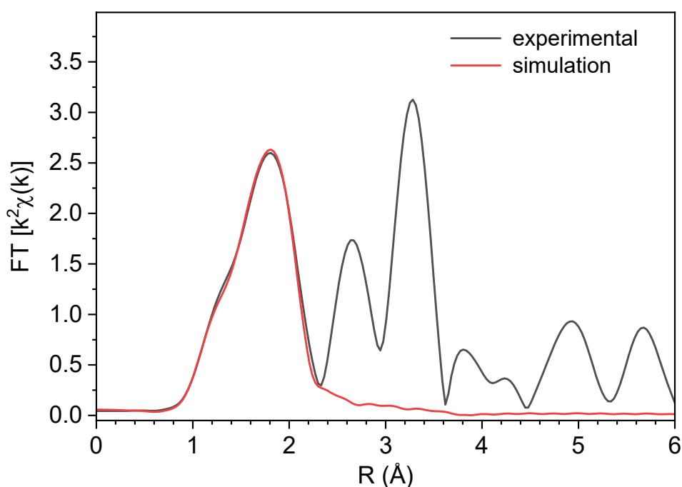
Figure 2.55. Simulation of the Fourier Transform of EXAFS oscillations on the peak in 0-2.25 Å for \text{Y}_{3.25}\text{Al}_{4.75}\text{O}_{12} .
