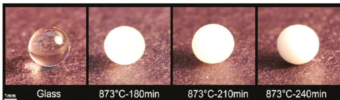
Figure 1.9. YAG–4Si glass and glass-ceramics obtained by annealing at 873 °C, for the different indicated times 22 .
