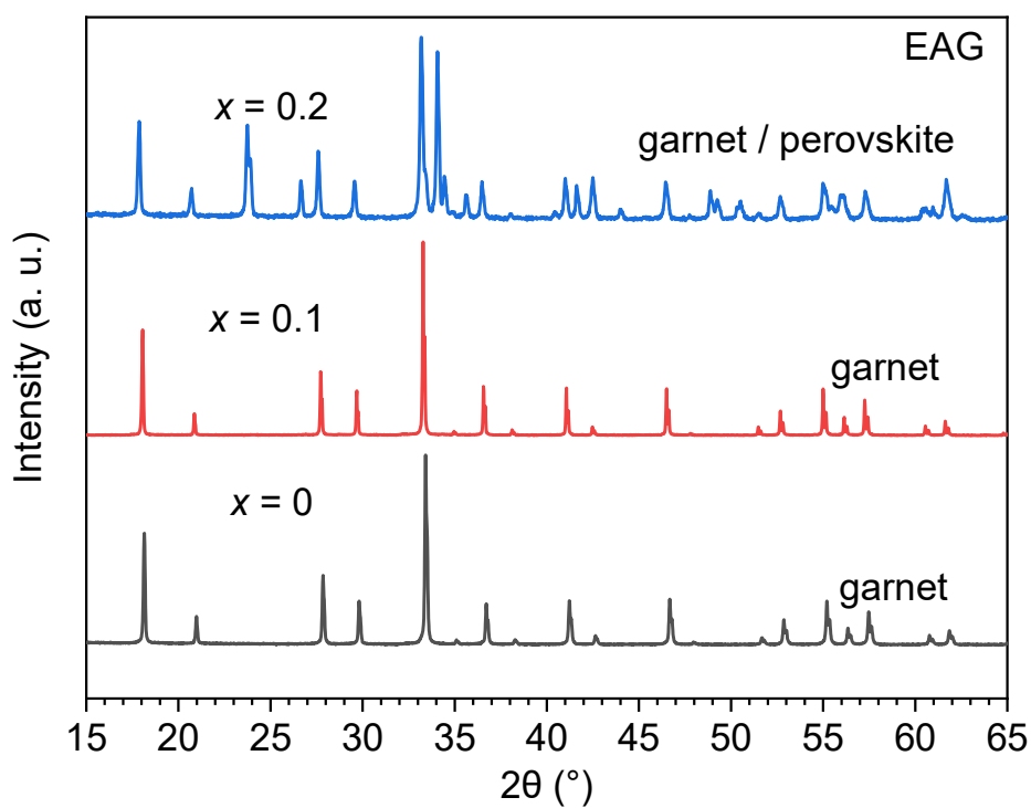
Figure 3.40. XRD patterns of \text{Er}_{3+x}\text{Al}_{5-x}\text{O}_{12} ( x = 0, 0.1 and 0.2 ) synthesized by ADL.
