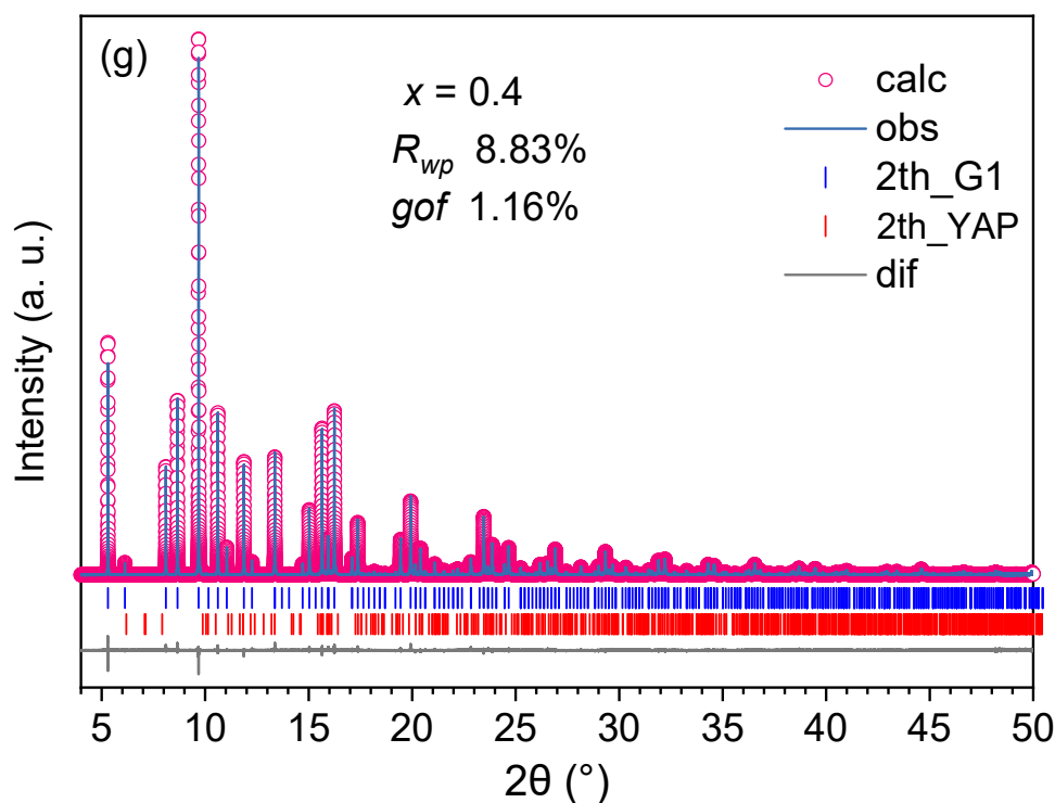
Figure B1 (a-g). Rietveld refinement plots for Y_{3+x}Al_{5-x}O_{12} ( x = 0.05, 0.1, 0.15, 0.25, 0.3, 0.35 and 0.4 ) garnets, the refinements were performed on SPD data. The blue line and pink circle respectively represent observed and calculated data. The grey line is the difference between observed and calculated data. The blue, cyan and red tick marks respectively Bragg positions of main garnet (G1), secondary garnet (G2) and perovskite (YAP).
