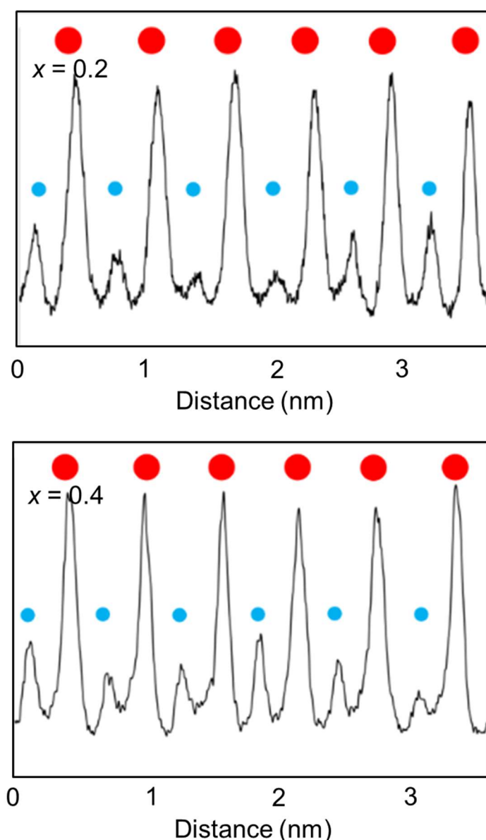
Figure 2.39. An examples of experimental intensity profiles corresponding to a succession of atomic columns of \underline{2Y1 + 2Al2} (red dots) and \underline{0.2Y + 1.8Al1} for x = 0.2 YAG, \underline{0.4Y + 1.6Al1} for x = 0.4 YAG (blue dots).
