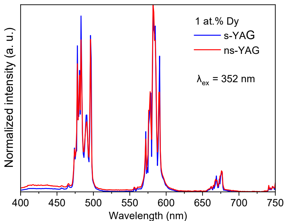
Figure 3.34. Normalized emission spectra of 1 at.% \text{Dy}^{3+} Doped s-and ns-YAGs under \lambda_{\text{ex}} = 352 nm excitation .
