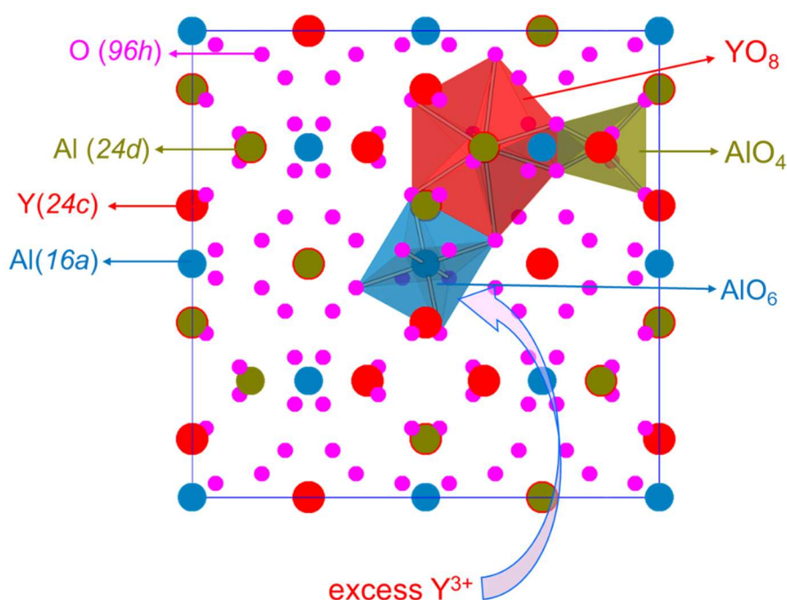
Figure 2.25. The crystal structure of Y_3Al_5O_{12} (space group: Ia-3d ). Yttrium atoms occupy 24c sites, Al atoms occupy 16a and 24d sites and O atoms occupy 96h sites. The three polyhedra indicate the Y atoms are coordinated by eight oxygen atoms, the Al atoms are coordinated by four or six oxygen atoms. The excess Y atoms form Y_{3+x}Al_{5-x}O_{12} ( x > 0 ) are expected to enter the Y 24c sites.
