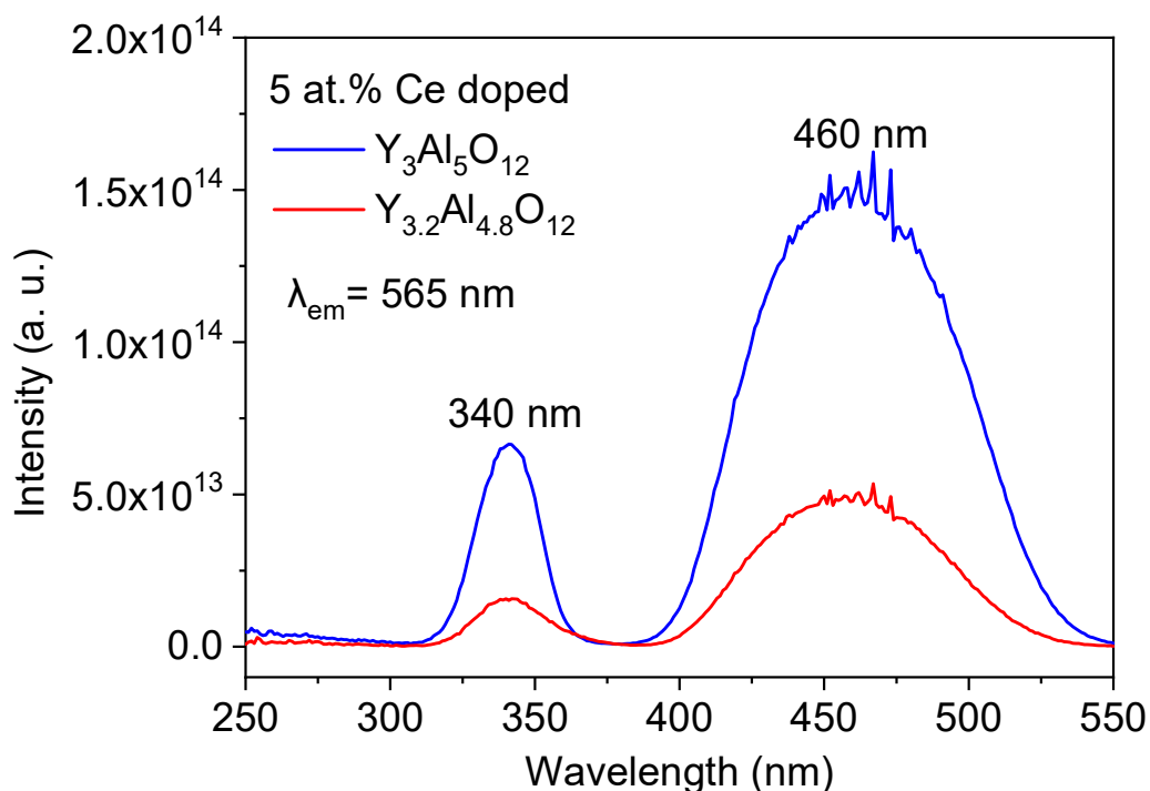
Figure 3.22. Raw excitation spectra at \lambda_{\text{em}} = 565 \text{ nm} of 5 at.% Ce doped \text{Y}_3\text{Al}_5\text{O}_{12} and \text{Y}_{3.2}\text{Al}_{4.8}\text{O}_{12} garnets.
