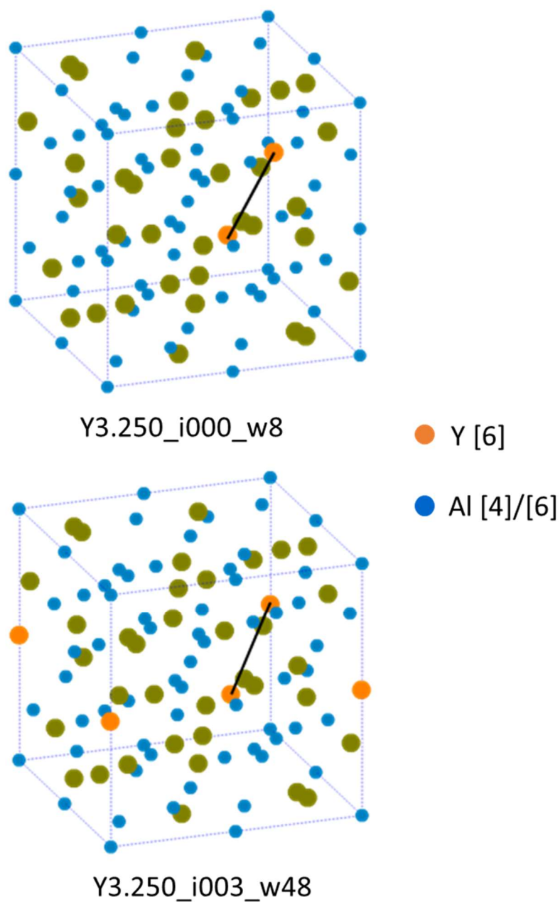
Figure 2. 44. Two examples of Y_{3.25}Al_{4.75}O_{12} model with two Y defects. The black line connects the involved Y defects in the two models. Y defects (6-coordiante) are labelled as closed orange circles and Al (4- and 6- coordinate) atoms are labelled as closed blue circles. Oxygen atoms are not shown in these models for the sake of clarity.
