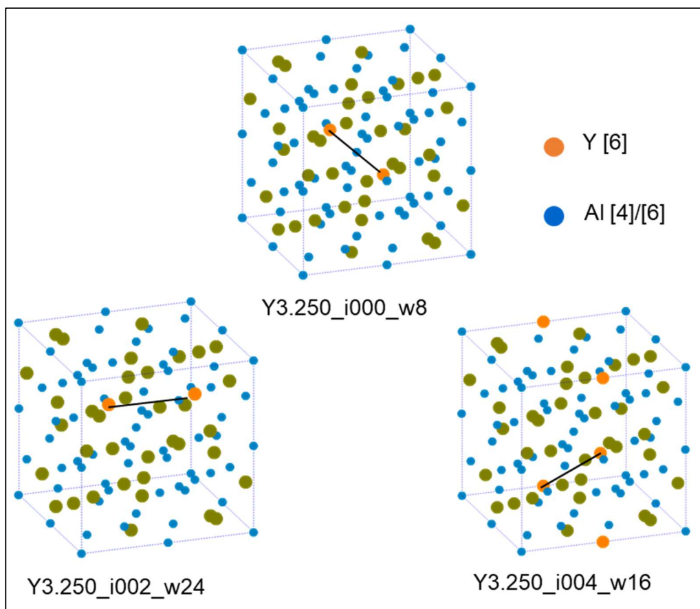
Figure B2. Three structural models for \text{Y}_{3.25}\text{Al}_{4.75}\text{O}_{12} , each model has two Y defects. The black line connects the involved two Y defects. Y defects (6-coordinate) are labelled as closed orange circles and Al (4- and 6- coordinate) atoms are labelled as closed blue circles. Oxygen atoms are not shown in these models for the sake of clarity.
