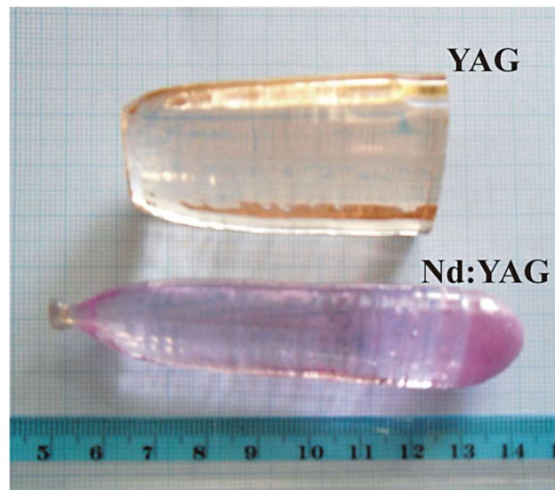
Figure 1.4. YAG and Nd: YAG crystal prepared through Czochralski method 24 by S.Kostić.
