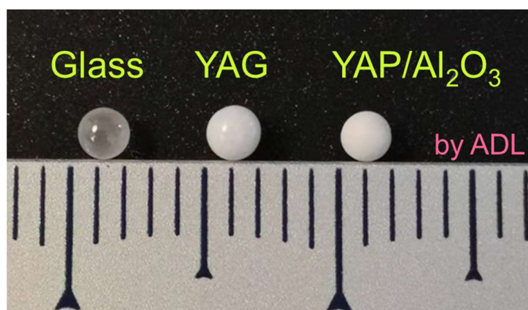
Figure 2.1. Photo of translucent glass, gloss YAG and matt \text{YAP}/\text{Al}_2\text{O}_3 beads with composition of \text{Y}_{3.2}\text{Al}_{4.8}\text{O}_{12} . All the beads were prepared by direct crystallisation in argon using ADL. The size of each bead is smaller than 2 mm in diameter.
