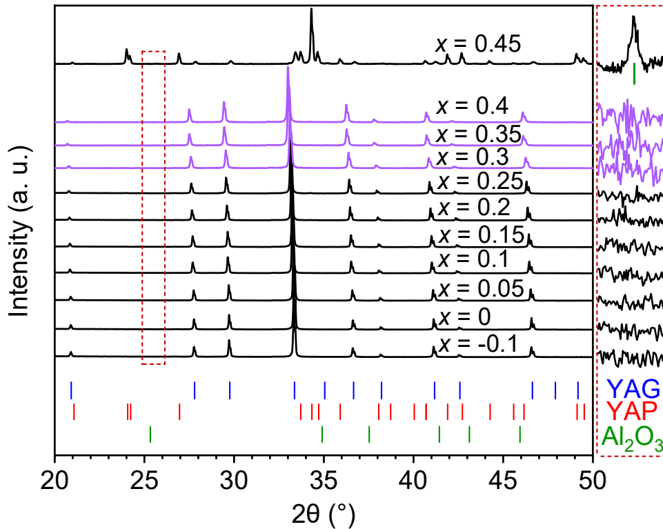
Figure 2.8. XRD patterns of Y_{3+x}Al_{5-x}O_{12} ( -0.1 \leq x \leq 0.45 ) ceramics. -0.1 \leq x \leq 0.25 (black) were crystallized directly from melt in argon, 0.3 \leq x \leq 0.4 (purple) were crystallized from glass which were obtained by fast cooling in oxygen. x = 0.45 was also prepared in oxygen and directly crystallized from melt, as it cannot be made into glass in oxygen. The blue, red and green ticks respectively indicate the Bragg diffraction positions of YAG, YAP and Al_2O_3 . XRD patterns in the dashed box on the right magnifies the diffraction patterns at 25\text{--}26^\circ 2\theta range.
