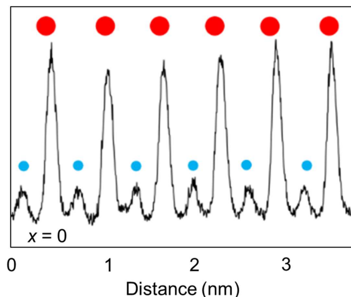
Figure 2.36. An example of experimental intensity profile considering a succession of atomic columns of 2Y1 + 2Al2 (red dots) and 2Al1 (blue dots) for x = 0 YAG.
