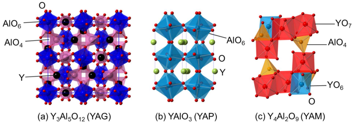
Figure 1.2. (a) YAG crystal structure. Black and red solid spheres are respectively Y and O atoms. \text{AlO}_4 tetrahedra (pink) and \text{AlO}_6 octahedra (blue) are corner-connected and, form 8-coordinate voids where \text{Y}^{3+} atoms locate. (b) YAP crystal structure. \text{AlO}_6 octahedra are corner connected, Y atoms (lime green) are in 8-coordinate voids formed by \text{AlO}_6 octahedra. Red spheres are oxygen atoms. (c) YAM crystal structure. Al atoms locate in 4-coordinate sites, Y atoms are coordinated to six or seven oxygen atoms (red).
