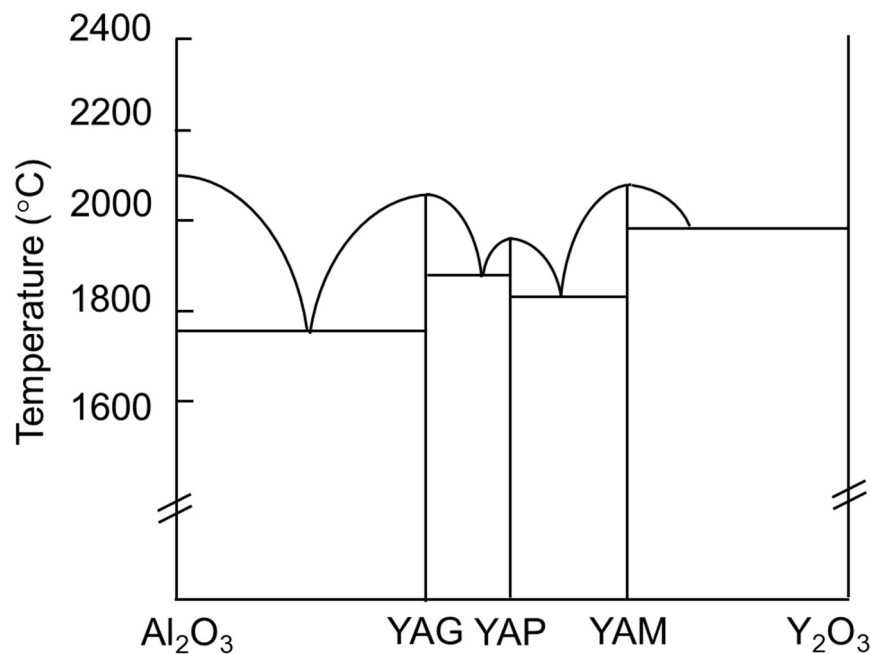
Figure 1.1. Redrawn \text{Y}_2\text{O}_3\text{--Al}_2\text{O}_3 equilibrium phase diagram by Abell et al. 40 .
