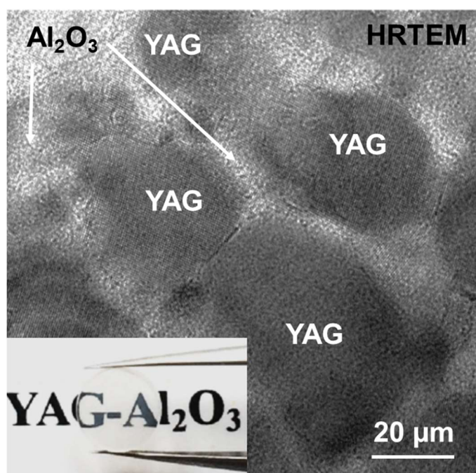
Figure 1.10. A HRTEM micrograph of the YAG- \text{Al}_2\text{O}_3 ceramic (bottom left corner), the YAG nanograins are surrounded by \text{Al}_2\text{O}_3 . This figure combined with two cropped figures the original figure from the article of X. Ma et al. 10 .
