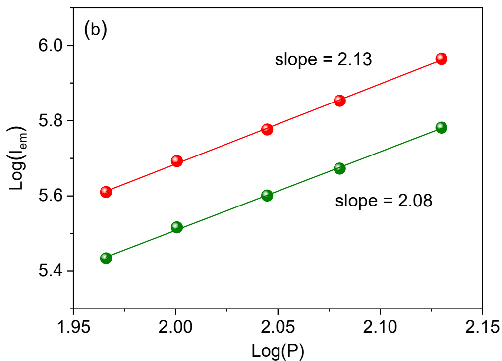
Figure 3.10. Logarithm dependence of emission intensity as a function of pump power of 980 nm laser excitation of green and red emission for 20 at.% Yb–1 at.% Er doped (a) \text{Y}_3\text{Al}_5\text{O}_{12} and (b) \text{Y}_{3.2}\text{Al}_{4.8}\text{O}_{12} .
