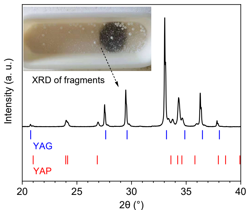
Figure 2.21. XRD pattern of fractions peeled from the sample surface. The inserted photo was recorded after the crystallisation at 1100^\circ\text{C} for 5h in a furnace, there are many fragments peeled from the sample surface.
