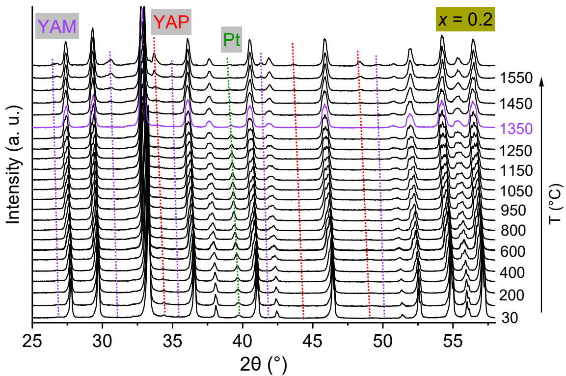
Figure 2.15. VT-XRD patterns of x = 0.2 ( \text{Y}_{3.2}\text{Al}_{4.8}\text{O}_{12} ) ns-YAG in 30–1600 °C (from fourth measurement). In 30–900 °C range and 900–1600 °C range, XRD data were respectively collected every 100 °C and 50 °C. Diffraction peak indexed by Pt comes from platinum ribbon used as sample holder.
