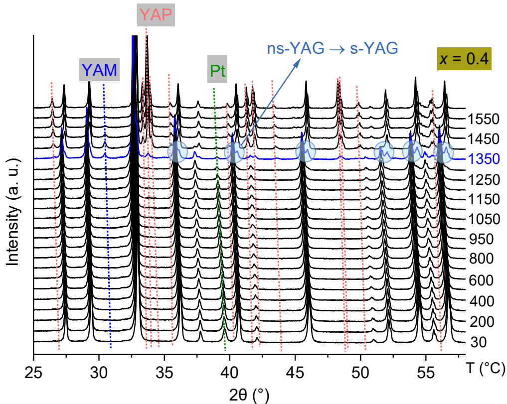
Figure 2.18. VT-XRD patterns of x = 0.4 ( \text{Y}_{3.4}\text{Al}_{4.6}\text{O}_{12} ) ns-YAG. The XRD patterns were collected under the same heating and data collecting conditions as for x = 0.2 composition. The diffraction peak of platinum comes from the ribbon where is exposed to the X-ray scanned area.
