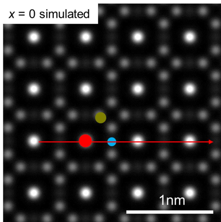
Figure 2.34. Simulated \text{Y}_3\text{Al}_5\text{O}_{12} ( x = 0 ) STEM-HAADF image extracted from cif file using JEMS software 102 . The red, dark yellow and blue dots respectively represent the \underline{2\text{Y1} + 2\text{Al2}} , \underline{1\text{Y1} + 1\text{Al2}} and 2\text{Al1} atomic columns.
