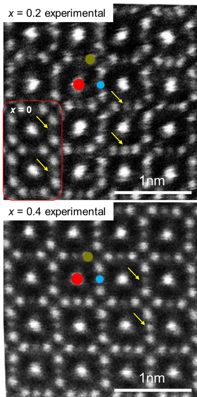
Figure 2.38. Experimental STEM-HAADF images of x = 0.2 ( \text{Y}_{3.2}\text{Al}_{4.8}\text{O}_{12} , above) and x = 0.4 ( \text{Y}_{3.4}\text{Al}_{4.6}\text{O}_{12} , below). The red, dark yellow and blue dots indicate the three typical atomic columns. The insert at the left bottom corner of the experimental STEM-HAADF image of x = 0.2 is a cropped experimental STEM-HAADF image of x = 0 ( \text{Y}_3\text{Al}_5\text{O}_{12} ). The two yellow arrows in each image point out the brightness of the two signal spots deviate from each other.
