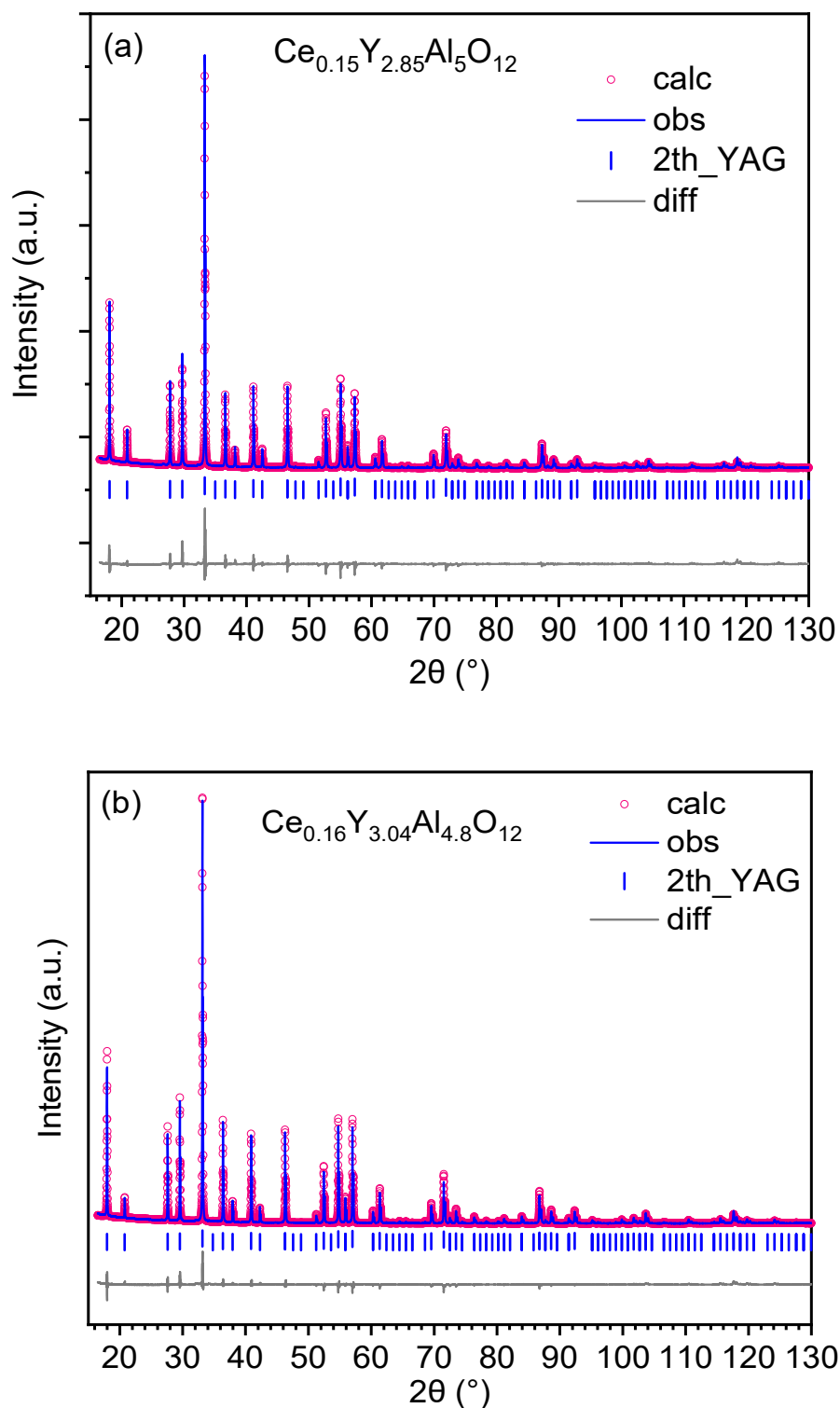
Figure 3.21. Rietveld refinement plot of \text{Ce}_{0.15}\text{Y}_{2.85}\text{Al}_5\text{O}_{12} (a) and \text{Ce}_{0.16}\text{Y}_{3.04}\text{Al}_{4.8}\text{O}_{12} (b) . The blue line and red circle respectively represent observed and calculated data, the blue tick marks represent Bragg positions of YAG phase, and the grey line represent difference between observed and calculated data. The resulted discrepancy values of the two plot (a) and (b) R_{wp} \sim 4.82\% and 4.97\% .
