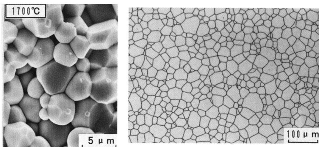
Figure 1.5. SEM photograph of YAG synthesized at 1700^\circ C (left) and reflection microscope photograph of standard 1.1 at.% Nd: YAG polycrystalline after thermal etching, produced by Ikesue et al. 45 .
