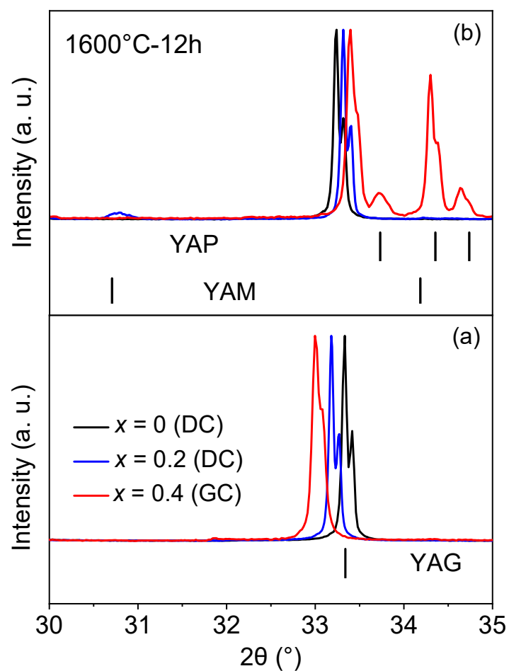
Figure 2.11. (a) XRD patterns of directly crystallized x = 0 s-YAG and x = 0.2 and fully glass crystallized 0.4 ns-YAG. (b) XRD patterns of x = 0, 0.2 and 0.4 after annealing their YAGs at 1600^{\circ}\text{C} for 12h. The ticks indicate Bragg positions of YAP, YAM and YAG as labeled.
