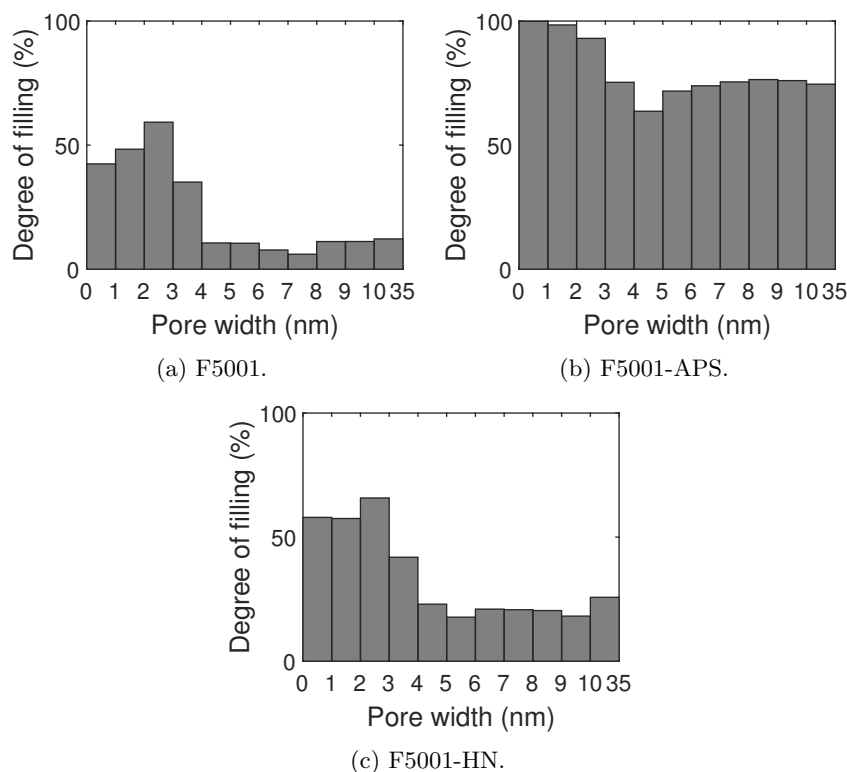
Figure 3.36: Degree of pore filling of carbon F5001 and its derivatives filled with \text{NaClO}_4 .
