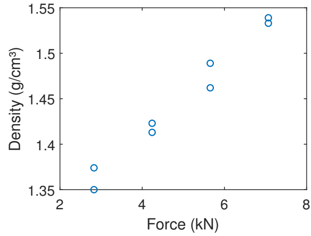
Figure A.12: Charge density in function of the force applied by means of a hydraulic press, for the filled carbon investigated in section 4.3.
