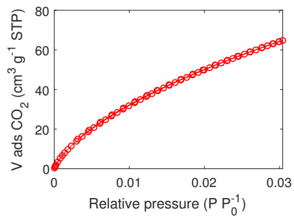
Figure C.25: \text{CO}_2 adsorption/desorption isotherm of carbon BPL measured at 273 K.
