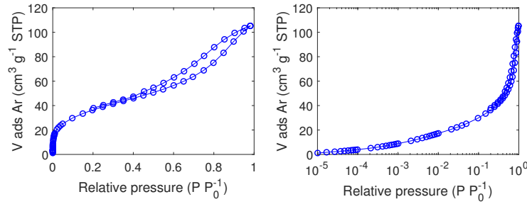
Figure D.5: Ar adsorption/desorption isotherm of carbon C filled with NaClO 4 from a 60 wt% aqueous solution measured at 87 K.
