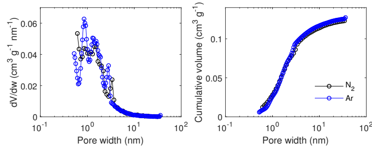
Figure D.27: Pore size distribution modelled by QSDFT based on \text{N}_2 at 77 K and \text{Ar} at 87 K adsorption/desorption isotherms for carbon BPL filled with \text{NaClO}_4 from a 40 wt% aqueous solution.
