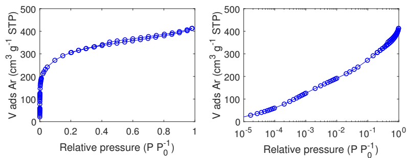
Figure C.24: \text{Ar} adsorption/desorption isotherm of carbon BPL measured at 87 K.
