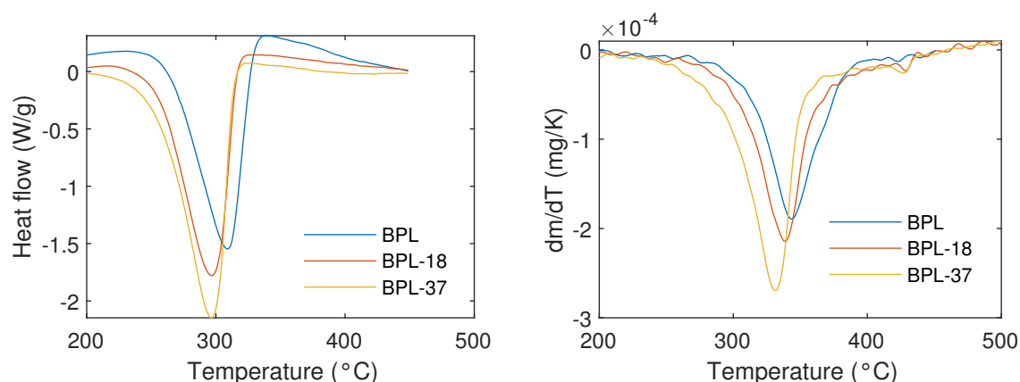
Figure 4.8: DSC and DTG results for carbon BPL and its derivatives obtained by overactivation filled with sodium perchlorate from a 56 wt% aqueous solution.
