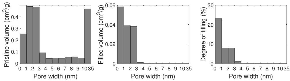
Figure 3.23: Degree of pore filling with respect to the pristine carbon for carbon F5001 filled with KNO_3 .
