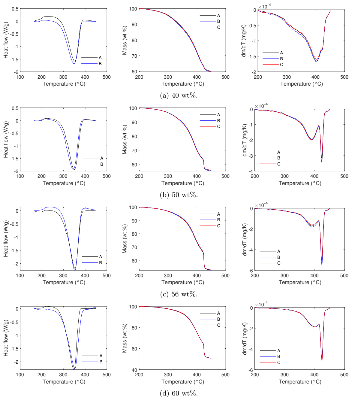
Figure H.1: DSC (left), TGA (middle) and DTG (right) results of carbon C filled with \text{NaClO}_4 from solution at different concentrations (40, 50, 56 and 60 wt%).
