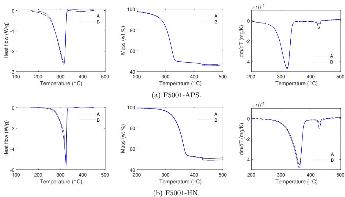
Figure H.4: DSC (left), TGA (middle) and DTG (right) results of carbon F5001 and its derivatives obtained by chemical oxidation filled with \text{NaClO}_4 from a 56 wt% solution.
