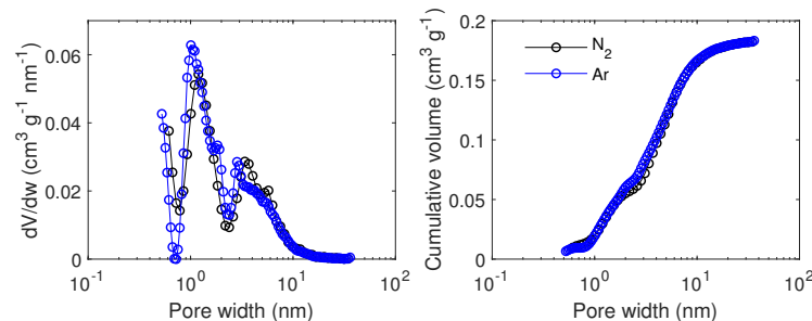
Figure D.9: Pore size distribution modelled by QSDFT based on \text{N}_2 at 77 K and \text{Ar} at 87 K adsorption/desorption isotherms for carbon C-R300 filled with \text{NaClO}_4 from a 56 wt% aqueous solution.
