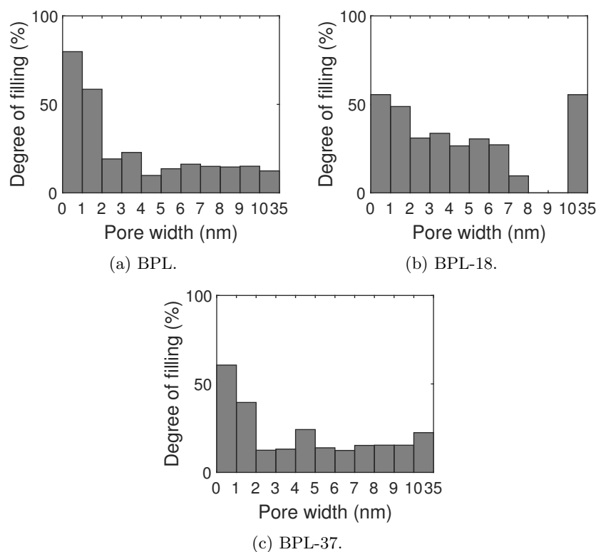
Figure 3.37: Degree of pore filling of carbon BPL and its derivatives filled with \text{NaClO}_4 .
