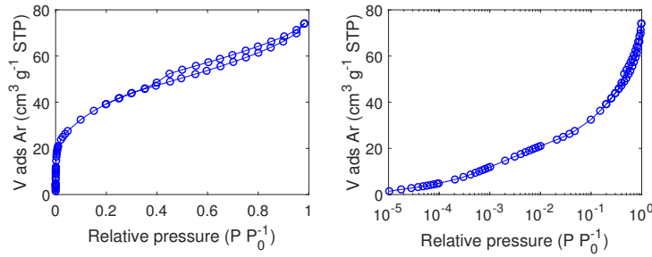
Figure D.29: \text{Ar} adsorption/desorption isotherm of carbon BPL filled with \text{NaClO}_4 from a 60 wt% aqueous solution measured at 87 K.
