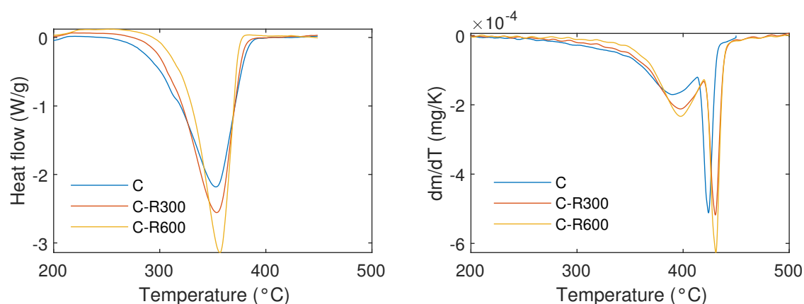
Figure 4.6: DSC and DTG results for carbon C and its derivatives obtained by thermal treatment filled with sodium perchlorate from a 56 wt% aqueous solution.
