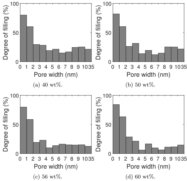
Figure 3.33: Influence of the solution concentration on the degree of pore filling for carbon BPL filled with \text{NaClO}_4 .
