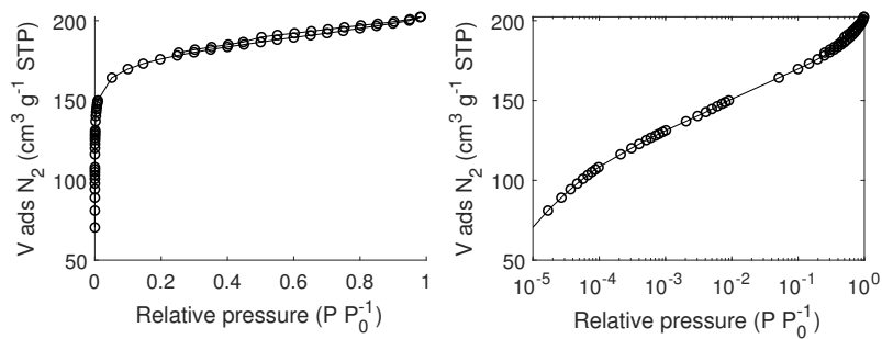
Figure C.34: \text{N}_2 adsorption/desorption isotherm of carbon FY5 measured at 77 K.
