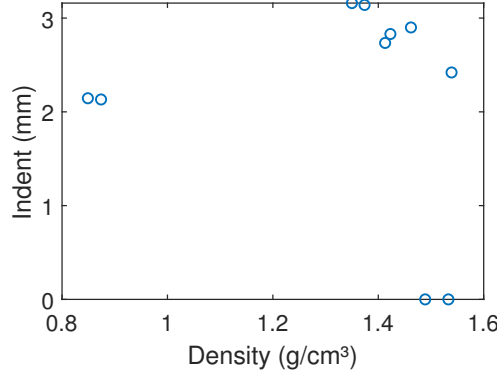
Figure 4.10: Results of the detonability preliminary study of carbon C filled with \text{NaClO}_4 from a 56 wt% aqueous solution, in a heavy confinement and initiated by a standard detonator.
