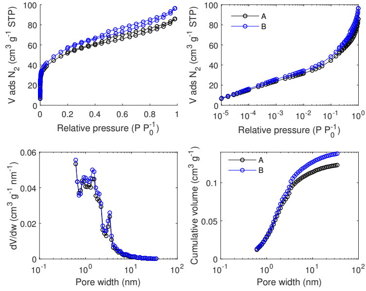
Figure F.13: N 2 adsorption/desorption isotherm data measured at 77 K and pore size analysis by equilibrium QSDFT for carbon BPL filled with NaClO 4 from a 40 wt% aqueous solution. A and B are repetitions (from the synthesis).
