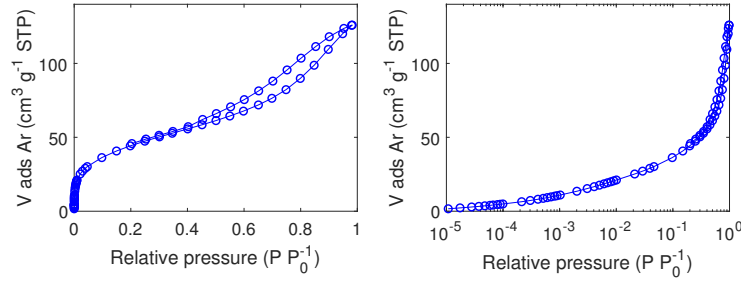
Figure D.2: \text{Ar} adsorption/desorption isotherm of carbon C filled with \text{NaClO}_4 from a 40 wt% aqueous solution measured at 87 K.
