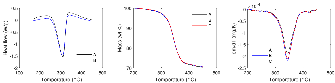
(c) 56 wt%.
