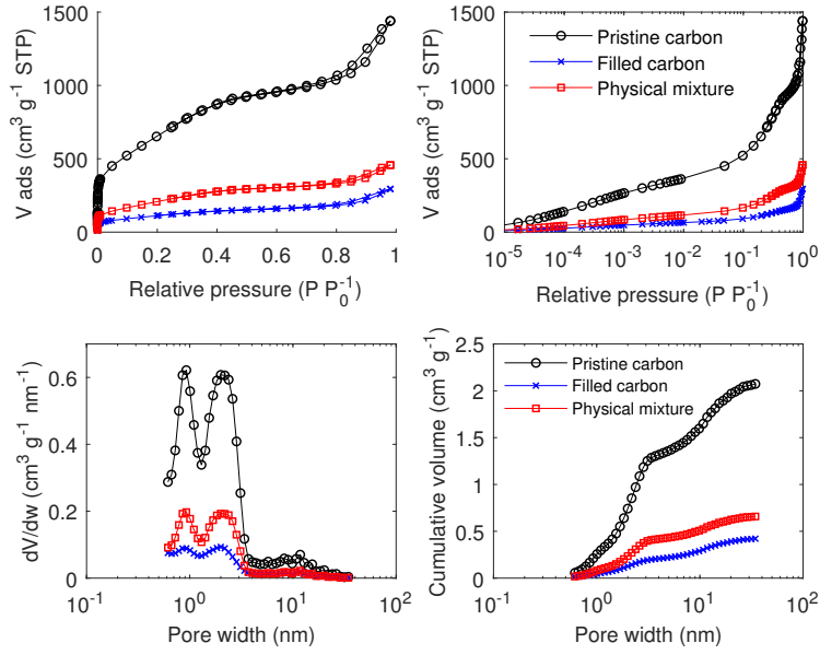
Figure 3.18: Comparison between N_2 adsorption isotherm and pore size analysis of the pristine carbon, the filled carbon and the corresponding theoretical physical mixture for carbon F5001 filled with NaClO_4 .
