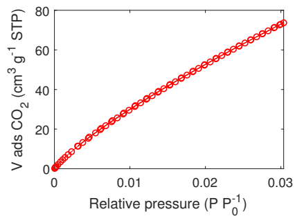
Figure C.14: \text{CO}_2 adsorption/desorption isotherm of carbon F5001 measured at 273 K.
