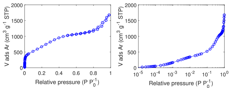
Figure C.13: \text{Ar} adsorption/desorption isotherm of carbon F5001 measured at 87 K.
