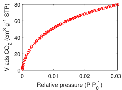
Figure C.36: \text{CO}_2 adsorption/desorption isotherm of carbon FY5 measured at 273 K.
