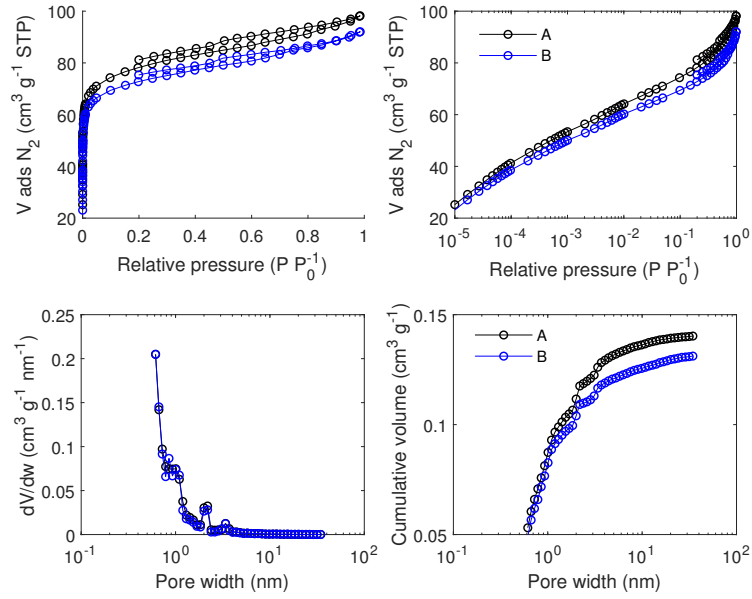
Figure F.23: N_2 adsorption/desorption isotherm data measured at 77 K and pore size analysis by equilibrium QSDFT for carbon FY5-21 filled with NaClO_4 from a 56 wt% aqueous solution. A and B are repetitions (from the synthesis).
