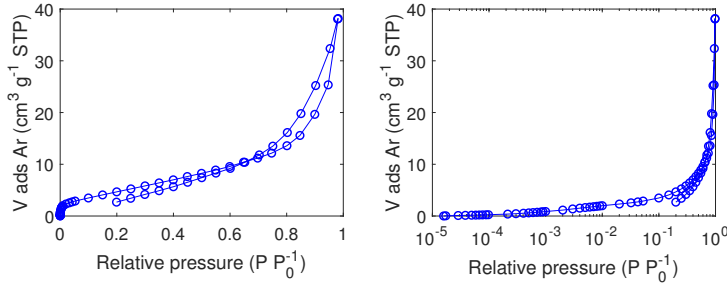
Figure D.20: \text{Ar} adsorption/desorption isotherm of carbon F5001-APS filled with \text{NaClO}_4 from a 56 wt% aqueous solution measured at 87 K.
