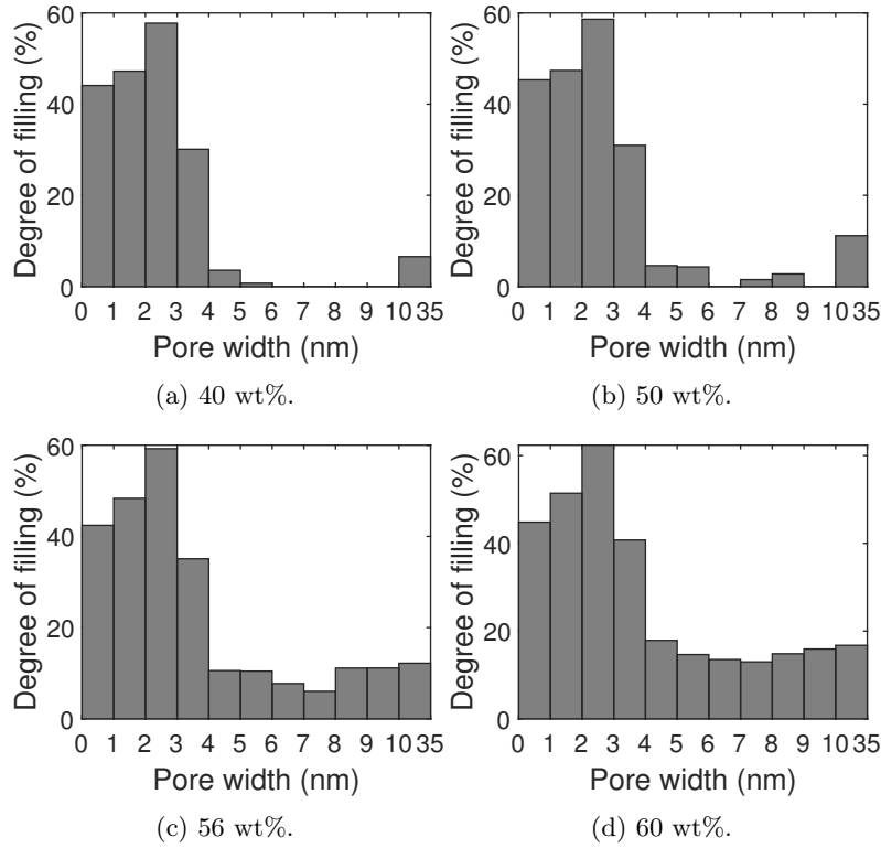
Figure 3.32: Influence of the solution concentration on the degree of pore filling for carbon F5001 filled with \text{NaClO}_4 .
