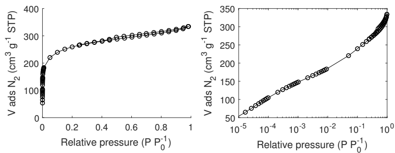
Figure C.23: \text{N}_2 adsorption/desorption isotherm of carbon BPL measured at 77 K.
