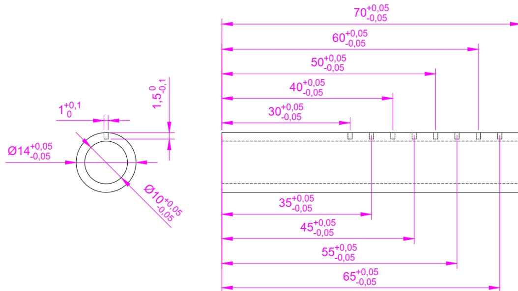
Figure A.6: Plan of the confinement tubes for charges with a diameter of 10 mm (dimensions in mm).
