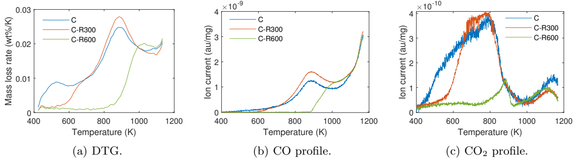
Figure 3.3: TPDMS analysis of carbon C and its derivatives obtained by thermal treatment.
