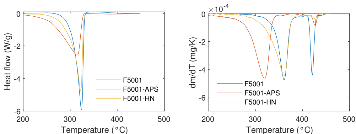
Figure 4.7: DSC and DTG results for carbon F5001 and its derivatives obtained by chemical oxidation filled with sodium perchlorate from a 56 wt% aqueous solution.
