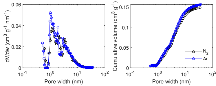
Figure D.3: Pore size distribution modelled by QSDFT based on \text{N}_2 at 77 K and \text{Ar} at 87 K adsorption/desorption isotherms for carbon C filled with \text{NaClO}_4 from a 40 wt% aqueous solution.
