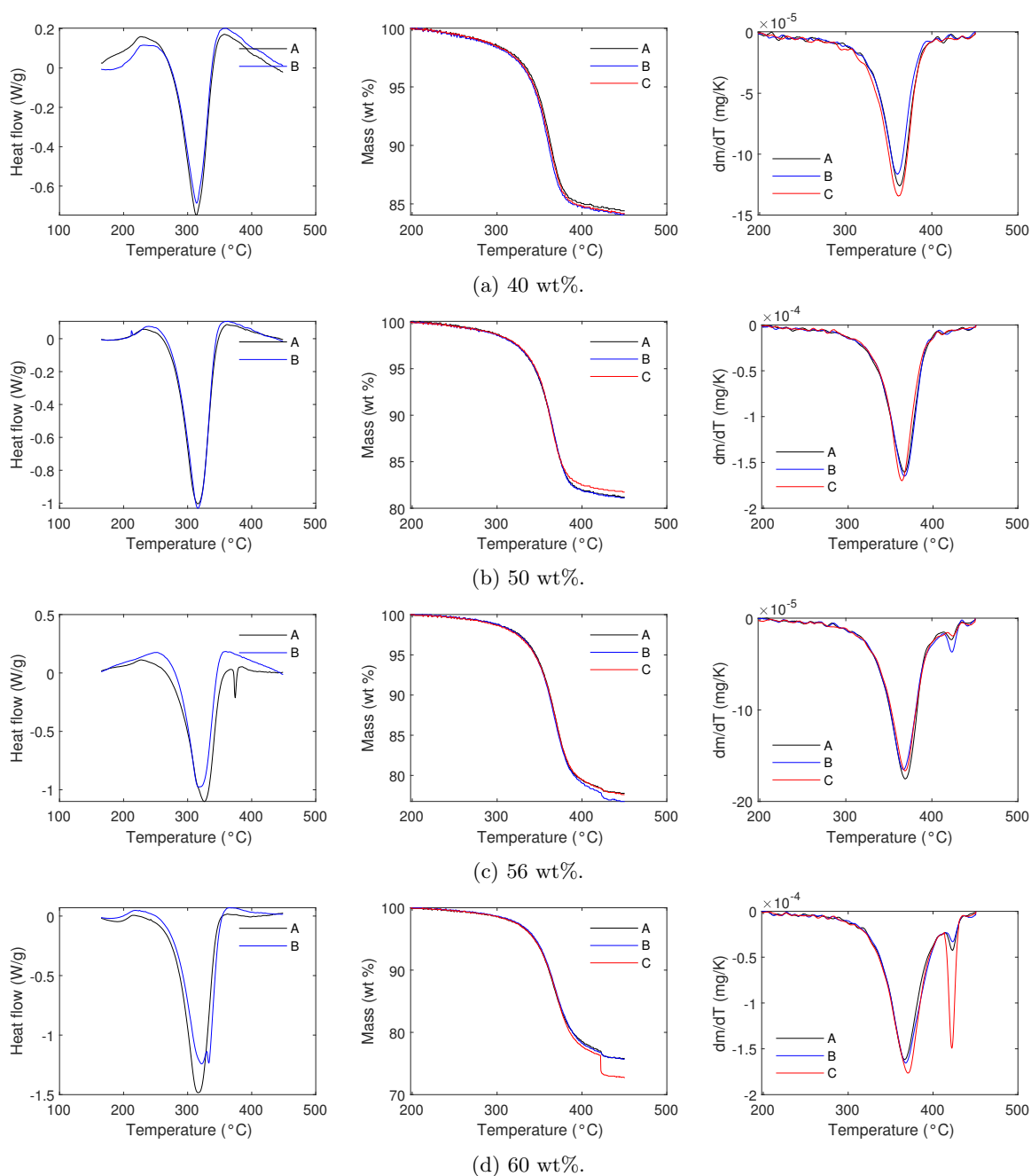
Figure H.7: DSC (left), TGA (middle) and DTG (right) results of carbon FY5 filled with \text{NaClO}_4 from solution at different concentrations (40, 50, 56 and 60 wt%).
