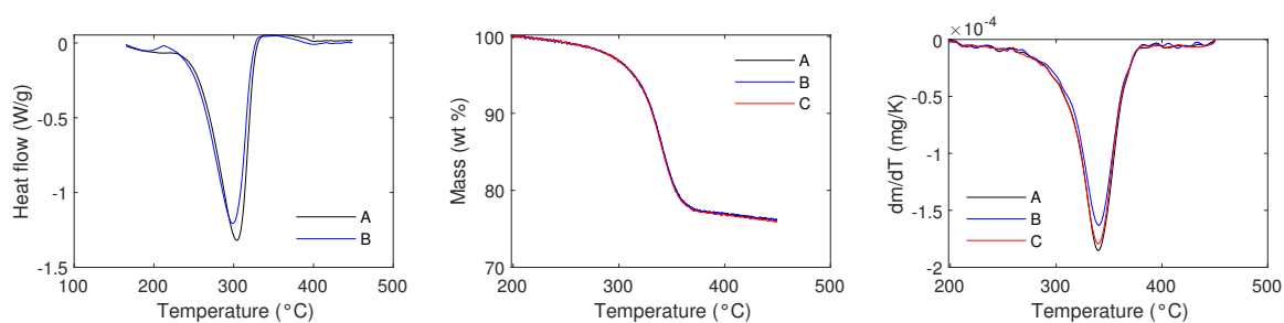
(a) 40 wt%.
