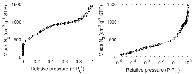
Figure C.12: \text{N}_2 adsorption/desorption isotherm of carbon F5001 measured at 77 K.
