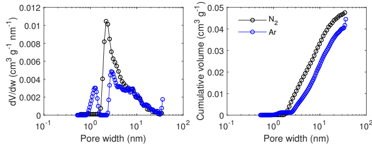
Figure D.21: Pore size distribution modelled by QSDFT based on \text{N}_2 at 77 K and \text{Ar} at 87 K adsorption/desorption isotherms for carbon F5001-APS filled with \text{NaClO}_4 from a 56 wt% aqueous solution.
