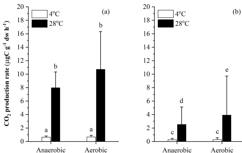
Fig. 2. CO 2 production rate ( \mu\text{gC g}^{-1} \text{ dw h}^{-1} ) of peat from (a) 5–10 cm layer and (b) 35–40 cm layer incubated at 4 and 28 °C during 7 days incubation under anaerobic and aerobic conditions. Different letters represent significant differences by ANOVA in each panel and error bars represent the standard error.
