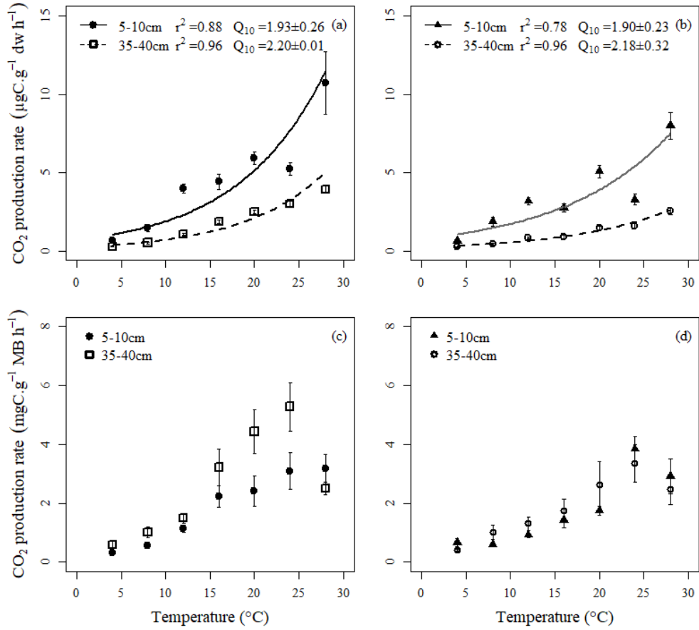
Figure VI-1 CO 2 production rate ( \mu\text{gC}\cdot\text{g}^{-1}\text{dw}\cdot\text{h}^{-1} ) under (a) aerobic and (b) anaerobic conditions; and CO 2 production per gram microbial biomass ( \text{mgC}\cdot\text{g}^{-1}\text{MB}\cdot\text{h}^{-1} ) under (c) aerobic and (d) anaerobic conditions as a function of temperature for peat from 5-10 cm and 35-40 cm layer. The lines in panels a and b correspond to the model fitted to the measurements. Error bars represent the standard deviation (SD).
