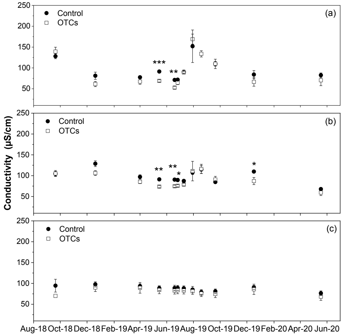
Figure III-7 Conductivity (μS/cm) of pore water from 5 (a), 15 (b) and 30 cm (c) of mesocosms under control and OTCs treatment. Error bar represents the standard error of the mean (SEM). Significant differences of one-way ANOVA are expressed as * p < 0.05 , ** p < 0.01 , *** p < 0.001 .
