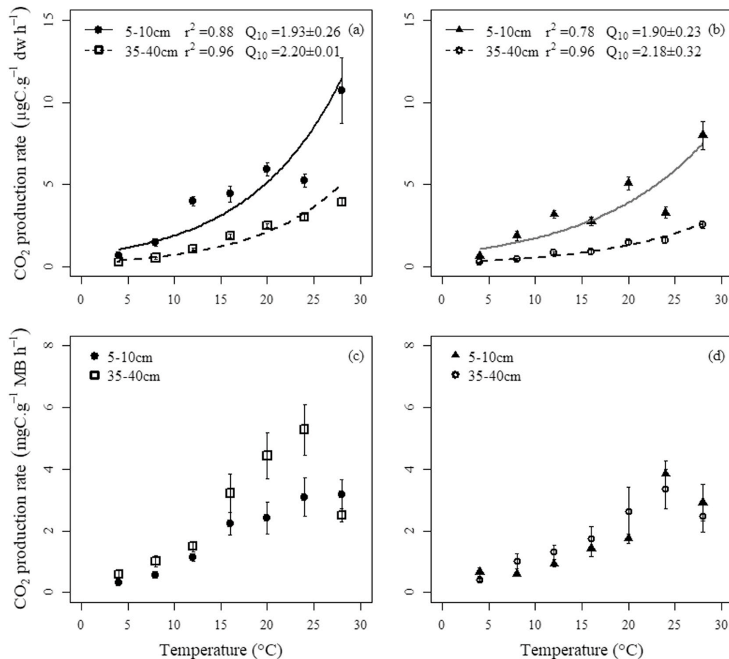
Fig. 1. CO 2 production rate ( \mu\text{gC g}^{-1} \text{dw h}^{-1} ) under (a) aerobic and (b) anaerobic conditions; and CO 2 production rate per gram microbial biomass ( \text{mgC g}^{-1} \text{MB h}^{-1} ) under (c) aerobic and (d) anaerobic conditions as a function of temperature for peat from 5–10 cm and 35–40 cm layer. The lines in panels a and b correspond to the model fitted to the measurements.
