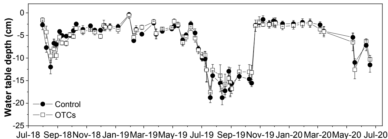
Figure III-4 Water table depth (WTD; cm) in mesocosms under control and OTCs treatment. Error bar represents the standard error of the mean (SEM).
