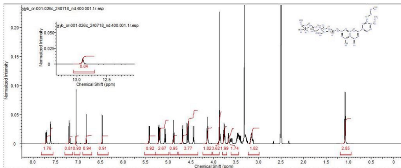
Fig. S5 ^1\text{H} NMR analysis of the Hidrosmin sample
