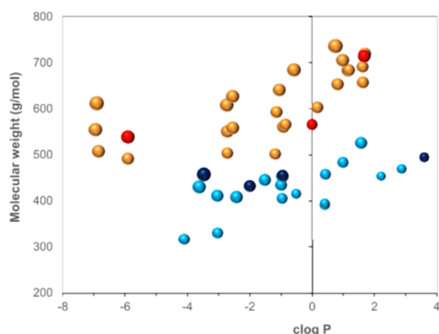
Fig. 2. Significant features of the 76 peptides examined. Molecular weight (g/mol) is plotted against calculated log P values. The bubble size is related to topological polar surface area (TPSA). Blue bubbles are linear tripeptides; orange and red bubbles are cyclic pentapeptides. The dark blue and red bubbles indicate the 10 peptides selected for method development (only 7 bubbles are visible because isomers were selected). (For interpretation of the references to color in this figure legend, the reader is referred to the web version of this article.)
