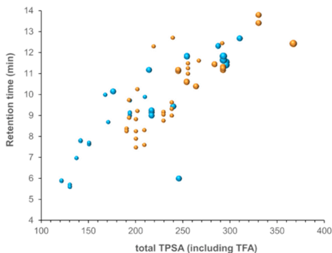
Fig. 7. Relation between retention time in the optimized method (Ascentis Express OH5 and mobile phase containing ammonium hydroxide, gradient conditions in Table 3) and topological polar surface area (TPSA) for the 76 peptides examined. Blue bubbles are linear tripeptides; orange bubbles are cyclic pentapeptides. Bubble size is related to trifluoroacetic acid (TFA) salts: smallest bubbles have no counter-ion, middle-size bubbles have one TFA counter-ion and the largest bubbles have two TFA counter-ions. (For interpretation of the references to color in this figure legend, the reader is referred to the web version of this article.)
