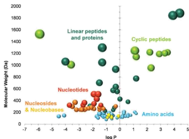
Fig. 3. Molecular weight and polarity features related to biomolecules previously analyzed with SFC or EFLC. The bubble size reflects the topological polar surface area (TPSA). The three descriptors were computed with MolDesc freeware ( http://moldesc.icoa.fr/ ).
