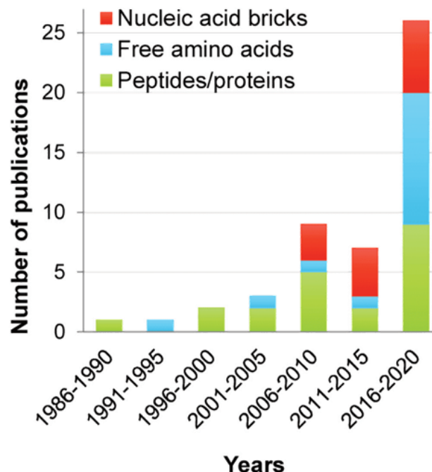
Fig. 2. Published papers related to SFC or EFLC analysis of free amino acids, peptides, proteins and nucleic acid bricks (nucleobases, nucleosides and nucleotides).
