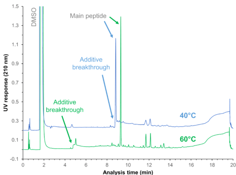
Fig. 5. Chromatograms of a selected degraded linear peptide (4693) with the generic gradient in Table S2 on Ascentis Express OH5 and mobile phase containing ammonium hydroxide at different column temperatures: 40°C or 60°C.
