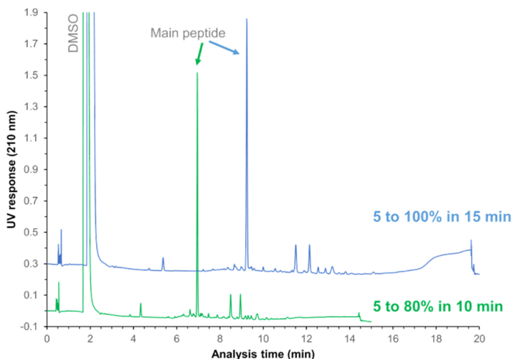
Fig. 6. Screening gradient (conditions in Table S2) and optimized gradient (conditions in Table 3) on Ascentis Express OH5 and mobile phase containing ammonium hydroxide on a selected degraded linear peptide (4693).
