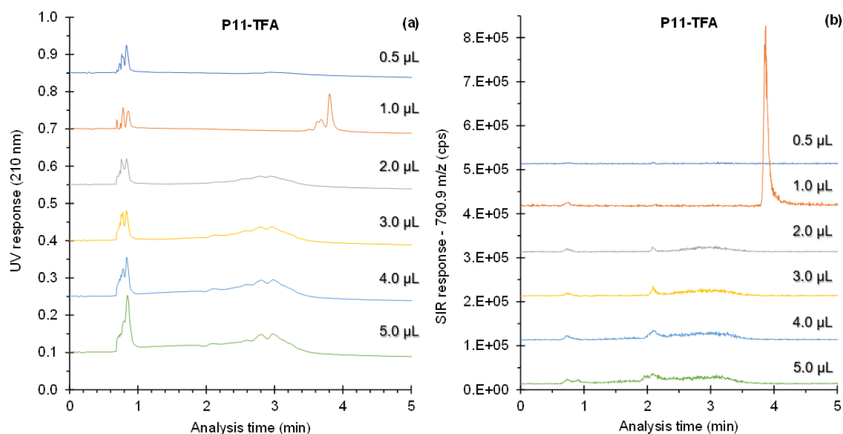
Figure 4. Impact of the injection volume (from 0.5 to 5 \mu L) on UV (a, c) and SIR (b, d) chromatograms in EFLC analysis on the peptides (a, b) P11-TFA and (c, d) P8-AcO. Each peptide was solubilized with the same solvent as the mobile phase co-solvent (methanol comprising 5% water (v/v) and 0.1% MSA). Other conditions as Figure 2.
