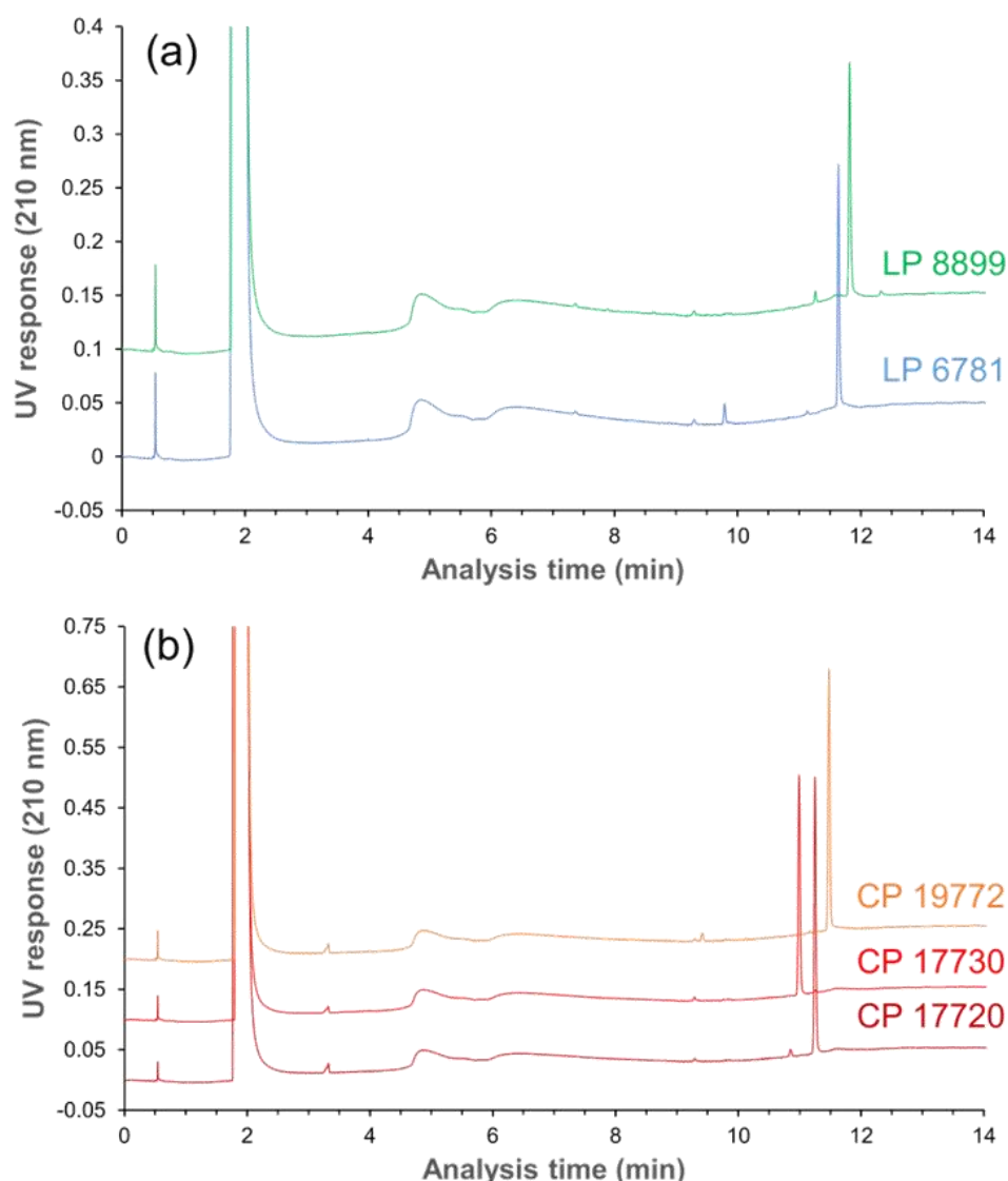
Fig. 8. Optimized conditions on Ascentis Express OH5 and mobile phase containing ammonium hydroxide (gradient conditions in Table 3) for two groups of isomers: (a) linear tripeptide positional isomers (b) cyclic pentapeptide positional and chain isomers.
