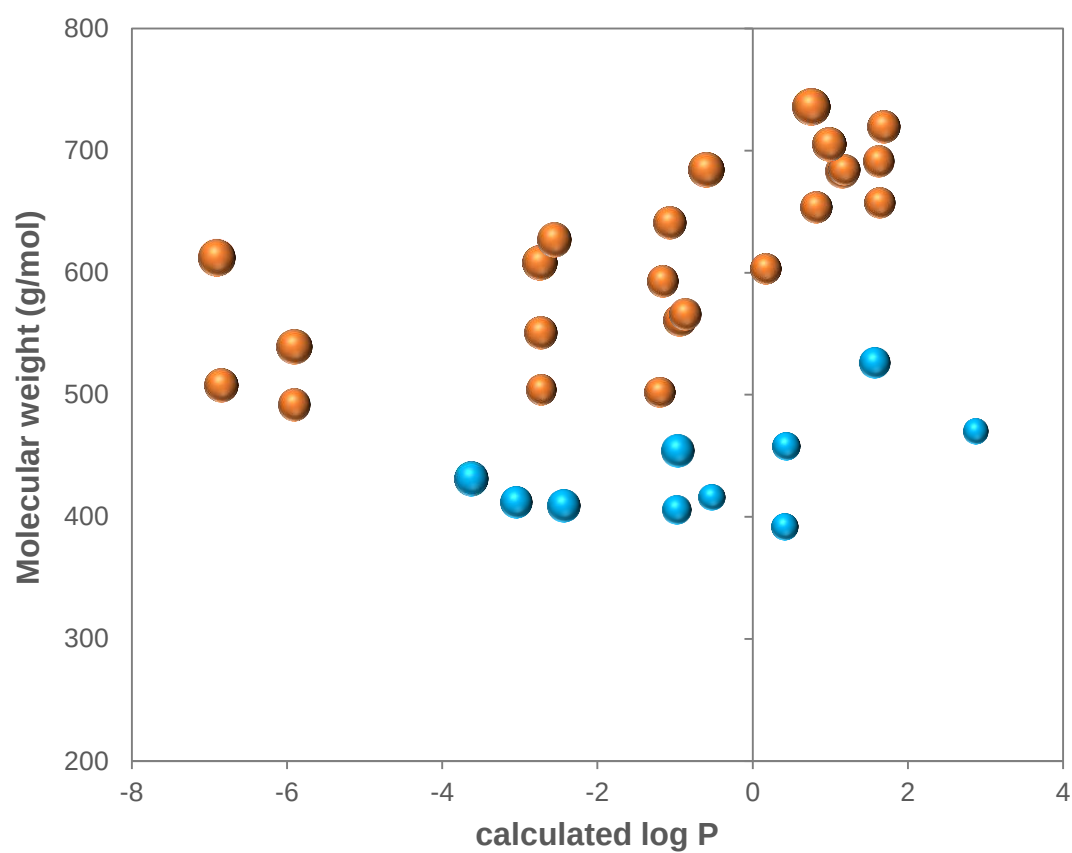
Figure S1. Significant features of the 43 peptides examined. Molecular weight (g/mol) is plotted against calculated log P values. The bubble size is related to topological polar surface area (TPSA). Blue bubbles are linear tripeptides; orange bubbles are cyclic pentapeptides.
