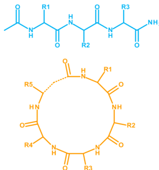
Fig. 1. General structures of the linear tripeptides and cyclic pentapeptides examined in this study.
