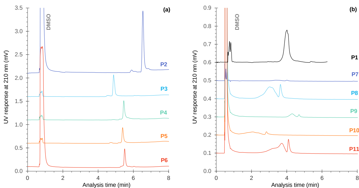
Figure 2. EFLC analysis of acidic (P2) and basic peptides TFA- salts (P1, P3-P11) on Torus 2-PIC with a co-solvent of methanol comprising 5% \text{H}_2\text{O} (v/v) and 0.1% MSA. Gradient elution from 50% to 90% co-solvent, with reversed flow-rate gradient from 0.7 to 0.5 ml/min. (a) Acceptable chromatographic peak shapes (b) distorted chromatographic peaks. Oven temperature 25°C, back-pressure 120 bar.
