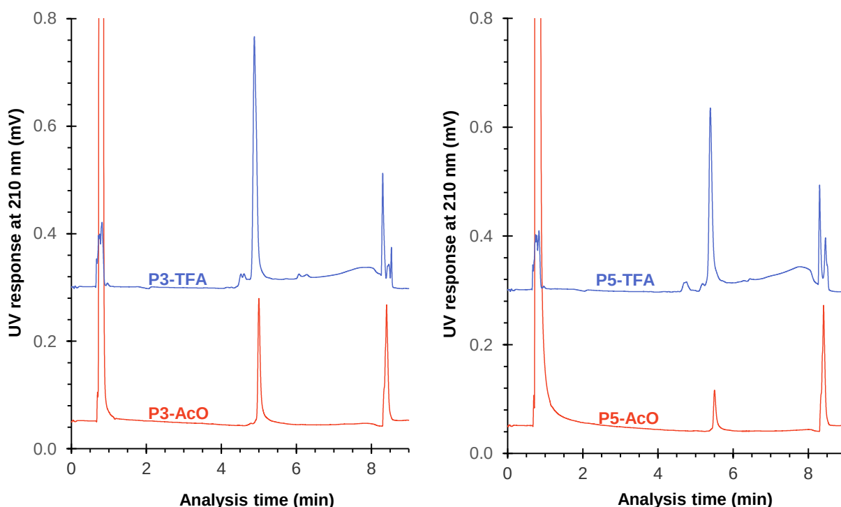
Figure 3. EFLC analysis of the same basic peptides (P3 and P5) with TFA- salts in blue or AcO- salts in red. Analysis on column Torus 2-PIC with a co-solvent of methanol comprising 5% H 2 O (v/v) and 0.1% MSA. Gradient elution from 50% to 90% co-solvent, with reversed flow-rate gradient from 0.7 to 0.5 ml/min. Oven temperature 25°C, back-pressure 120 bar.
