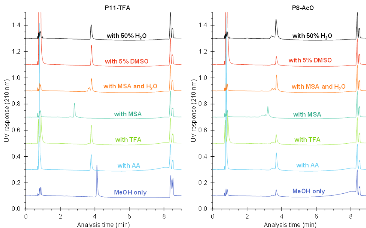
Figure 5. Impact of the dilution solvent composition on UV chromatograms in EFLC analysis on the basic peptide salts P11-TFA and P8-AcO. 1 \mu L injected. Other conditions as Figure 2
