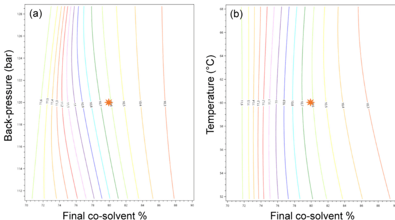
Fig. 7. Design of experiment to assess the variation of retention factor in UC conditions. (a) Effect of back-pressure vs. final gradient composition. (b) Effect of oven temperature vs. final gradient composition. The stars indicate the set conditions in generic UC gradient.
