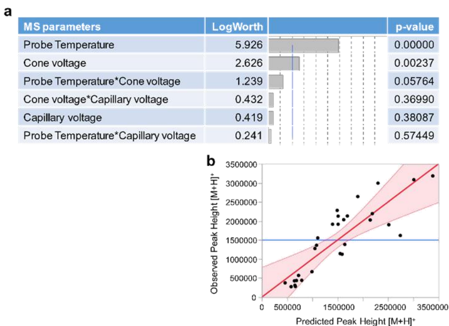
Fig. 3 Results of the design of experiments for MS response optimization on epigallocatechin gallate. a Effects of the three selected parameters. b Observed vs. predicted peak heights of the [M+H] + ion
