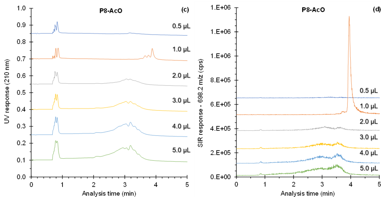
Figure 4. (continued). Impact of the injection volume (from 0.5 to 5 \mu\text{L} ) on UV (a, c) and SIR (b, d) chromatograms in EFLC analysis on the peptides (a, b) P11-TFA and (c, d) P8-AcO. Each peptide was solubilized with the same solvent as the mobile phase co-solvent (methanol comprising 5% water (v/v) and 0.1% MSA). Other conditions as Figure 2.
