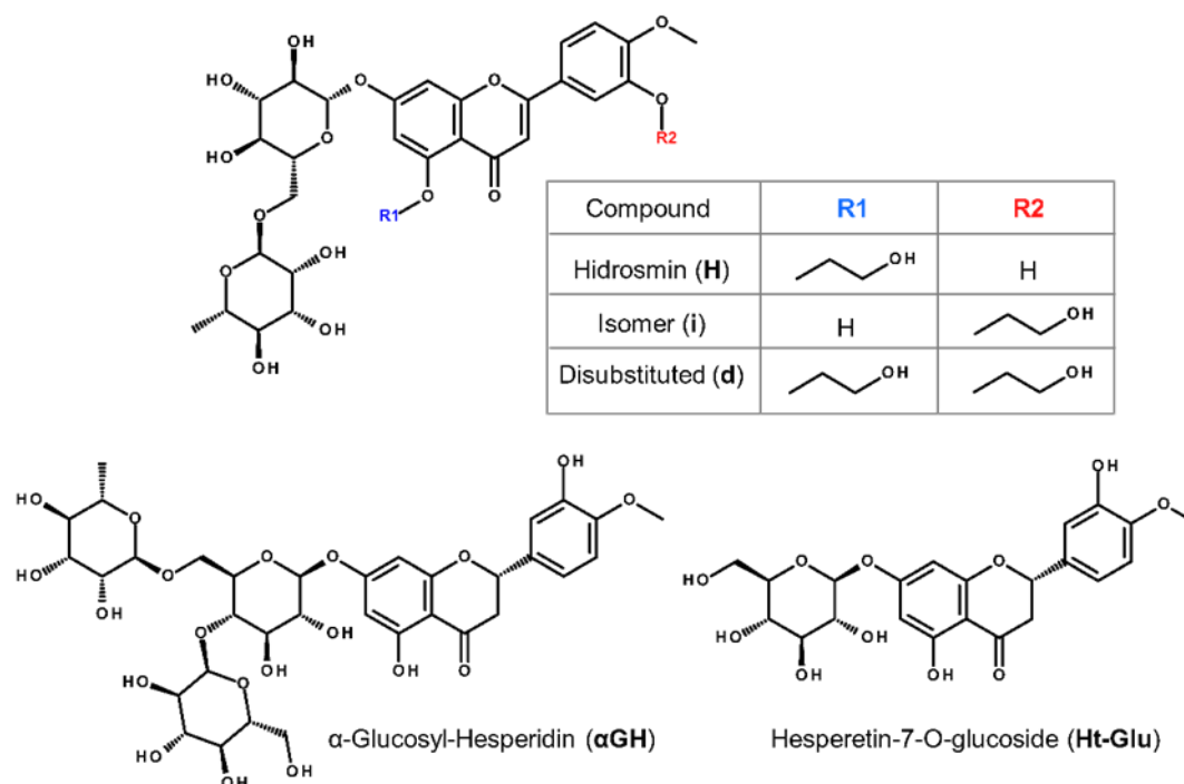
Fig. 6 Structures expected and observed in the pharmaceutical and cosmetic samples
