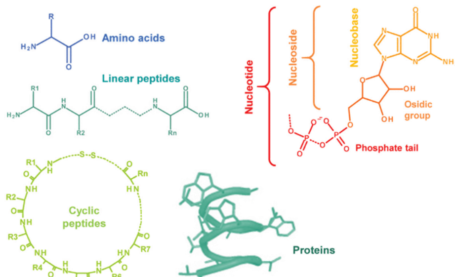
Fig. 1. Generic and representative structures of the target molecules reported in the literature reviewed in this paper.
