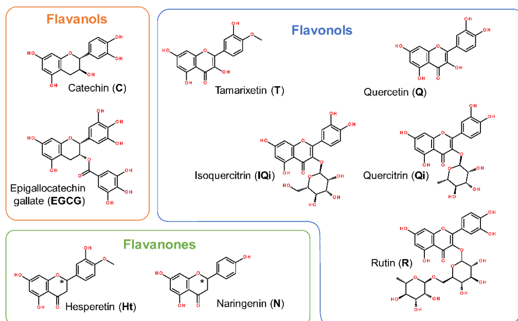
Fig. 1 Structures of the standard molecules used to develop the UC-DAD-ESI-MS method
