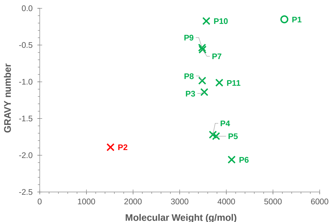
Figure 1. Description of the peptide set by physical properties. Crosses are linear peptides, the circle is a cyclic peptide (disulfide bridges). The red cross is an acidic peptide while all others are basic peptides.
