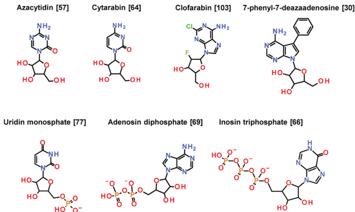
Fig. 6. Sample nucleosides and nucleotides previously analyzed with SFC and EFLC.
