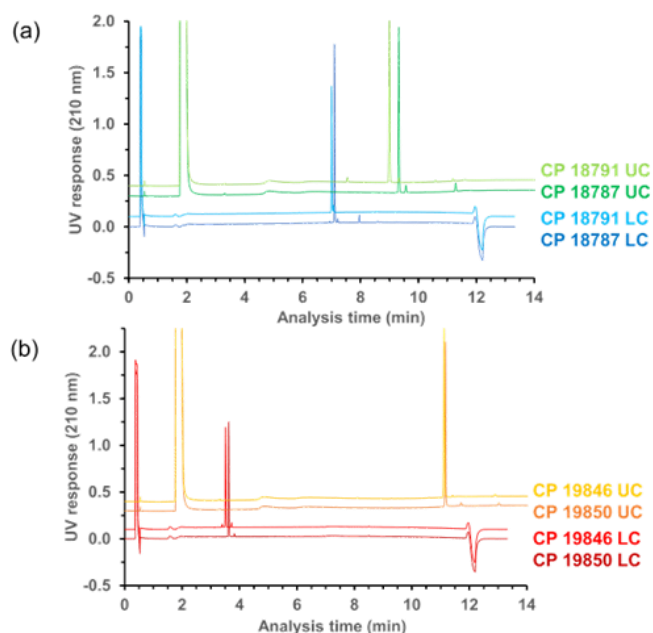
Fig. 6. Chromatograms for two pairs of isomers in UC and RPLC under generic gradient conditions (a) cyclic pentapeptides better resolved with UC (b) cyclic pentapeptides better resolved with RPLC.
