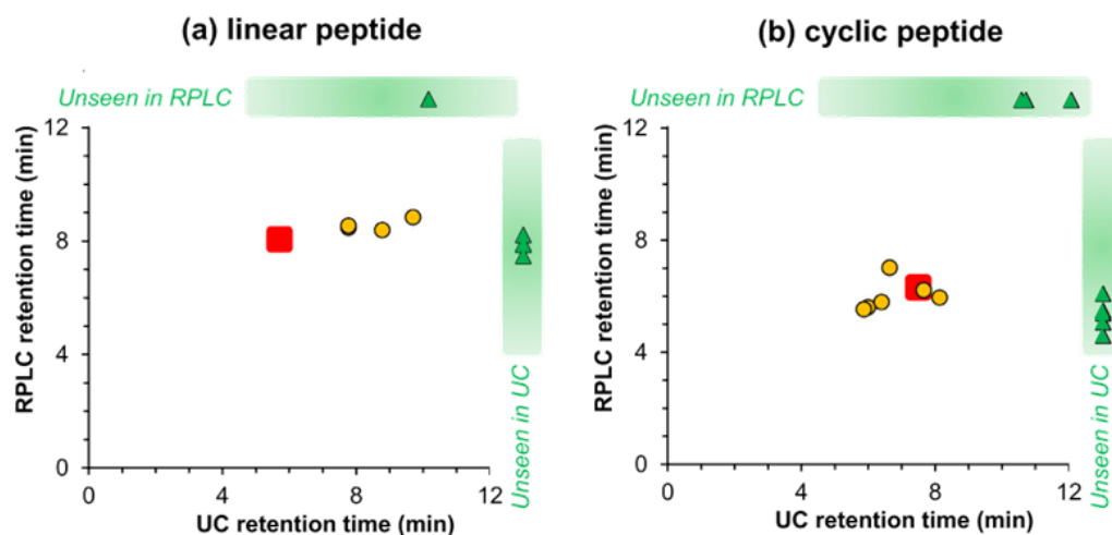
Fig. 5. Comparison of retention times obtained for the API (red square) and impurities. Yellow circles are impurities observed with both RPLC and UC methods, green triangles are impurities observed with only one method: green triangles at the top of the figure were seen with UC only, green triangles at the right of the figure were seen with RPLC only.
