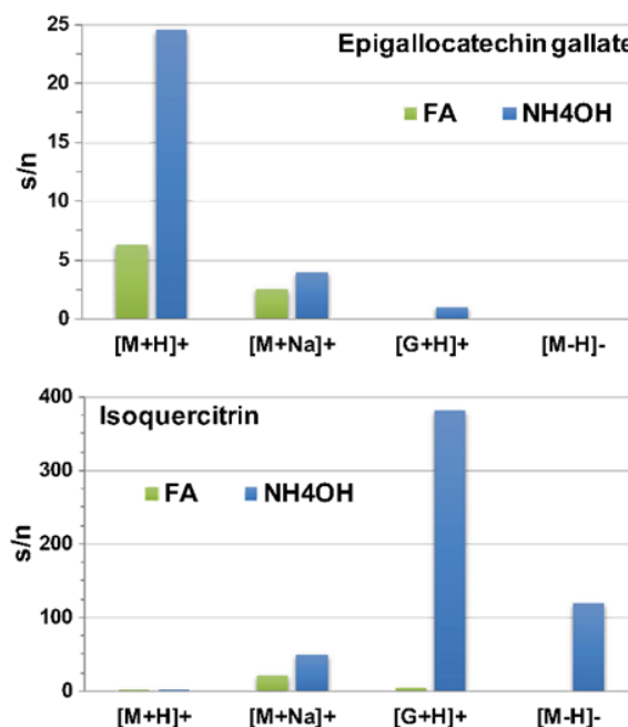
Fig. 4 Comparison of signal-to-noise (s/n) measured on the DEA column with the gradient method in Table 2a and mobile phase co-solvent containing 0.1% MSA. Make-up fluid contains either formic acid (FA, in green) or ammonium hydroxide and water (NH 4 OH, in blue)
