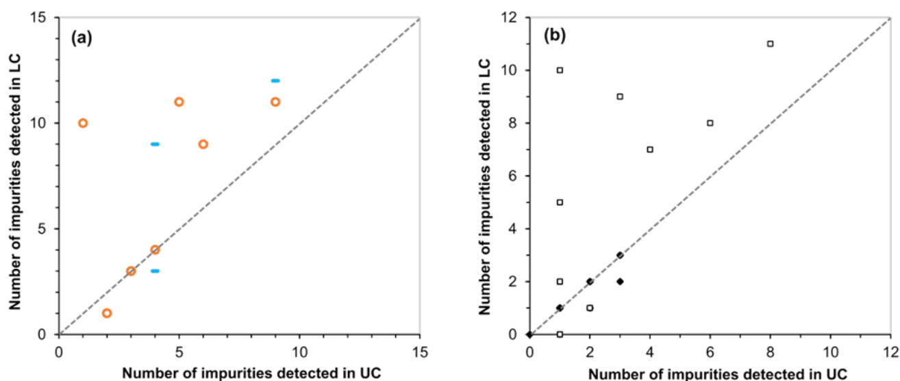
Fig. 4. Comparison of the number of impurities observed with both generic gradient methods, for 12 peptides that were successfully analyzed with both methods. (a) Total number of impurities observed for linear peptides (blue dashes) and cyclic peptides (orange circles). (b) Impurities with large concentration (>1%, black diamonds) and low concentration (<1%, open squares). The interrupted grey line is the first bisector, indicating identical values measured with both methods.
