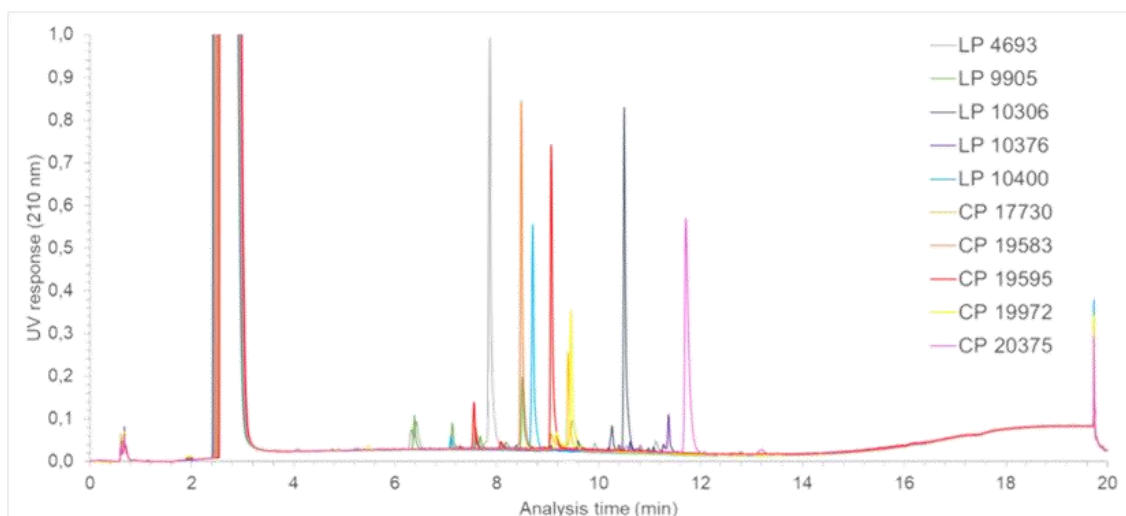
Figure S1. Superimposed chromatograms for the ten selected peptides in Table 1 in the 9 chromatographic systems compared with Derringer functions in Figure 4. UV detection (210 nm).
