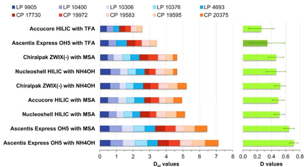
Fig. 4. Derringer desirability functions obtained for the ten individual peptides ( D_{pi} ) in each chromatographic system assessed, and the average D values with standard deviation. Linear peptides are indicated in blue colors, cyclic peptides in orange-red colors. (For interpretation of the references to color in this figure legend, the reader is referred to the web version of this article.)
