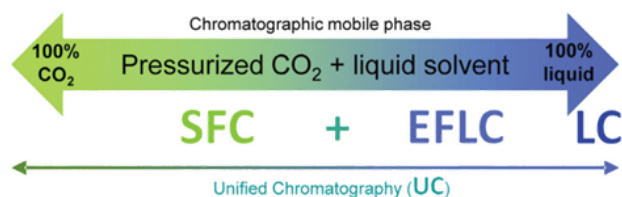
Fig. 4. Usual operating domains of SFC, EFLC and LC. Unified chromatography (UC) operates with large elution gradients covering a wide range of mobile phase compositions.
