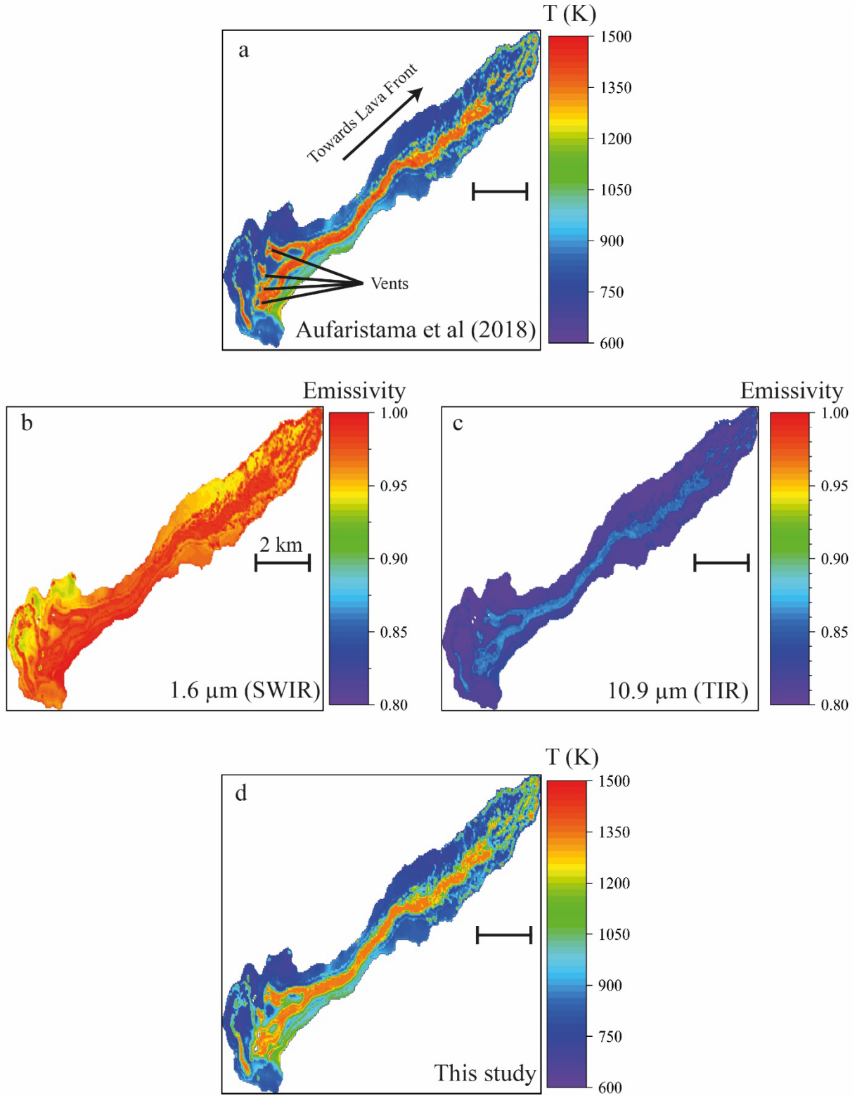
Figure 5-2: Results from Aufaristama and the refined models for thermal distribution of Holuhraun lava flow. a) Thermal maps obtained with Aufaristama model (constant \epsilon ). b,c) Emissivity maps obtained in the refined model –based on laboratory data for 1.6 \mu\text{m} SWIR and 10.9 \mu\text{m} TIR bands, respectively.
