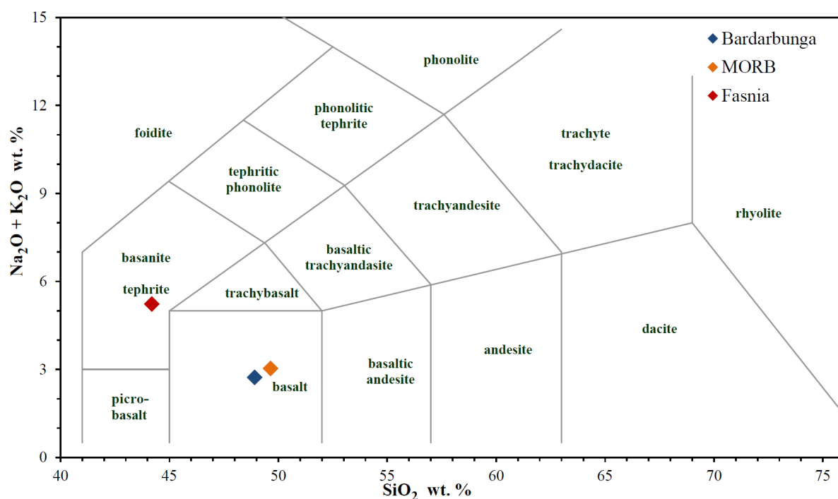
Figure 3-1: TAS diagram with basaltic compositions sensu lato studied in this work (from Bas et al. 1986).
