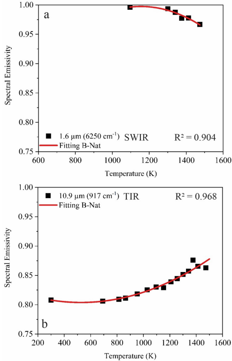
Figure 5-1: Temperature evolution of spectral Emissivity values for B-Nat in SWIR band 1.6 \mu\text{m} (a) and TIR band 10.9 \mu\text{m} (b) that allows deriving equations for \varepsilon -T relationship. Note that the sample must first reach high temperature before emitting in SWIR, thus explaining the limited number of data compared to TIR.
