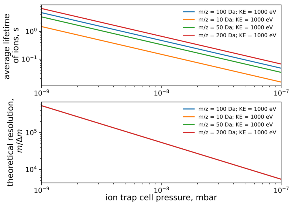
Figure C-3. Theoretical estimation of the life-time for ions in the QLEIT and theoretically achievable mass resolution at different residual gas pressure inside the trap for ions with Integral ion-molecule collision cross-section equal to 10^{-15} cm 2 . Maximal theoretical mass resolution limited by the ion scattering processes is not mass dependent.
