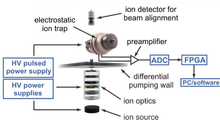
Figure C-2. Scheme of OLYMPIA setup components.
