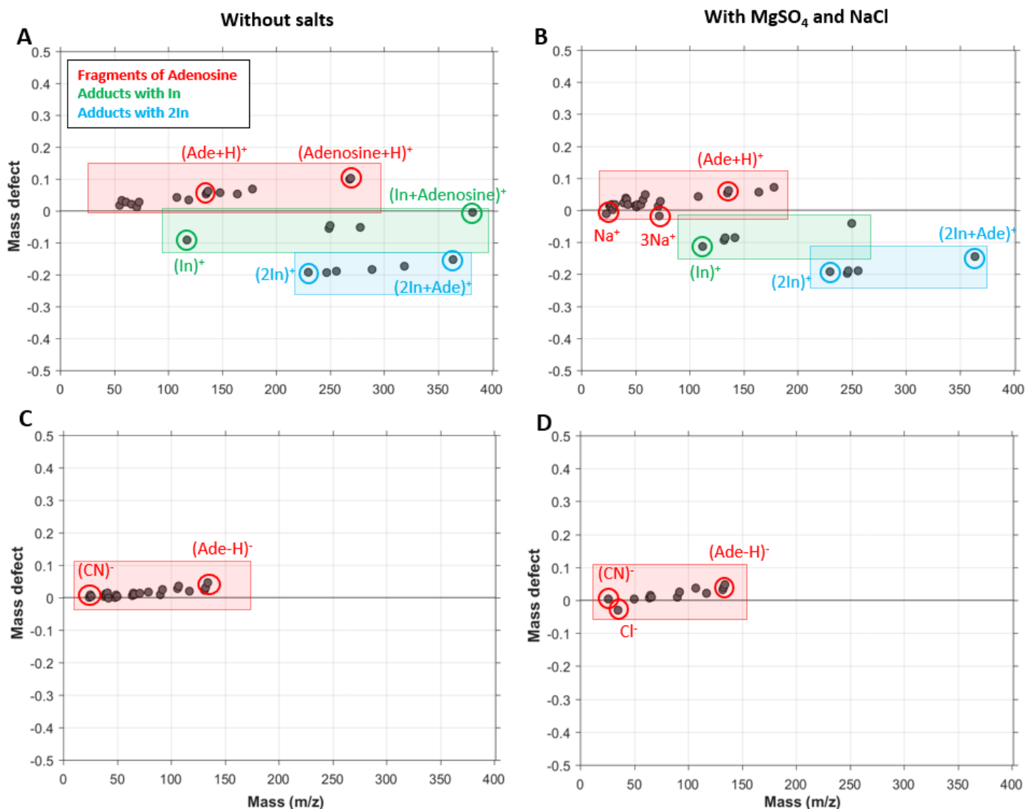
Figure B-7 : Mass defect of detected peaks versus m/z in Adenosine and Adenosine+MgSO 4 +NaCl samples. FFT has been applied on the signals between 100 and 838 ms. Panels A and B correspond to single laser shot positive ion mode experiments with the LAB-CosmOrbitrap prototype; panels C and D to the same experiments in negative ion mode. Panels A and C correspond to the pure Adenosine sample; panels B and D to the Adenosine+MgSO 4 +NaCl sample. For each panel, characteristic peaks such as the pseudomolecular one, the [Ade+H] + one, adducts with In, Na + , Cl - and CN - have been highlighted, as well as groups corresponding to different adduct types.
