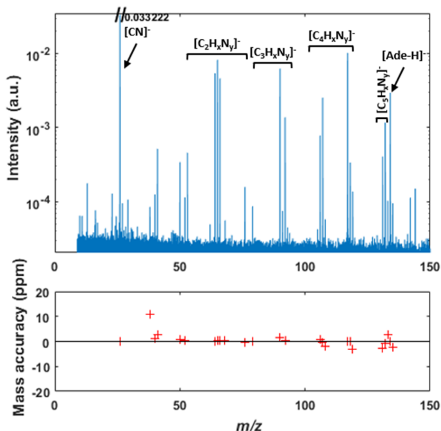
Figure B-5 : Lab-CosmOrbitrap Adenine spectrum with FFT applied on the signal between 25 and 325 ms. Top panel: single laser shot negative mass spectrum of Adenine calibrated on \text{CN}^- and [\text{Ade-H}]^- peaks. Bottom panel: mass accuracy of the identified (\text{C}_a\text{H}_b\text{N}_y\text{O}_\delta + \text{In}_\epsilon)^- molecules corresponding to peaks from the spectrum.
