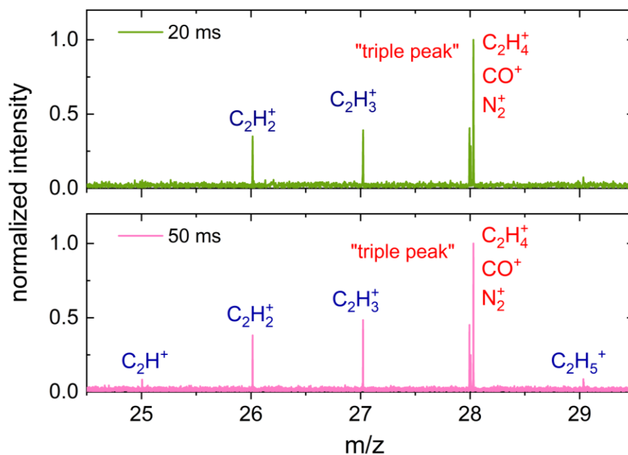
Figure C-4. Measured EI ionization mass spectrum of N_2:CO:C_2H_4 gas mixture with ratio 1:1:1. Ionization cell pressure is estimated as 1 mbar.
