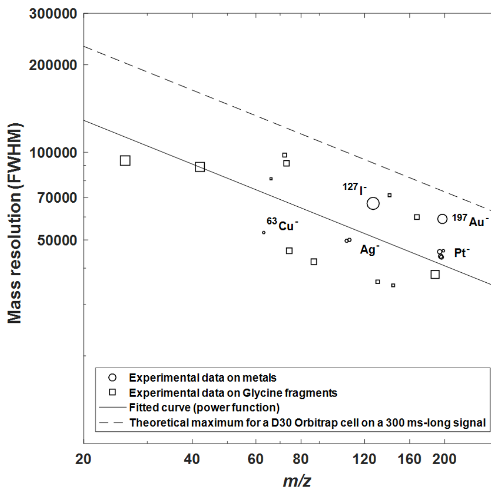
Figure B-3 : Mass resolving powers of the LAb-CosmOrbitrap as a function of m/z . The data from single laser shots have been generated by a FT of the transient recorded for 300 ms and a sampling rate of 5 MHz. The circles represent metallic samples. The squares represent TriGlycine sample pseudo-molecular peak ( m/z = 188.0747 ) and its detected fragments. The size of the two types of points is proportional to the signal-to-noise ratio of the corresponding peaks. Solid black curve is a fit taken from the data presented here, according to the power function y = a * x^m . Black dash curve shows the maximum resolution for an emitted spectrum of a 300ms-long signal sampled at 5 MHz.
