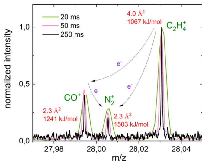
Figure C-5. Mass spectra of the N_2/CO/C_2H_4 triplet peak measured with varied acquisition time.
