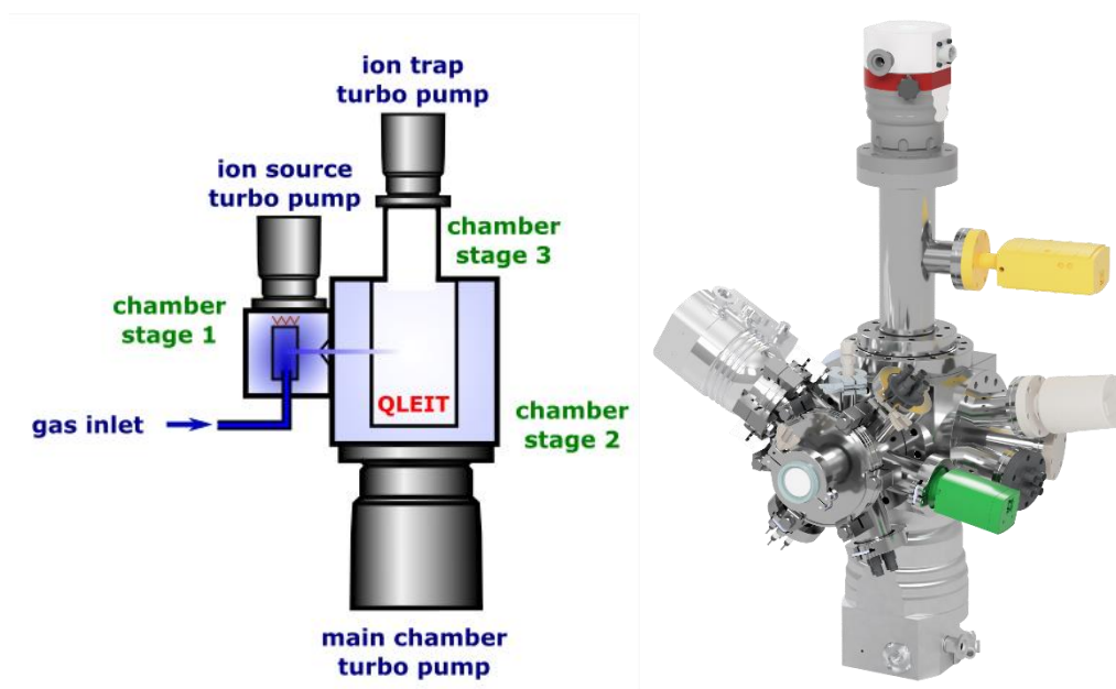
Figure C-1. Scheme of the OLYMPIA instrument: a) principal components of the vacuum system; b) arrangement of the vacuum system made of Pfeiffer Vacuum, Edwards Vacuum and Hositrad Vacuum Technologies COTS components.
