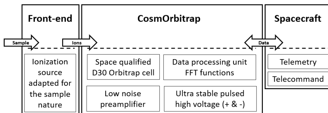
Figure B-1 : Diagram of the components of a CosmOrbitrap-based instrument.
