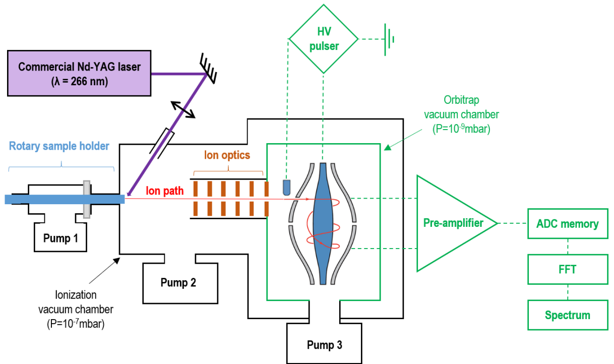
Figure B-2 : Scheme of the LAb-CosmOrbitrap instrument. Green parts are CosmOrbitrap elements under development, other parts are commercial elements.
