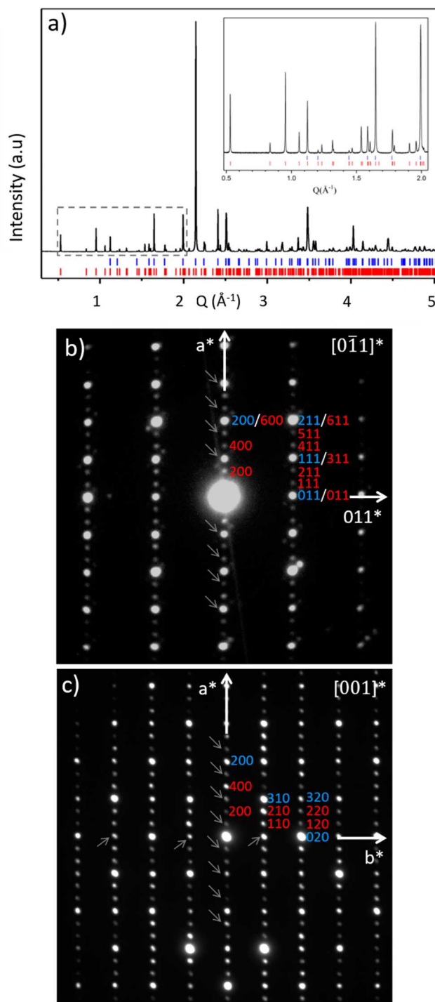
Figure 1. (a) Synchrotron powder diffraction data of the SrYbGa_3O_7 melilite phase indexed with the P4_2/m melilite substructure (blue marks) and in the 3 \times 1 \times 1 P2_12_12 superstructure (red marks). (b) [0-11]^* and [001]^* Selected Area Electron Diffraction patterns of the SrTmGa_3O_7 melilite phase synthesized by full crystallization from glass. The indexations of the tetragonal melilite substructure ( a = 7.9 Å \times c = 5.2 Å, P4_2/m ) and the 3 \times 1 \times 1 superstructure ( a = 23.7 Å \times b = 7.9 Å \times c = 5.2 Å, P2_12_12 ) are shown in blue and red, respectively. The arrows point to the reflections assigned to double diffraction.
