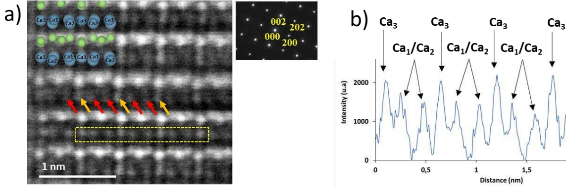
Figure V.12. a) High resolution STEM-HAADF image of \text{La}_{0.25}\text{Ca}_{4.75}\text{Ga}_6\text{O}_{14} ( x = 0.25 ) sample oriented along the [010] (see Figure V.13b for its related crystal structure projection). The crystal related SAED is shown on the top right insert while the top left insert shows an overlay of the structure. Orange and red arrows indicate the \text{Ca}_3 and \text{Ca}_1/\text{Ca}_2 sites. b) the drawn Z profile from the integrated area highlighted by yellow rectangle in (a).
