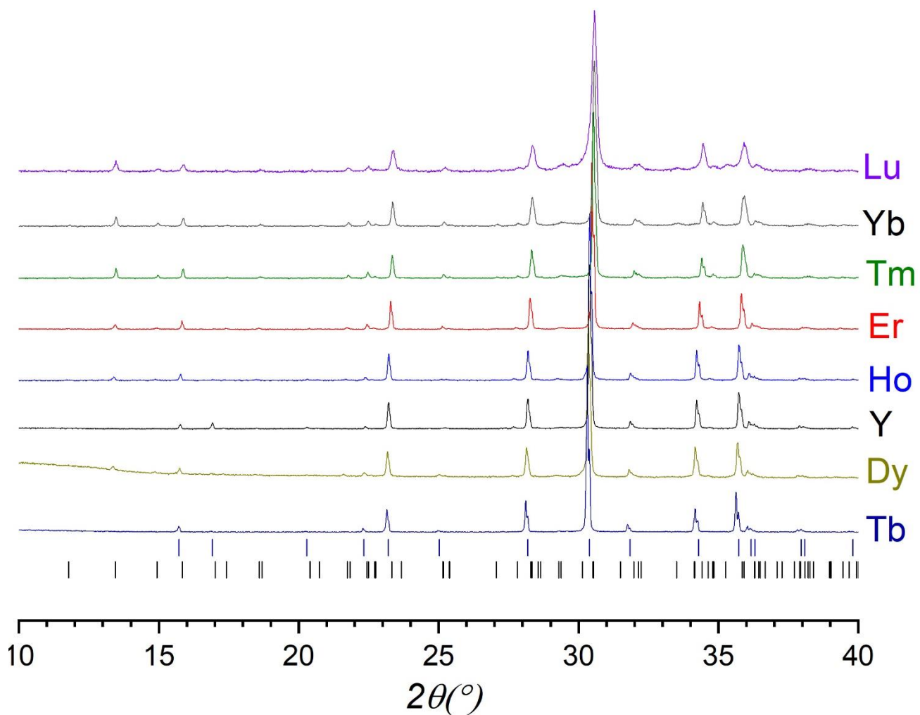
Figure S5. Post-DSC PXRD data of \text{SrREGa}_3\text{O}_7 , where black and dark blue tick marks correspond to the P2_12_12 3 \times 1 \times 1 ordered superstructure (exhibited by RE = \text{Dy} - \text{Lu}, \text{Y} ) and the P-42_1m disordered structure (exhibited by \text{SrTbGa}_3\text{O}_7 only) respectively.
