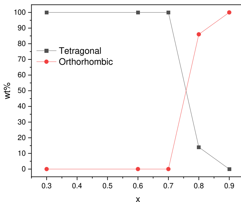
Figure IV.13. Refined wt% of both tetragonal and orthorhombic melilite polymorphs from neutron data as a function of substituted Ba by La, noted x from the \text{La}_{1+x}\text{Ba}_{1-x}\text{Ga}_3\text{O}_{7+x/2} solid solution.
