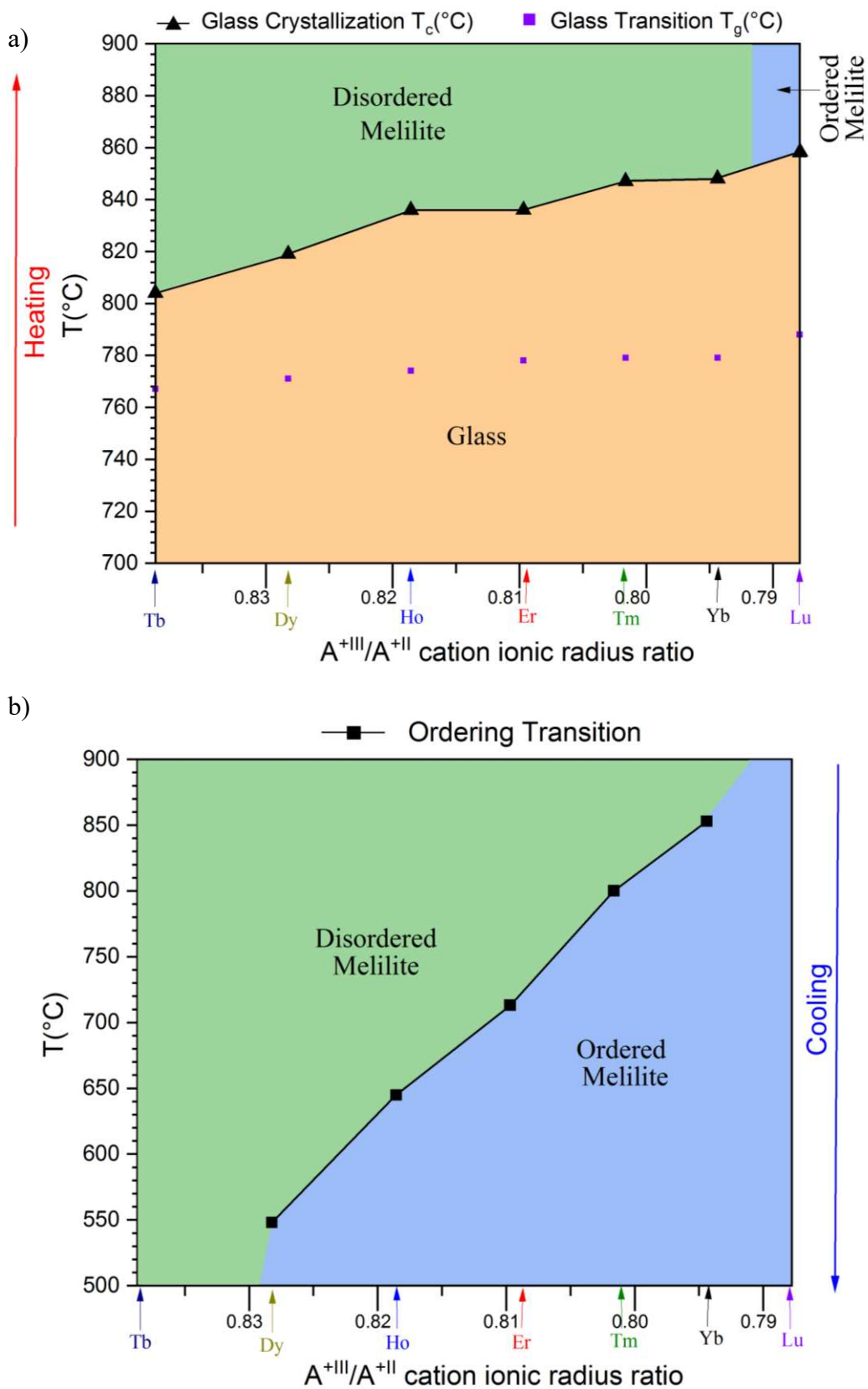
Figure S6. Glass, ordered and disordered melilite \text{SrREGa}_3\text{O}_7 ( \text{RE} = \text{Tb} - \text{Lu}, \text{Y} ) domains of stability on (a) heating and (b) cooling at rates of 10^{\circ}\text{C min}^{-1} , drawn from DSC results (Figure 7, main manuscript) and PXRD measurements performed post-DSC (Figure S5).
