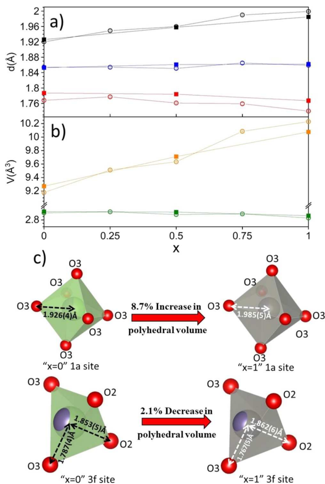
Figure 10. Refined M\text{--}O distances from SPD and NPD (hollow circles and filled squares, respectively) for compositions 0 \leq x \leq 1 . (a) B–O3 (black), C–O2 (blue), and C–O3 (red) distances and (b) their corresponding polyhedral volumes \text{BO}_6 (1a, orange) and \text{CO}_4 (3f, green). (c) Cationic 1a and 3f site coordination and their nearby interatomic distances for both x = 0 and x = 1 compounds from NPD refinements.
