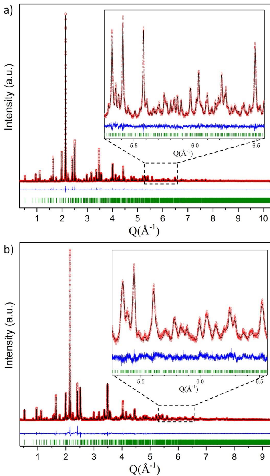
Figure S11. Rietveld refinement of a) \text{SrHoGa}_3\text{O}_7 ( R_p = 4.85\% , R_{wp} = 6.30\% ) and b) \text{SrLuGa}_3\text{O}_7 ( R_p = 6.87\% , R_{wp} = 9.18\% ) ordered melilites (SPD data). Observed (black dot), calculated (red line), and difference (blue line) profiles are shown. The set of green vertical lines corresponds to reflection positions.
