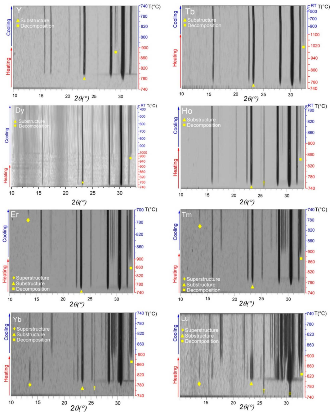
Figure 6. Variable temperature powder X-ray diffraction (VT-PXRD) on \text{SrREGa}_3\text{O}_7 ( \text{RE} = \text{Tb}–\text{Lu}, \text{Y} ) on heating and cooling, starting from the precursor glasses. Peaks representing the initial melilite (substructure) crystallization, the 3 \times 1 \times 1 structural ordering (superstructure), and the onset of decomposition are indicated, respectively, by triangle, diamond, and square symbols. Note that the maximum intensities of the decomposition peaks are between 1 and 3% (Tb, Dy, Ho, Er, Y) or 5 and 8% (Tm, Yb) of the most-intense melilite peak, while Lu decomposed substantially ( \sim 50\% ). Peaks labeled \dagger arise from the alumina sample holder. The precursor glass for \text{RE} = \text{Lu} contained a small amount of crystallized melilite, indicated by \ddagger .
