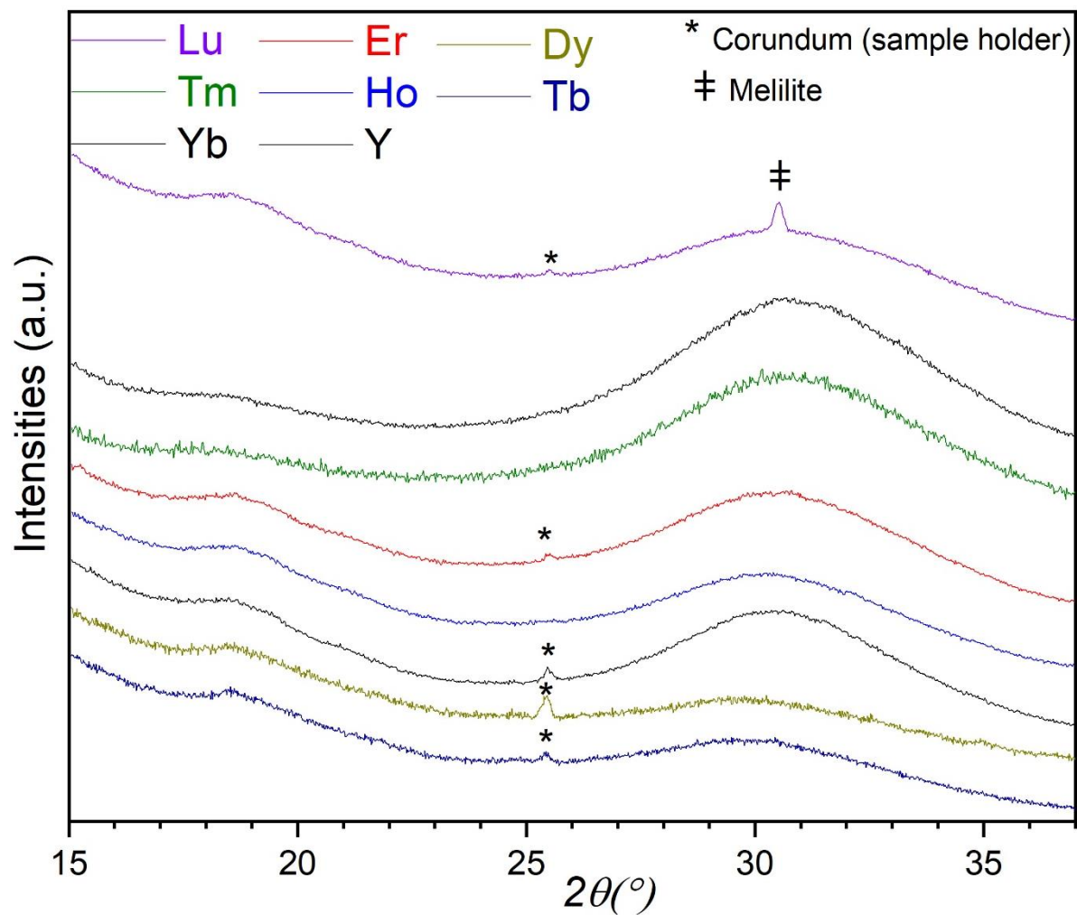
Figure S1. Laboratory X-ray powder diffraction data of \text{SrREGa}_3\text{O}_7 ( \text{RE} = \text{Tb-Lu, Y} ) glass samples synthesized by aerodynamic levitation coupled to laser heating (ADL).
