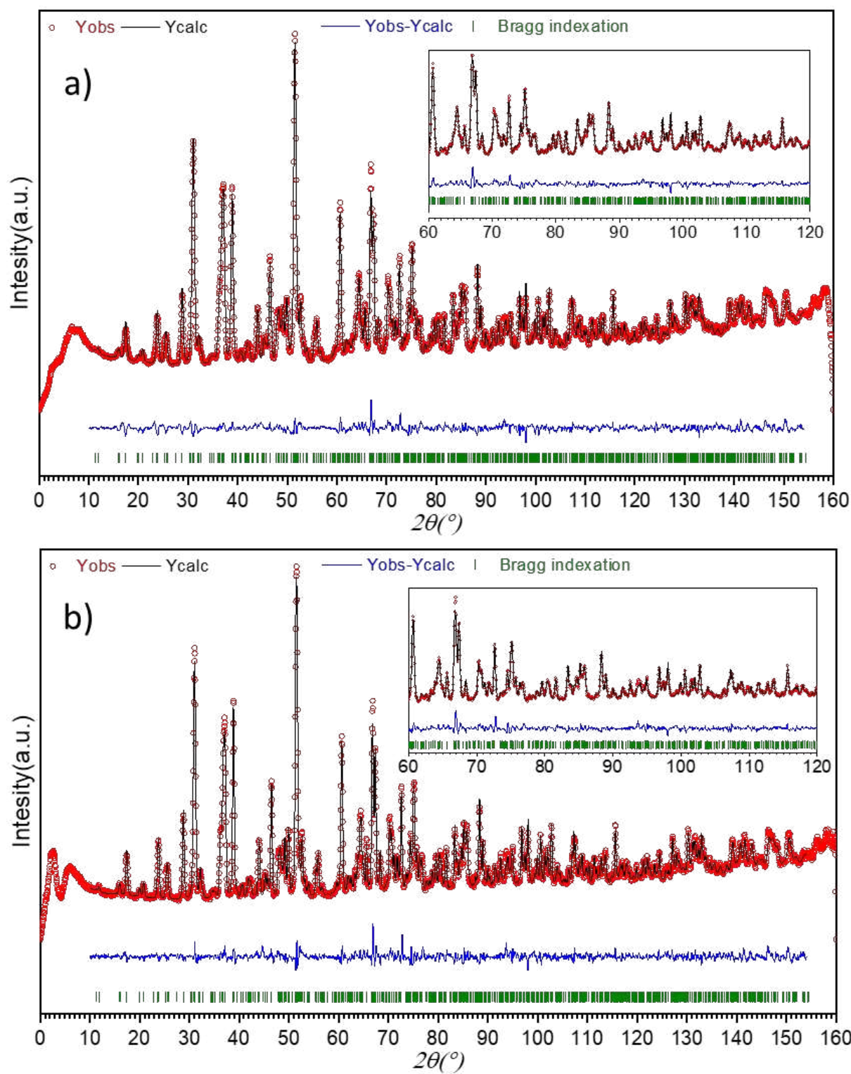
Figure A. 29. 525°C NPD (a) HI, (b) HR data Rietveld refinement of the \text{La}_{1.9}\text{Ba}_{0.1}\text{Ga}_3\text{O}_{7.45} ( x = 0.9 ) composition.
