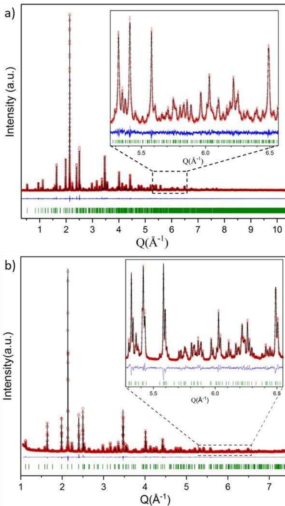
Figure A. 13. Rietveld refinement of a) \text{SrHoGa}_3\text{O}_7 ordered melilite (SPD data, R_p = 4.85\% R_{wp} = 6.30\% ) and b) \text{SrHoGa}_3\text{O}_7 disordered melilite (lab data, R_p = 1.41\% R_{wp} = 2.08\% ). Observed (black dot), calculated (red line), and difference (blue line) profiles are shown. The set of green vertical lines corresponds to reflection positions.
