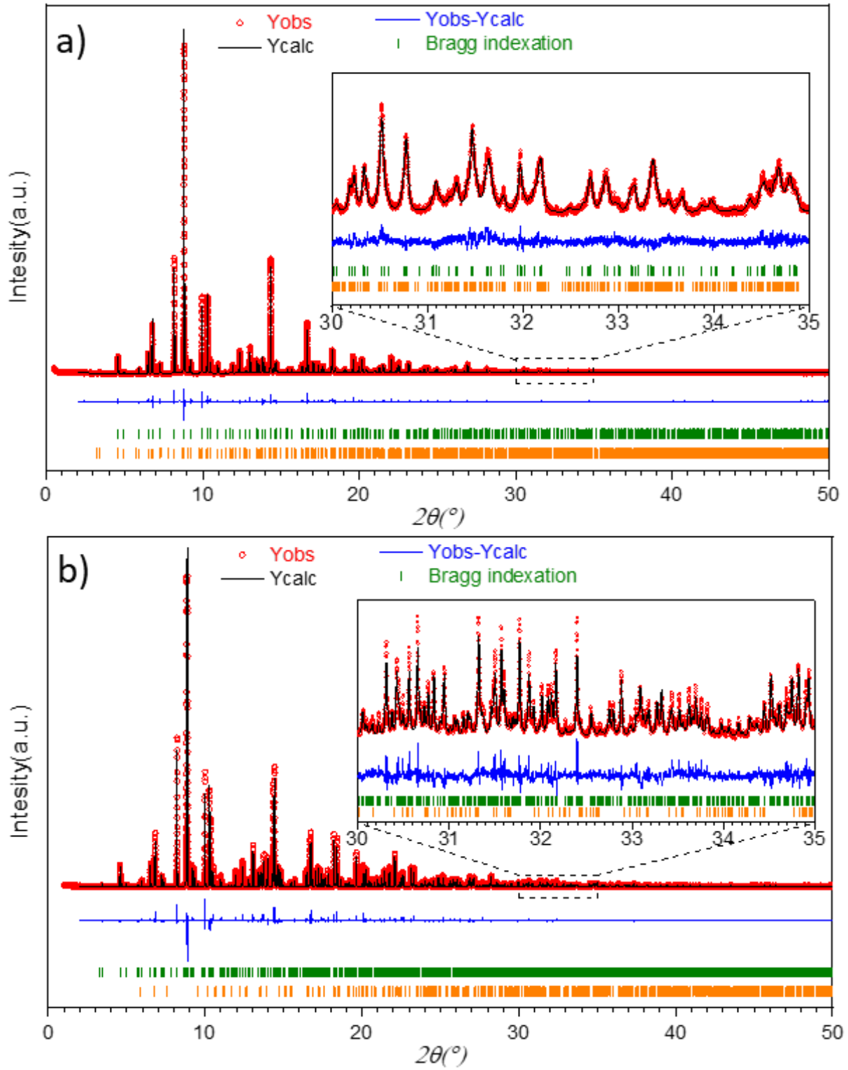
Figure IV.9. SPD data Rietveld refinement of the a) \text{La}_{1.75}\text{Ba}_{0.25}\text{Ga}_3\text{O}_{7.375} ( x = 0.75 ) composition ( R_{wp} = 9.11\% , \text{GOF} = 1.51 ). b) \text{La}_{1.9}\text{Ba}_{0.1}\text{Ga}_3\text{O}_{7.45} ( x = 0.9 ) composition ( R_{wp} = 13.21\% , \text{GOF} = 1.96 ). In both panels red, black and blue data corresponds to the measured, calculated and difference curves. In the (a) panel green and orange tick marks corresponds to the P4_21m and \text{Ima}2 melilites. Where in panel (b) green and orange tick marks corresponds to \text{Ima}2 melilite and \text{LaGaO}_3 perovskite.
