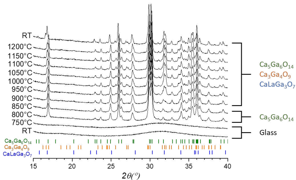
Figure V.6. VT-PXRD measurements of \text{La}_{0.3}\text{Ca}_{4.7}\text{Ga}_6\text{O}_{14.15} ( x = 0.3 ) glass compounds between 750°C and 1200°C. The different crystallised phases are indicated by green, orange and blue tick marks, corresponding to the \text{Ca}_5\text{Ga}_6\text{O}_{14} , \text{Ca}_3\text{Ga}_4\text{O}_9 and \text{CaLaGa}_3\text{O}_7 compounds respectively.
