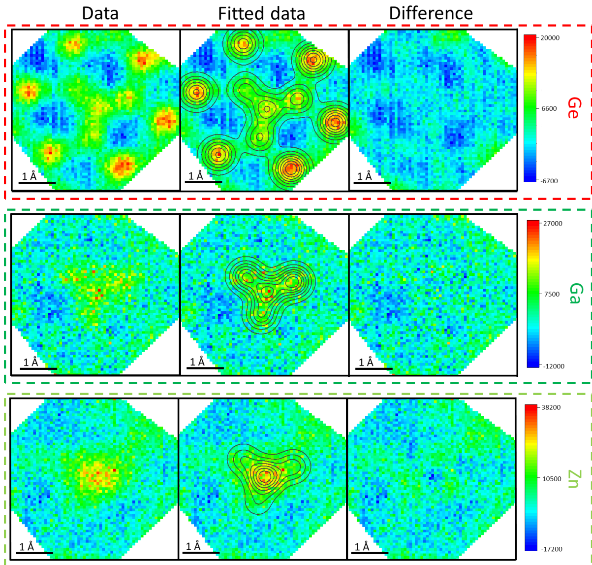
Figure III.23. STEM-EDS 2D refinement plots of Ge, Ga and Zn from zone1, where the left column represents the data (after processing), middle column fitted data (fit in black contours) and the difference plots in the right column.
