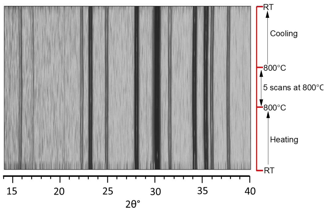
Figure IV.23. VT-PXRD between RT and 800°C measurements of the \text{La}_{1.6}\text{Ba}_{0.4}\text{Ga}_3\text{O}_{7.3} compound, using a step of 50°C/scan in the range of 14°-40°C ( 2\theta ) with a step of 0.016° and a measuring time of 1s/step. All measured diffraction patterns were indexed with the P\bar{4}2_1m melilite cell.
