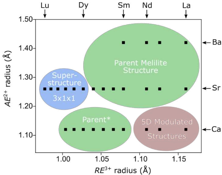
Figure II.17. Phase diagram indicating the different structural orderings reported for the (\text{AE}, \text{RE})\text{Ga}_3\text{O}_7 melilite family, according to the ionic radii of their A site cations. The parent structure and 5D-modulated structure regions have been compiled from the literature [16], [27], [28]. Note that the parent structure region for \text{AE} = \text{Ca} is marked with an asterisk, as it was reported prior to the discovery of structural modulation in \text{CaLaGa}_3\text{O}_7 and \text{CaNdGa}_3\text{O}_7 .
