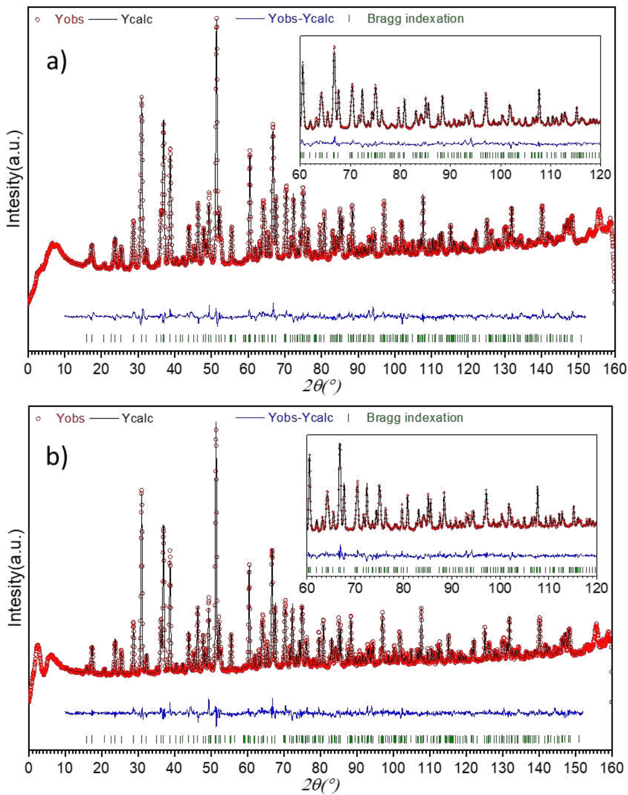
Figure A. 32. 820°C NPD (a) HI, (b) HR data Rietveld refinement of the \text{La}_{1.9}\text{Ba}_{0.1}\text{Ga}_3\text{O}_{7.45} ( x = 0.9 ) composition.
