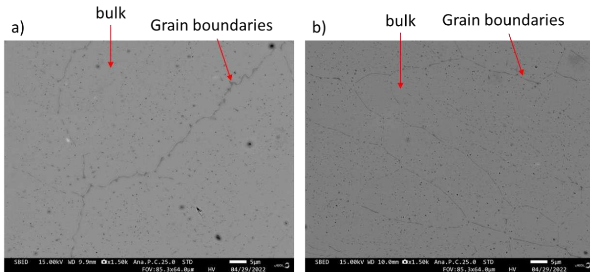
Figure IV.24. SEM measurements on a) as-synthesised bead b) heat treated bead (replicating the AS-impedance measurement thermal protocol), in back scattered electron mode on beads of \text{La}_{1.6}\text{Ba}_{0.4}\text{Ga}_3\text{O}_{7.3} composition. Both images are shown at the same enlargement scale.
