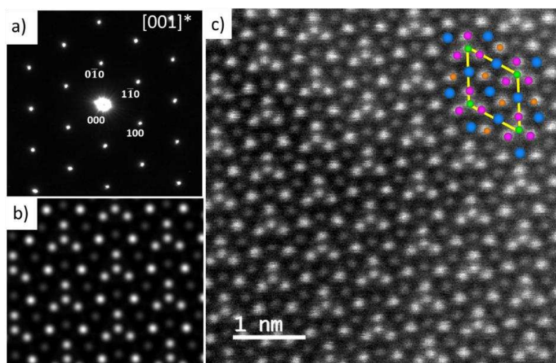
Figure III.19. a) Selected area electron diffraction (SAED) pattern of the \text{Ca}_3\text{GaZn}_{0.5}\text{Ge}_{4.5}\text{O}_{14} ( x = 0.5 ) sample oriented along the [001]^* direction, with b) and c) showing simulated (using JEMS software) [53] and measured STEM-HAADF images respectively. The corresponding crystal structure projection is overlaid on the top-right corner of the image, where blue, green, pink and orange points represent the 3e, 1a, 3f and 2d crystallographic sites respectively.
