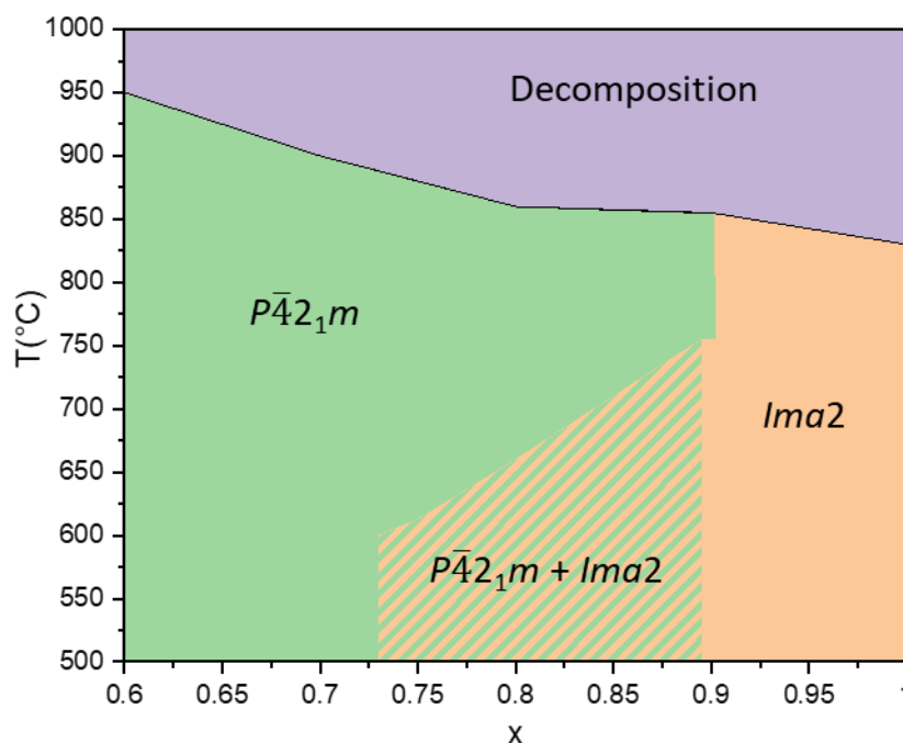
Figure IV.20. Phase-diagram like plot of the \text{La}_{1+x}\text{Ba}_{1-x}\text{Ga}_3\text{O}_{7+x/2} solid solution studied compositions, evidencing the polymorphs stability limits against x “amount of substituted barium” and temperature drawn from VT-PXRD measurement. The transition temperatures from the mixed P\bar{4}2_1m + Ima2 to fully P\bar{4}2_1m in the 0.725 < x < 0.8 region were extrapolated from the measured x = 0.8 and 0.9 compositions. The x = 1 compound decomposition temperature was taken from [11].
