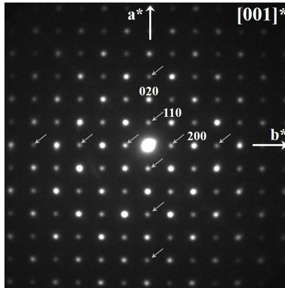
Figure II.13. [001]^* Selected Area Electron Diffraction (SAED) pattern of the SrTmGa_3O_7 parent melilite synthesised by full crystallisation from glass, with the indexing of its tetragonal structure ( a=7.9 \text{ \AA} , c=5.2 \text{ \AA} , P\bar{4}2_1m ). Evidencing a total absence of satellite peaks. The arrows point the reflections assigned to double diffraction.
