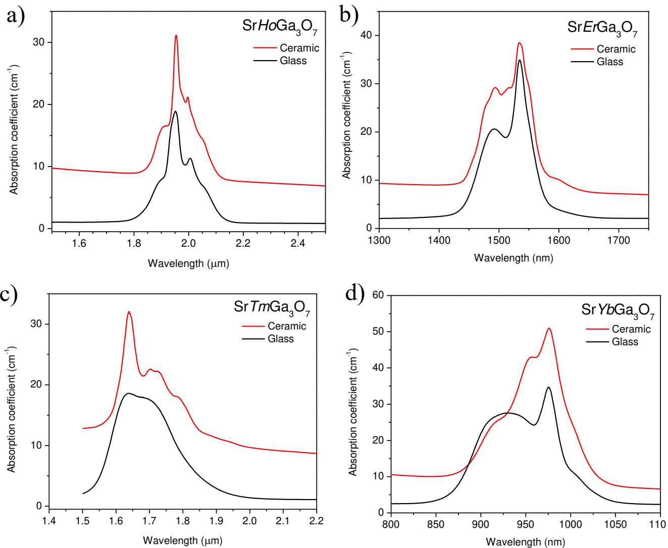
Figure S16. Absorption coefficient spectra of the SrHoGa 3 O 7 (a), SrErGa 3 O 7 (b), SrTmGa 3 O 7 (c), and SrYbGa 3 O 7 (d) glass and ceramic melilites. Data were not corrected with respect to Fresnel optical losses; the increase of background absorption observed in the ceramics' spectra is due to scattering losses (see Figure S15).
