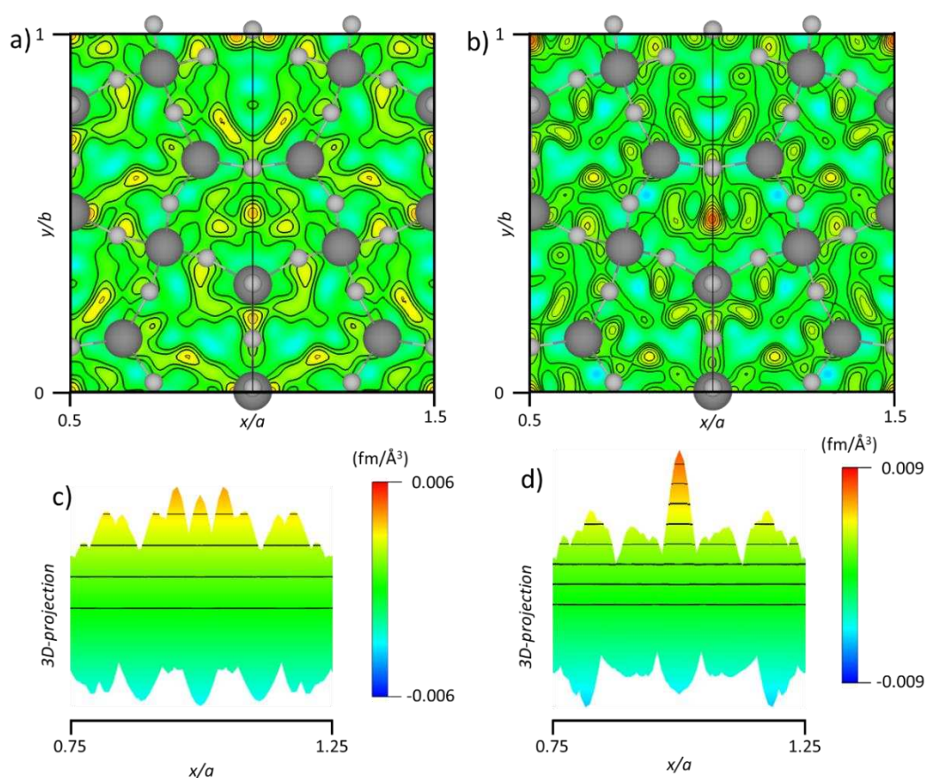
Figure A. 35. a) and b) Fourier difference map section at z=0.51 centered at the Ca3 channels from \text{La}_{0.25}\text{Ca}_{4.75}\text{Ga}_6\text{O}_{14.125} NPD (HR) and NPD (HI) refined data respectively. One [\text{GaO}_4]_n sheet is overlaid in both a) and b) panels with dark grey and light grey spheres corresponding to Ga and O atoms. c) and d), 3D-projection of the Fourier difference maps shown in a) and b) respectively.
