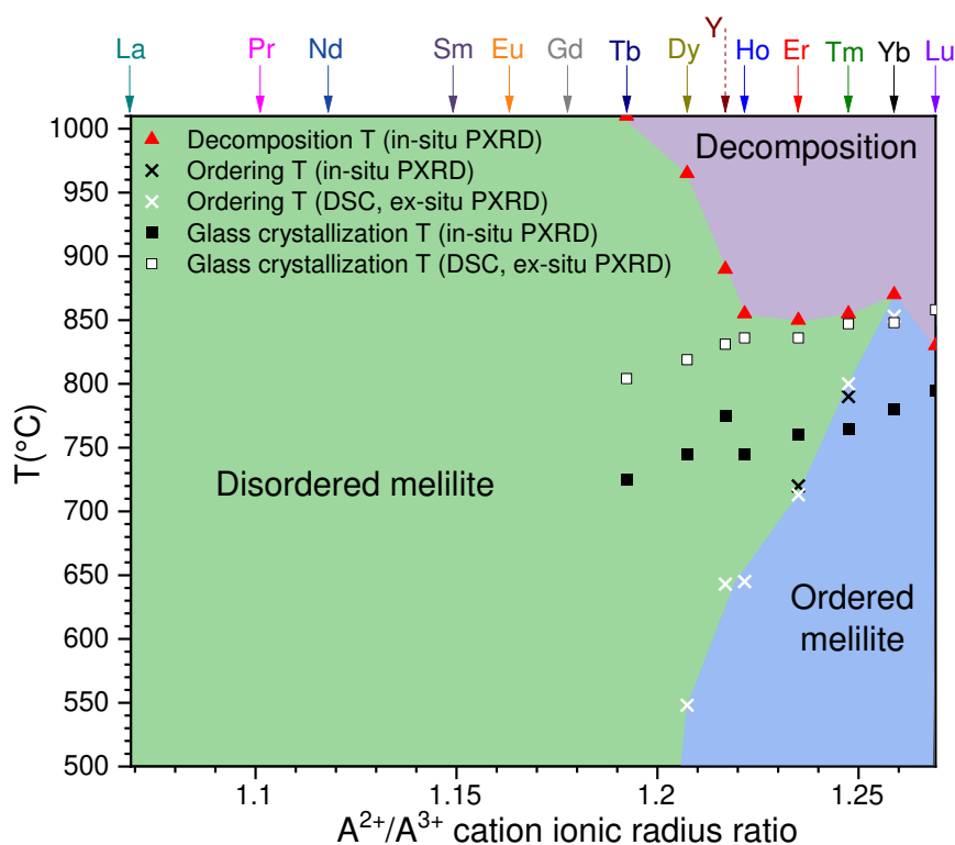
Figure II.8. \text{SrREGa}_3\text{O}_7 ( \text{RE} = \text{Tb} - \text{Lu} ) melilites stability diagram drawn from DSC and VT-PXRD resumes, coupled to previous results from Jan Skakle et al [16] ( \text{RE} = \text{La} - \text{Gd} ). The ordering region was drawn according to the highest stability temperature of each compound from both DSC and VT-PXRD.
