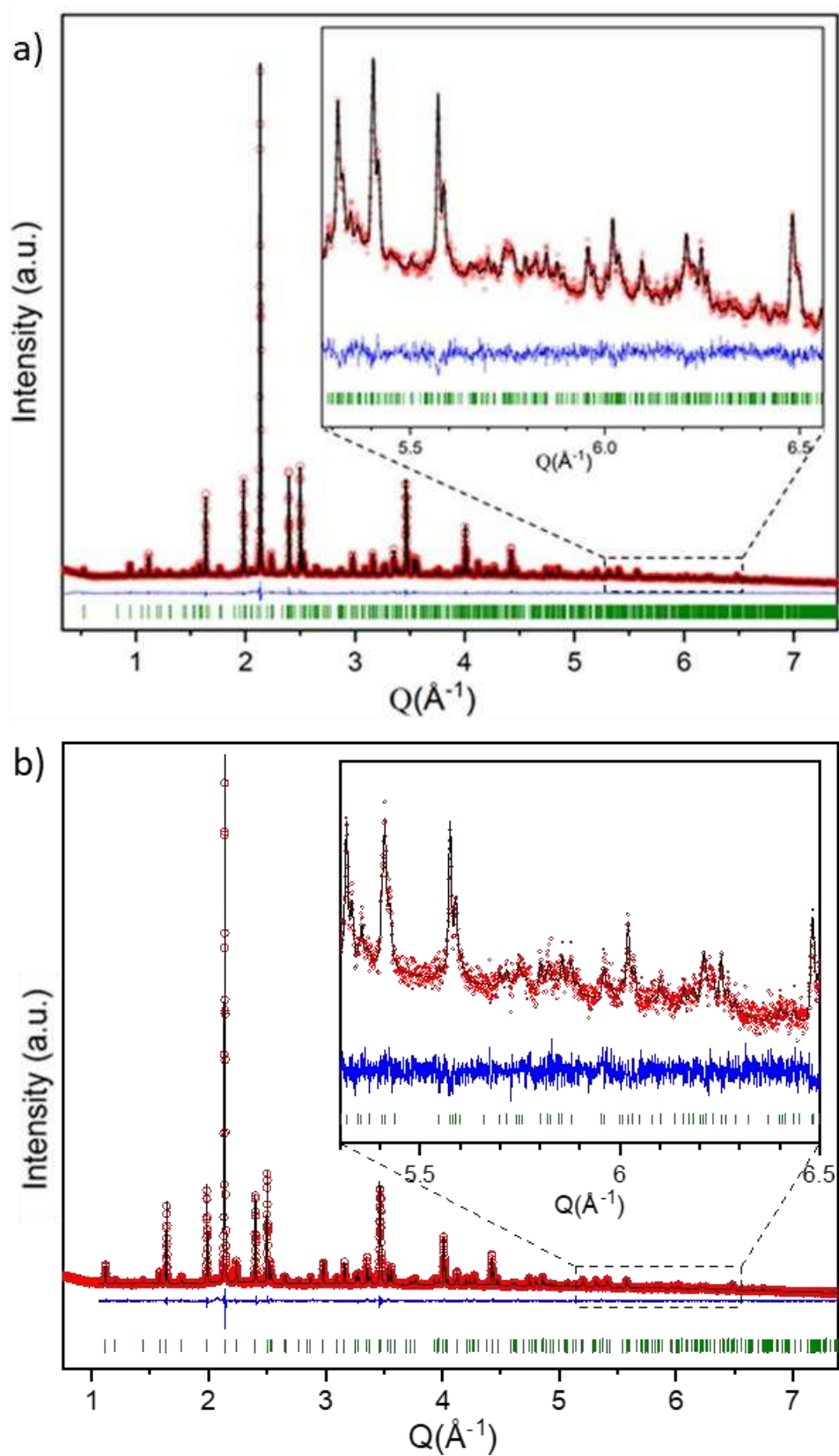
Figure A. 14. Rietveld refinement of a) \text{SrDyGa}_3\text{O}_7 ordered melilite (lab data, R_p = 1.66\% R_{wp} = 2.21\% ) and b) \text{SrDyGa}_3\text{O}_7 disordered melilite (lab data, R_p = 2.62\% R_{wp} = 3.35\% ). Observed (black dot), calculated (red line), and difference (blue line) profiles are shown. The set of green vertical lines corresponds to reflection positions.
