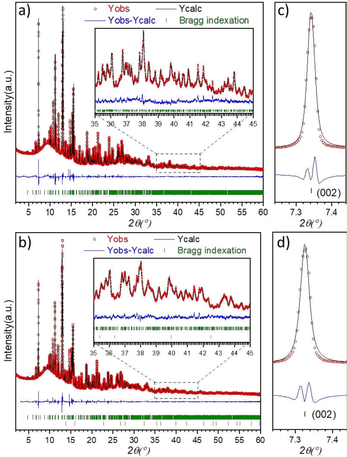
Figure V.9. Final Rietveld refined SPD data of a) \text{Ca}_5\text{Ga}_6\text{O}_{14} ( x = 0 ) ( R_{wp} = 2.06\% GOF = 3.23 ), and b) \text{La}_{0.25}\text{Ca}_{4.75}\text{Ga}_6\text{O}_{14.125} ( x = 0.25 ) ( R_{wp} = 1.67\% GOF = 2.63 ). c) and d) shows a zoom on the (002) peak which exhibits the first biggest misfit.
