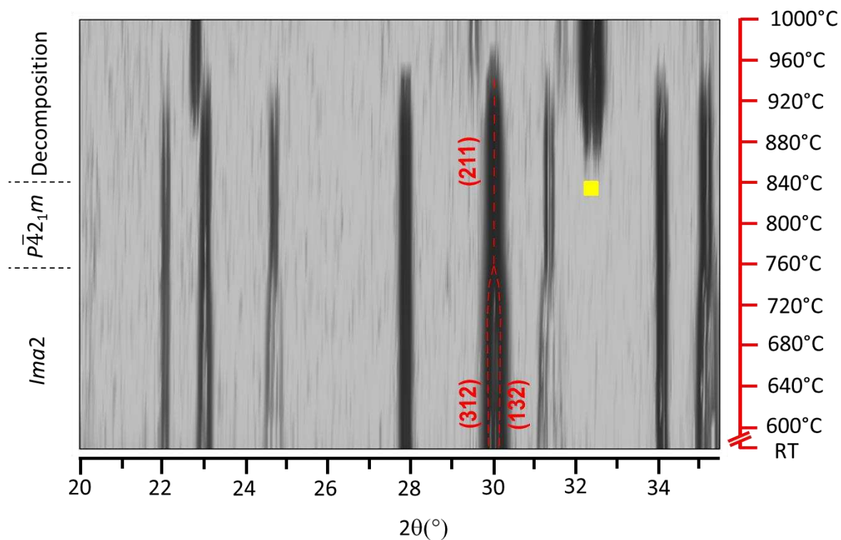
Figure IV.18. VT-PXRD measurements ( 20^{\circ}\text{C} step size) of \text{La}_{1.9}\text{Ba}_{0.1}\text{Ga}_3\text{O}_{7.45} ( x=0.9 ) composition, evidencing the stability of the orthorhombic Ima2 melilite vs temperature. The yellow box shows the beginning of decomposition into \text{LaGaO}_3 + \text{LaBaGa}_{11}\text{O}_{20} + \text{Ga}_2\text{O}_3 .
