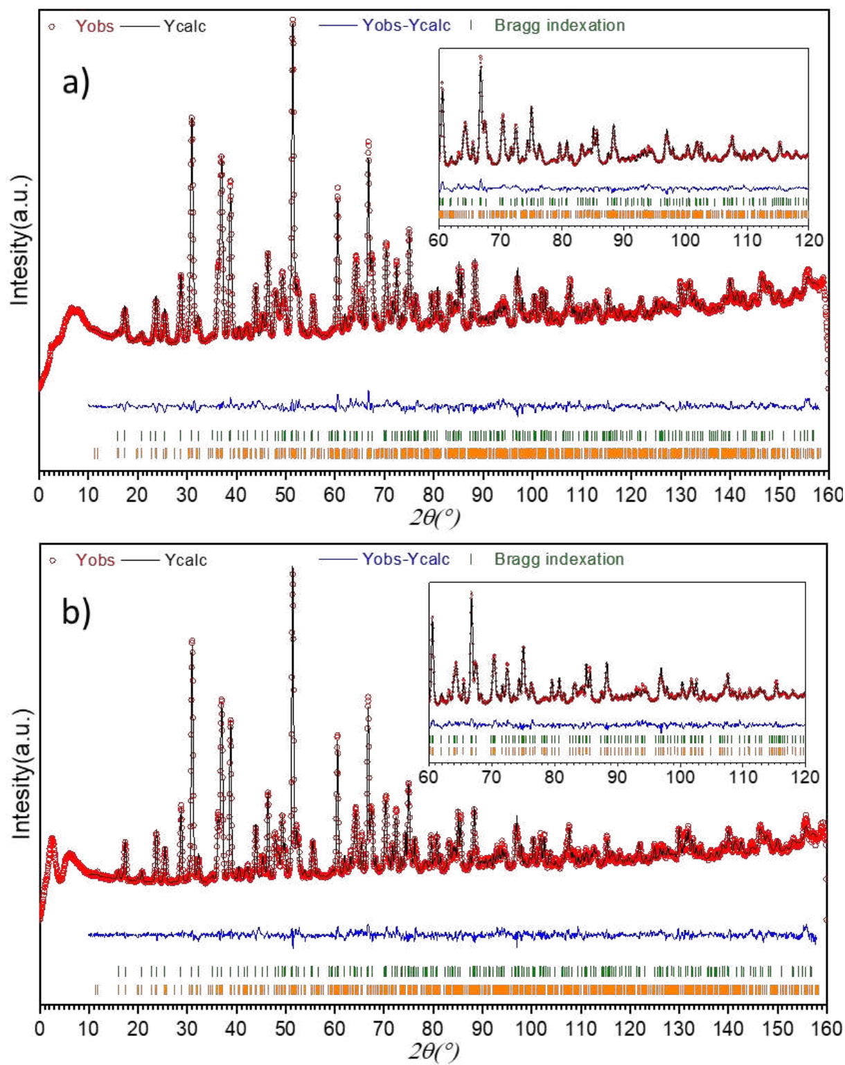
Figure A. 31. 770°C NPD (a) HI, (b) HR data Rietveld refinement of the \text{La}_{1.9}\text{Ba}_{0.1}\text{Ga}_3\text{O}_{7.45} ( x = 0.9 ) composition.
