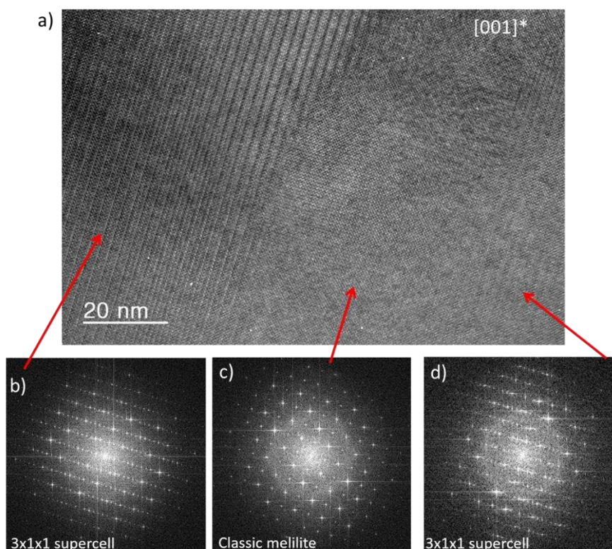
Figure II.11. a) [001]^* HRTEM image and b), c), d) associated FFTs of the SrYGa_3O_7 melilite parent synthesised by full crystallization from glass showing the coexistence of both cation-ordered and cation-disordered domains.
