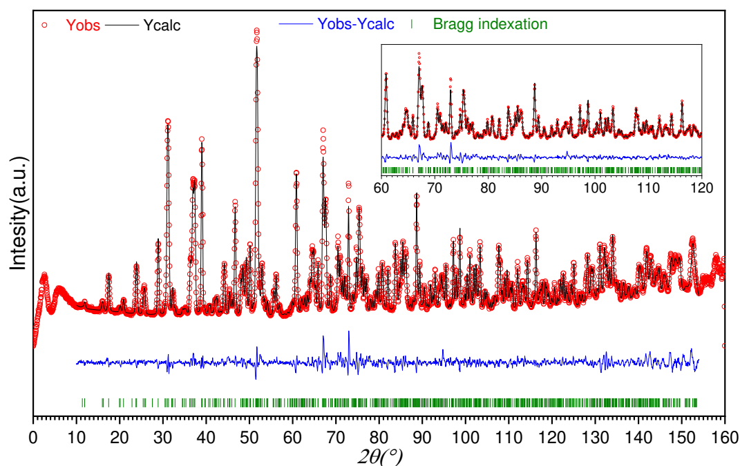
Figure IV.12. Room temperature NPD HR data Rietveld refinement of the \text{La}_{1.9}\text{Ba}_{0.1}\text{Ga}_3\text{O}_{7.45} ( x = 0.9 ) composition ( R_{\text{wp}} = 4.84\% , \text{GOF} = 2.02 ).
