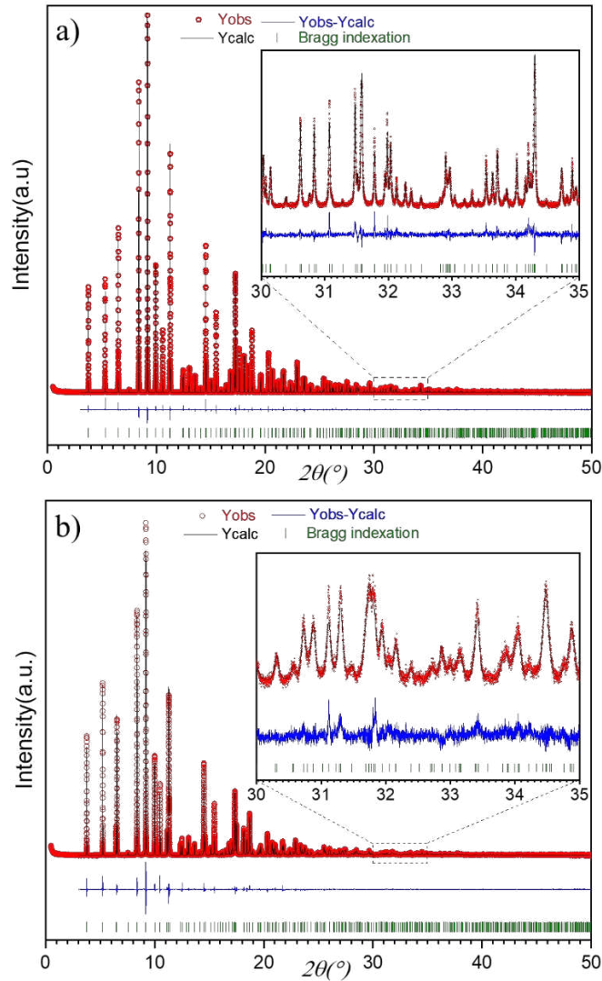
Figure III.12. Rietveld refinement of a) \text{Ca}_3\text{Ga}_2\text{Ge}_4\text{O}_{14} ( x = 0 ) (SPD data, R_p = 7.617\% R_{wp} = 9.506\% ) and b) \text{Ca}_3\text{ZnGe}_5\text{O}_{14} ( x = 1 ) (SPD data, modelled strain R_p = 7.02\% R_{wp} = 8.75\% ). Observed (red dot), calculated (black line), and difference (blue line) profiles are shown. The set of green vertical lines corresponds to reflection positions.
