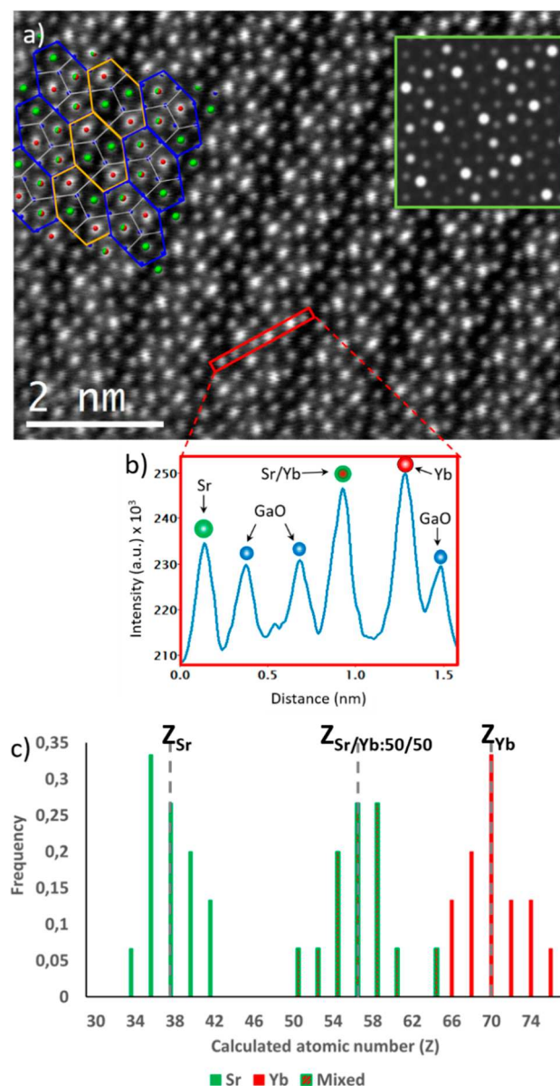
Figure 4. (a) Atomic scale STEM-HAADF micrograph of the \text{SrYbGa}_3\text{O}_7 superstructure sample oriented along the [001] zone axis. The hexagonal ABA' tiling, from the discussion in section 4.1, is overlaid to highlight the superstructure (Ga, Yb1/Sr1, Yb2, and Sr3 atoms are respectively represented in blue, red, green/red, and green). The green framed inset corresponds to a STEM-HAADF simulated image by JEMS software. (b) Experimental profile corresponding to the red framed box area. (c) Distribution of the calculated atomic number ( Z ) from the measured peak volumes for each crystallographic site (Yb1/Sr1, Yb2, and Sr3).
