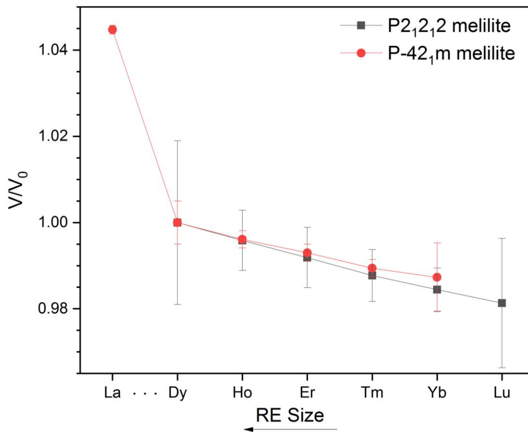
Figure S14. Evolution of the unit cell volume across the \text{SrREGa}_3\text{O}_7 ( \text{RE} = \text{Dy} - \text{Lu} ) series. \text{RE} = \text{Dy} was chosen as V_0 . The cell volume for \text{SrLaGa}_3\text{O}_7 is added for comparison.
