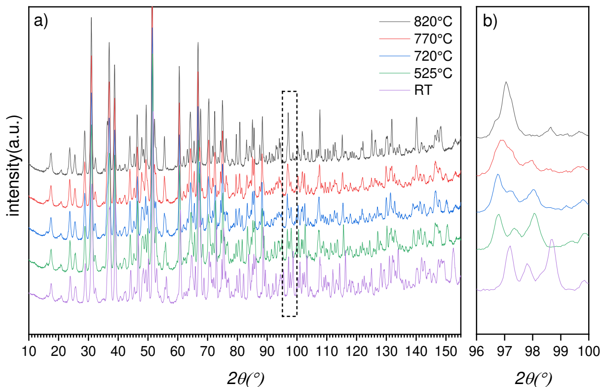
Figure IV.19. a) Stacked high temperature neutron powder diffraction patterns of the \text{La}_{1.9}\text{Ba}_{0.1}\text{Ga}_3\text{O}_{7.45} ( x=0.9 ) composition measurement. A zoom on the 96^{\circ} - 100^{\circ} ( 2\theta ) region is shown in (b) panel.
