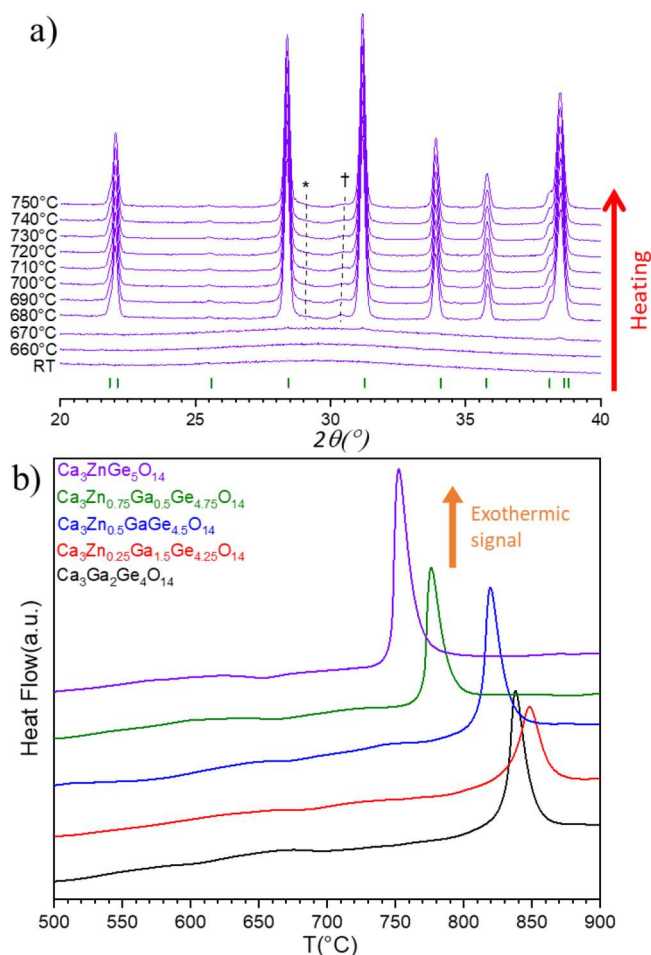
Figure 2. (a) Variable temperature PXRD measurements on the \text{Ca}_3\text{ZnGe}_5\text{O}_{14} x = 1 glass composition showing its crystallization upon heating (0.5 °C/min heating rates), where * and † represent the \text{CaZnGe}_2\text{O}_6 and \text{Ca}_2\text{ZnGe}_2\text{O}_7 impurities, respectively. Green tick marks represent the P321 \text{Ca}_3\text{ZnGe}_5\text{O}_{14} indexation. (b) DSC measurements of \text{Ca}_3\text{Ga}_{2-2x}\text{Zn}_x\text{Ge}_{4+x}\text{O}_{14} x = 0 (black), 0.25 (red), 0.5 (blue), 0.75 (green), and 1 (purple) samples, using a 10 °C/min rates upon heating.
