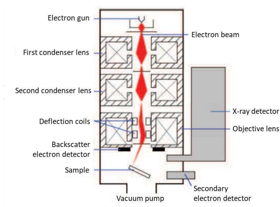
Figure A. 5. Scheme of an SEM components.
