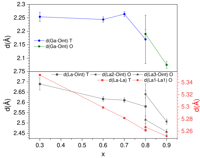
Figure IV.17. \text{Ga-O}_{\text{int}} , \text{La-O}_{\text{int}} and \text{La-La} interatomic distances obtained from neutron refined structures across the room temperature measured composition series ( x values in \text{La}_{1+x}\text{Ba}_{1-x}\text{Ga}_3\text{O}_{7+x/2} ). With T and O referring to tetragonal P\bar{4}2_1m and orthorhombic \text{Ima}2 structures.
