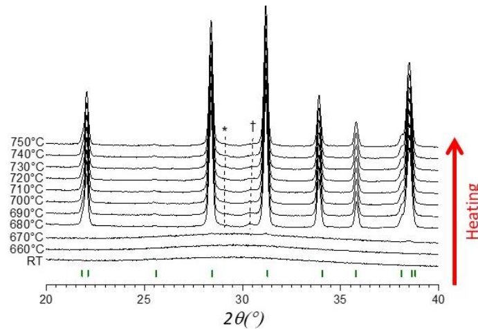
Figure III.5. Variable temperature PXRD measurements on the \text{Ca}_3\text{ZnGe}_5\text{O}_{14} x=1 glass composition showing its crystallisation upon heating, where * and † represent the clinopyroxene \text{CaZnGe}_2\text{O}_6 and melilite \text{Ca}_2\text{ZnGe}_2\text{O}_7 impurities respectively. Green tickmarks represent the P321 \text{Ca}_3\text{ZnGe}_5\text{O}_{14} indexation.
