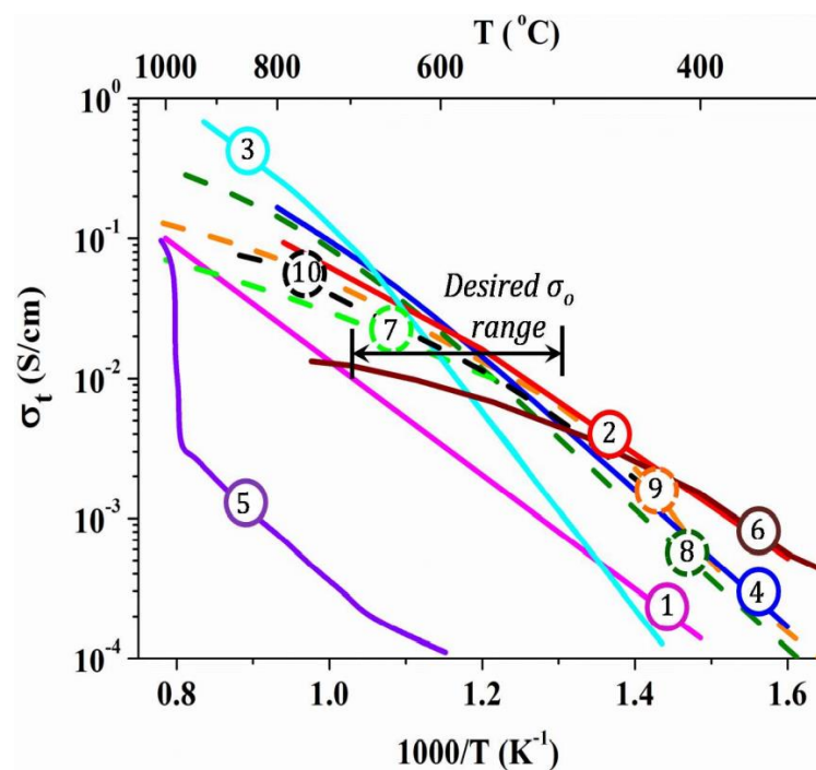
Figure I.12. Arrhenius plots of the total conductivity of, (1) \text{Zr}_{0.9}\text{Y}_{0.1}\text{O}_{1.95} (YSZ), (2) \text{Ce}_{0.9}\text{Gd}_{0.1}\text{O}_{1.95} (GDC), (3) \text{Bi}_{0.75}\text{Y}_{0.25}\text{O}_{1.5} (Stabilized \delta\text{-Bi}_2\text{O}_3 ), (4) \text{La}_{0.8}\text{Sr}_{0.2}\text{Ga}_{0.83}\text{Mg}_{0.17}\text{O}_{2.815} (LSGM), (5) \text{Ba}_2\text{In}_2\text{O}_5 (Brownmillerite), (6) \text{Bi}_4\text{Cu}_{0.15}\text{Ti}_{0.15}\text{V}_{1.7}\text{O}_{11.6} (BICUTIVOX), (7) \text{La}_{9.75}\text{Sr}_{0.25}(\text{SiO}_4)_6\text{O}_{2.895} (Si-apatite), (8) \text{La}_{9.5}(\text{Ge}_{5.5}\text{Al}_{0.5}\text{O}_{24})\text{O}_2 (Ge-apatite), (9) \text{La}_{1.54}\text{Sr}_{0.46}\text{Ga}_3\text{O}_{7.27} (Sr-melilite) and (10) \text{La}_{1.64}\text{Ca}_{0.36}\text{Ga}_3\text{O}_{7.32} (Ca-melilite). Solid and dashed lines correspond to vacancies and interstitial conductor materials. This figure was taken from [94].
