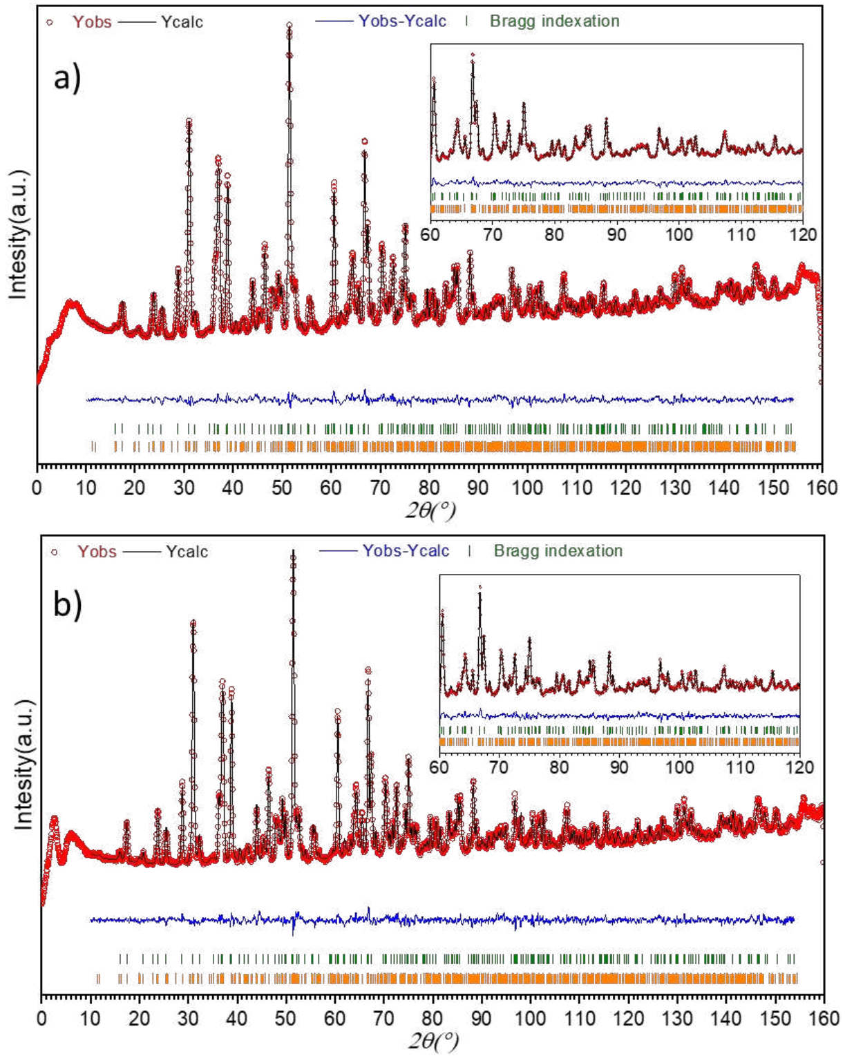
Figure A. 30. 720°C NPD (a) HI, (b) HR data Rietveld refinement of the \text{La}_{1.9}\text{Ba}_{0.1}\text{Ga}_3\text{O}_{7.45} ( x = 0.9 ) composition.
