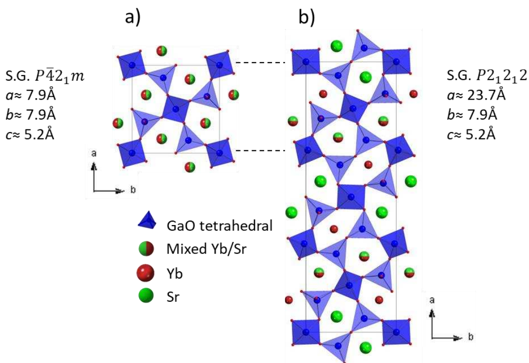
Figure II.1. \text{SrYbGa}_3\text{O}_7 melilite structure projection within the c -axis of both, a) disordered and b) ordered polymorphs.
