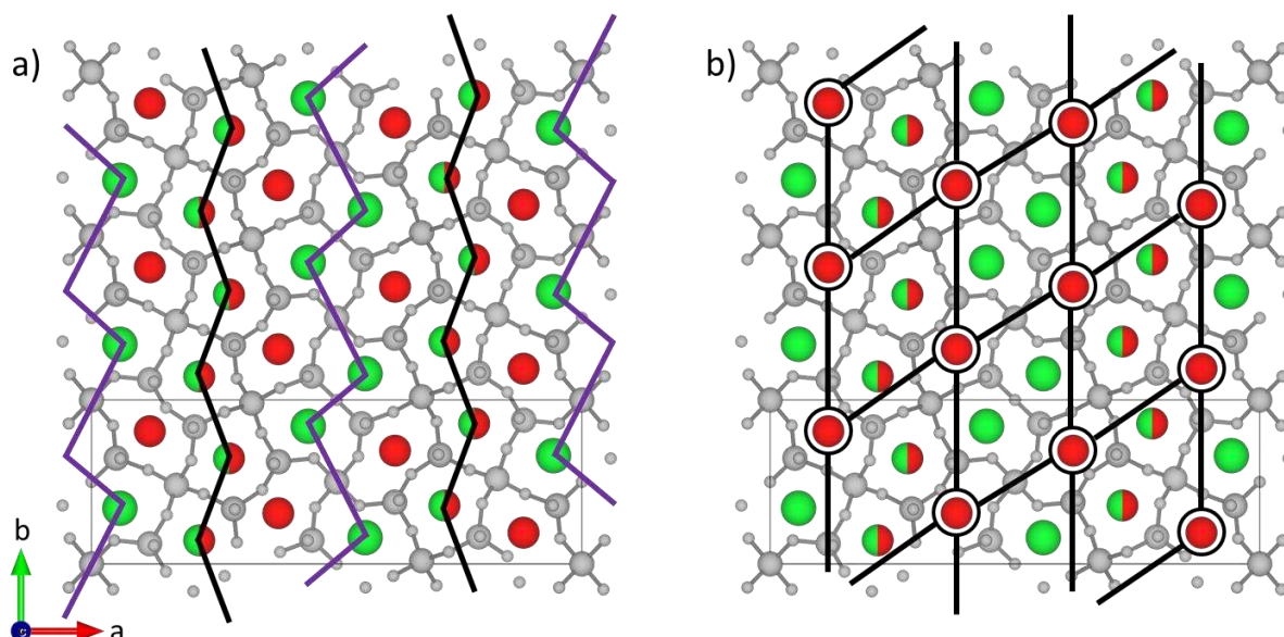
Figure II.15. The cationic substructure of the P2_12_12 ordered melilite, where a) shows the chain-like and stripe-like arrangement of mixed Sr/RE and Sr-only sites, while b) shows the pseudo-hexagonal sub-cell of the RE-only sites.
