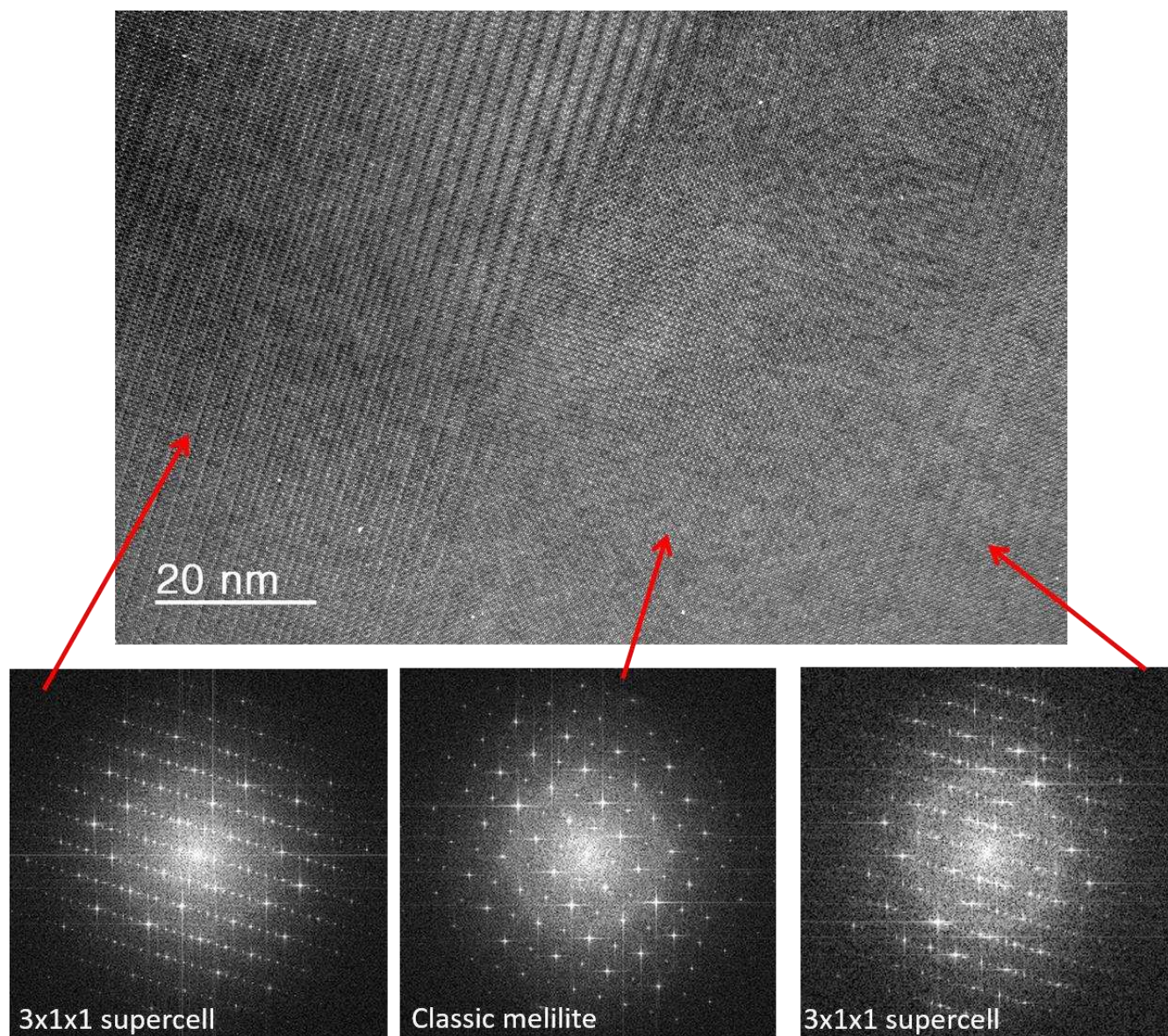
Figure S13. [001]* HRTEM image and associated FFTs of the \text{SrYGa}_3\text{O}_7 melilite parent synthesized by full crystallization from glass. Disordered classic tetragonal P\text{-}4_2\text{m} melilite structure and ordered 3\times1\times1 P2_12_12 melilite supercell coexist like close neighboring nanodomains.
