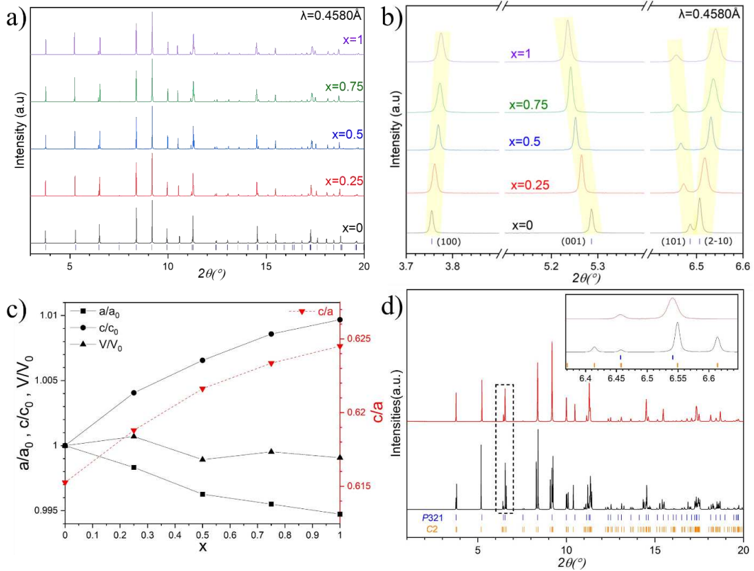
Figure III.10. a) SPD data of \text{Ca}_3\text{Ga}_{2-2x}\text{Zn}_x\text{Ge}_{4+x}\text{O}_{14} x = 0 (black), 0.25 (red), 0.5 (blue), 0.75 (green) and 1 (purple) compositions, with dark blue tickmarks corresponding to \text{Ca}_3\text{Ga}_2\text{Ge}_4\text{O}_{14} indexing. b) Zoom view on the (100) , (001) , (101) and (2\bar{1}0) (S.G P321) peaks shown in (a), highlight the peaks shift. c) Normalised simulated monoclinic \text{Ca}_3\text{ZnGe}_5\text{O}_{14} C2 [2] (in black) and measured \text{Ca}_3\text{ZnGe}_5\text{O}_{14} glass crystallised sample (in red), synchrotron powder diffraction (SPD) plots, with their respective cell indexations in orange and blue tick marks. d) Normalised refined cell parameters (from SPD data) of the P321 langasite structure across the solid solution series to the parent \text{Ca}_3\text{Ga}_2\text{Ge}_4\text{O}_{14} cell parameters.
