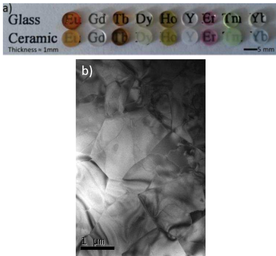
Figure S3. (a) Photograph of the \text{SrREGa}_3\text{O}_7 polished glass and ceramic materials (from Boyer et al., J. Mater. Chem. C, 2016, 4, 3238). (b) Bright field TEM micrograph of the \text{SrYbGa}_3\text{O}_7 transparent ceramic showing a wide grain size distribution and the absence of residual glass, porosity or secondary phase.
