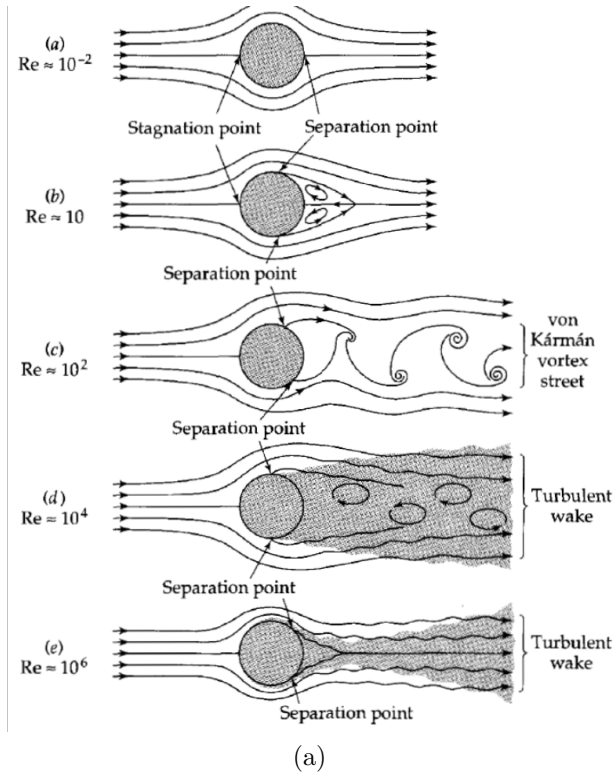
Figure 1.3: Schematic of different flow regimes in the wake of a circular cylinder depending on the Reynolds number of the flow (a) - adopted from [23], and the schematic showing the primary vortex shedding, small-scale modes and the large-scale vortex dislocations (b) - adopted from [200].
