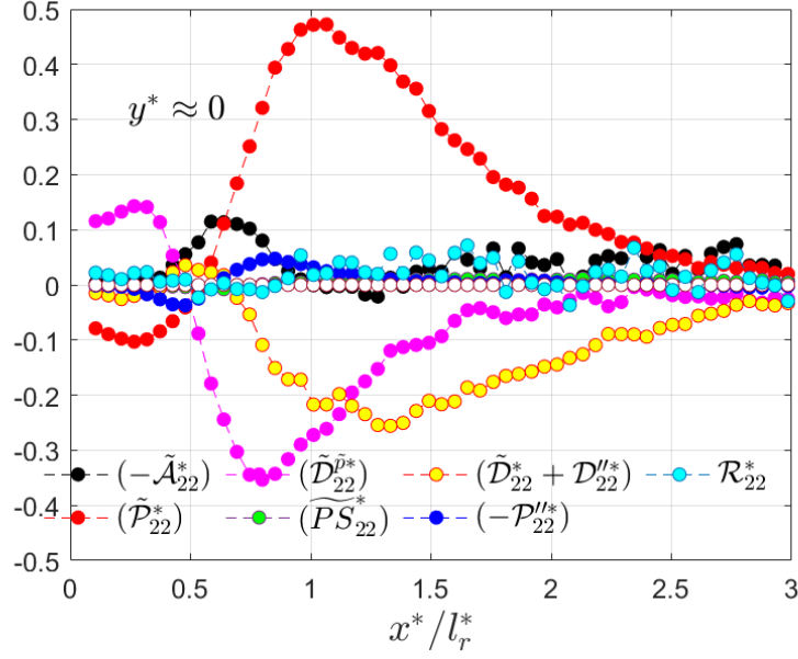
Figure 5.30: Local balance of the transport equation for the coherent transverse normal stress \overline{\tilde{v}^2}^* performed along the wake centerline for the flow at Re_h \approx 2.8 \times 10^4 .
