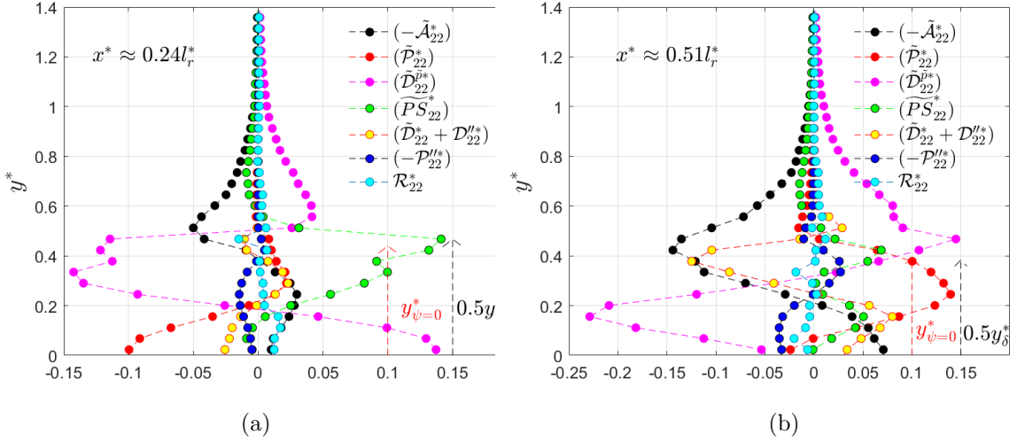
Figure 5.26: Local balance of equation for the transport of Reynolds transverse coherent normal stress \tilde{v}^2 for the flow at Re_h \approx 2.8 \times 10^4 , carried out at x^* \approx l_r^*/4 (a) and x^* \approx l_r^*/2 (b) .
