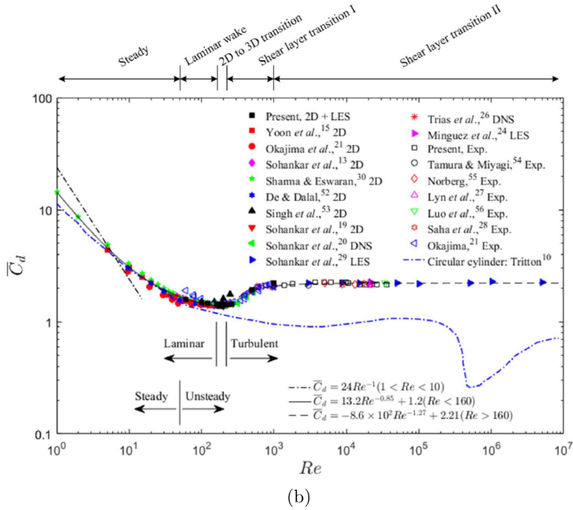
Figure 1.4: Variation of the recirculation length and the formation length (a) and the drag coefficient (b) as a function of Re . Figures adopted from [10]. For the works cited in the figure, one may refer to the references in [10].
