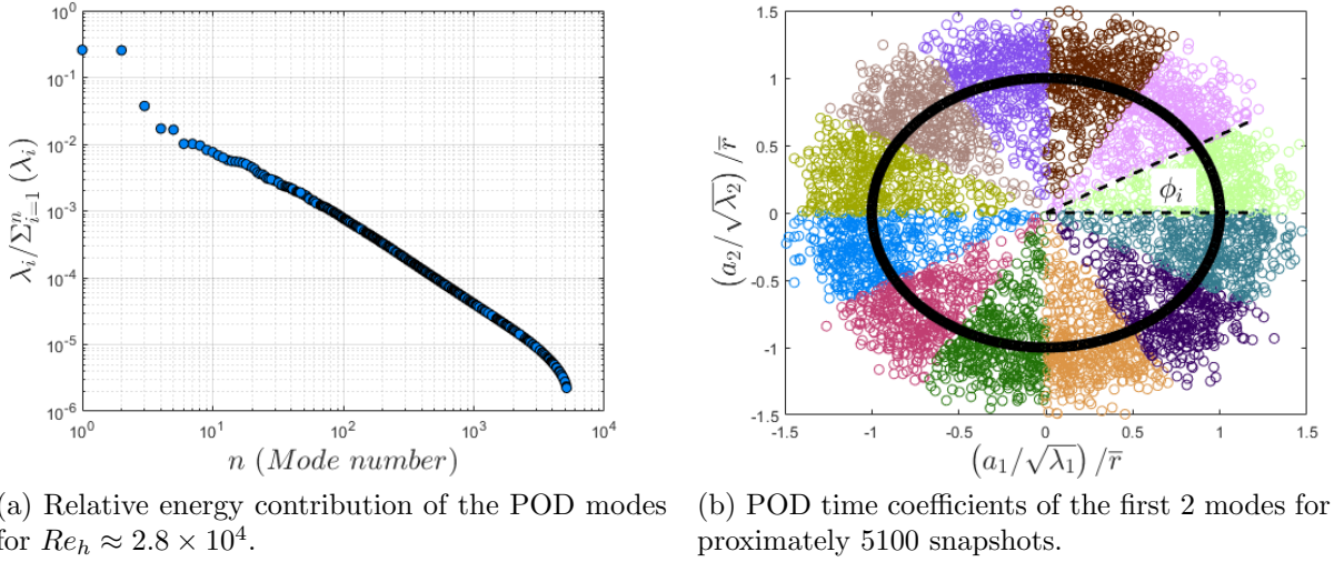
Figure 5.1: Modal energy contribution of POD modes (a) and the time coefficients of the first two modes (b). The color codes in (b) represent the flow split into 12 phases to sort the flow based on the time coefficients in (a_1, a_2) plane (a) and to phase average for the extraction of coherent structures.
