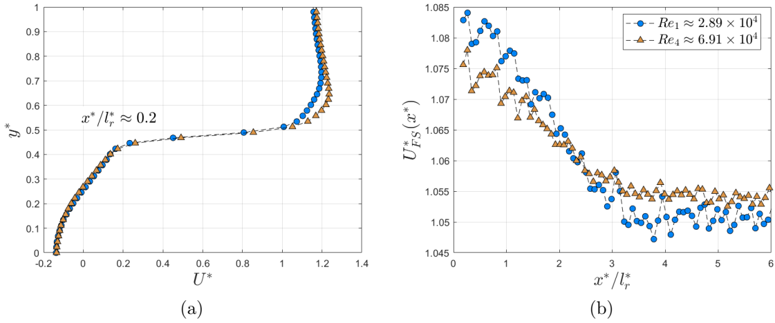
Figure 6.2: Profile of mean streamwise velocity at x^* \approx 0.2l_r^* (a) and the variation of the free stream velocity U^* (b) for the lowest and highest Re_h test cases.
