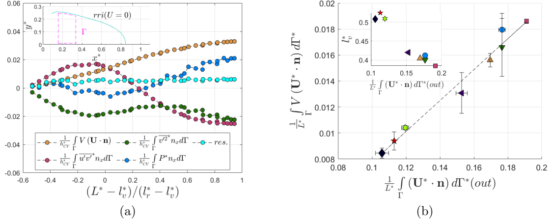
Figure 6.11: Balance of the vertical mean momentum budget carried out on a CV defined by the rrr (shown in the inset) (a) and the variation of mean momentum and mass transported by the mean flow, with the inset showing the variation of l_v^* with the mass entrained by the shear layer.
