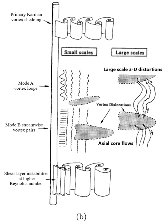
Figure 1.3: Schematic of different flow regimes in the wake of a circular cylinder depending on the Reynolds number of the flow (a) - adopted from [23], and the schematic showing the primary vortex shedding, small-scale modes and the large-scale vortex dislocations (b) - adopted from [200].
