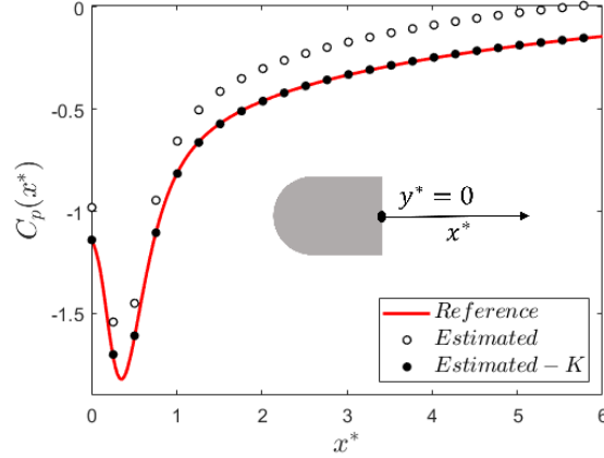
Figure 3.2: Evolution of the mean C_p along the wake centerline at y^* = 0 . ‘Reference’ represents the pressure directly obtained from the turbulent solver and ‘Estimated’ represents the pressure computed using the synthetic flow fields.
