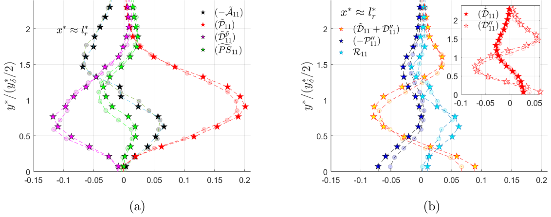
Figure 6.16: Comparison of Local contributions to the transport of coherent streamwise Reynolds normal stresses (a) & (b) at the streamwise location x^* \approx l_r^* , for the baseline flow (circles) and the perturbed flow-field (pentagram) at Re_h \approx 2.89 \times 10^4 . The transverse distance is normalised by the local width of the upper symmetric plane of the wake ( y_\delta^*/2 ).
