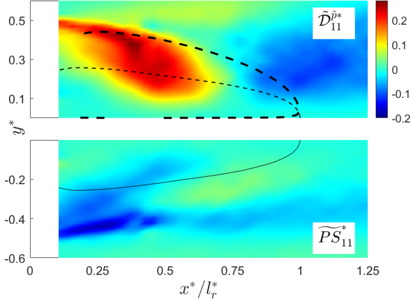
Figure 5.23: Colormap of the pressure diffusion \tilde{\mathcal{D}}_{11}^{\tilde{p}} and the pressure strain \widetilde{PS}_{11} fields for the flow at Re_h \approx 2.8 \times 10^4 . The fields being symmetric, only one of the symmetric planes is shown.
