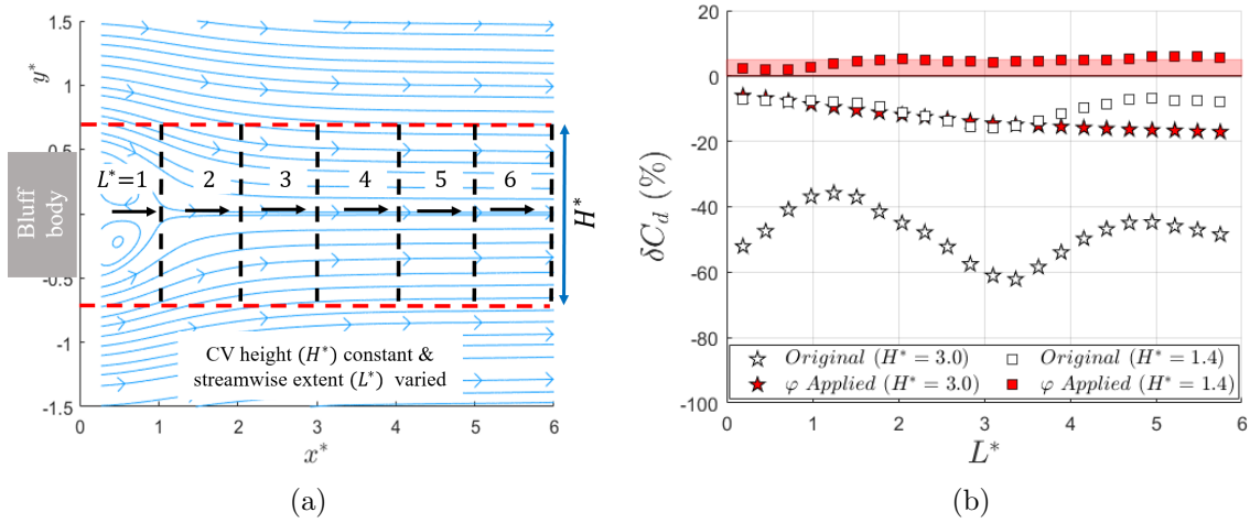
Figure 3.11: Choice of CV size for computation of C_d (a) and C_d computed with a constant CV inlet height H^* and a varying outlet location L^* (b). The red and black dashed line in (a) represent the extent of H^* and L^* respectively.
