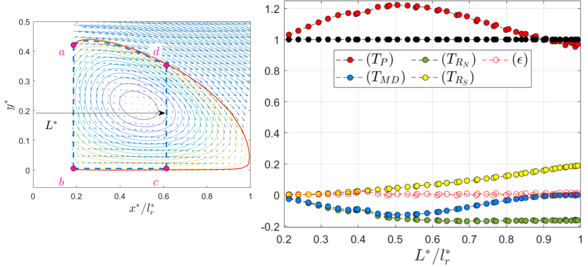
Figure 4.19: The control volume (CV) defined using the stream function \psi = 0 that encloses the recirculating flow region (left) and the budget of base pressure drag (right). Here, L^* refers to the streamwise location of the CV outlet and l_r^* forms the streamwise extent of the recirculating flow region.
