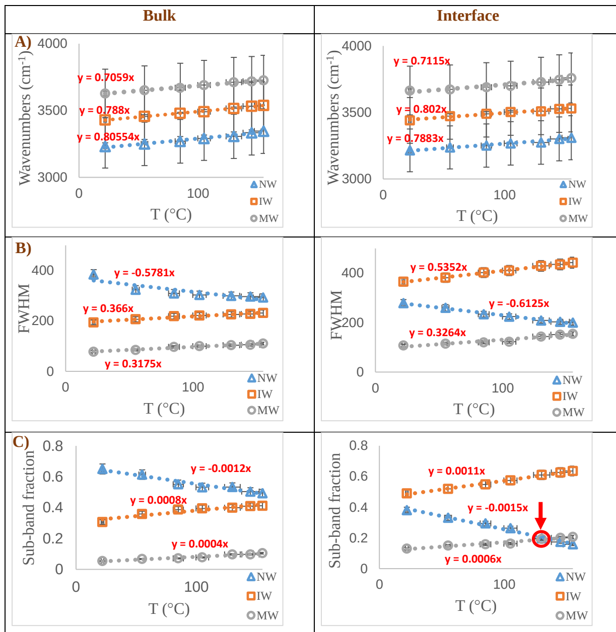
Figure 4.17. The main peak parameters of micro-FTIR water spectrum, such as A) peak position, B) FWHM, and C) sub-band fraction (contribution of each sub-bands) in bulk and interface (near the quartz boundary) at different temperatures. The circle in panel C shows the temperature at which the sub-band fraction of MW becomes more dominant than the NW.
