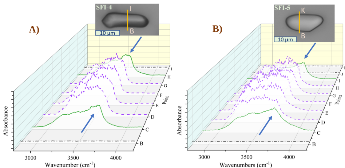
Figure 4.28. The variation of the OH stretching band recorded across the A) SFI-4 ( \text{NaOH } 0.5\text{M} ) (from point B to I)) and B) SFI-5 ( \text{NaOH } 1\text{M} ) (from point B to point K). Black lines (dash-dot line) correspond to quartz, green (solid line) to the near liquid-solid interface, and purple (dash line) to bulk behavior.
