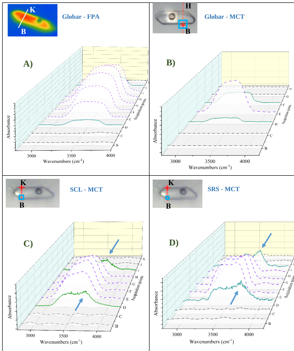
Figure 4.9. The variation of OH stretching band recorded across the SFI-1 before processing steps (from point B to point H or K) with A) Global source with FPA detector (aperture-less microscope), B) Global source with MCT detector, C) supercontinuum laser with MCT detector, and D) synchrotron beam with MCT detector. Black lines (dash-dot line) correspond to quartz, green (solid line) to the near liquid-solid interface, and purple (dash line) to bulk water behavior. The blue squares in panels B, C, and D correspond to the aperture size.
