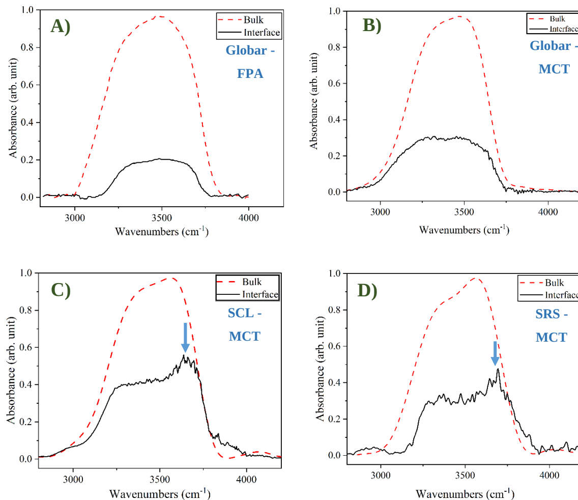
Figure 4.8. The representative spectra of bulk and interface water (along the quartz boundary) using A) Global source with FPA detector ( setup I ), B) Global source with MCT detector ( setup II ), C) supercontinuum laser with MCT detector ( setup III ), and D) synchrotron beam with MCT detector ( setup IV ). The spectra were normalized, and the baseline was corrected. The arrows show the interfacial signature of water recording with setups exploiting supercontinuum laser and synchrotron beam as an infrared source.
