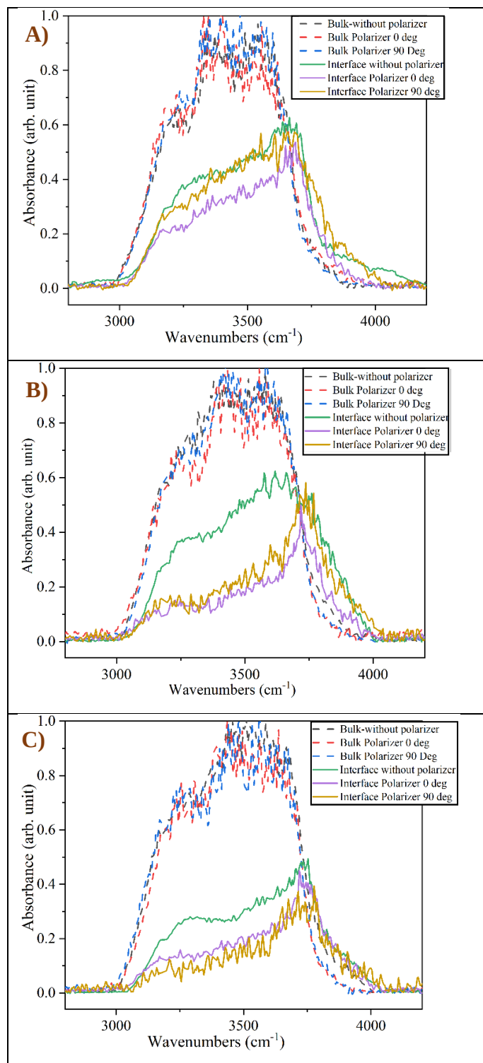
Figure 4.21. The effect of the polarization on the representative micro-FTIR water spectra in bulk and near the solid-liquid interface at A) Z_0 , B) Z_{+40} steps ( +1\ \mu\text{m} ), and C) Z_{-40} steps ( -1\ \mu\text{m} ) after processing steps, such as baseline correction, normalization, and interference fringes removal.
