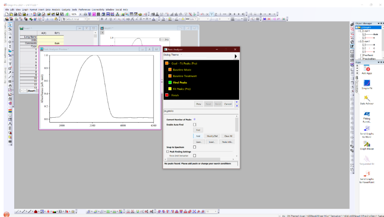
Fig. 11. Defining manually the peak location for each of three desired sub-bands.
