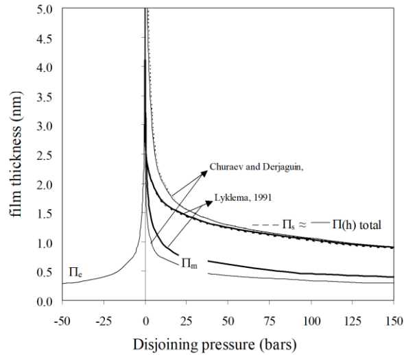
Figure 2.11. Disjoining pressure components (molecular \Pi_m , structural \Pi_s , electrostatic \Pi_e ) as a function of film thickness in a 100 nm slit-shaped pore. Dotted and continuous lines highlight the difference between structural component (dotted line) and total (solid line) disjoining pressure [172].
