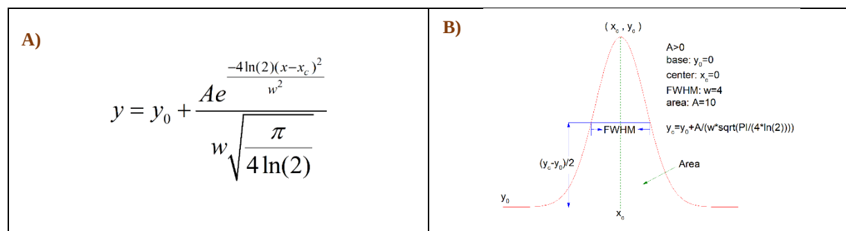
Fig. 13. Choosing the Gaussian model to fit with our recorded bulk water spectrum.
