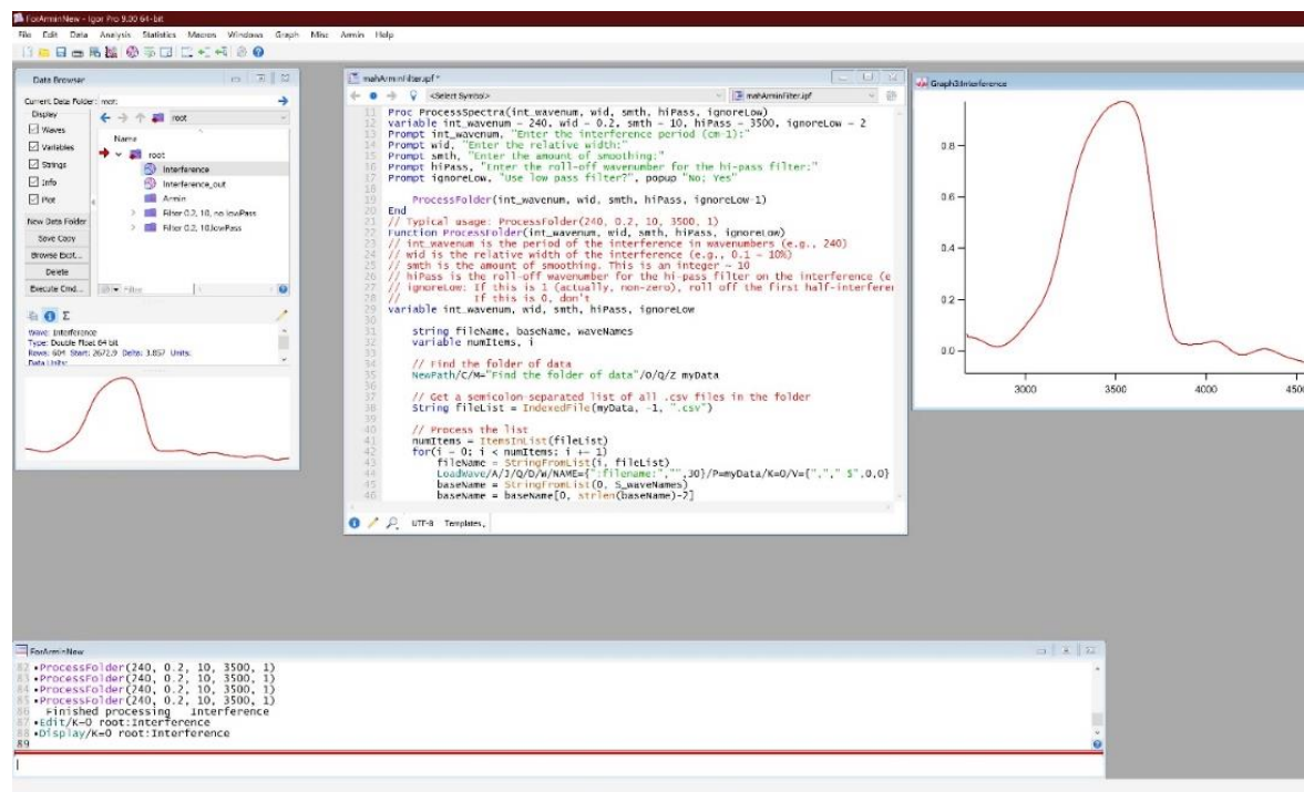
Fig. 3. Added spectrum with the interference fringe.
