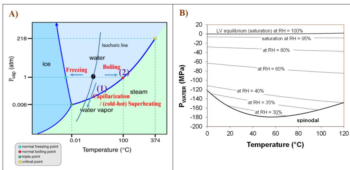
Figure 6.3. A) Schematic pressure-temperature ( P - T ) diagram of water (scales not respected). The black dot corresponds to the ambient conditions. Paths (1) and (2) provide the conditions of water in a superheated metastable state. The appearance of bubbles in the metastable liquid is called cavitation (path 1) and boiling (path 2). B) Saturation curves of capillary water at different relative humidity.
