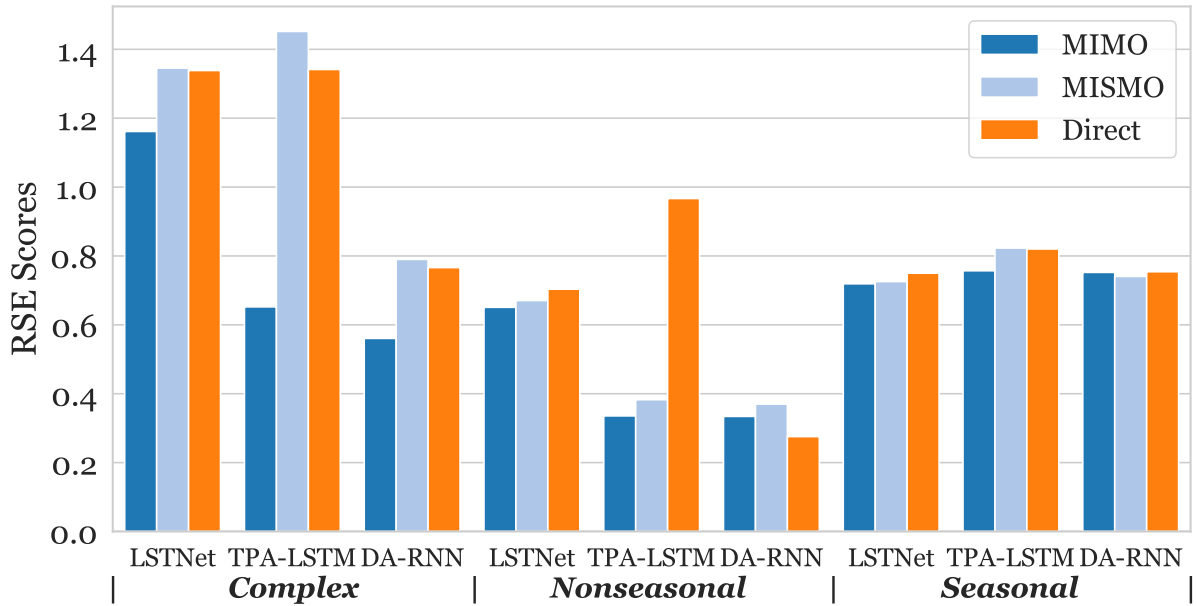
Figure 6.8: Average RSEs for different datasets in MIMO , MISMO , and Direct strategy.
