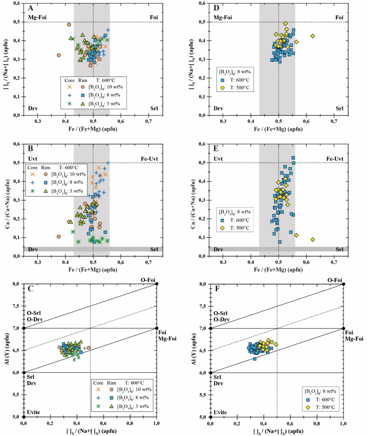
Figure 3.10: Compositions of experimental tourmalines as a function of [B_2O_3]_{fluid} at 600°C (A; B; C) and of temperature at [B_2O_3]_{fluid} = 8 wt% (D; E; F). The grey vertical band represents the at. Fe/(Fe+Mg) of the starting biotite and the horizontal grey band the at. Ca/(Ca+Na) of the starting plagioclase. In [B_2O_3]_{fluid} diagrams (A; B; C), the data come from the charges B600-3, B600-8G and B600-10. In temperature diagrams (D; E; F), the data come from the charges B600-8G and B500-8G. See Table 3.2 and text for experimental conditions. Diagrams A to E from Hawthorne and Henry (1999) and C and F from Bačík et al. (2017).
