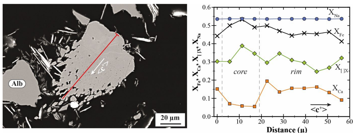
Figure 3. 11: Profil of microprobe analysis on Group II tourmaline in B600-3, plotted in terms of cation ratio. X_{Fe} : at. Fe/(Fe+Mg); X_{Ca} : at. Ca/(Ca+Na+[X]); X_{[X]} : [X]/(Ca+Na+[X]) ; X_{Na} : Na/(Ca+Na+[X])
