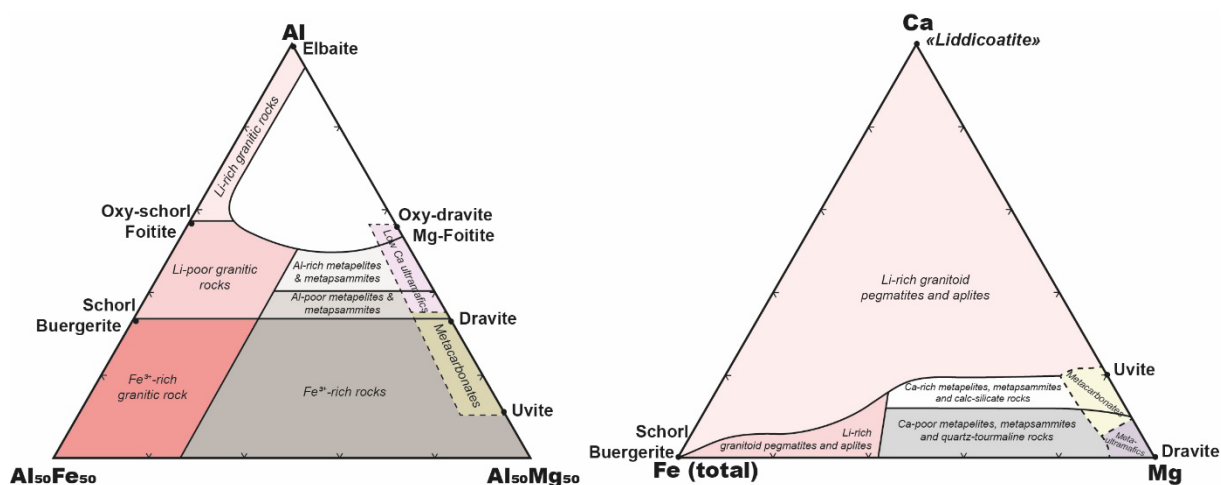
Figure 7: Petrogenetic classification of tourmaline by Henry & Guidotti and van Hinsberg et al. (2011b). The domains delimited by dotted lines are superimposed on the others, delimited by solid lines.
