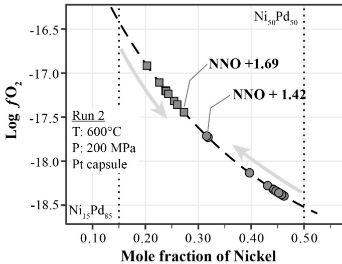
Figure 2. 1: Evolution of the alloy phase of the NiO-NiPd sensor as a function of \log fO_2 in Run 2 (Table 2). The dashed line gives the relation between the mole fraction of Ni in the alloy phase ( X_{Ni} ) and fO_2 at 600°C and 200 MPa using the calibration of Pownceby and O'Neill (1994). The initial X_{Ni} of the two pellets is represented by the dotted vertical lines and their final compositions by squares and circles on the dashed line. Directions of evolution of alloys in each pellet are indicated by arrows.
