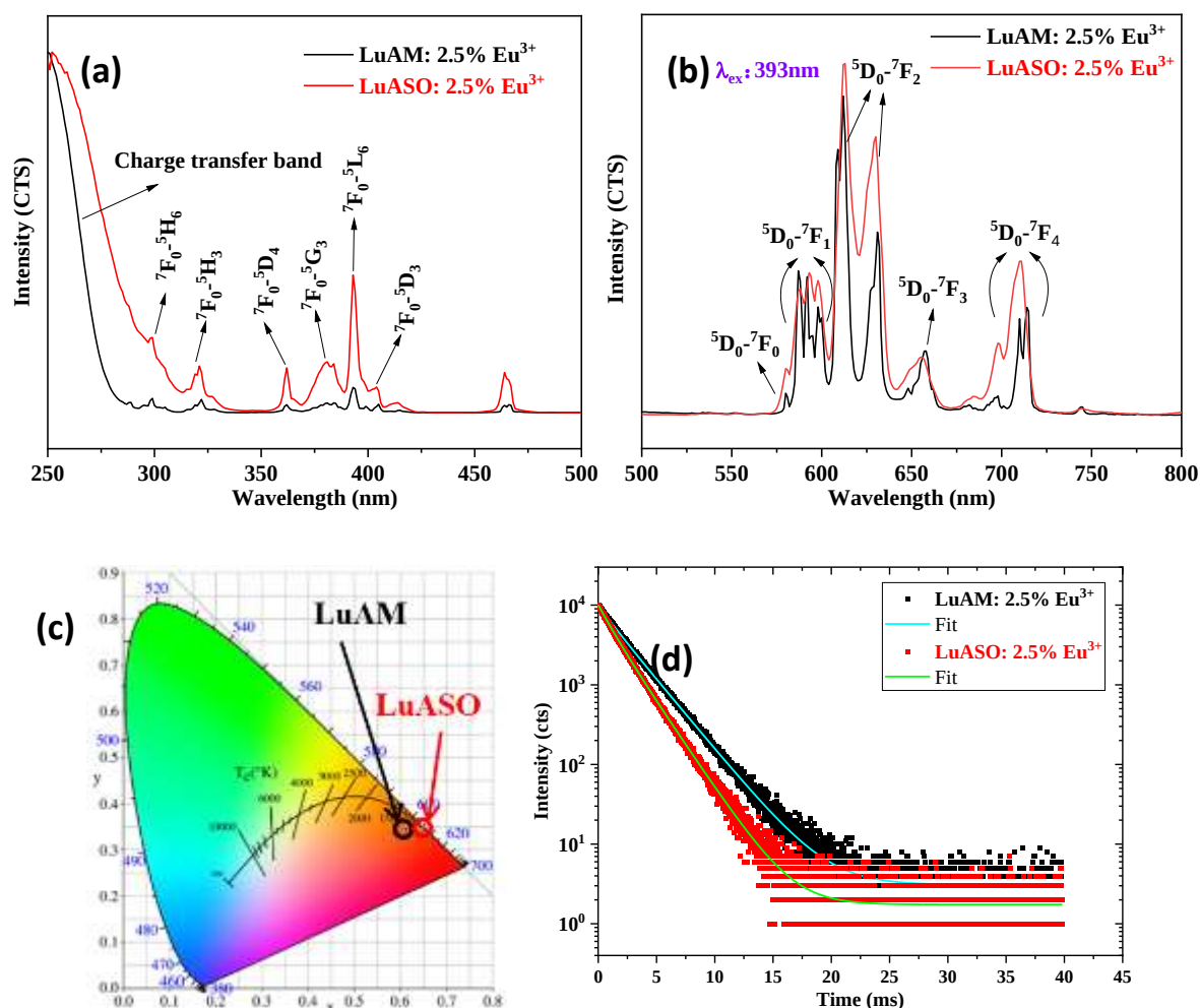
Fig 4.24 Luminescence properties of LuAM: 2.5% Eu^{3+} and LuASO: 2.5% Eu^{3+} (a) PLE and (b) PL spectra measured at room-temperature. (c) CIE chromaticity coordinates diagram. (d) Decay curves.
