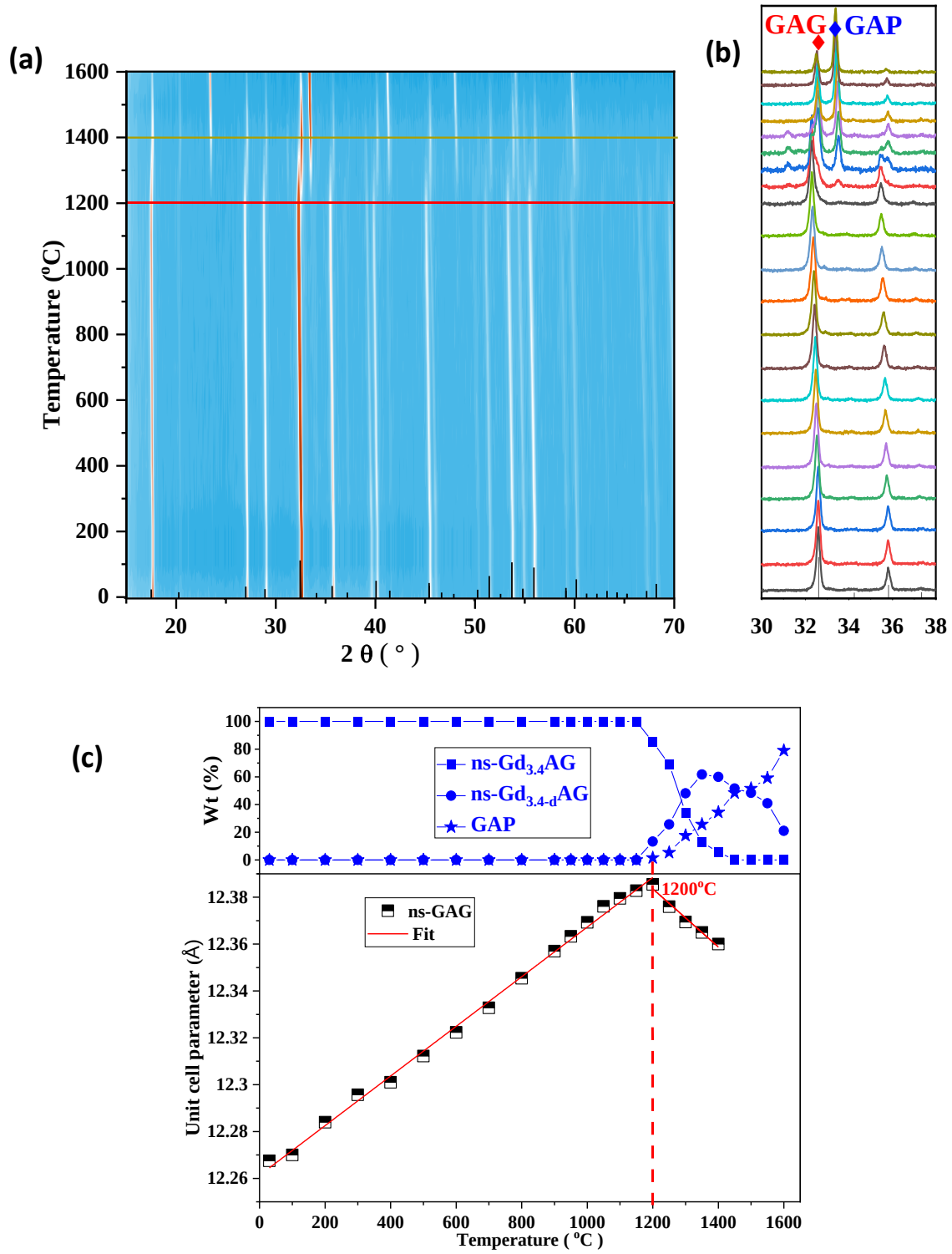
Fig 2.6 VT-XRD measurement of Gd_{3.4}Al_{4.5}O_{12} measured collected from room temperature to 1600°C at intervals of 50 °C (a) Contour figure of X-ray diffraction peaks from 15°- 70° (blue marks are GdAlO_3 perovskite phase) (b) Enlarged diffraction peak pattern from 30° - 38°. (c) The unit cell parameter evolution of ns-GAG (lower) and the wt% of decomposed phase with the temperature increasing (upper).
