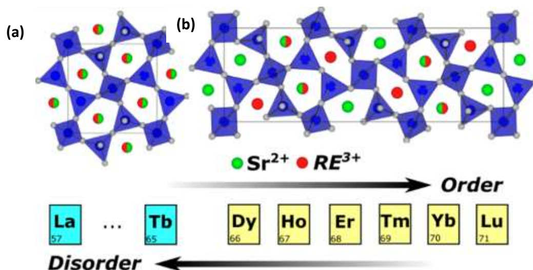
Fig 1.10 [27] Crystal structure of \text{SrREGa}_3\text{O}_7 (a) ( \text{RE} = \text{La to Tb} ) in P421m and (b) ( \text{RE} = \text{Dy to Lu} ) in 3 \times 1 \times 1 orthorhombic ( P2_12_12 ) superstructure.
