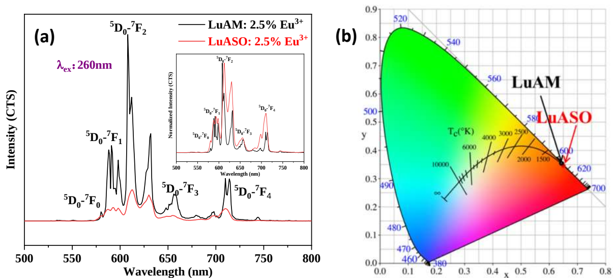
Fig E.3.1 Luminescence properties of LuAM: 2.5% \text{Eu}^{3+} and LuASO: 2.5% \text{Eu}^{3+} under 260nm excitation.
