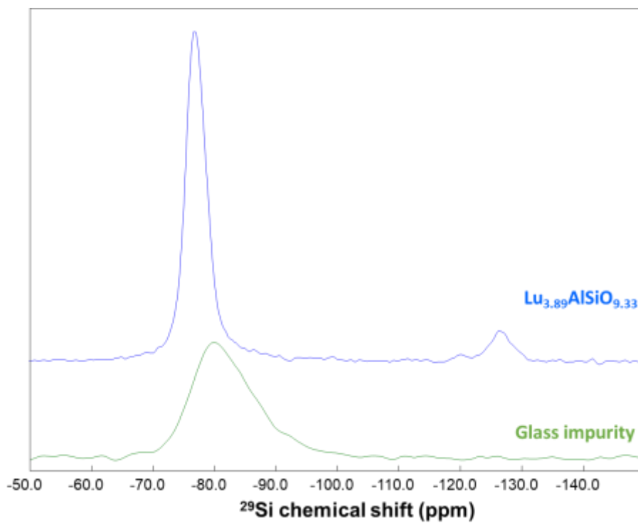
Fig E.2.6 Comparison of ^{29}\text{Si} NMR spectra of glass impurity phases (green curve) and \text{Lu}_{3.89}\text{AlSiO}_{9.33} (blue curve)
