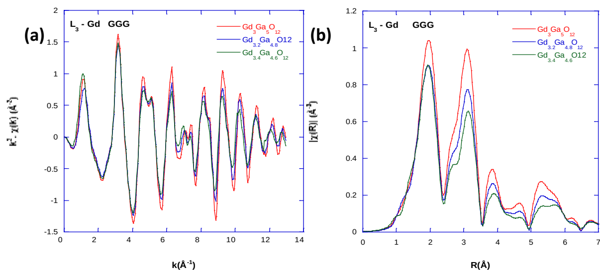
Fig 3.7 (a) EXAFS spectra extracted from the linear absorption coefficient and (b) Fourier transforms of the EXAFS spectra of \text{Gd}_{3+x}\text{Ga}_{5-x}\text{O}_{12} ( x = 0, 0.2, 0.4 ) measured at Gd L_3 edge (7243 eV)
