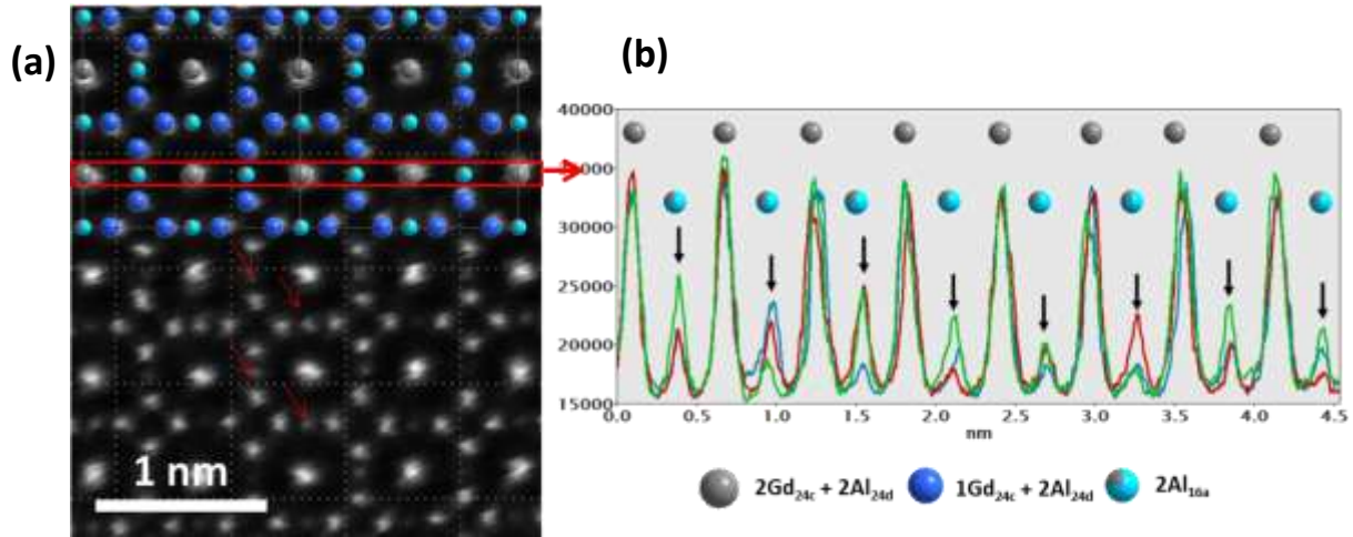
Fig 2.9 STEM information of (\text{Gd}_{0.9}\text{Tb}_{0.1})_{3.4}\text{Al}_{4.6}\text{O}_{12} (a) STEM-HAADF image along [001] orientation and corresponding atoms distribution image superimposed on the HAADF image (the red arrow indicates the bright spot of the 2Al atomic column) (b) Intensity profile extracted from the red box in the HAADF image.
