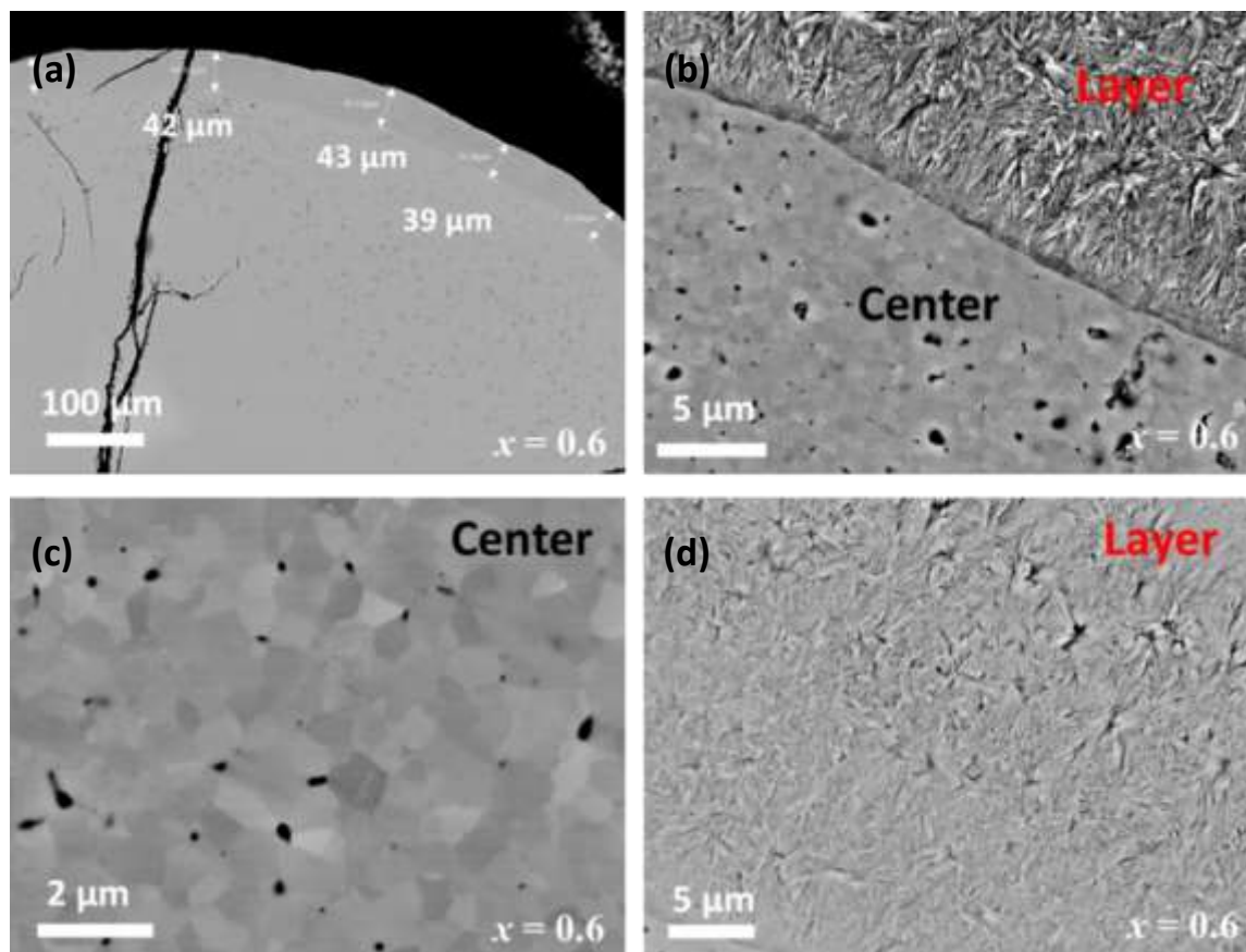
Fig 3.13 SEM (BSE) image of polished Gd_{3+x}(Al_{0.4}Ga_{0.6})_{5-x}O_{12} ( x = 0.6 ) bead. (a-b) Overall microscopic morphology image of a bead surface. Microscopic morphology of the (c) central and (d) layer part.
