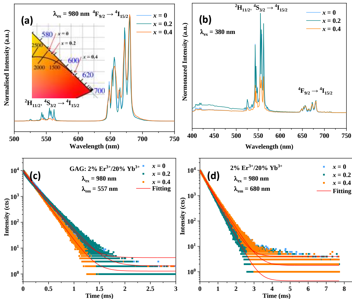
Fig 2.20 Luminescence performance of Gd_{3+x}Al_{5-x}O_{12} (x = 0, 0.2, 0.4): co-doped 2%Er 3+ /20%Yb 3+ polished bead measured at room temperature. (a) Up-conversion emission spectra (CIE chromaticity inset) under excitation at 980 nm. (b) Emission spectra of Er 3+ under excitation at 380 nm. (The intensity of all spectra are normalised by the highest peaks) Decay curves of Er 3+ (c) 557 nm and (d) 680nm emission peak.
