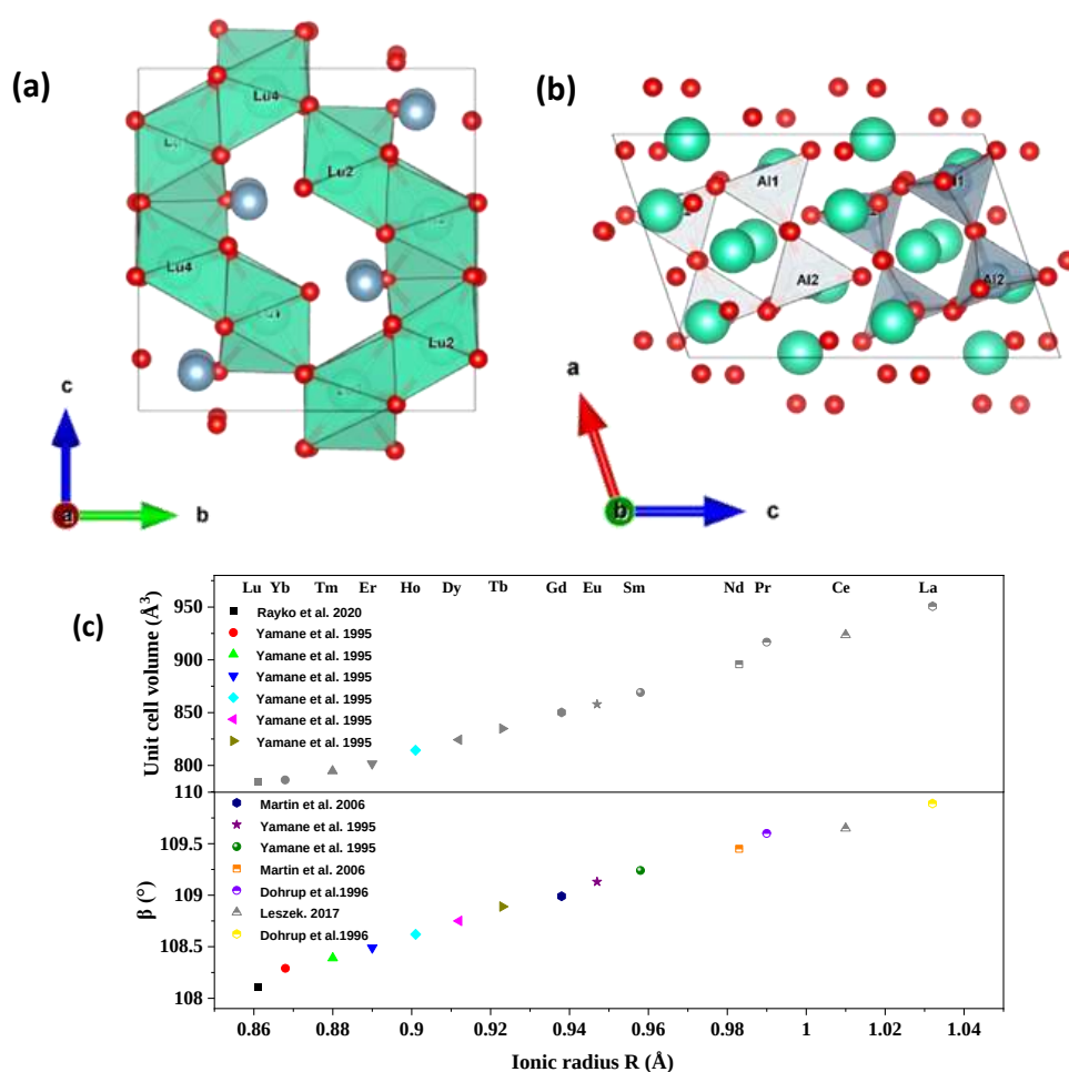
Fig 1.19 Crystal structure of \text{Lu}_4\text{Al}_2\text{O}_9 (a) the Lu centered polyhedra viewed down a axis (b) the \text{Al}_2\text{O}_7 ditetrahedra viewed down b axis. (c) The cell parameters \beta -angle and cell volume V of \text{RE}_4\text{Al}_2\text{O}_9 vs \text{RE}^{3+} ionic radius.
