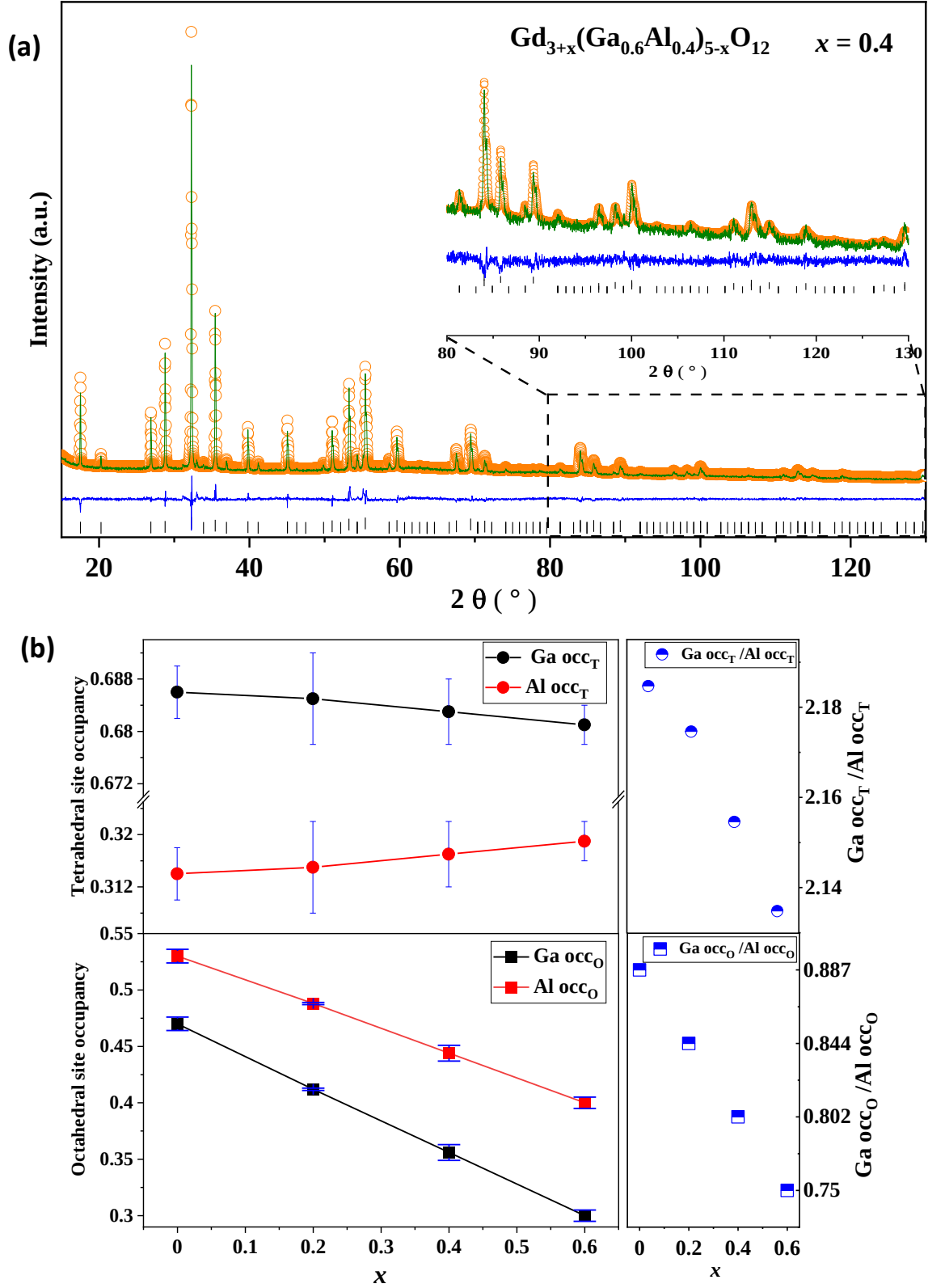
Fig 3.10 (a) XRD Rietveld refinement profile of \text{Gd}_{3.4}(\text{Ga}_{0.6}\text{Al}_{0.4})_{4.6}\text{O}_{12} ( R_{wp} = 4.64\% , Gof = 1.50 ) (b) Occupancy of Ga (black line) and Al (red line) in octahedra (lower) and tetrahedral (upper).
