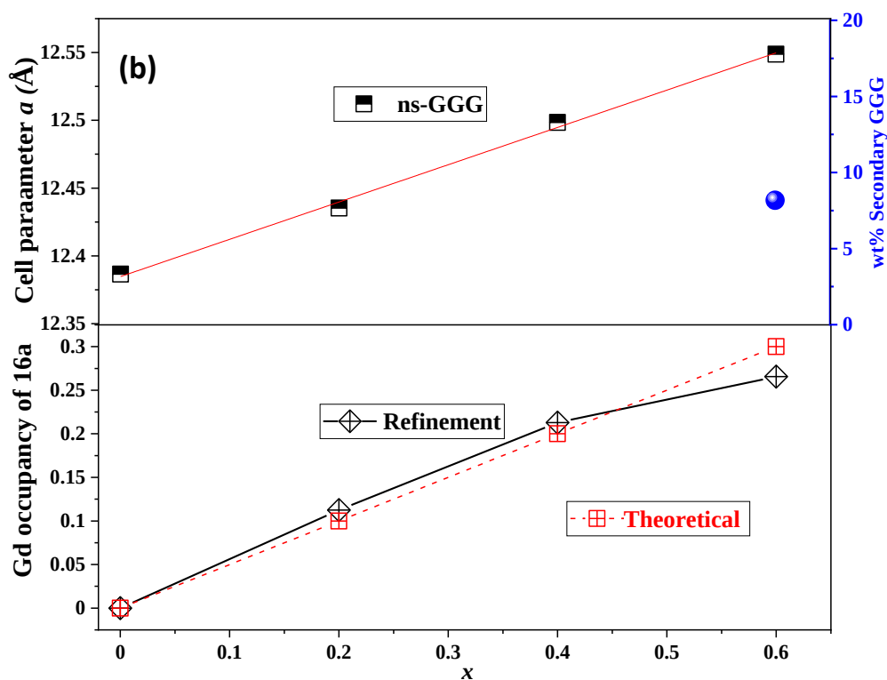
Fig 3.3 (a) SPD Rietveld refinement profile of \text{Gd}_{3.4}\text{Ga}_{4.6}\text{O}_{12} ( R_{wp} = 10.54\% , Gof = 1.92 ) (b) Refined lattice parameter a of ns-GGG (black points) and secondary GGG (blue point) with different x value (upper), plots of refined occupancy of the \text{GaO}_6 octahedral site by \text{Gd}^{3+} (black line) and theoretical occupancy (red line) vs x value (lower).
