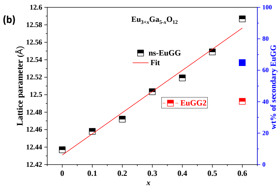
Fig D.1.6 (a) Laboratory XRD pattern of \text{Eu}_{3+x}\text{Ga}_{5-x}\text{O}_{12} ( x = 0 – 0.6 ) sample synthesized by crystallization from melt. (b) Laboratory XRD data refined lattice parameter a of ns-EuGG (blank line) and secondary EuGG (red line) with different x value, and the wt% of the secondary EuGG2 is on the right axis.
