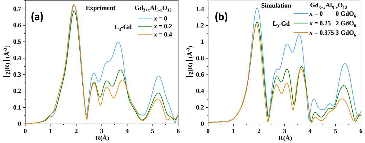
Fig 2.7 (a) Experimental Fourier transforms EXAFS spectra extracted from the linear absorption coefficient measured at the Gd \text{L}_3 -edge. (b) Fourier transforms of EXAFS spectra calculated by FEFF8 on 1 \times 1 \times 1 cells with 0, 2, and 3 substituted \text{GdO}_6 units after DFT relaxation.
