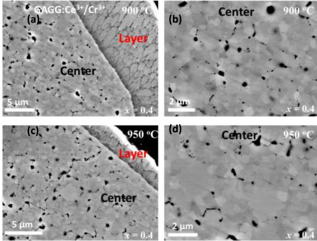
Fig 3.15 SEM (BSE) image of pholished Gd_{3+x}(Al_{0.4}Ga_{0.6})_{5-x}O_{12} ( x = 0.4 ) bead crystallisation at (a-b) 900 °C and (c-d) 950 °C
