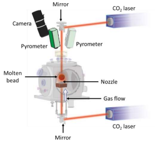
Fig 1.4 The diagram of ADL combined with laser heating setup at CEMHTI.
