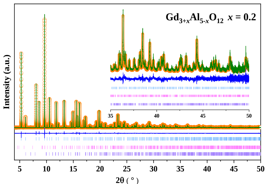
Fig B.1.2 SPD Rietveld refinement profiles of \text{Gd}_{3.2}\text{Al}_{4.8}\text{O}_{12} ( R_{wp} = 9.17\% , Gof = 1.89 ) (light blue ticks marks are ns-GAG garnet reflections, pink tick marks correspond to 1.35(1) wt% \text{Al}_2\text{O}_3 , purple ticks marks correspond to 0.35(1) wt% \text{GdAlO}_3 (GAP) perovskite)
