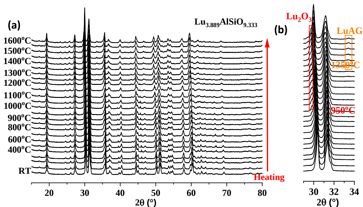
Fig 4.18 (a) VT-XRD pattern from 15°- 70° and (b) 29°-34° enlarged view of \text{Lu}_{3.889}\text{AlSiO}_{9.333} collected from room temperature to 1600°C.
