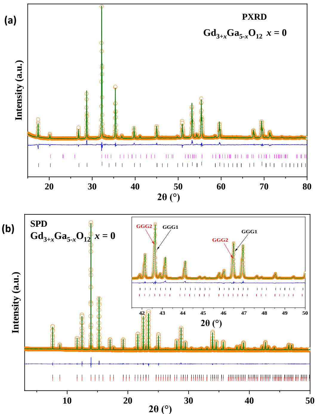
Fig C.1.1 (a) PXRD ( R_{wp} = 3.85\% Gof = 1.97 ) and (b) SPD Rietveld refinement profiles of \text{Gd}_3\text{Ga}_5\text{O}_{12} with 28.7(5) wt% ns-GGG2 (black tick marks are GGG reflections, red tick marks are GGG2 reflections, pink tick marks are \text{GdGaO}_3 reflections).
