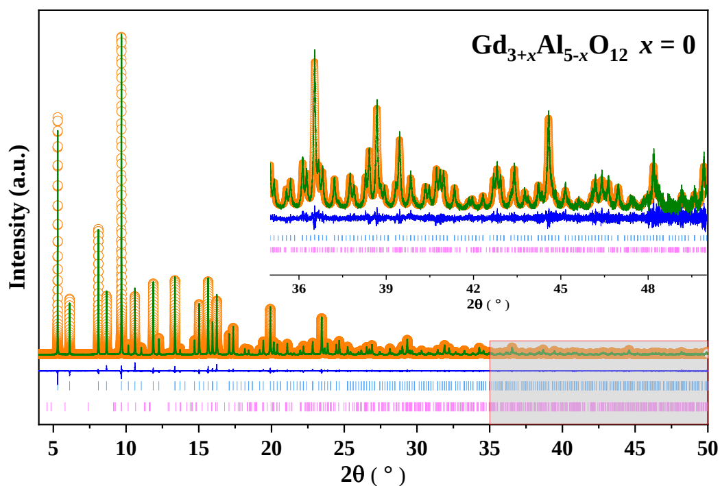
Fig B.1.1 SPD Rietveld refinement profiles of \text{Gd}_3\text{Al}_5\text{O}_{12} ( R_{wp} = 7.41\% , Gof = 1.76 ) (light blue ticks marks are GAG garnet reflections, pink tick marks correspond to 2.36(1) wt% \text{Al}_2\text{O}_3 )
