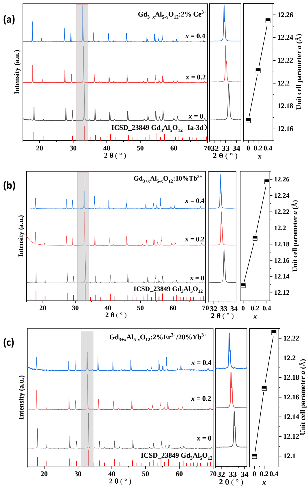
Fig 2.11 The PXRD pattern with zoom of the (211) plane shift and refinement cell parameter a as x value increasing of (a) GAG: 2% \text{Ce}^{3+} (b) GAG: 10% \text{Tb}^{3+} and (c) GAG: 2% \text{Er}^{3+} /20% \text{Yb}^{3+} .
