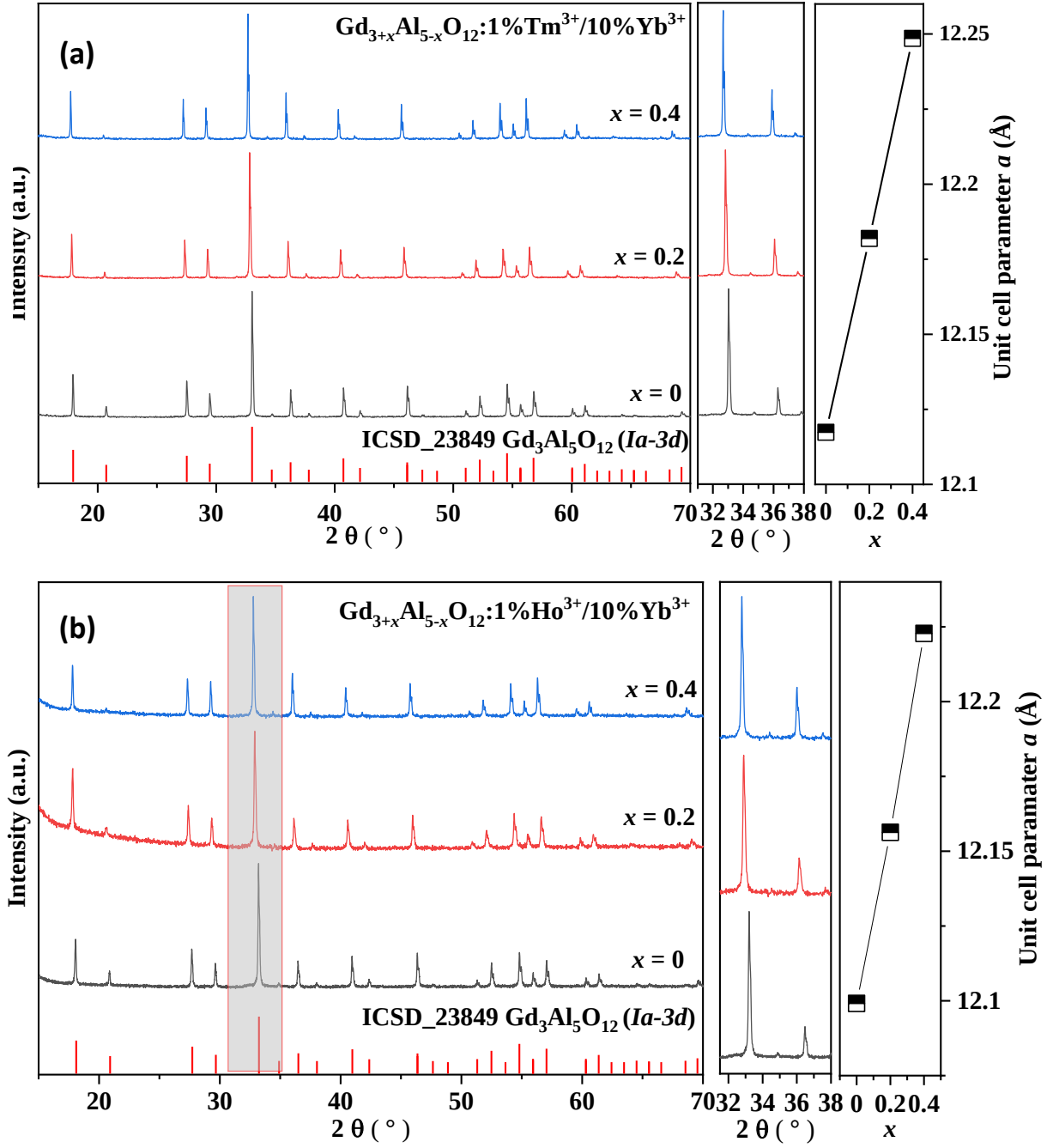
Fig B.1.4 XRD pattern of GAG doped sample \text{Gd}_{3+x}\text{Al}_{5-x}\text{O}_{12} ( x = 0, 0.2, 0.4 ): (a) 1% \text{Tm}^{3+}/10\% \text{Yb}^{3+} , (b) 1% \text{Ho}^{3+}/10\% \text{Yb}^{3+} .
