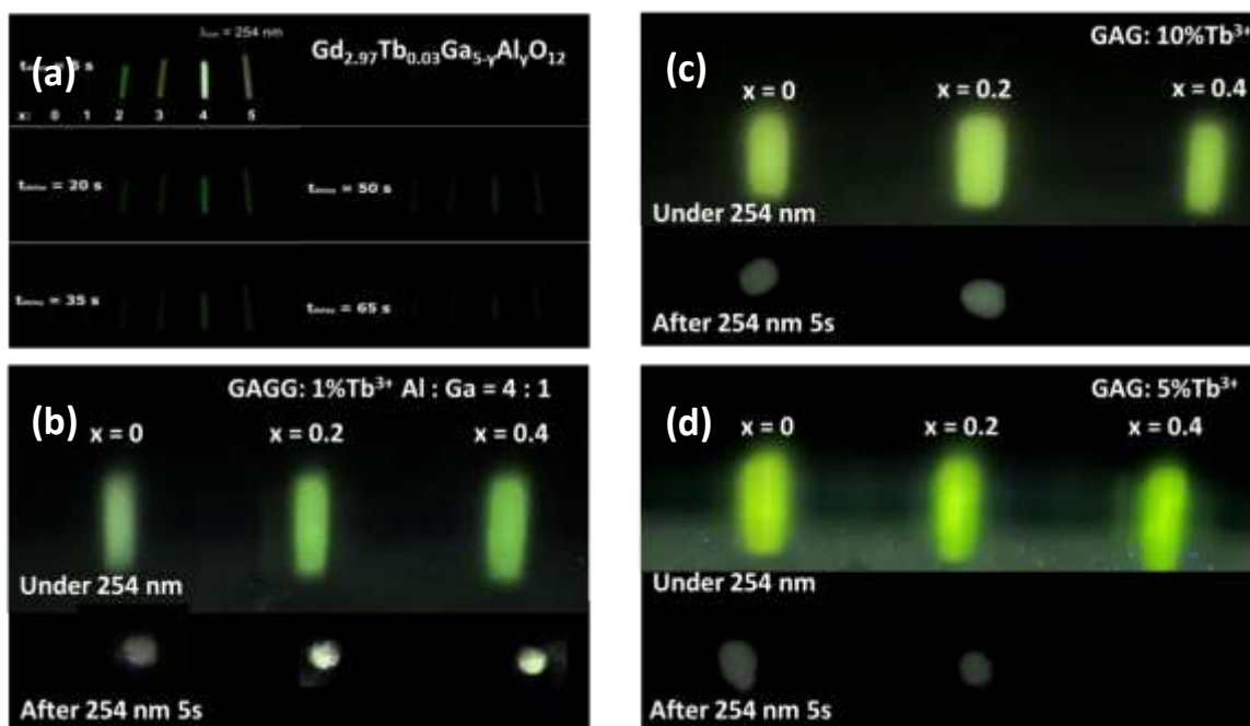
Fig 3.18 The photographs of (a) Gd_{2.97}Tb_{0.03}Ga_{5-y}Al_yO_{12} (adapted from Tomala's paper [16] ), (b) Gd_{3+x}Al(0.8Ga_{0.2})_{5-x}O_{12}: 1\%Tb^{3+} (this work), (c) GAG:10% Tb^{3+} (this work) and (d) 5% Tb^{3+} (this work) emission under 254nm and persistent emission after excitation taken in dark.
