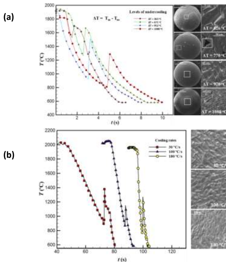
Fig 1.7 [21] Forsterite ( \text{Mg}_2\text{SiO}_4 ). (a) Cooling curves for different levels of undercooling (left) and SEM images of a solidified spherule for different level undercooling, enlarged view of square box (right) (b) Cooling curves for experiments conducted at different cooling rates and SEM images.
