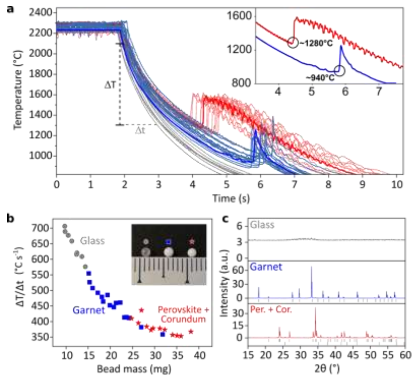
Fig 1.6 [20] (a) Cooling curves recorded in-situ for 36 quenched melts \text{Y}_{3.2}\text{Al}_{4.8}\text{O}_{12} , colour coded to show melts that formed glass (grey), garnet (blue) and mixed phase perovskite/corundum (red). The inset shows a direct comparison of crystallized from low temperature and high temperature undercooled liquid. (b) Cooling rates of three type sample with different mass. (c) PXR patterns of the resulting samples.
