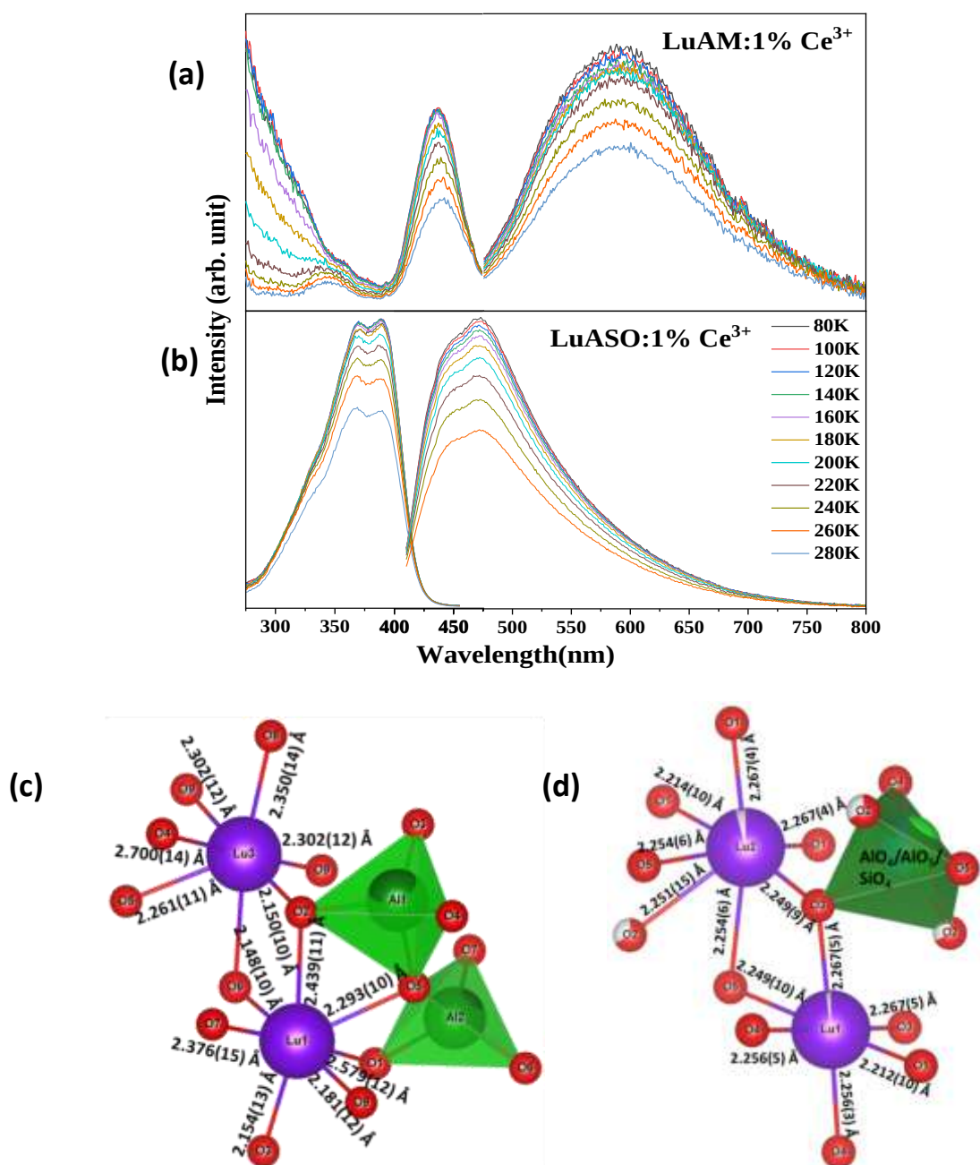
Fig 4.22 PLE and PL spectra of (a) LuAM and (b) LuASO measured at low-temperature ranging from 80k -280k. Ce 3+ environment in two compounds (c) Lu1/Lu3O 7 in LuAM and (d) Lu1O 6 , Lu2O 7 in LuASO.
