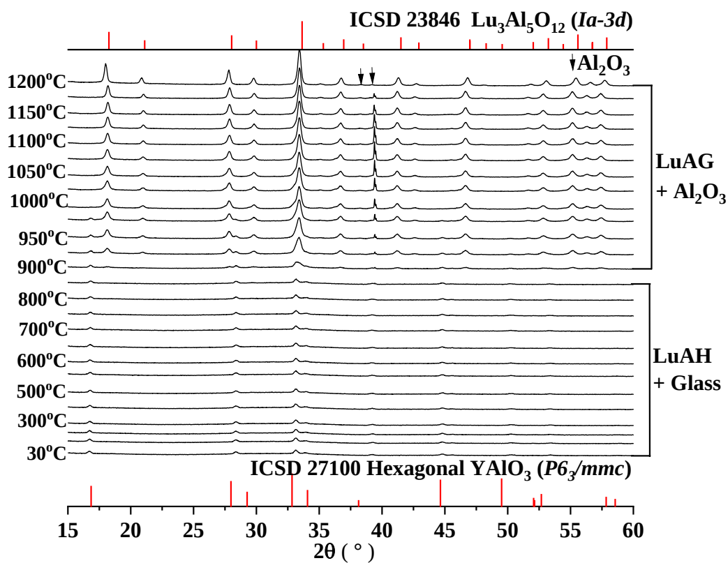
Fig 4.30 VT-XRD pattern of \text{LuAl}_3\text{O}_6 transparent beads measured from room temperature to 1200°C.
