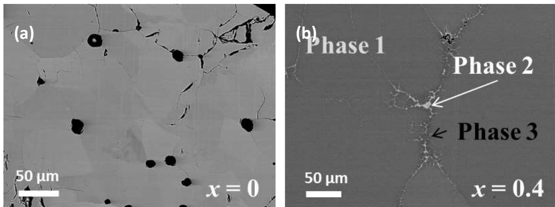
Fig 3.6 SEM (BSE) image of polished (a) \text{Gd}_3\text{Al}_5\text{O}_{12} and (b) \text{Gd}_{3.4}\text{Al}_{4.6}\text{O}_{12} crystallised beads.
