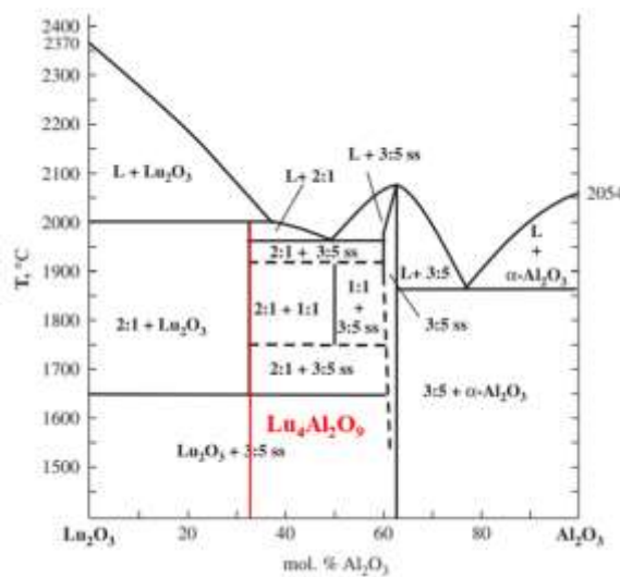
Fig 1.18 [109] \text{Al}_2\text{O}_3 - \text{Lu}_2\text{O}_3 system phase diagram. (red line is \text{Lu}_4\text{Al}_2\text{O}_9 compound)
