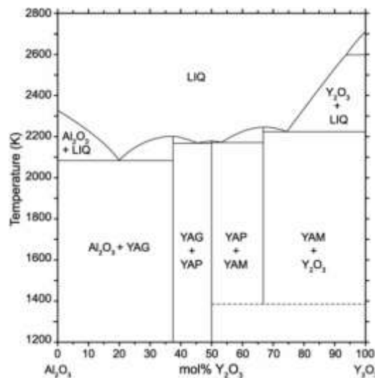
Fig 1.11 [52] Phase diagram of \text{Al}_2\text{O}_3\text{-Y}_2\text{O}_3 . (YAP is \text{YAlO}_3 perovskite, YAG is \text{Y}_3\text{Al}_5\text{O}_{12} garnet, and YAM is \text{Y}_4\text{Al}_2\text{O}_9 monoclinic phase)
