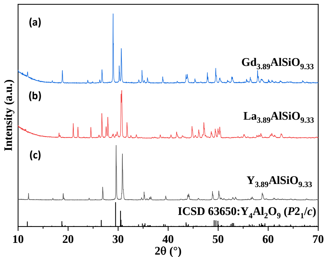
Fig E.2.5 PXRD pattern of (a) \text{Gd}_{3.89}\text{AlSiO}_{9.33} , (b) \text{La}_{3.89}\text{AlSiO}_{9.33} , (c) \text{Y}_{3.89}\text{AlSiO}_{9.33} .
