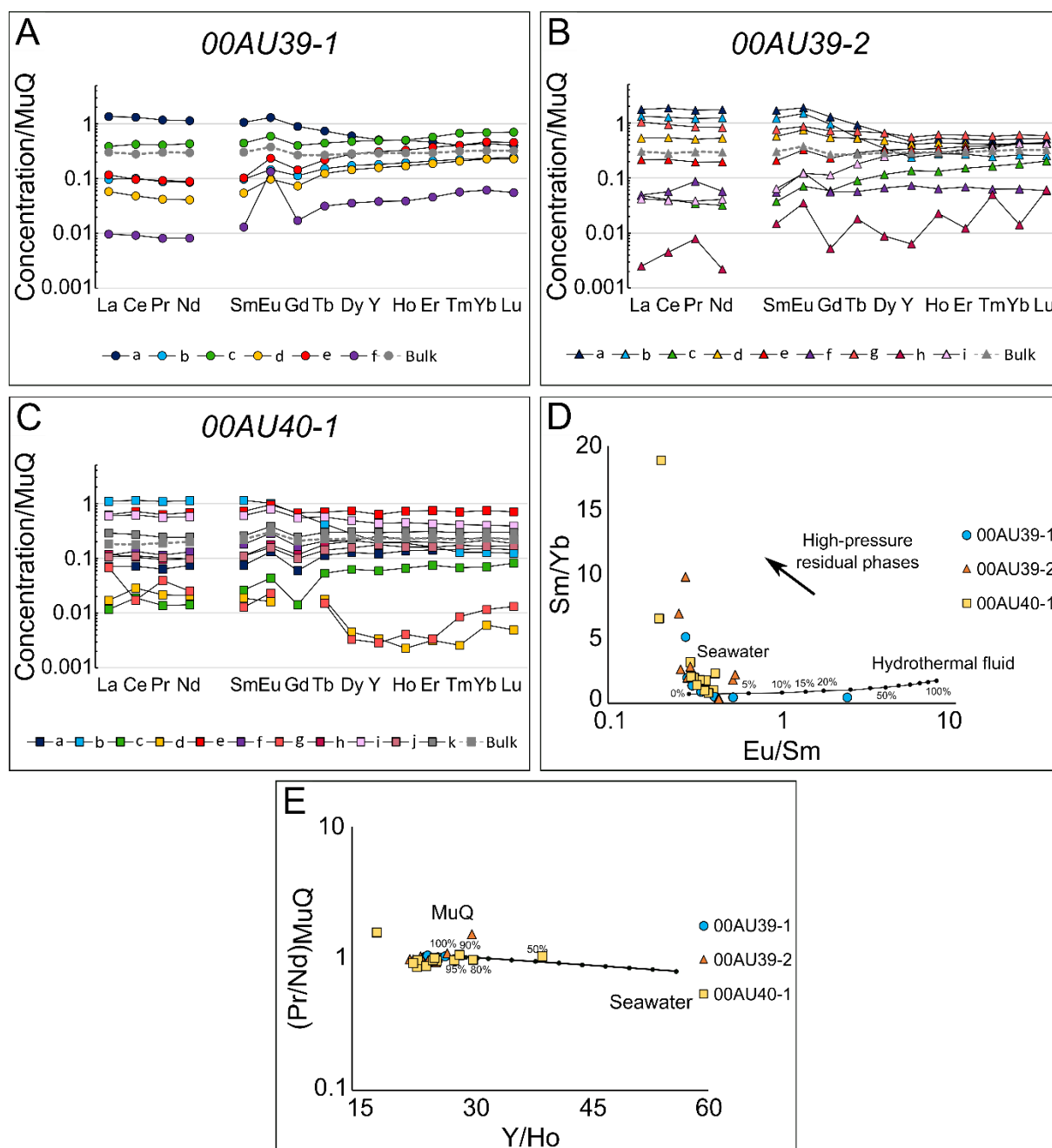
Figure III.10: In situ LA-ICP-MS results. ( A, B, C ) In situ LA-ICP-MS results (solid lines) compared with bulk ICP-MS (dashed lines), showing MuQ-normalized REE + Y composition in samples 00AU39-1, 00AU39-2 and 00AU40-1. ( D, E ) In situ LA-ICP-MS and bulk ICP-MS data plotted against the hydrothermal fluid–seawater and MuQ–seawater mixing lines. ( D, E ) are plotted after methods described in Gourcerol et al. (2016); modified after Hickman-Lewis et al. (2020a).
