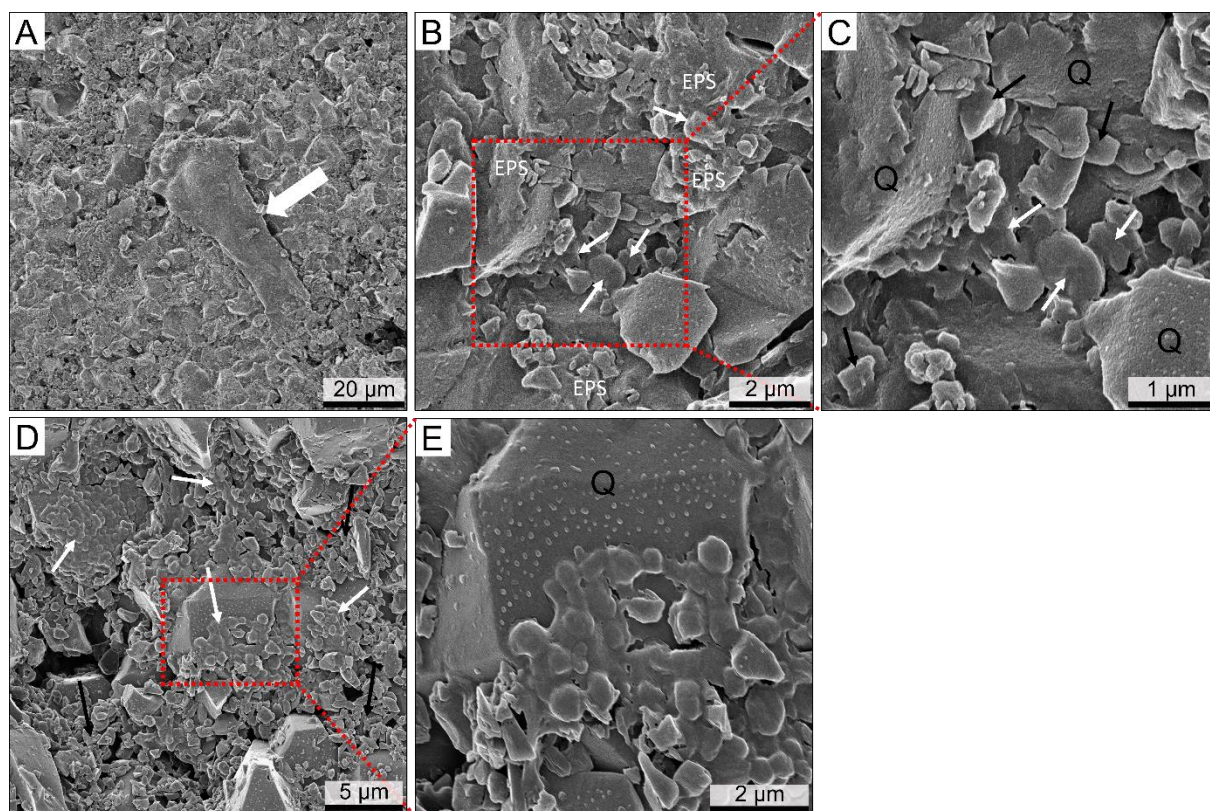
Figure IV.2: Helium ion microscopy (HIM) micrographs of carbonaceous structures in the sediments of the Kitty's Gap Chert. (A) Large (>50 µm long) detrital particle of solid, angular carbonaceous matter embedded in the volcanoclastic sediments (white arrow). (B) Small associations (on the order of micrometers) of dispersed, dividing cells (white arrows) and associated EPS, interpreted as chemolithotrophic microorganisms, with red dotted box indicating the area corresponding to the image displayed in (C). (C) Slightly degraded cells (white arrows) and their associated EPS (see Westall et al., 2015b for further details of degraded cells in the Kitty's Gap sediments). For comparison, minute, angular volcanic dust particles trapped in the EPS matrix are highlighted with black arrows. (D) One of the rare areas in which a larger association (colony) of coccoids has been preserved, with white arrows showing locations of the coccoidal microfossils and black arrows the fine-grained volcanic dust-silica gel matrix comprising small, angular particles having the same dimensions (but not the same morphology) as the coccoidal cells. Red dotted box indicates the area corresponding to the image displayed in (E). (E) Slightly degraded cells embedded in EPS exhibiting cracks probably due to syneresis (i.e., expulsion of fluids from sediments or forms of soft material; e.g., EPS in this case, following the contraction of the silica gel under the effect of diagenesis). The nm sized blobs on the quartz crystal (Q) surface are gold particles from the coating process (the sample was first prepared in 2000 and it was necessary to renew the Au coating for the analyses presented herein). The HIM images were acquired
