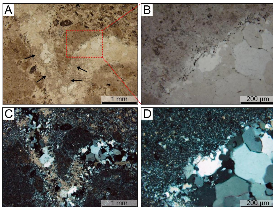
Figure III.5: Silica vein in sample 00AU39. (A) Transmitted light optical image of a large silica vein a few millimeters wide composed of microcrystalline quartz (<200 \mu\text{m} in diameter) and outlined with flakes of sericite (black arrows). The red dotted box indicates the area corresponding to the image displayed in (B). (B) Enlarged view of the silica vein showing large crystals of quartz with a hexagonal shape. The silica vein is also surrounded by dark nanocrystals of anatase (small black dots). (C, D) Polarized light optical images of the same areas highlighting the different polarization shades of quartz depending on the orientation of the crystals (from white to black), and sericite flakes (in beige). The darker areas around the silica vein are fine-grained volcanic dust particles mixed with silica.
