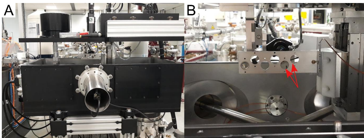
Figure II.12: Pictures of the microbeam line chamber for PIXE analyses at AIFIRA facility where the sample fixed on its metal sample holder with carbon tape is visible from behind (red arrows).
