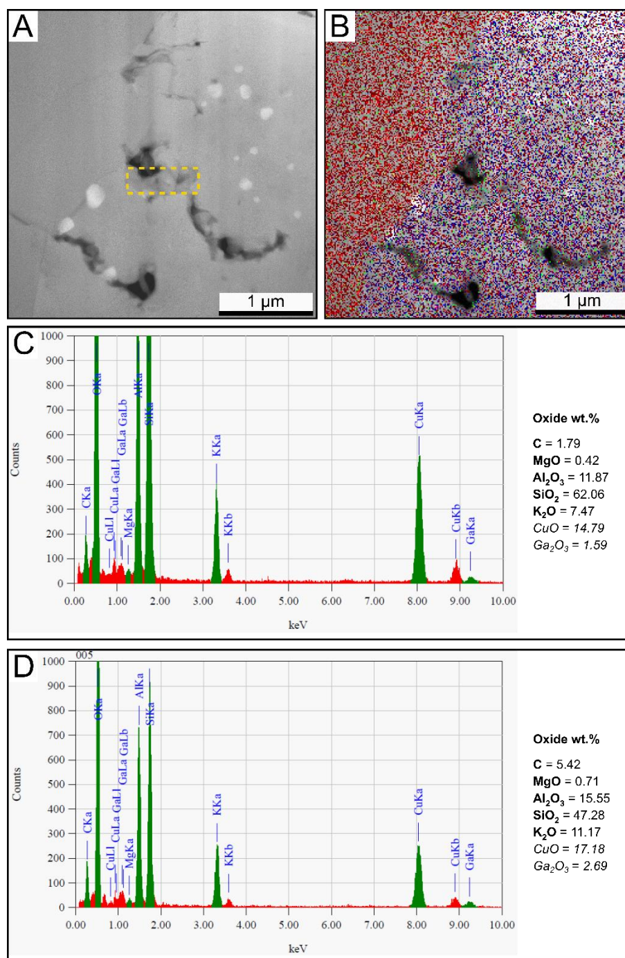
Figure B9: EDX-STEM results of the analysis of the silica-dust gel matrix in sample 00AU40. (A) STEM image of elongated structures of carbonaceous matter (dark color) in a microcrystal of feldspar, with the yellow dashed box corresponding to the location where the EDX measurement was performed and whose spectra is shown in (D) , and the global spectrum associated to this area is shown in (C) . (B) Color-coded composition image of the area analyzed in (A) , with the microcrystalline quartz enriched in silicon (red) and the microcrystal of feldspar enriched in aluminum (blue) where the elongated structures of carbonaceous matter (green) are embedded. (C) EDX global spectrum of the area analyzed in (A) . (D) EDX spectrum associated to the location analyzed in (A) . The mass percentage of each compound is given in oxide wt.% to the right of the spectra (the copper comes from the sample holder and the gallium from the laser beam used to make the FIB section).
