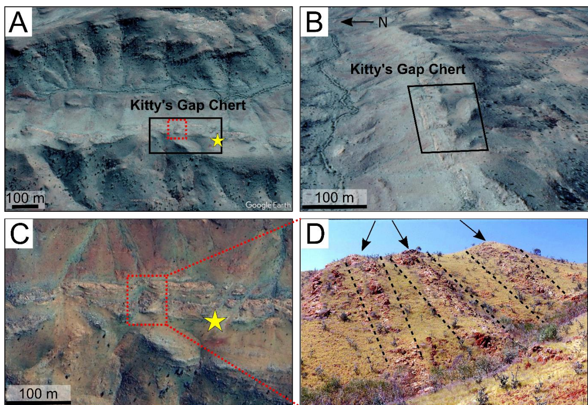
Figure II.3: Aerial and field images of the Kitty's Gap Chert. (A) Satellite image (Google Earth) of the Kitty's Gap Chert with black box indicating the location of the main study area from which the studied samples were obtained and red dotted box indicating the area corresponding to the image displayed in (C). (B) Satellite image (Google Earth) of the same area seen in profile; black arrow indicates the direction of north. (C) Close-up view (Google Earth) of the outcrop of the Kitty's Gap Chert with red dotted box showing the location of the outcrop on the field in (D). (D) Field photograph of the outcrop of the Kitty's Gap Chert showing vertical bars of silicified sediments (black arrows and black dashed lines) separated by mafic lavas. Photograph taken by Frances Westall in August 2000. The yellow star in (A) and (C) corresponds to the location where the samples were collected.
