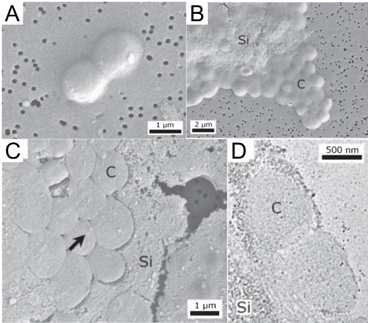
Figure I.5: Experimental fossilization of cells. Scanning electron microscopy (SEM) micrographs of (A) fresh, dividing Pyrococcus abyssi cells (C), (B) aggregates of cells (C) and light silica precipitates (Si) after 24h of silicification, (C) cells (C) trapped in the amorphous silica precipitate (Si) after 24h; silica particles precipitated on the cells are visible (black arrow). Transmission electron microscopy (TEM) micrograph of (D) cells (C) with silica (Si) deposited around the cell envelope after 1 month (after Orange et al., 2009).
