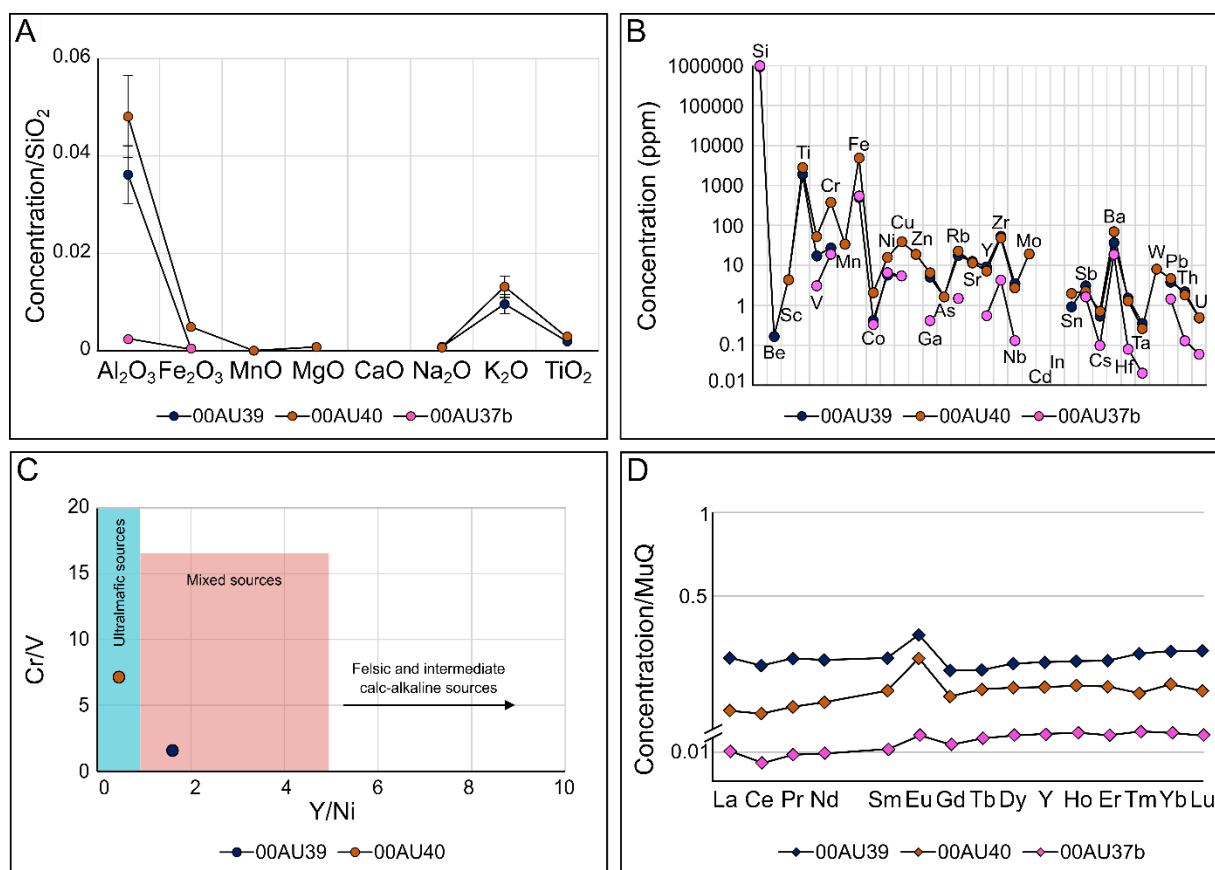
Figure III.9: ICP-OES and ICP-MS results. (A) ICP-OES analyses of major element concentrations normalized to \text{SiO}_2 in bulk samples 00AU39 (blue), 00AU40 (orange) and 00AU37b (pink). The error bars indicate uncertainties calculated for oxides whose concentration relative to that of \text{SiO}_2 is >0.01 (uncertainties for other oxides are too small to be represented). (B) Extended ICP-MS major and trace element concentrations (ppm) in the samples (modified after Hickman-Lewis et al., 2020a). (C) Bulk ICP-MS results of \text{Cr/V} versus \text{Y/Ni} for samples 00AU39 and 00AU40 (modified after Hickman-Lewis et al., 2020a). (D) MuQ-normalized bulk ICP-MS measurements of REE + Y in the samples.
