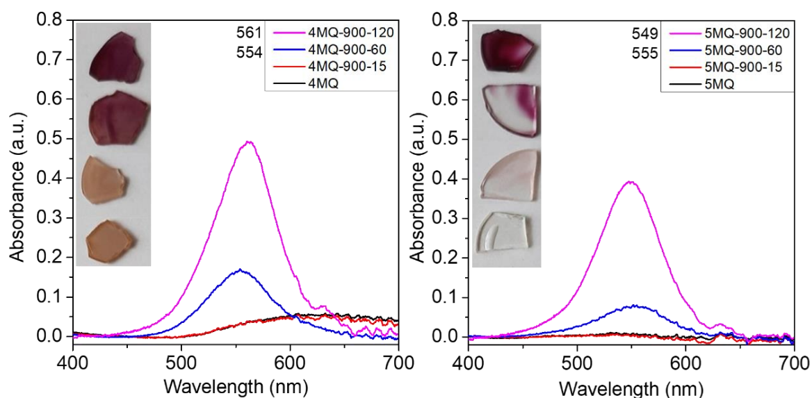
Figure 47 The effect of annealing on the absorption spectra of samples 4MQ (highest Au content + \text{SnO}_2 ) and 5MQ (medium Au content + \text{SnO}_2 ). Au nanoparticles prepared in \text{Li}_2\text{O-SiO}_2 system
