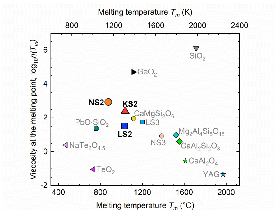
Figure 27 Correlation between melting temperatures T_m and viscosity at T_m \log_{10}\eta(T_m) for a range of representative glass-forming melts, based on viscosity data from this work (LS2, NS2 and KS2) and reliable literature sources (see related text for references).
