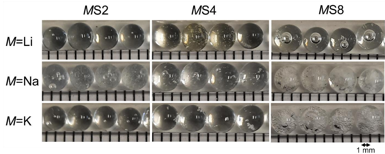
Figure 24 Pictures of beads synthesized by ADL. Visible influence of silica content and different alkali oxides. The distance between the vertical black bars is 1 mm.
