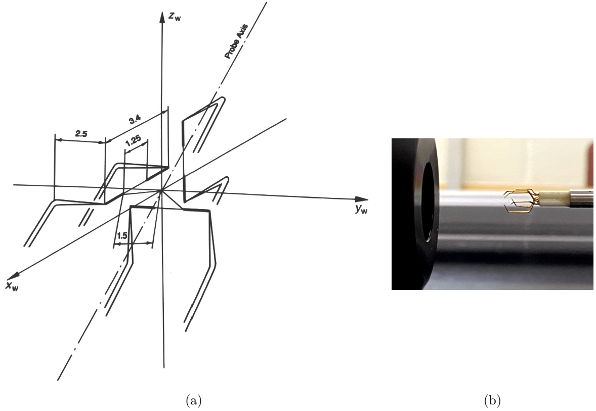
Figure 3.14: Schematic diagram showing (a) the wire and prong configuration of the DAN-TEC 55P91 claw-type three-wire probe (taken from Bruun (1996)) and (b) The probe during the velocity calibration process. The dimensions are depicted in millimetres.
