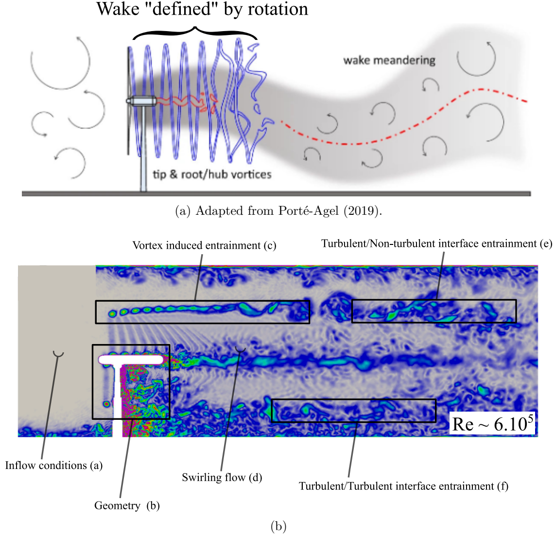
Figure 1.15: Schematic diagram showing (a) an instantaneous HAWT wake and (b) the different physical processes involved in the wake of a HAWT. LES flow visualisation taken from B  nard et al. (2018), showing iso-contours of the norm of vorticity.
