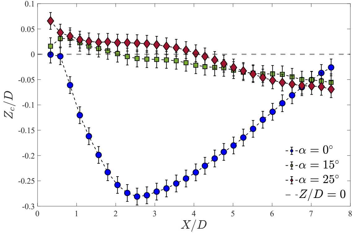
Figure 4.17: Streamwise evolution of the mean wake centre vertical coordinate \overline{Z_c}(x)/D for \alpha = [0^\circ, 15^\circ, 25^\circ] . Only 1/15 of the markers are plotted for visibility. The error bars are the PIV spatial resolution (chapter 3 §3.5.3).
