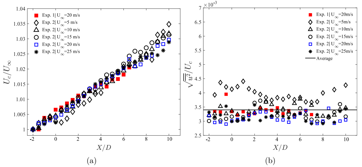
Figure 3.9: Centreline ( z = y = 0 ) streamwise evolution of (a) the mean streamwise velocity U_c(x) and of (b) the turbulence intensity \sqrt{u^2}/U_c for the empty test section.
