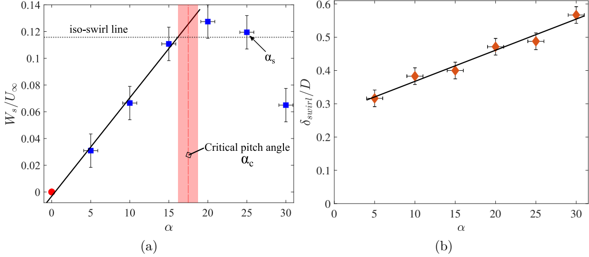
Figure 4.5: (a) Peak-to-peak swirling velocity W_s/U_\infty and (b) swirling length \delta_{swirl}/D as a function of the pitch angle \alpha evaluated at X = 6D .
