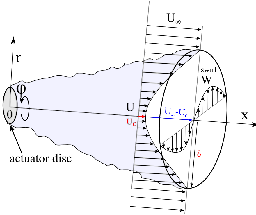
Figure 2.1: Schematic of an axisymmetric swirling wake generated by an actuator disc in the cylindrical coordinates (x, r, \phi) . The origin is set at the centre of the actuator disc. U and W are the mean axial and azimuthal velocity components, respectively. U_\infty is the streamwise undisturbed free-stream velocity, U_c is the wake streamwise centreline velocity, and \delta is the wake width.
