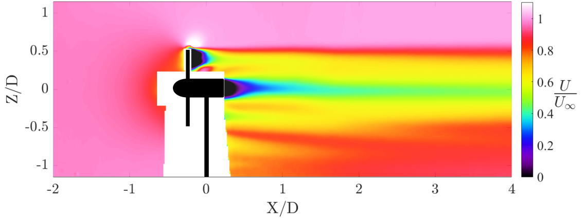
Figure 6.4: Normalised mean streamwise velocity fields U/U_\infty of the test rig with a bluff body-like nacelle.
