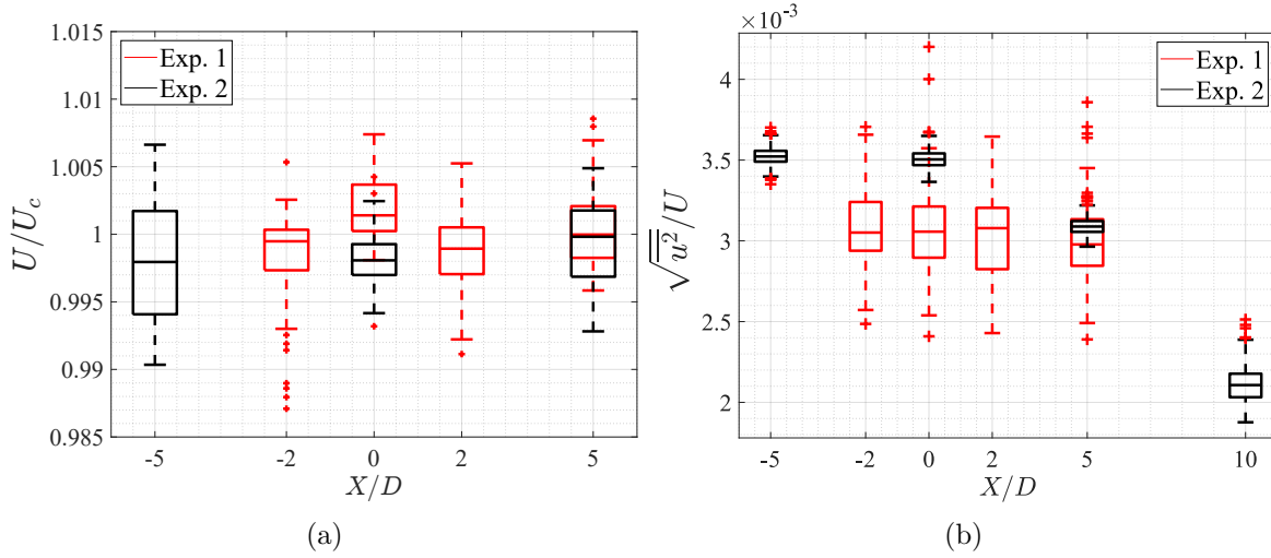
Figure 3.10: Cross-sectional spatial statistics at different streamwise locations of (a) the normalised mean streamwise velocity U/U_c and (b) the turbulence intensity \sqrt{u^2}/U .
