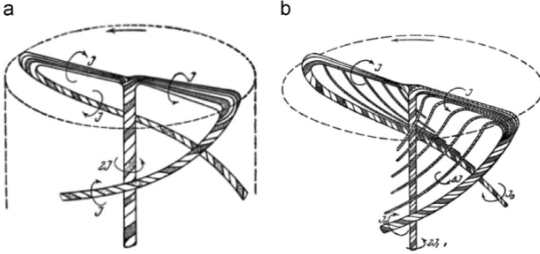
Figure 1.18: The original diagrams of screw vortex system with circulation distributions by (a) Joukowski (1912) and (b) Vetchinkin (1913). Taken from the review paper of Okulov et al. (2015) on the rotor theories of Professor Joukowski.
