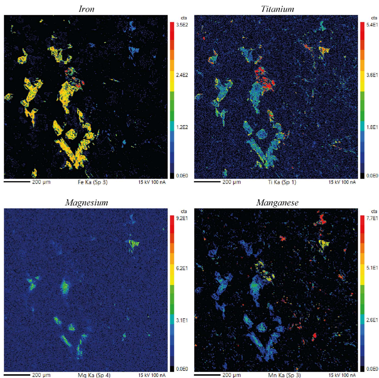
Figure A5. WDS mapping for 10 elements on thin section SA4 (near SA3; Western margin). Maps of aluminum, silicium, sodium and chlorine reveal the presence of feldspathoids. In particular, the sodium and chlorine maps allow distinguish between nepheline and sodalite, the latter being richer in sodium and containing chlorine. The potassium map reveals the presence of alkali feldspars. Calcium, iron and magnesium maps reveal the presence of aegirine. The titanium and iron maps, reveal aenigmatite.
