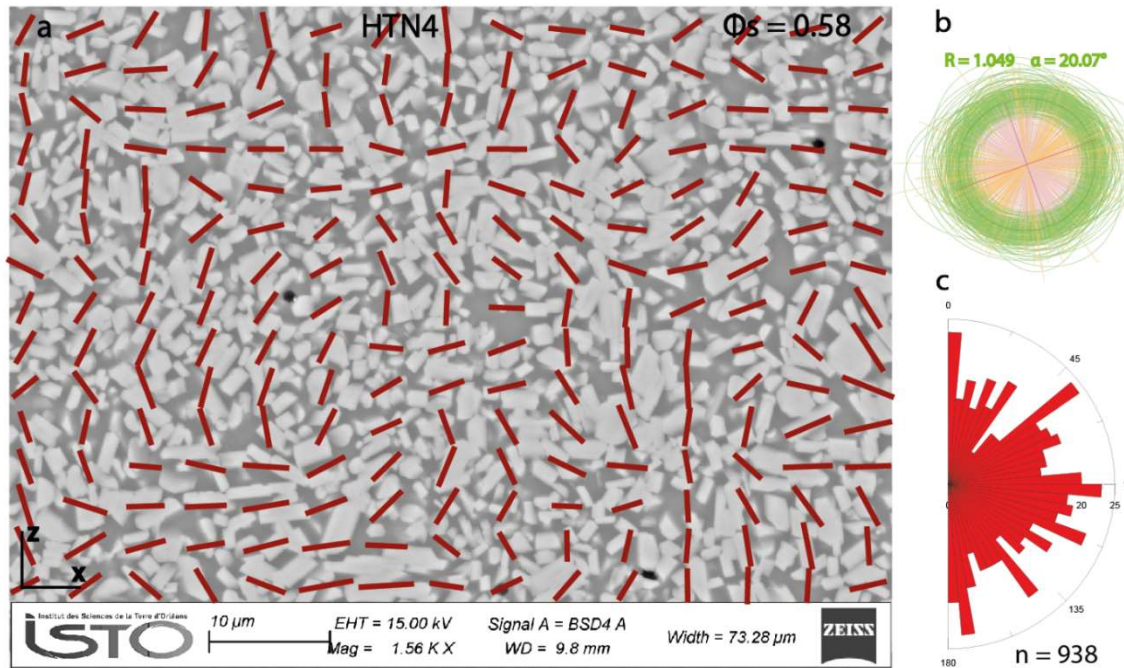
Figure III.17. Determination of textures for HTN4 sample. SEM image in backscattered electrons. (b) Local tensor ellipses of shape fabric. c) Rose of the directions of the long axes of local shape fabric ellipses. n = number of measures.
