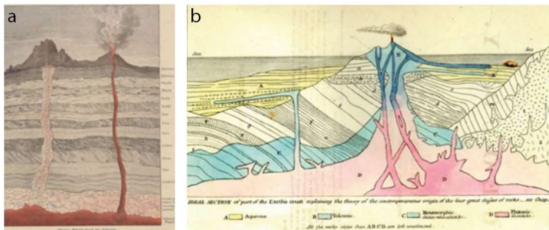
Figure I.1. a) An idealized section of earth's crust, from Emile with "L'Ecorce terrestre" (1874), showing the stratigraphic order of the sediments deposited during various geological epochs. From https://blogs.scientificamerican.com/history-of-geology/granite-wars-episode-i-fire-water . b): Frontispiece of (Lyell, 1838). The ideal section of the Earth crust by Charles Lyell (1797-1875), Student of James Hutton, showing the -modern – concept of magma storage at depth, magma transfer and emplacement at the surface.
