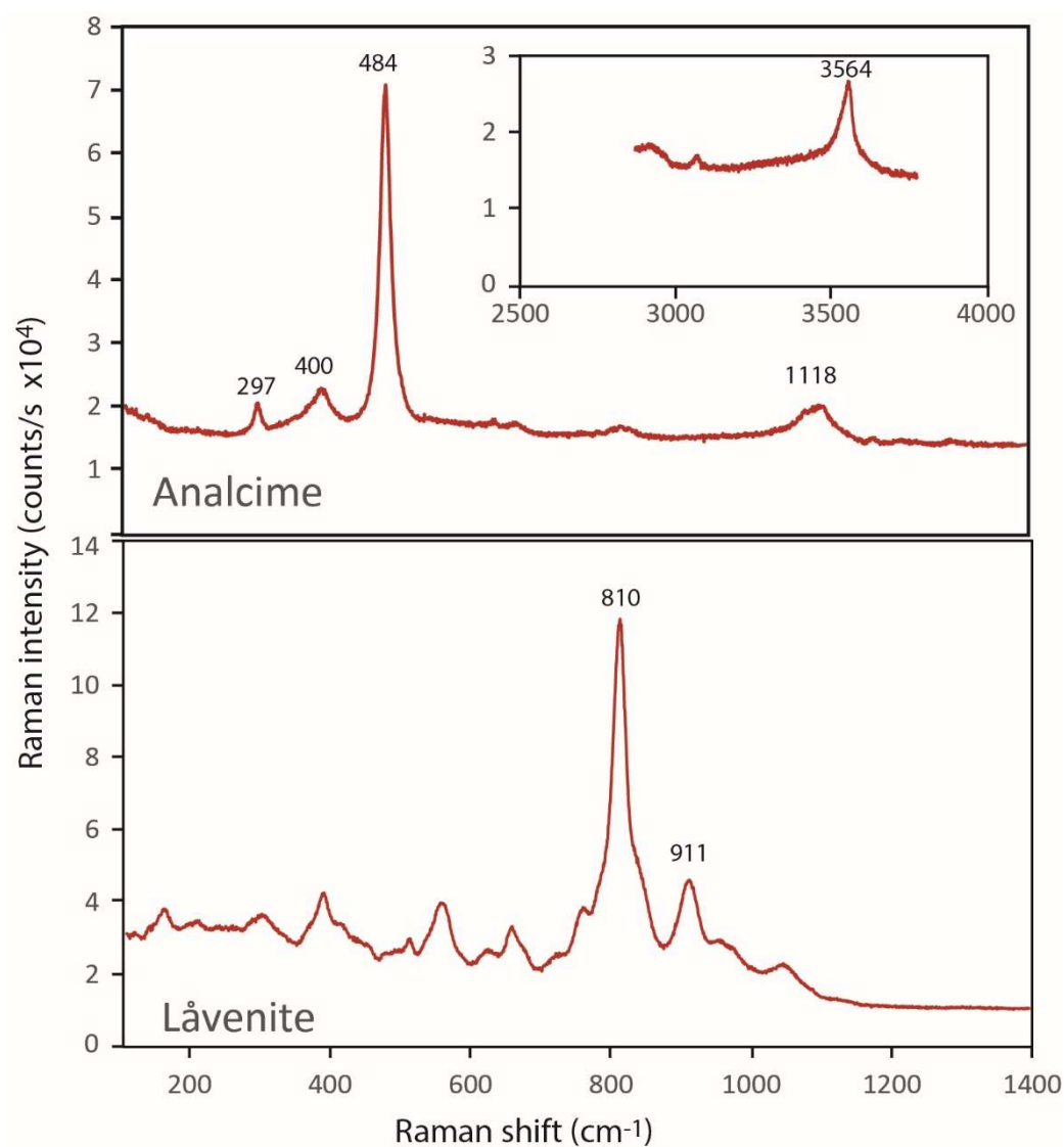
Figure A7. Raman spectra of analcime and lāvenite measured in SA3 (see location in Fig. 14a).
