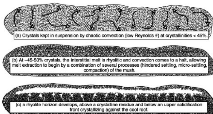
Figure I.8. Schematic illustration of the melt expulsion model for the generation of crystal-poor rhyolites (Bachmann and Bergantz, 2004).
