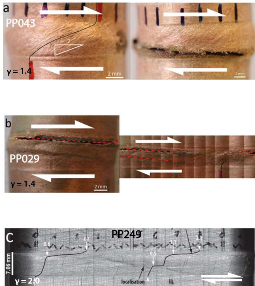
Figure IV.1. Panoramic reconstruction of the samples still embebbed in their copper jacket subject to torsion deformation. a) PP043, b) PP029, c) PP249. Deformation rates (black line) are indicated on each image. Modified from (Laumonier, 2013; Picard et al., 2011).
