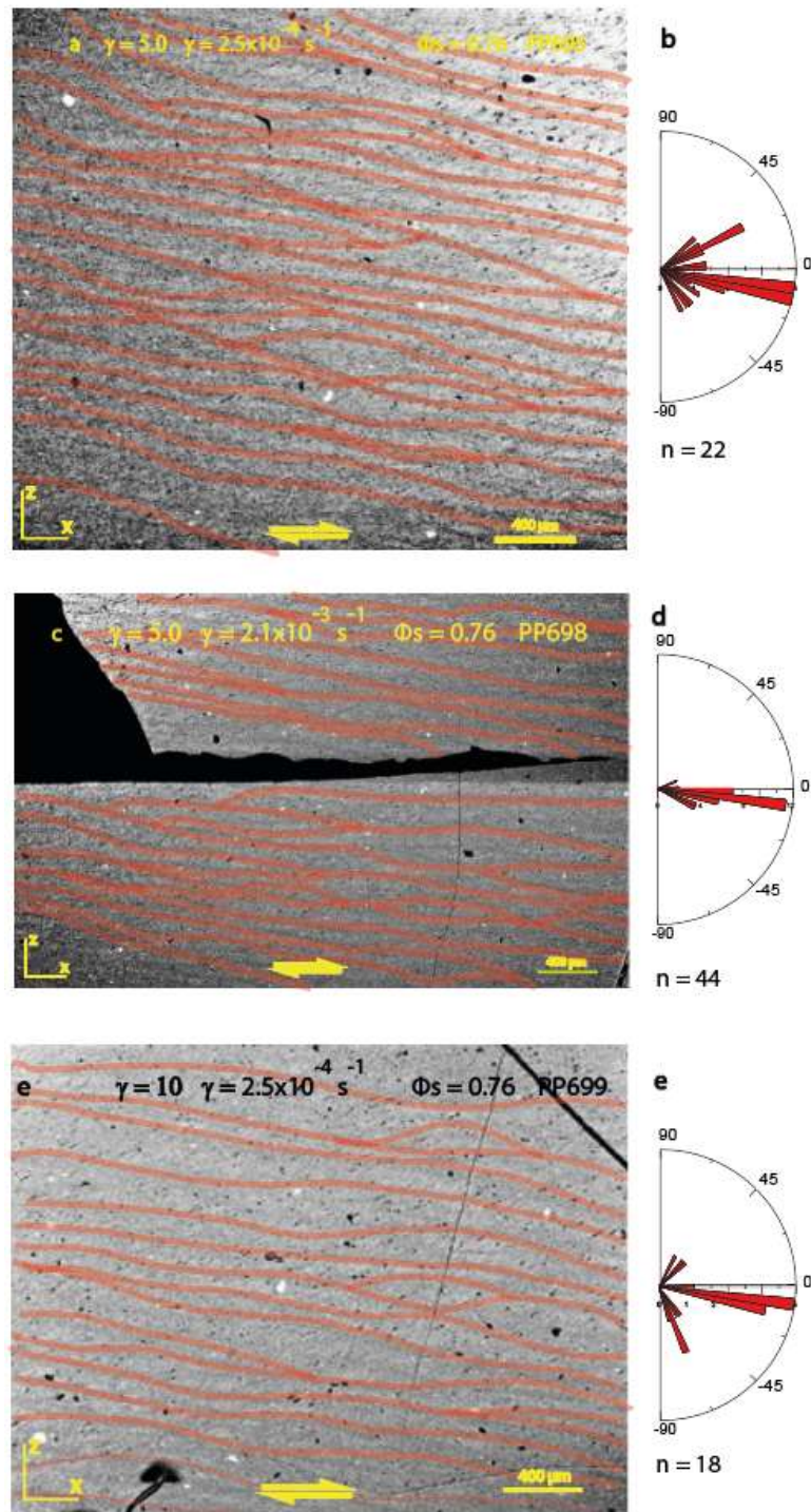
Figure VI.7. SEM images of all samples showing banding. The development of banding is highlighted by the red lines. a) SEM image of sample PP695, b) rose diagram of long axes of local tensor ellipses of sample PP695, c) SEM image of sample PP698, d) rose diagram of long axes of local tensor ellipses of sample PP698, e) SEM image of sample PP699, f) rose diagram of long axes of local tensor ellipses of sample PP699. n = numbr of measures.
