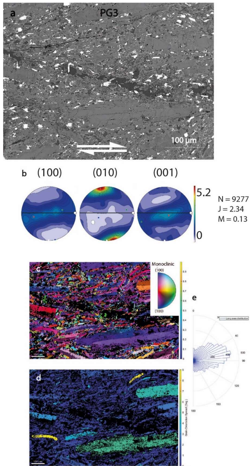
Figure VIII.10. a) SEM image of the natural sample PG3. b) Pole figures. c) Inverse pole figure map. d) Grain orientation spread map. e) Long axis orientation rose of the plagioclase.
