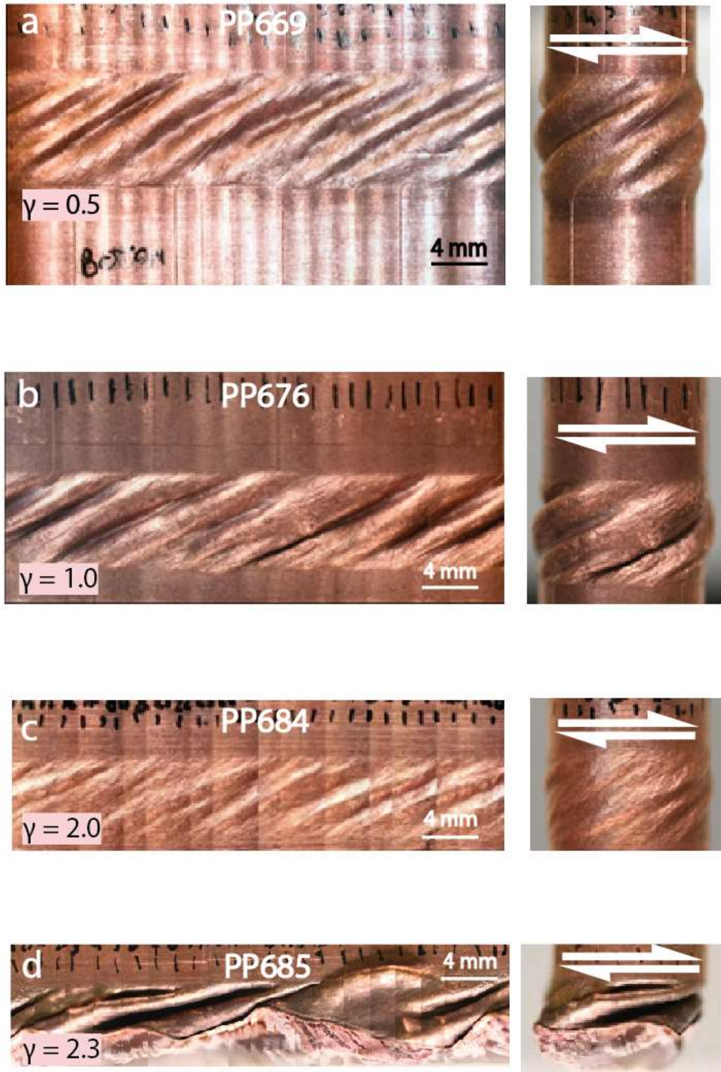
Figure V.1. Panoramic reconstruction of the samples still embebbed in their copper jacket subject to torsion deformation. a) PP669 ( \phi_s = 0.58 , \gamma = 0.5 , \dot{\gamma} = 1.0 \cdot 10^{-4} ), b) PP676 ( \phi_s = 0.58 , \gamma = 1.0 , \dot{\gamma} = 1.0 \cdot 10^{-4} ), c) PP684 ( \phi_s = 0.59 , \gamma = 2.0 , \dot{\gamma} = 2.1 \cdot 10^{-3} ), d) PP685 ( \phi_s = 0.59 , \gamma = 2.3 , \dot{\gamma} = 1.0 \cdot 10^{-4} ).
