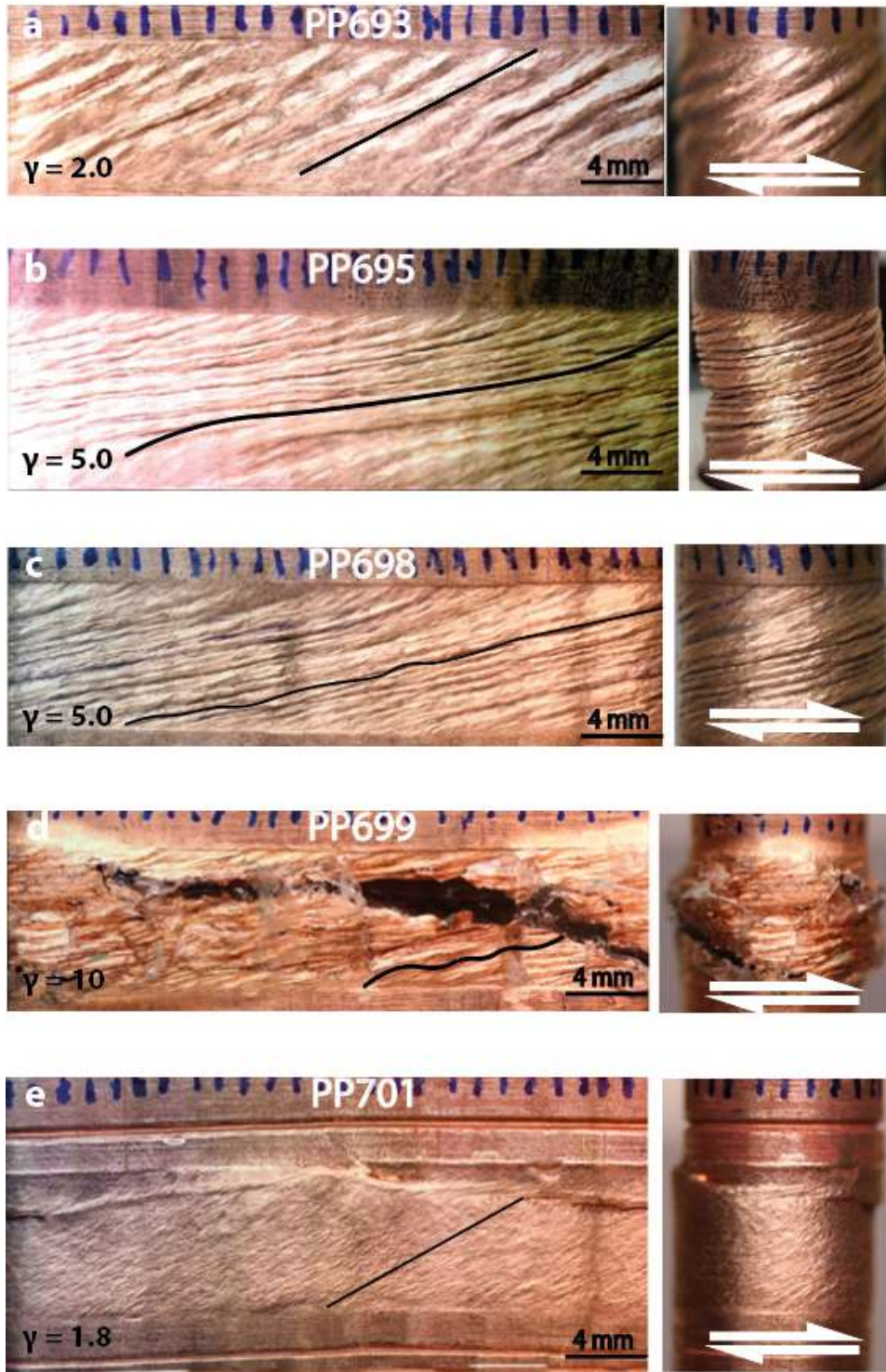
Figure VI.1. Panoramic reconstruction of the samples still embbeded in their copper jacket subject to torsion deformation. a) PP693 ( \phi_s = 0.73 \gamma = 2.0 , \dot{\gamma} = 2.5 \cdot 10^{-4} ) b) PP695( \phi_s = 0.76 , \gamma = 5.0 , \dot{\gamma} = 2.5 \cdot 10^{-4} ), c) PP698( \phi_s = 0.76 , \gamma = 5.0 , \dot{\gamma} = 1.0 \cdot 10^{-3} ), d) PP699 ( \phi_s = 0.76 \gamma = 10.0 , \dot{\gamma} = 2.5 \cdot 10^{-4} ), e) PP701 ( \phi_s \approx 0.95 , \gamma = 1.8 , \dot{\gamma} = 5.0 \cdot 10^{-5} ). The deformation is highlighted but the black line.
