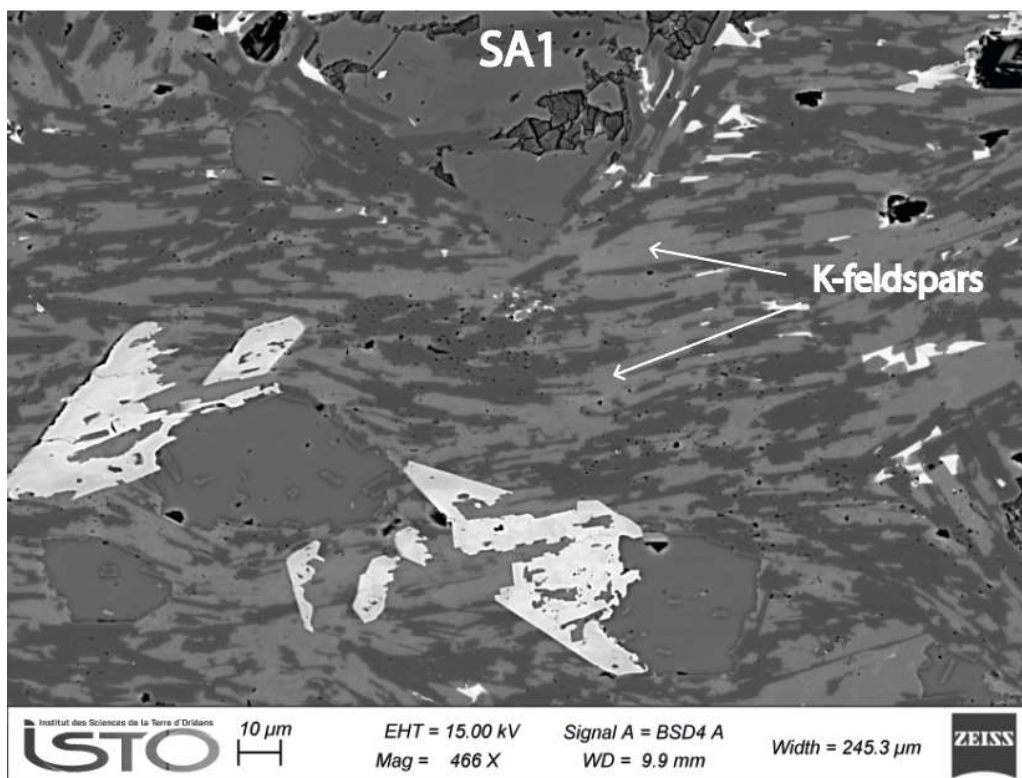
Figure VII.30. SEM picture of SA1 sample. The k-feldspars are in light grey.
