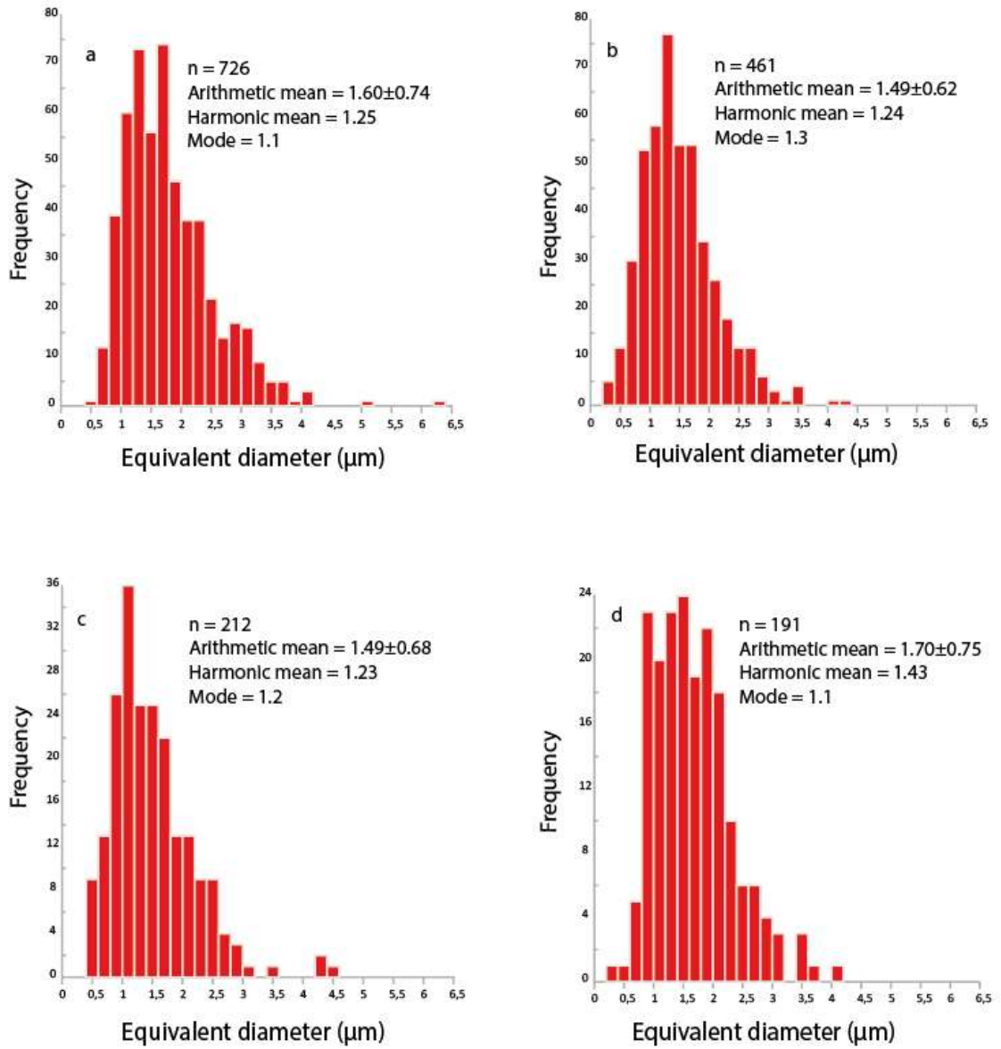
Figure VI.2. Histograms of equivalent diameters calculated in groups of crystals in deformation experiments. a) PP693 ( \phi_s = 0.73 , \gamma = 2.0 , \dot{\gamma} = 2.5 \times 10^{-4} ) b) PP695 ( \phi_s = 0.76 , \gamma = 5.0 , \dot{\gamma} = 2.5 \times 10^{-4} ), c) PP698 ( \phi_s = 0.76 , \gamma = 5.0 , \dot{\gamma} = 1.0 \times 10^{-3} ), d) PP699 ( \phi_s = 0.76 , \gamma = 10.0 , \dot{\gamma} = 2.5 \times 10^{-4} ).
