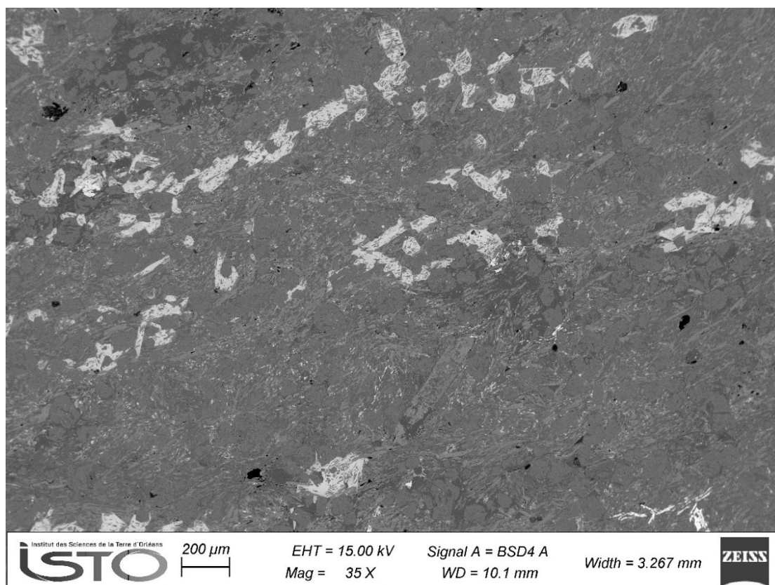
Figure VII.14. Backscattered electron image of the banded tinguaite facies few meters away from the western margin of the Suc de Sara (SA4 sample).
