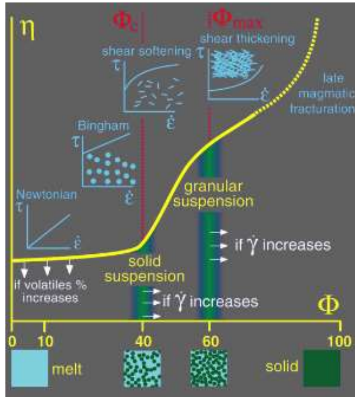
Figure I.19. General model of magma rheology. At low crystal contents, the suspension has Newtonian behaviour and moves by fluctuation and convection. At crystal contents between 40% and 60% a solid suspension forms, with shear softening behaviour if deformation is applied. At crystal contents of around 60%, the suspension is granular and the behaviour is shear thickening. At crystall contents above 70%, deformation results in the formation of late magmatic fracturation. (Arbaret 2021, unpublished).
