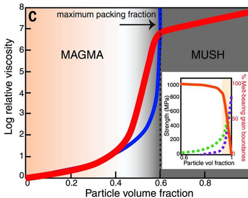
Figure I.3. Limit between magma and mush as function of particle volume fraction and viscosity. The inset shows the correlation between mush strength and particle volume fraction (from Cashmann et al., 2017).
