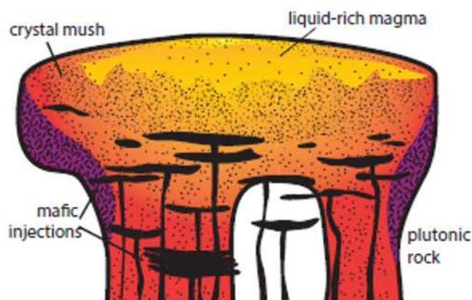
Figure I.2. Schematic diagram illustrating a crystal-mush dominated reservoir. Modified from Hildreth and Wilson (2007).
