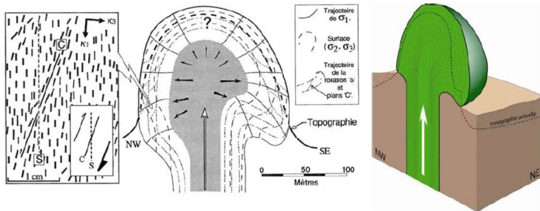
Figure VII.3. Left: local rearrangement of feldspar crystals on the C plane crosscutting the S foliation plane. Centre: schematic section NW – SE showing the radial disposition of the C microbands reorganising the mineral foliation S. Right: Formation of phonolitic extrusion Gouleiou (modified from (Arbaret et al., 1993)).
