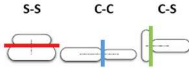
Figure V.13. Principal contact modes: side-side (s-s), cap-cap (c-c), cap-side (c-s). Modified from (Azema and Radjaï, 2012).
