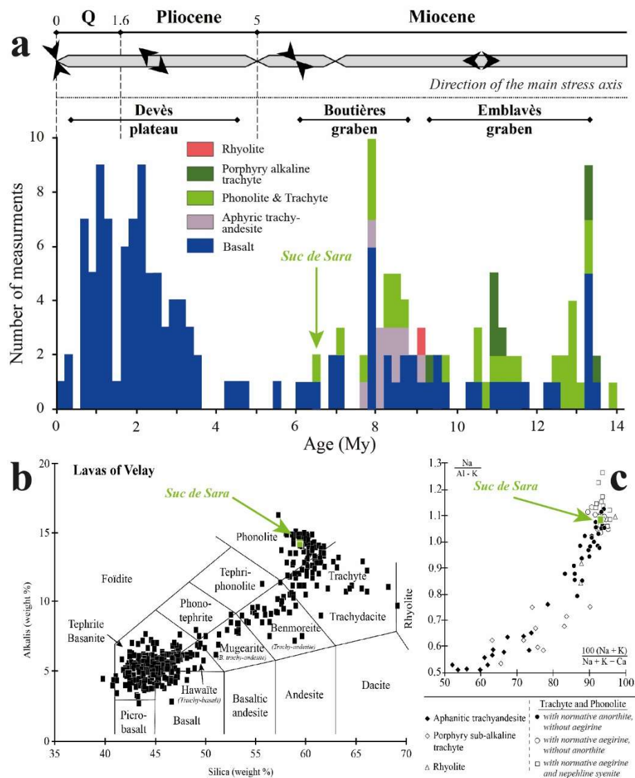
Figure 2. a – Histogram summarizing the number of geochronological ages of volcanic edifices in the Velay massif according to their composition (modified after Mergoil and Boivin, 1993) and direction of the main constraints represented by the black arrows (modified after Blès et al., 1989). The 6.5 Ma old Suc de Sara represents the youngest phonolitic edifice. b – TAS diagram (Le Bas et al., 1986) of the Velay alkaline series (modified after Mergoil and Boivin, 1993). c – Peralkalinity diagram for differentiated products from the Velay province (modified after Mergoil and Boivin, 1993).
