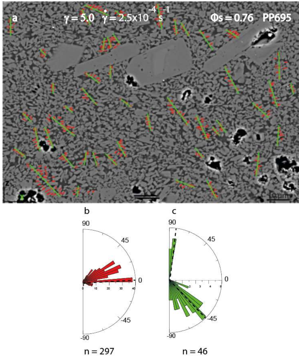
Figure VI.40. a) SEM image of sample PP695 with hand-drawn orientation of the clusters. b) Rose diagram of orientation of the contacts in the clusters, c) rose diagram of the preferred orientations of the clusters.
