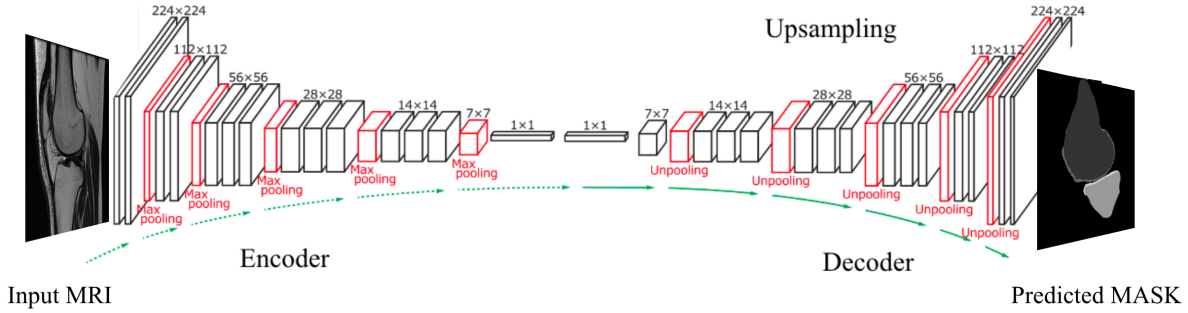
Figure 3.2: Generic overview of image MRI segmentation pipeline.
