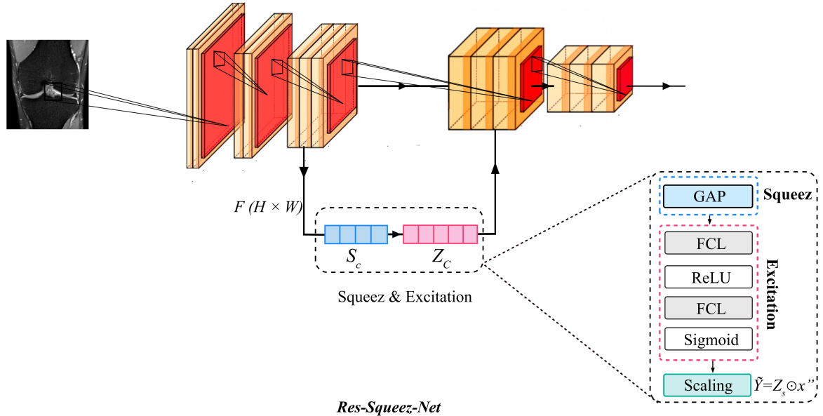
Figure 6.2: Proposed Res-Squeeze-Net model. The figure delineates the Squeeze and Excitation operations within convolutional layers.
