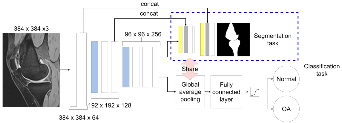
Figure 7.2: Architecture of the proposed method (Model B) that incorporates mask segmentation as an auxiliary task.
